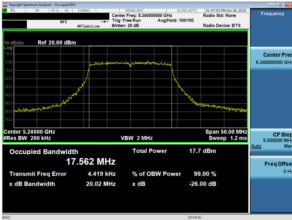
Plot 7-61. 26dB Bandwidth Plot MIMO ANT2 (802.11n – 20MHz BW (UNII Band 1) – Ch. 48)
