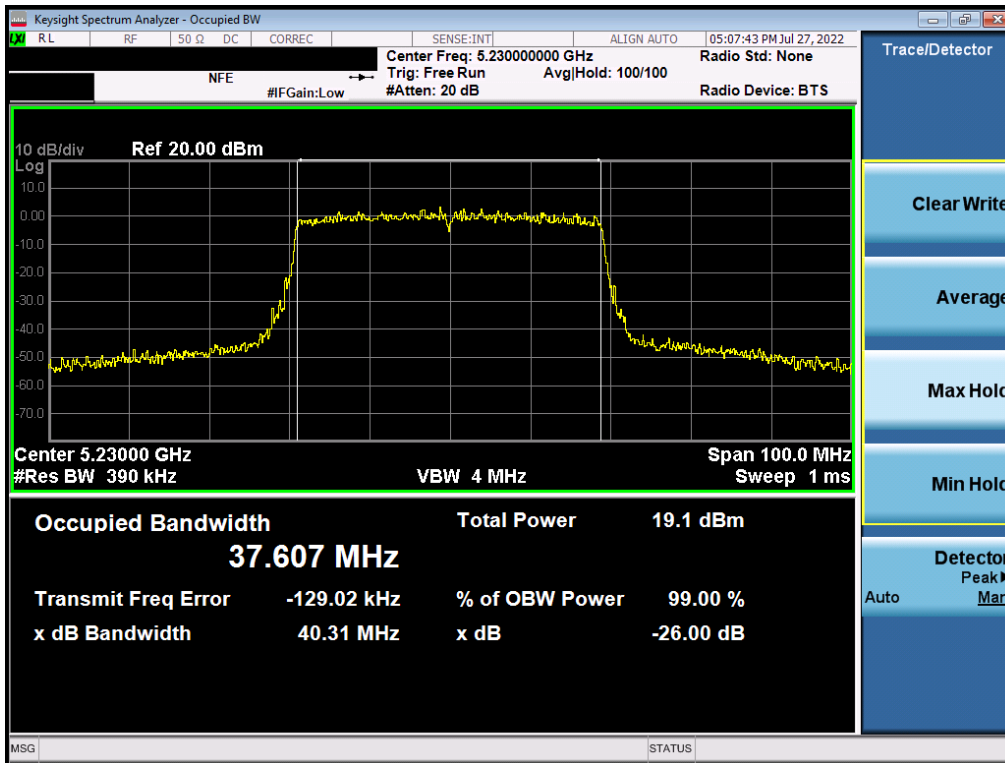
Plot 7-68. 26dB Bandwidth Plot MIMO ANT2 (802.11ax – 40MHz BW (UNII Band 1) – Ch. 46)
