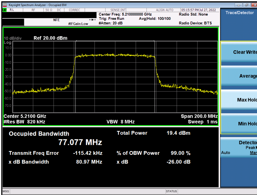
Plot 7-70. 26dB Bandwidth Plot MIMO ANT2 (802.11ax – 80MHz BW (UNII Band 1) – Ch. 42)
