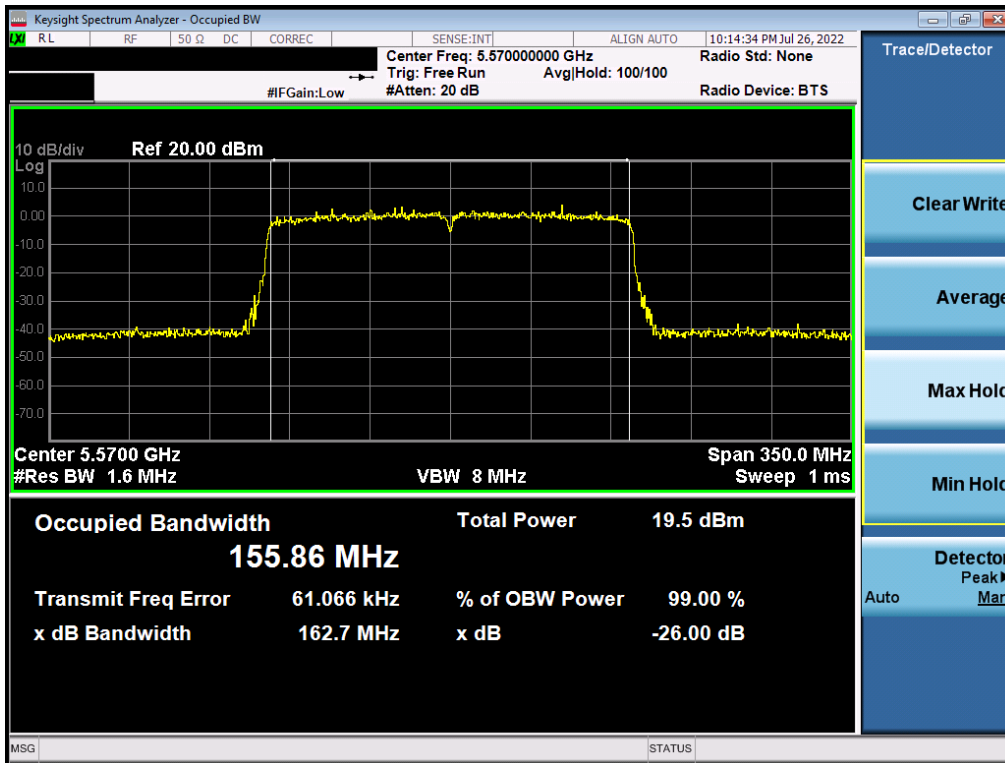
Plot 7-55. 26dB Bandwidth Plot MIMO ANT1 (802.11ax – 160MHz BW (UNII Band 2C) – Ch. 114)
