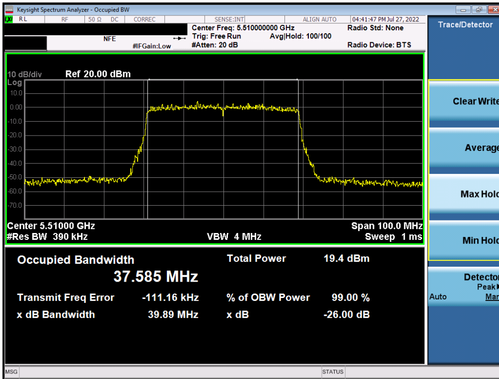
Plot 7-45. 26dB Bandwidth Plot MIMO ANT1 (802.11ax – 40MHz BW (UNII Band 2C) – Ch. 102)
