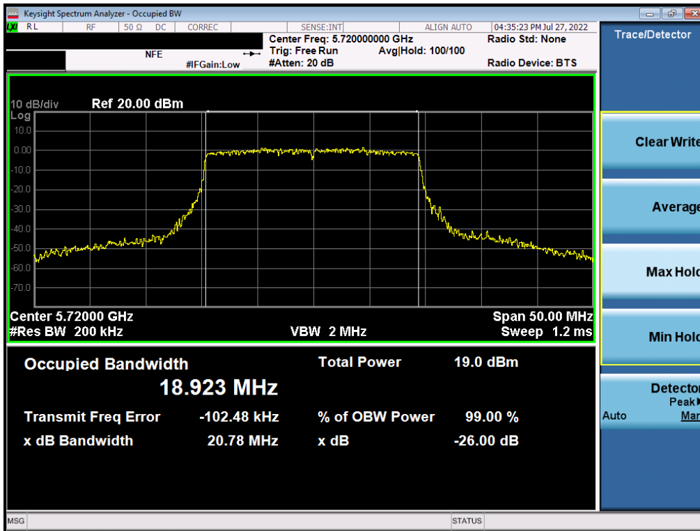
Plot 7-41. 26dB Bandwidth Plot MIMO ANT1 (802.11ax – 20MHz BW (UNII Band 2C) – Ch. 144)
