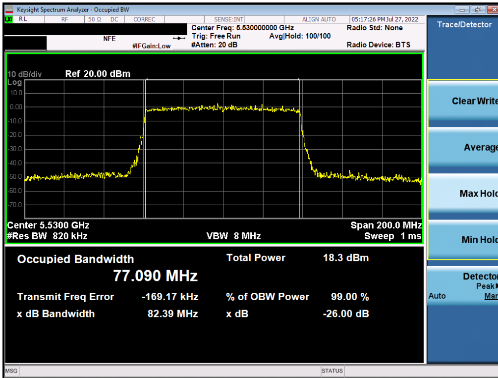
Plot 7-106. 26dB Bandwidth Plot MIMO ANT2 (802.11ax – 80MHz BW (UNII Band 2C) – Ch. 106)
