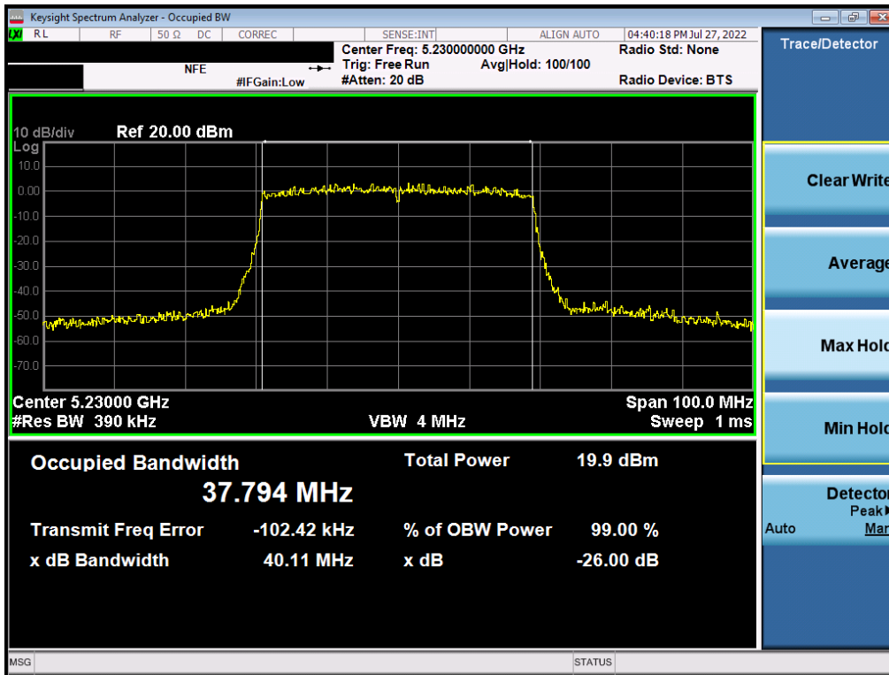
Plot 7-13. 26dB Bandwidth Plot MIMO ANT1 (802.11ax – 40MHz BW (UNII Band 1) – Ch. 46)
