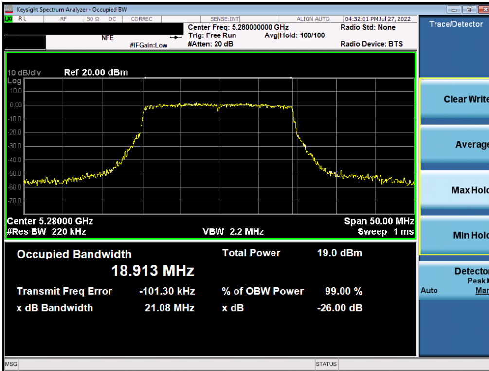
Plot 7-25. 26dB Bandwidth Plot MIMO ANT1 (802.11ax – 20MHz BW (UNII Band 2A) – Ch. 56)
