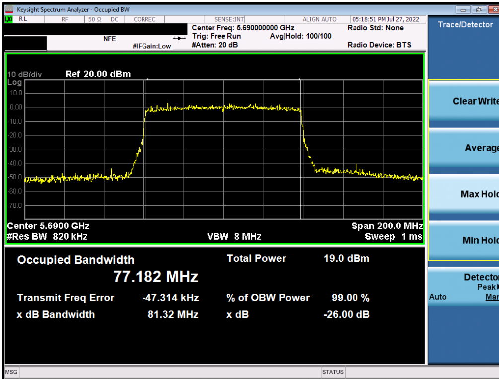
Plot 7-108. 26dB Bandwidth Plot MIMO ANT2 (802.11ax – 80MHz BW (UNII Band 2C) – Ch. 138)
