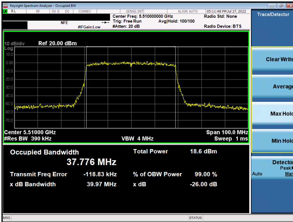
Plot 7-100. 26dB Bandwidth Plot MIMO ANT2 (802.11ax – 40MHz BW (UNII Band 2C) – Ch. 102)
