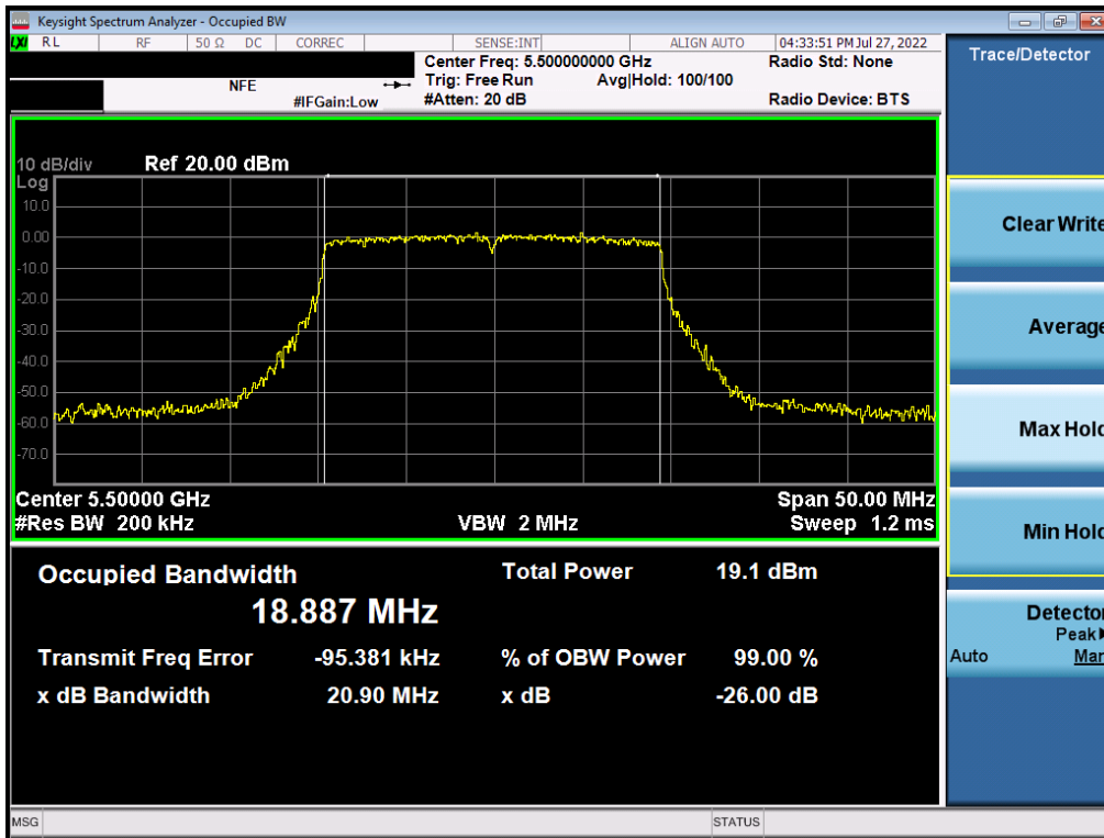
Plot 7-39. 26dB Bandwidth Plot MIMO ANT1 (802.11ax – 20MHz BW (UNII Band 2C) – Ch. 100)
