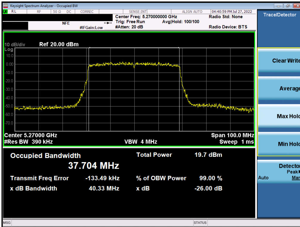
Plot 7-29. 26dB Bandwidth Plot MIMO ANT1 (802.11ax – 40MHz BW (UNII Band 2A) – Ch. 54)
