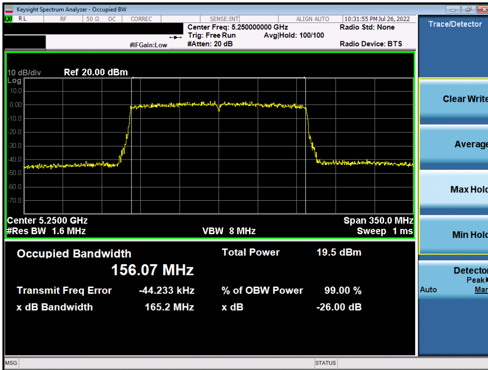
Plot 7-72. 26dB Bandwidth Plot MIMO ANT2 (802.11ax – 160MHz BW (UNII Band 1/2A) – Ch. 50)
