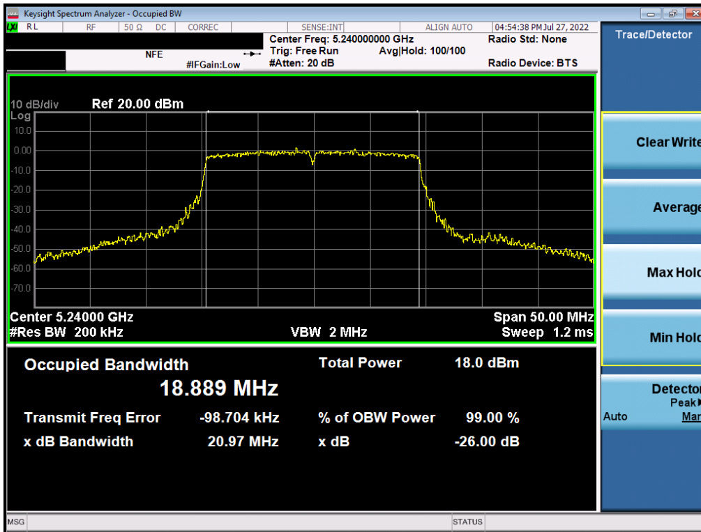
Plot 7-64. 26dB Bandwidth Plot MIMO ANT2 (802.11ax – 20MHz BW (UNII Band 1) – Ch. 48)
