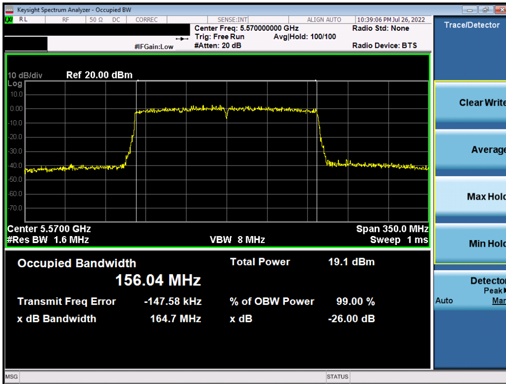
Plot 7-110. 26dB Bandwidth Plot MIMO ANT2 (802.11ax – 160MHz BW (UNII Band 2C) – Ch. 114)
