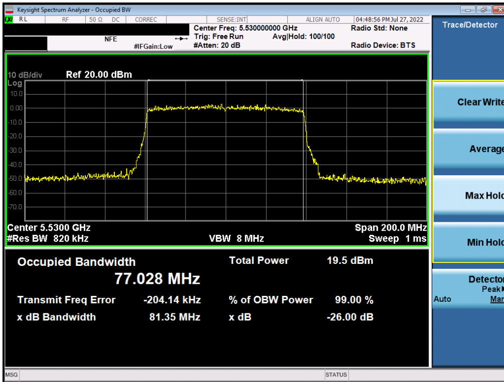
Plot 7-51. 26dB Bandwidth Plot MIMO ANT1 (802.11ax – 80MHz BW (UNII Band 2C) – Ch. 106)
