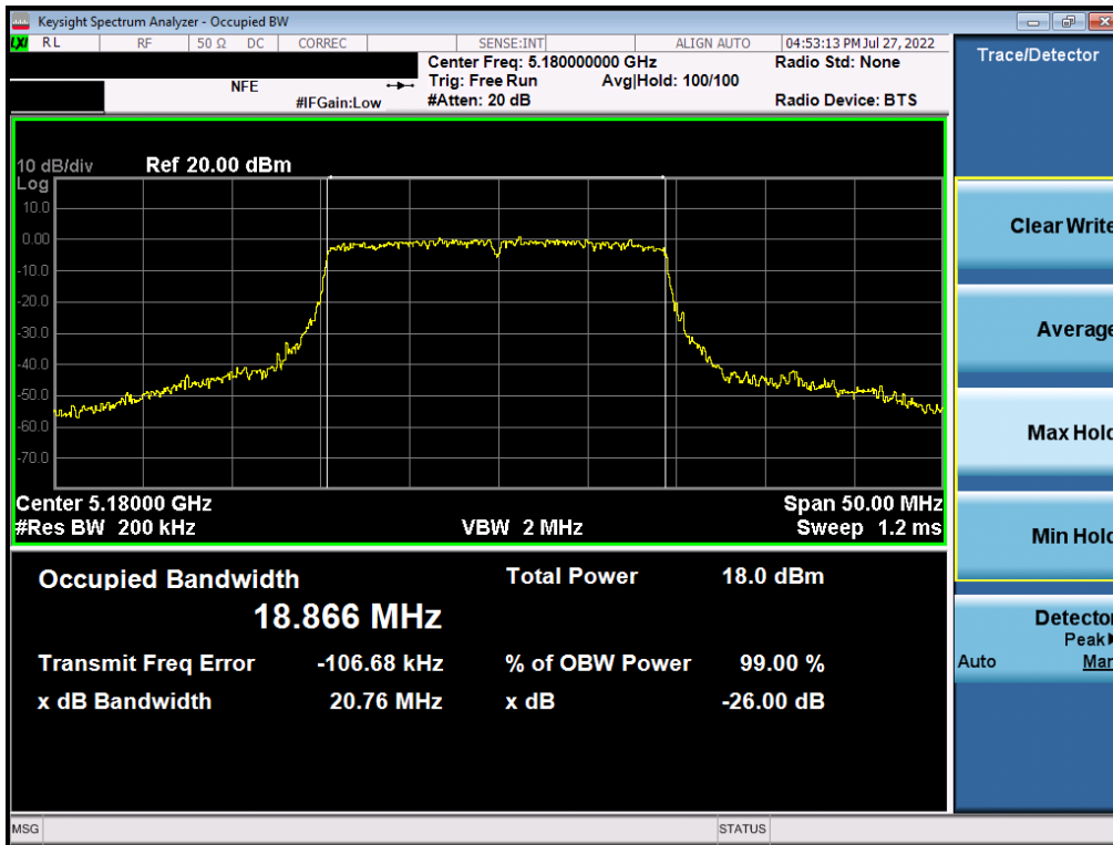
Plot 7-62. 26dB Bandwidth Plot MIMO ANT2 (802.11ax – 20MHz BW (UNII Band 1) – Ch. 36)
