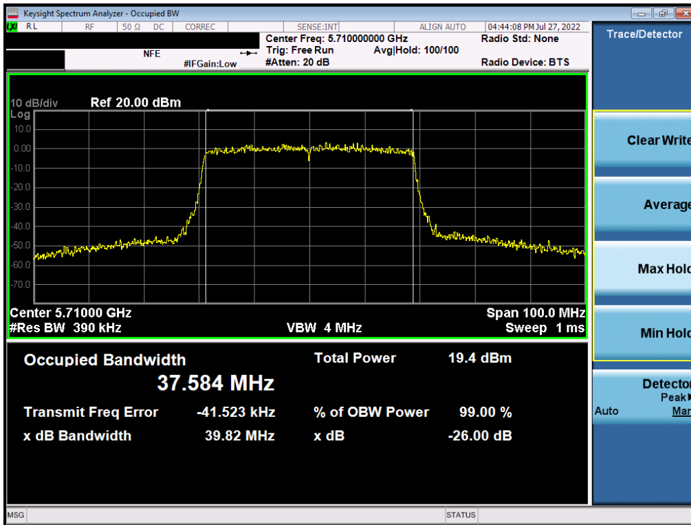
Plot 7-47. 26dB Bandwidth Plot MIMO ANT1 (802.11ax – 40MHz BW (UNII Band 2C) – Ch. 142)
