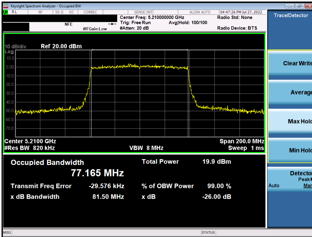
Plot 7-15. 26dB Bandwidth Plot MIMO ANT1 (802.11ax – 80MHz BW (UNII Band 1) – Ch. 42)
