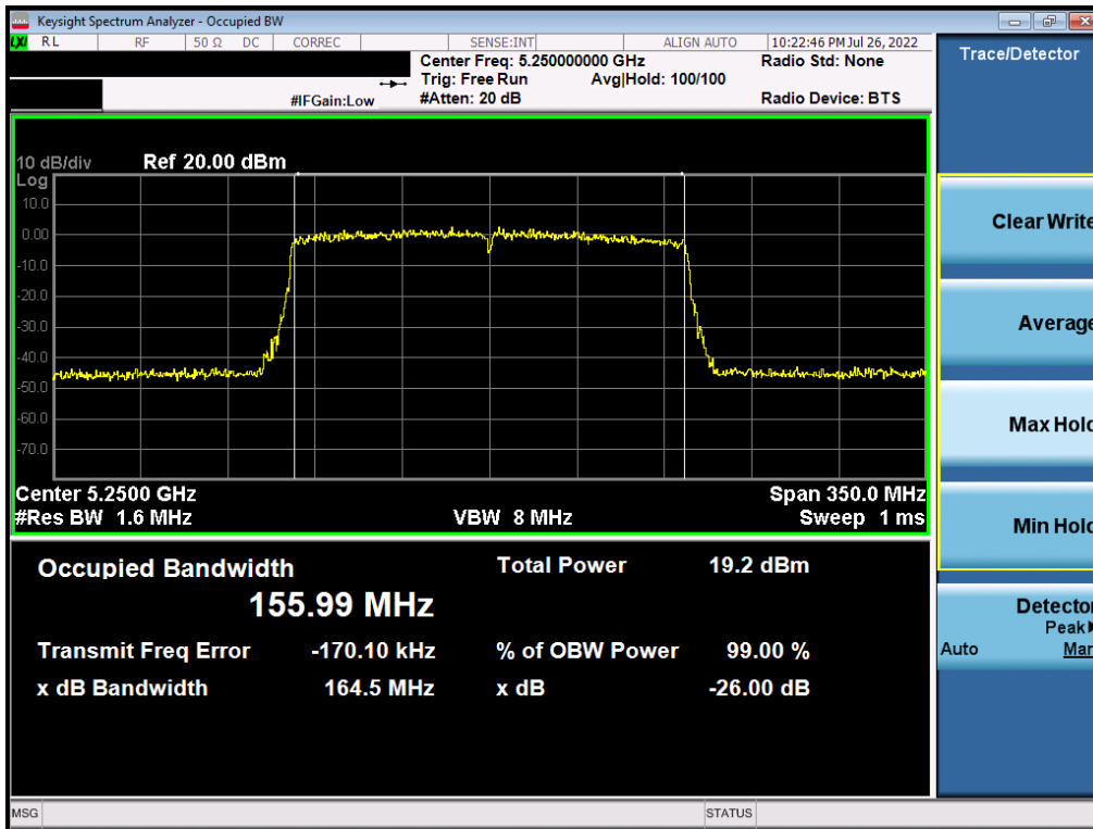
Plot 7-17. 26dB Bandwidth Plot MIMO ANT1 (802.11ax – 160MHz BW (UNII Band 1/2A) – Ch. 50)
