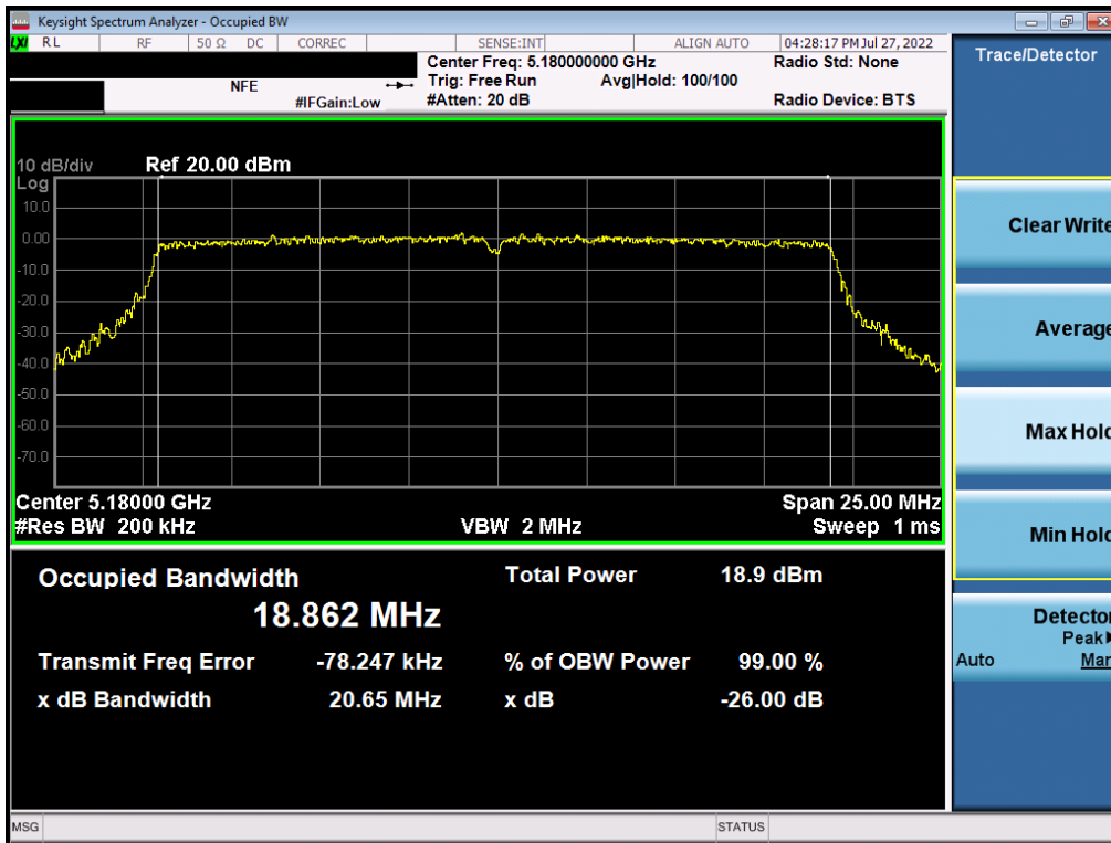
Plot 7-7. 26dB Bandwidth Plot MIMO ANT1 (802.11ax – 20MHz BW (UNII Band 1) – Ch. 36)
