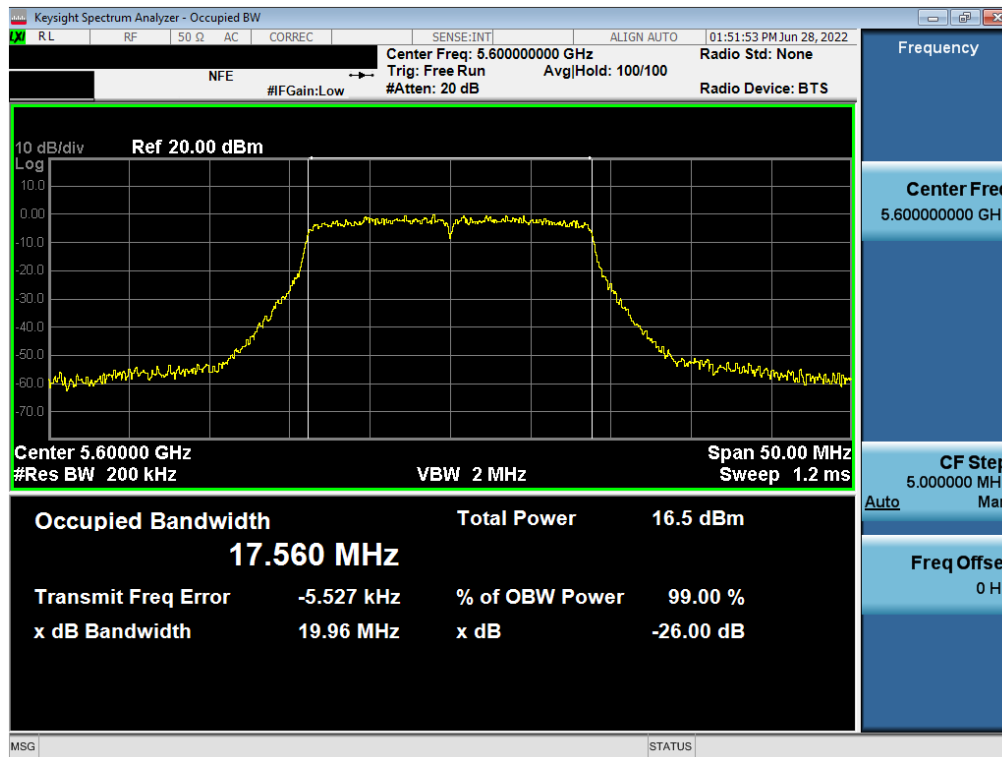
Plot 7-92. 26dB Bandwidth Plot MIMO ANT2 (802.11n – 20MHz BW (UNII Band 2C) – Ch. 120)
