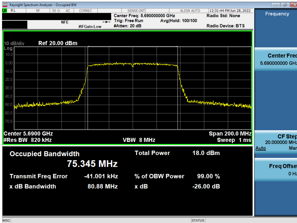
Plot 7-50. 26dB Bandwidth Plot MIMO ANT1 (802.11ac – 80MHz BW (UNII Band 2C) – Ch. 138)
