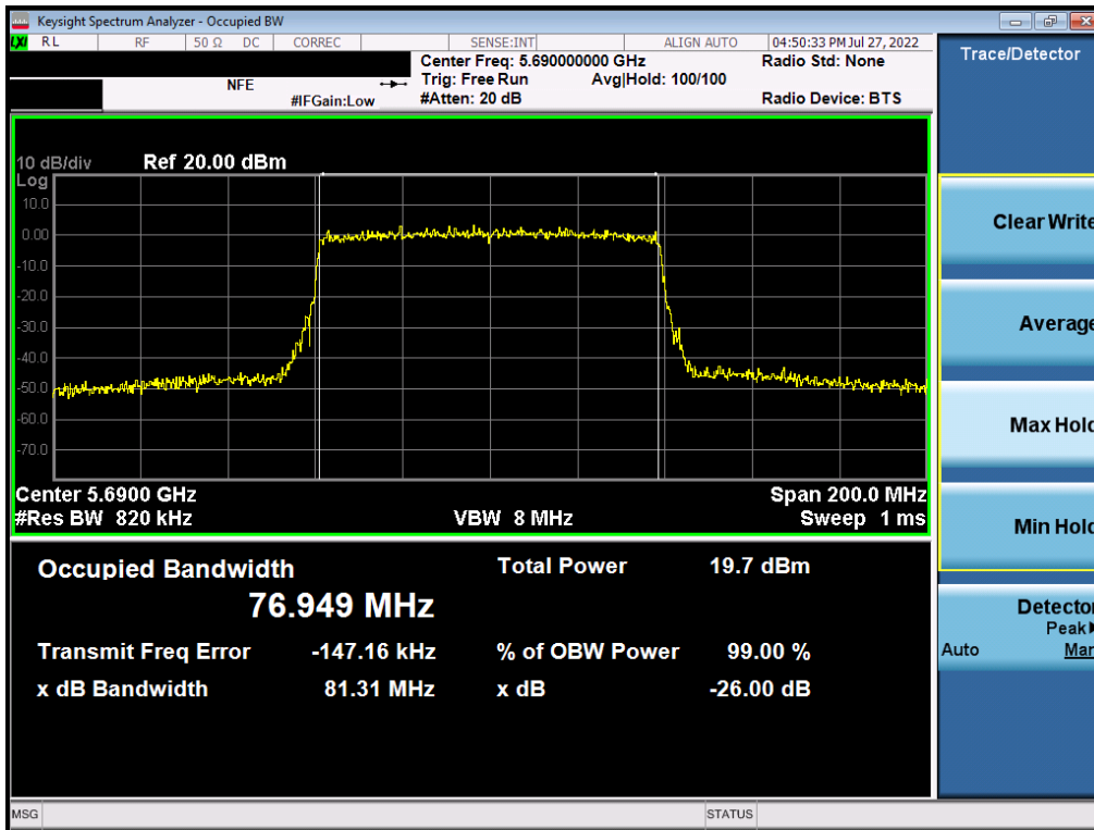
Plot 7-53. 26dB Bandwidth Plot MIMO ANT1 (802.11ax – 80MHz BW (UNII Band 2C) – Ch. 138)
