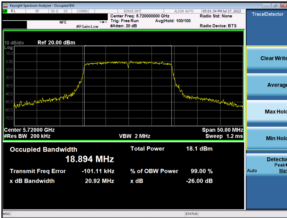
Plot 7-96. 26dB Bandwidth Plot MIMO ANT2 (802.11ax – 20MHz BW (UNII Band 2C) – Ch. 144)
