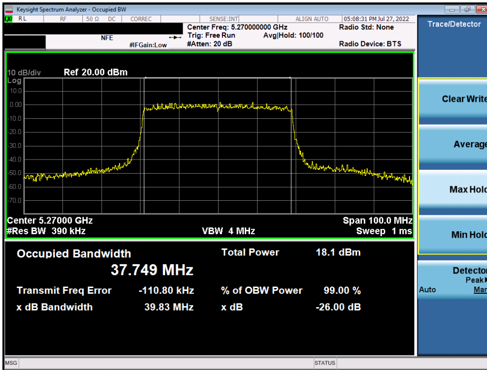
Plot 7-84. 26dB Bandwidth Plot MIMO ANT2 (802.11ax – 40MHz BW (UNII Band 2A) – Ch. 54)
