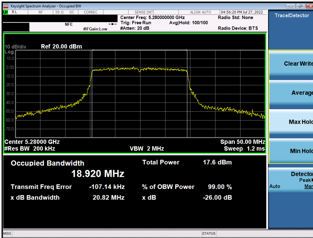
Plot 7-80. 26dB Bandwidth Plot MIMO ANT2 (802.11ax – 20MHz BW (UNII Band 2A) – Ch. 56)
