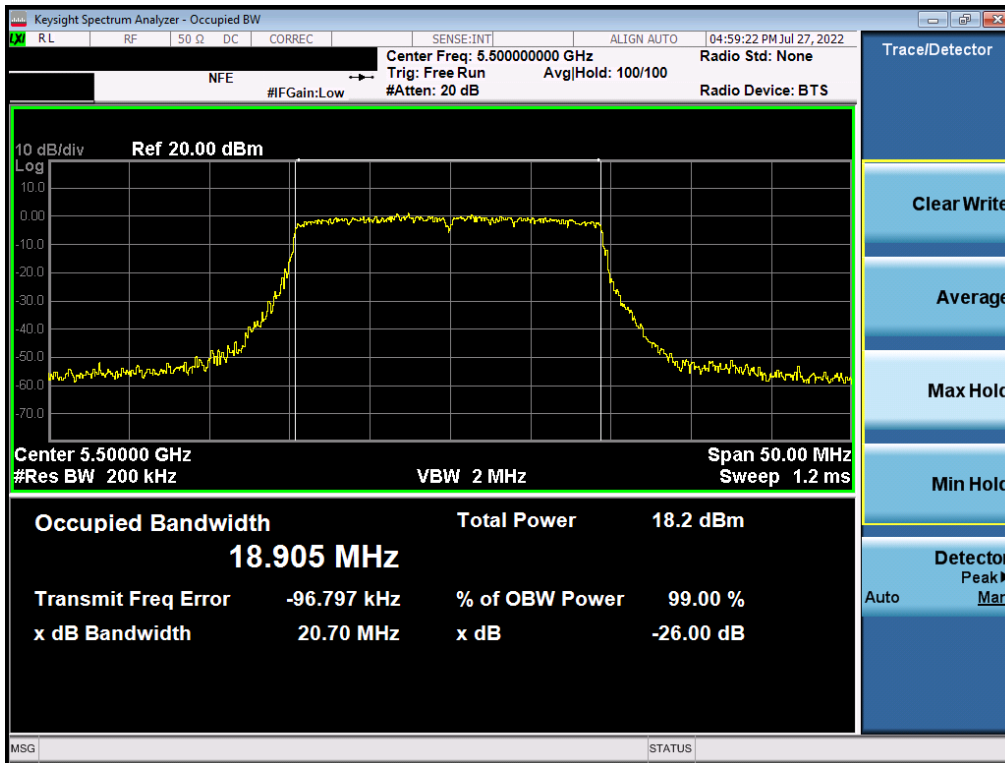
Plot 7-94. 26dB Bandwidth Plot MIMO ANT2 (802.11ax – 20MHz BW (UNII Band 2C) – Ch. 100)
