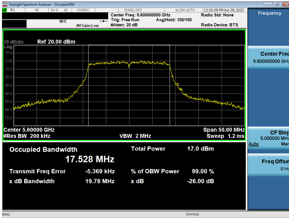
Plot 7-37. 26dB Bandwidth Plot MIMO ANT1 (802.11n – 20MHz BW (UNII Band 2C) – Ch. 120)
