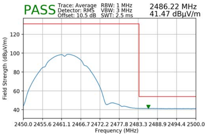
Plot 7-91. Radiated Restricted Upper Band Edge Measurement SISO ANT1 (Average)
