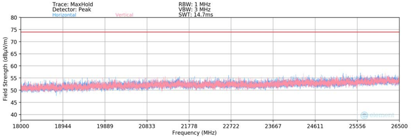
Plot 7-88. Radiated Spurious Plot above 18GHz MIMO/CDD
