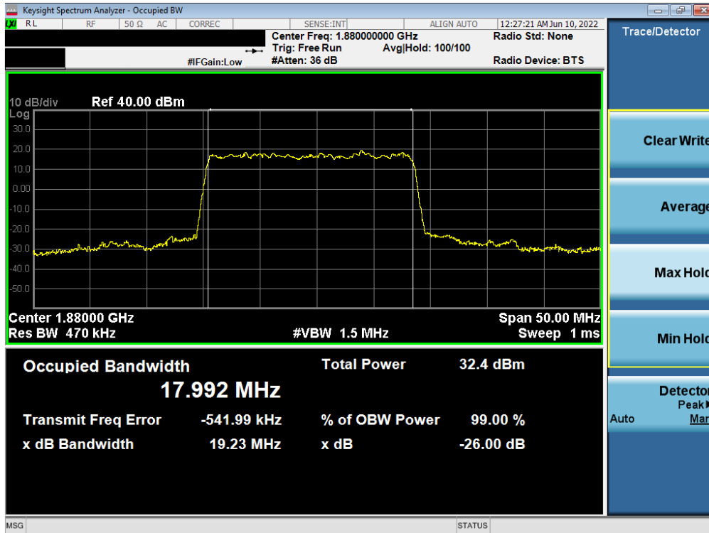
Plot 7-16. Occupied Bandwidth Plot (NR Band n2 - 20.0MHz DFT-s-OFDM BPSK - Full RB)
