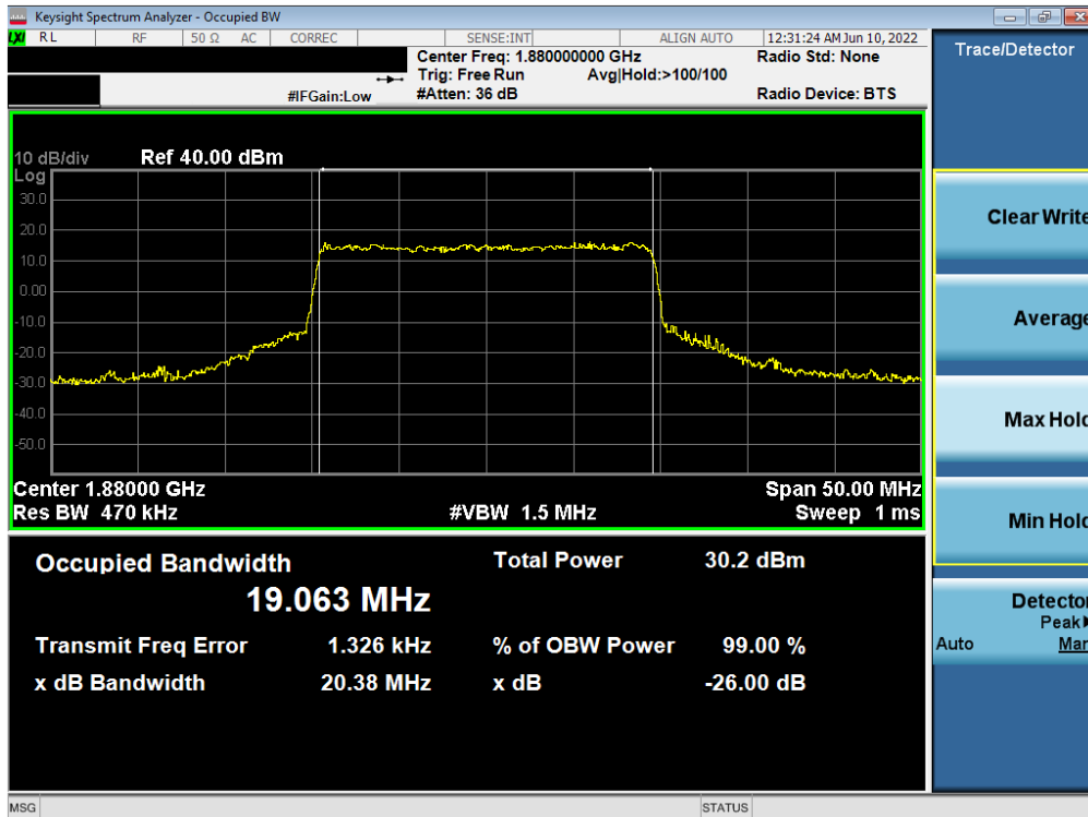
Plot 7-17. Occupied Bandwidth Plot (NR Band n2 - 20.0MHz CP-OFDM QPSK - Full RB)
