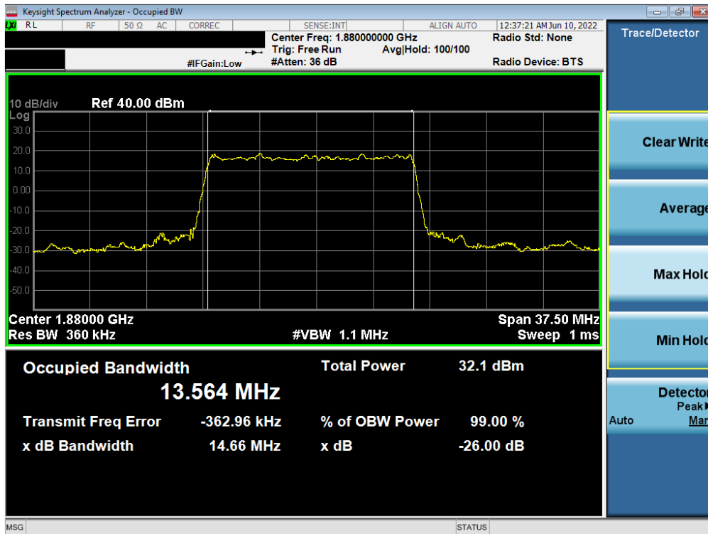
Plot 7-19. Occupied Bandwidth Plot (NR Band n2 - 15.0MHz DFT-s-OFDM BPSK - Full RB)
