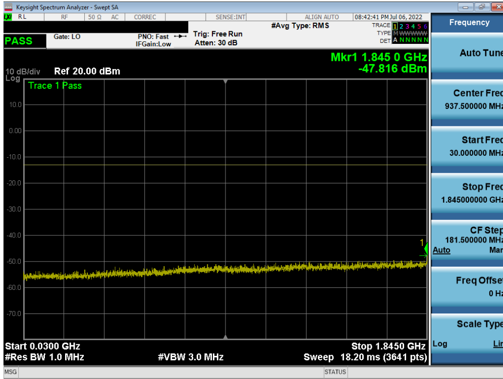
Plot 7-28. Conducted Spurious Plot (GPRS Ch. 512)
