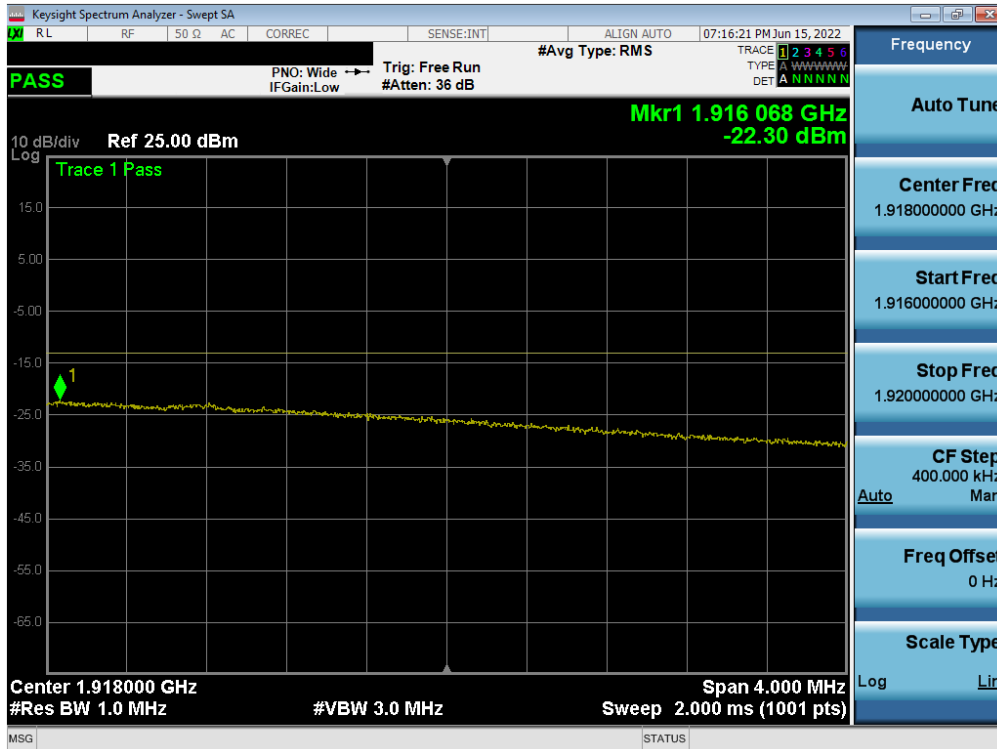
Plot 7-81. Extended Upper Band Edge Plot (LTE Band 25 - 15MHz QPSK – Full RB)
