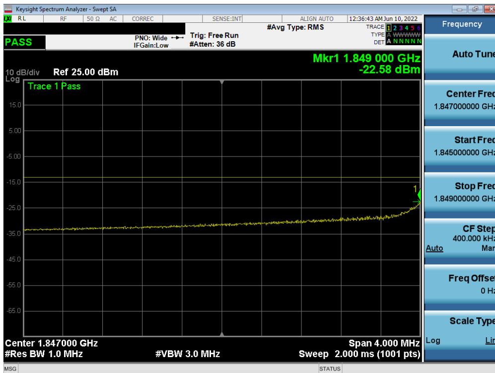
Plot 7-111. Lower Extended Band Edge Plot (NR Band n2 – 15.0MHz - Full RB)
