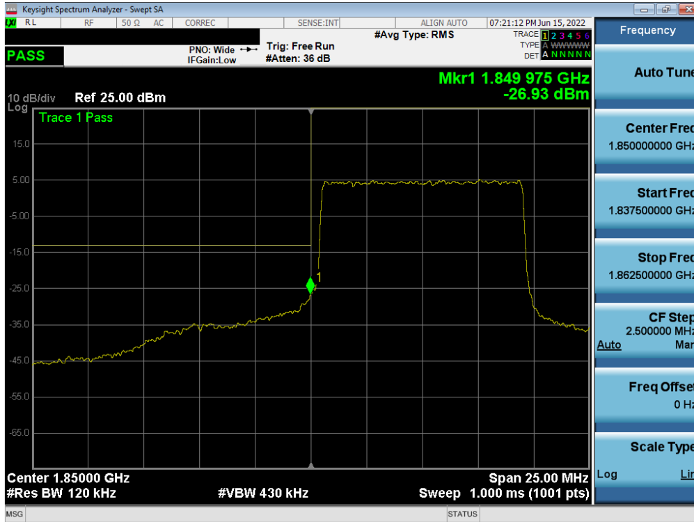
Plot 7-82. Lower Band Edge Plot (LTE Band 25/2 - 10MHz QPSK – Full RB)
