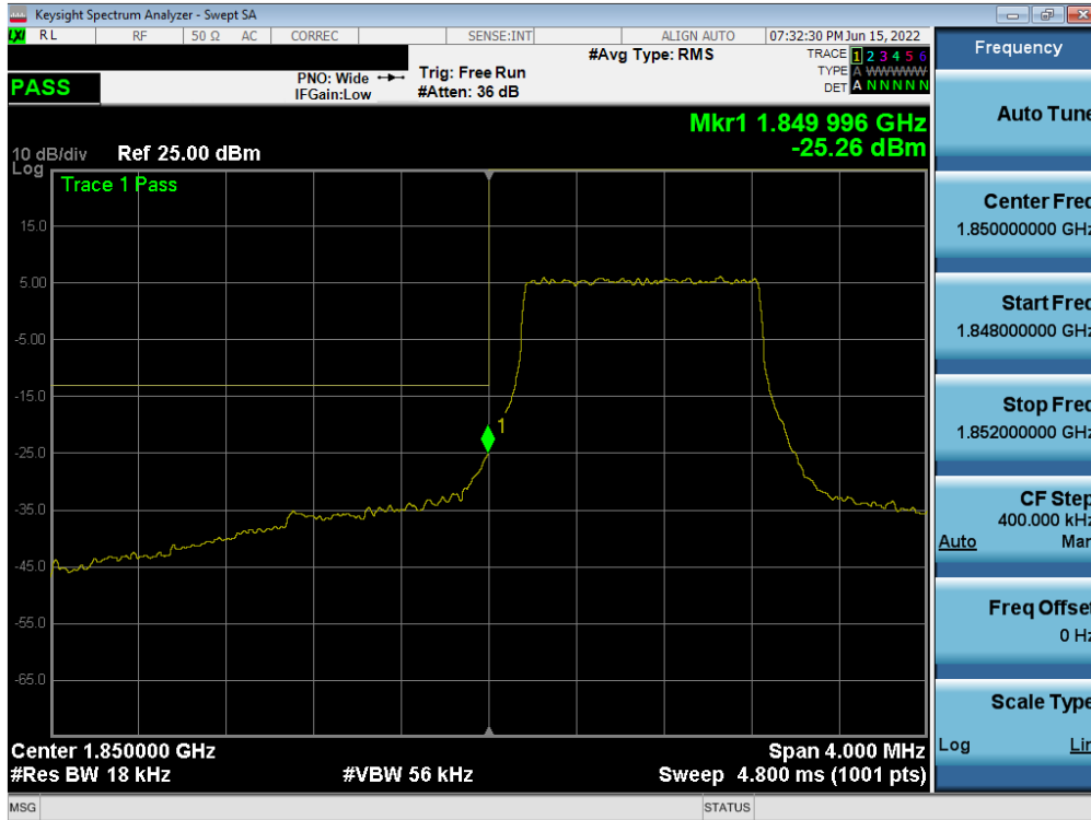
Plot 7-100. Lower Band Edge Plot (LTE Band 25/2 – 1.4MHz QPSK – Full RB)
