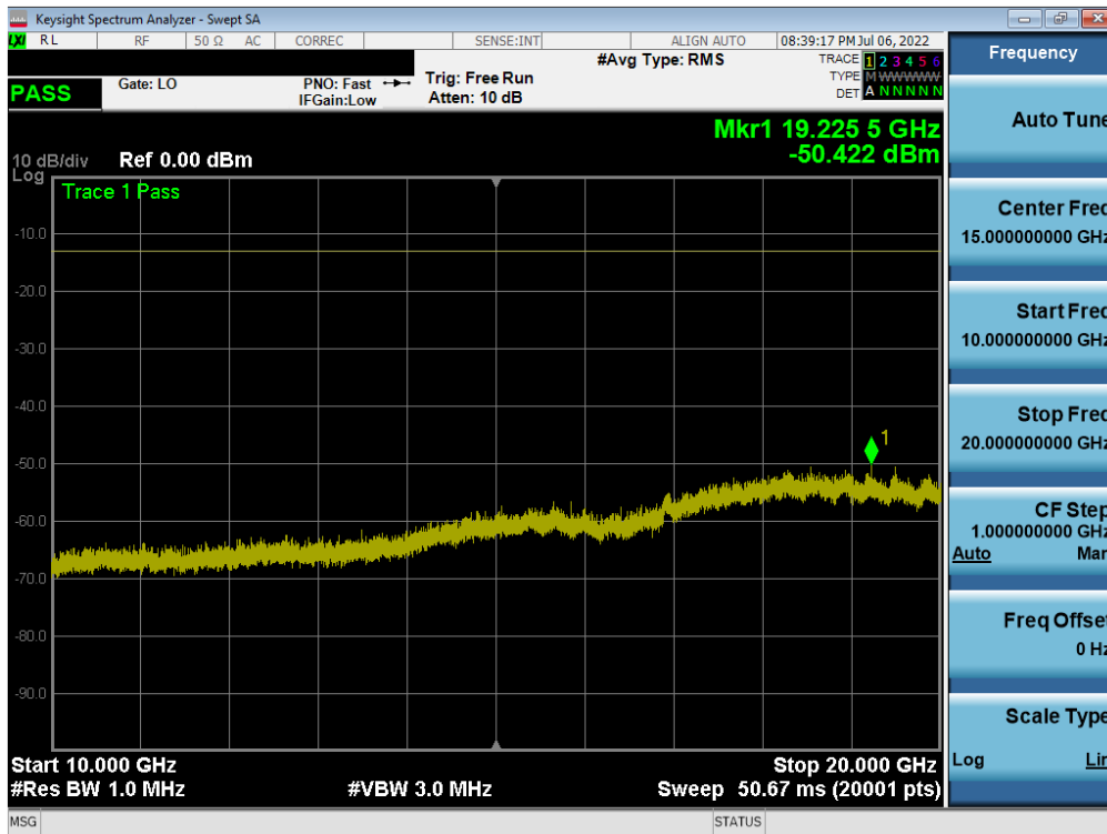
Plot 7-33. Conducted Spurious Plot (GPRS Ch. 661)
