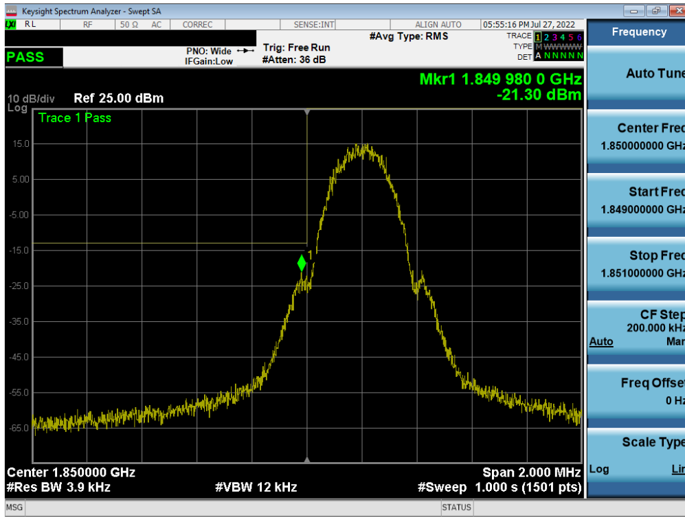
Plot 7-64. Lower Band Edge Plot (GPRS PCS – Ch. 512)
