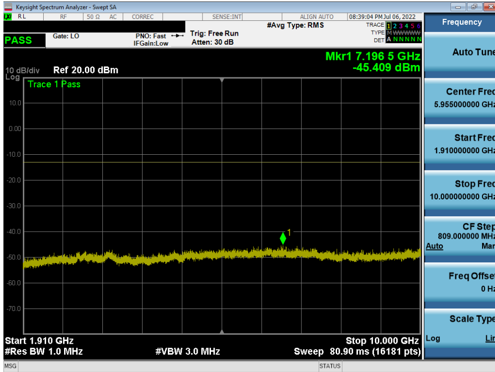
Plot 7-32. Conducted Spurious Plot (GPRS Ch. 661)
