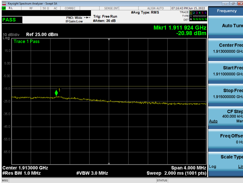
Plot 7-79. Extended Upper Band Edge Plot (LTE Band 2 - 15MHz QPSK – Full RB)
