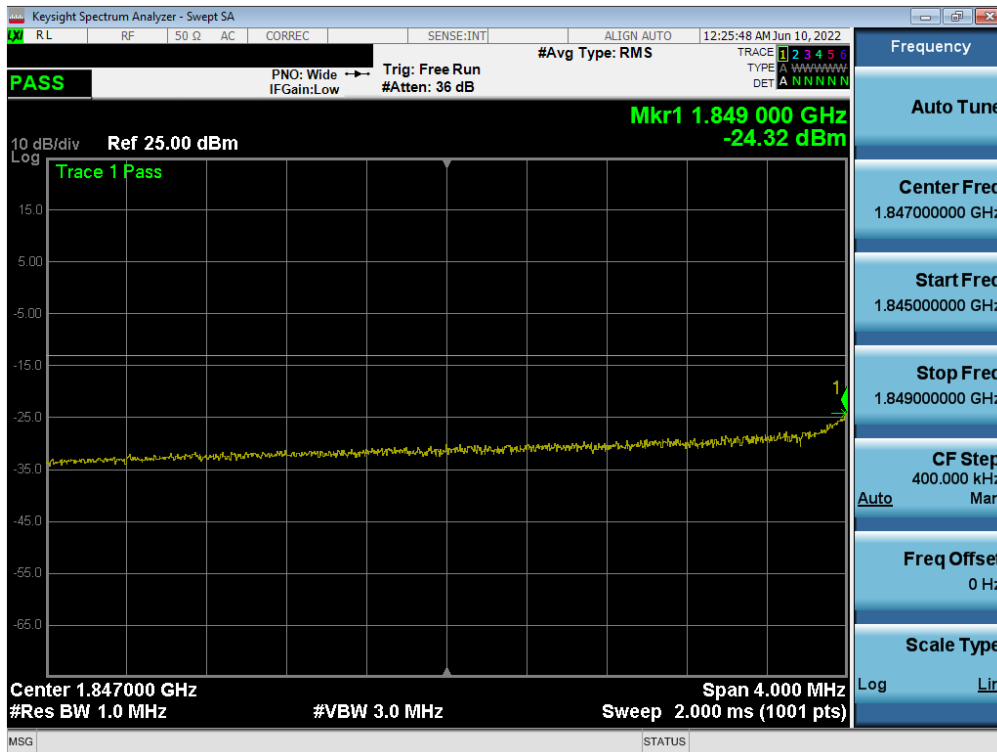
Plot 7-107. Lower Extended Band Edge Plot (NR Band n2 – 20.0MHz - Full RB)
