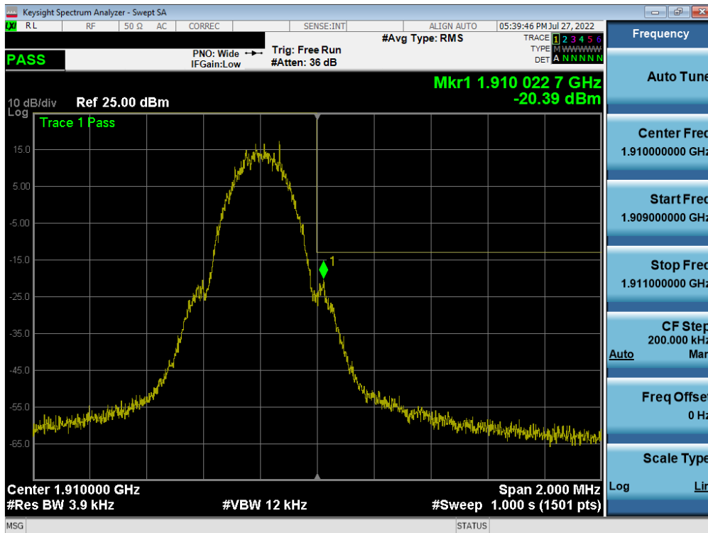
Plot 7-65. Upper Band Edge Plot (GPRS PCS – Ch. 810)
