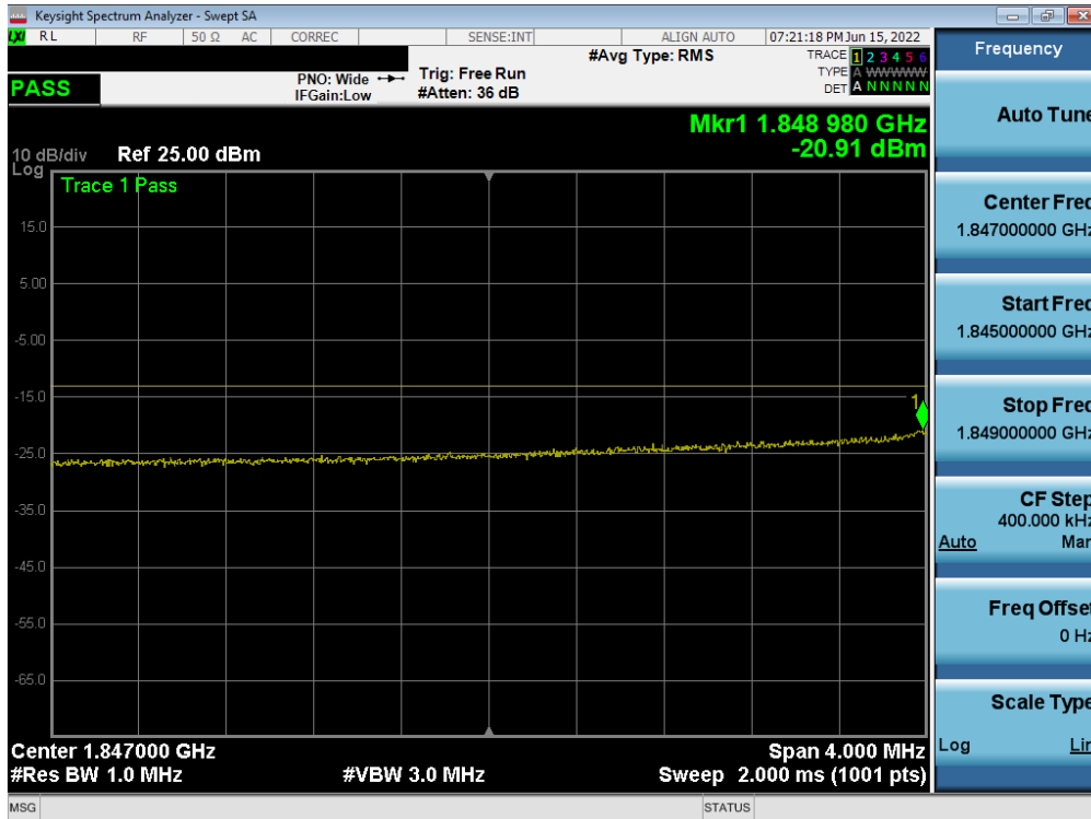
Plot 7-83. Extended Lower Band Edge Plot (LTE Band 25/2 - 10MHz QPSK – Full RB)
