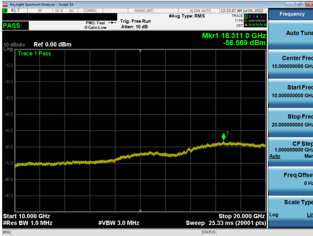
Plot 7-45. Conducted Spurious Plot (WCDMA Ch. 9538)
