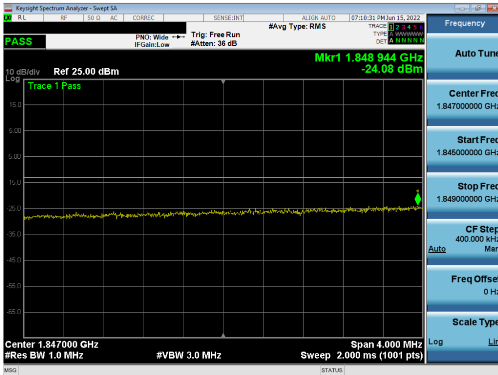
Plot 7-71. Extended Lower Band Edge Plot (LTE Band 25/2 - 20MHz QPSK – Full RB)
