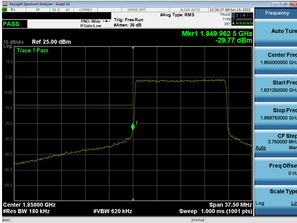
Plot 7-110. Lower Band Edge Plot (NR Band n2 – 15.0MHz - Full RB)
