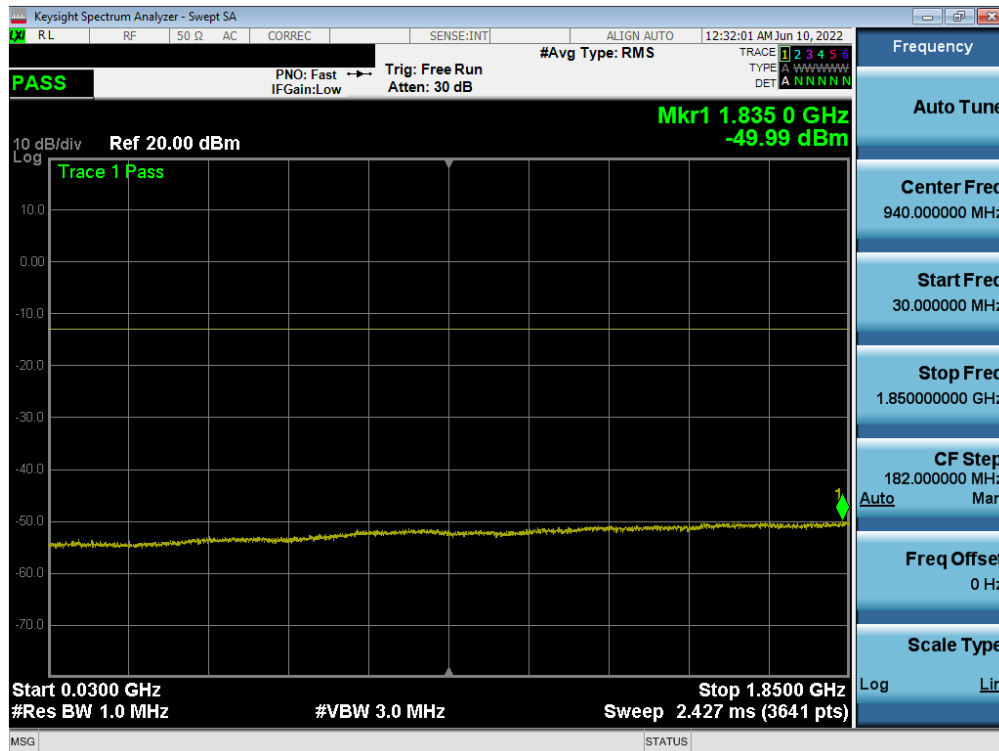
Plot 7-58. Conducted Spurious Plot (NR Band n2 - 20.0MHz - 1RB - Mid Channel)
