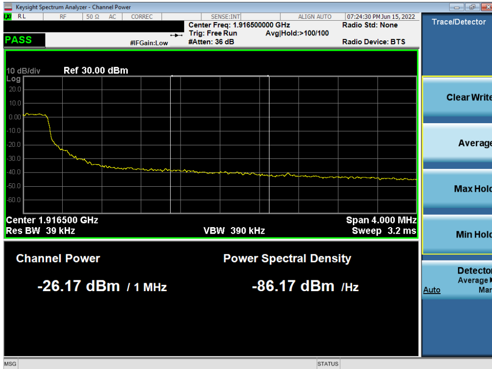
Plot 7-93. Extended Upper Band Edge Plot (LTE Band 25 - 5MHz QPSK – Full RB)
