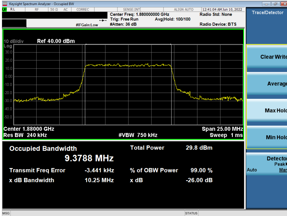
Plot 7-24. Occupied Bandwidth Plot (NR Band n2 - 10.0MHz CP-OFDM 16QAM - Full RB)
