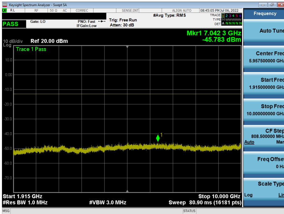
Plot 7-35. Conducted Spurious Plot (GPRS Ch. 810)
