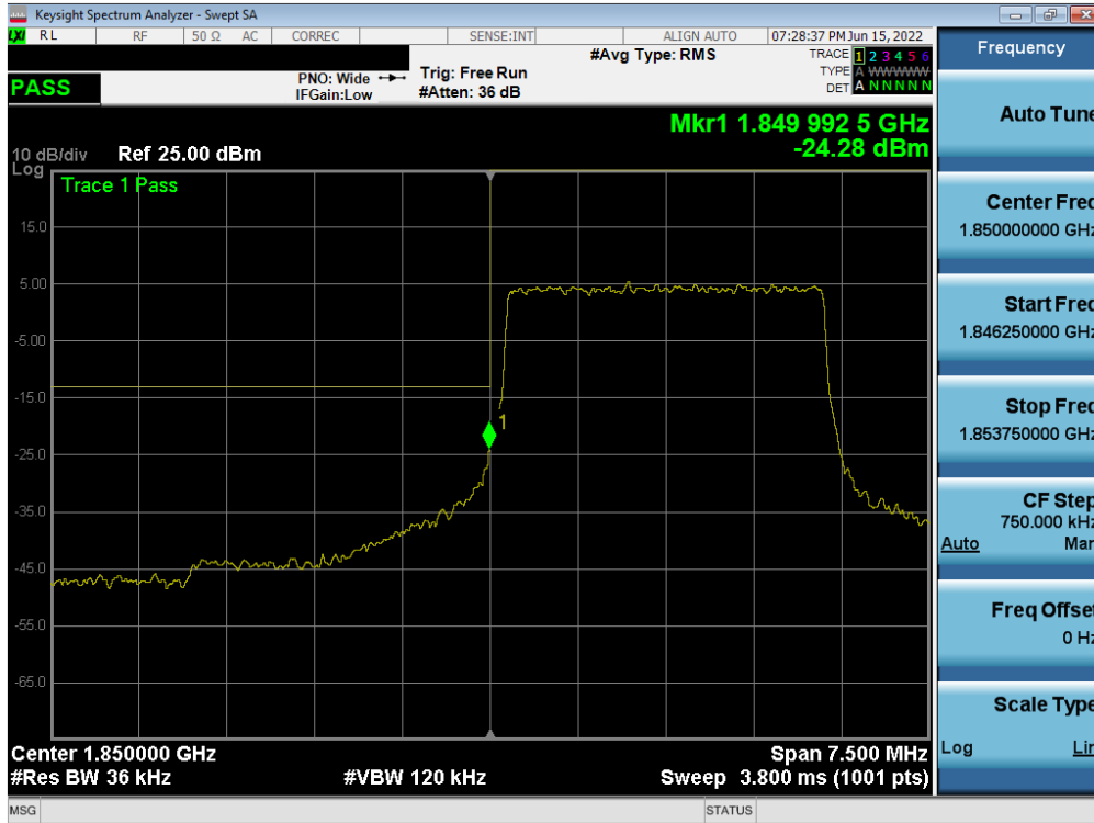
Plot 7-94. Lower Band Edge Plot (LTE Band 25/2 - 3MHz QPSK – Full RB)
