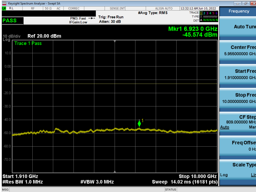
Plot 7-59. Conducted Spurious Plot (NR Band n2 - 20.0MHz - 1RB - Mid Channel)
