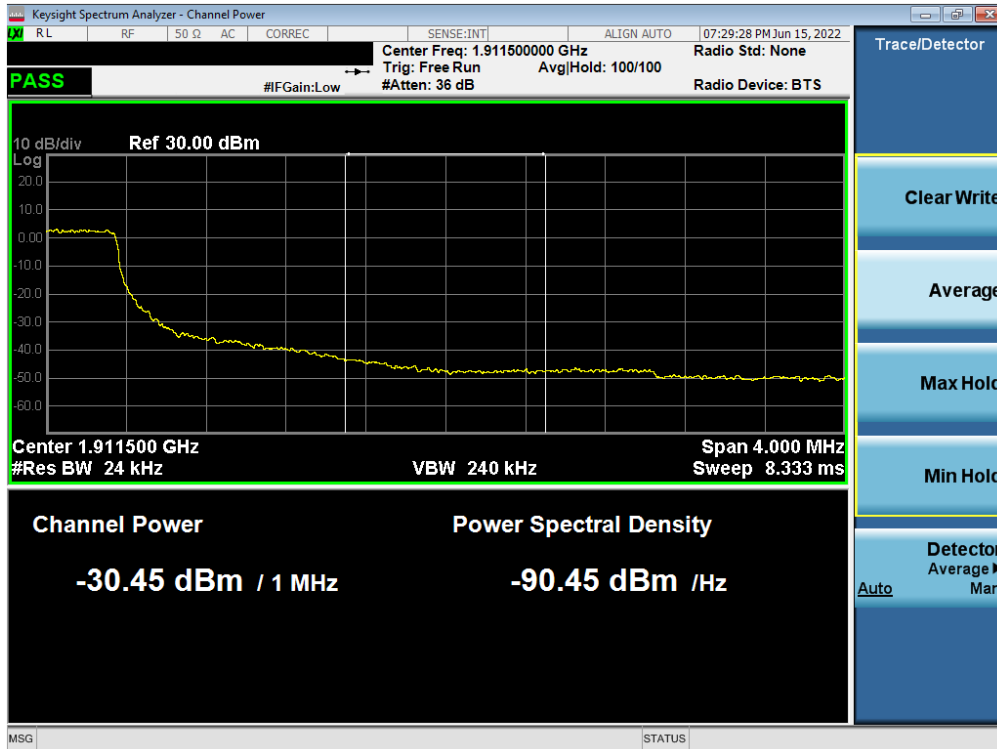
Plot 7-97. Extended Upper Band Edge Plot (LTE Band 2 - 3MHz QPSK – Full RB)
