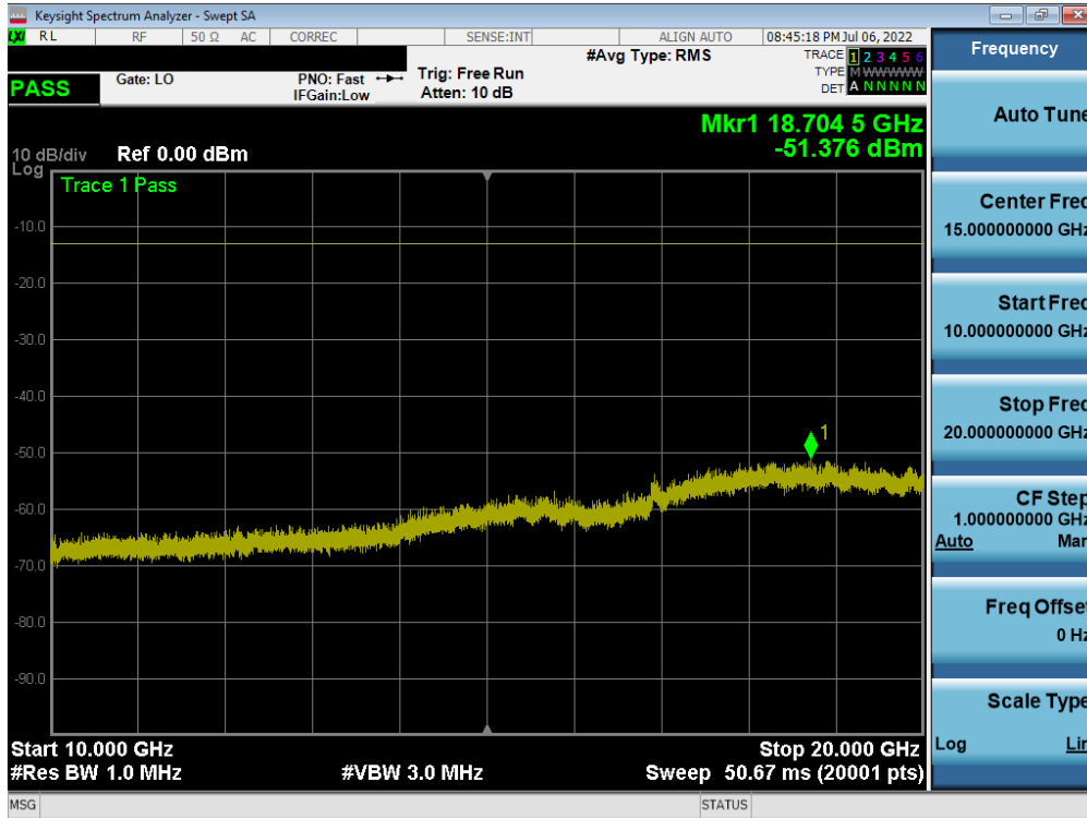
Plot 7-36. Conducted Spurious Plot (GPRS Ch. 810)
