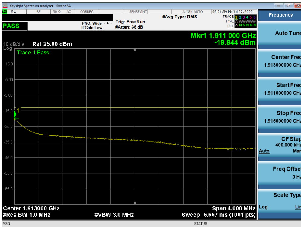
Plot 7-69. Extended Upper Band Edge Plot (WCDMA PCS – Ch. 9538)
