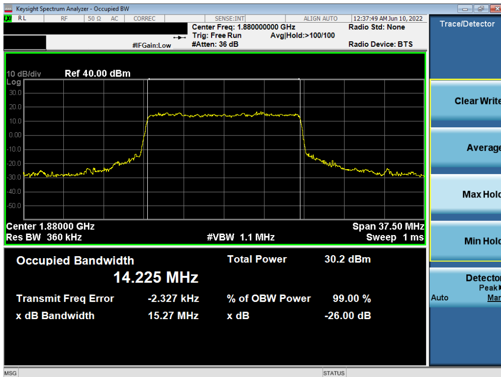
Plot 7-21. Occupied Bandwidth Plot (NR Band n2 - 15.0MHz CP-OFDM 16QAM - Full RB)
