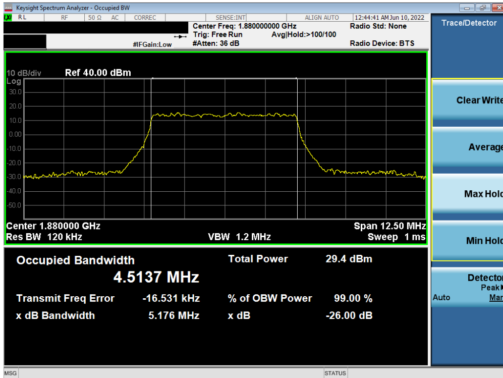
Plot 7-27. Occupied Bandwidth Plot (NR Band n2 - 5.0MHz CP-OFDM 16QAM - Full RB)
