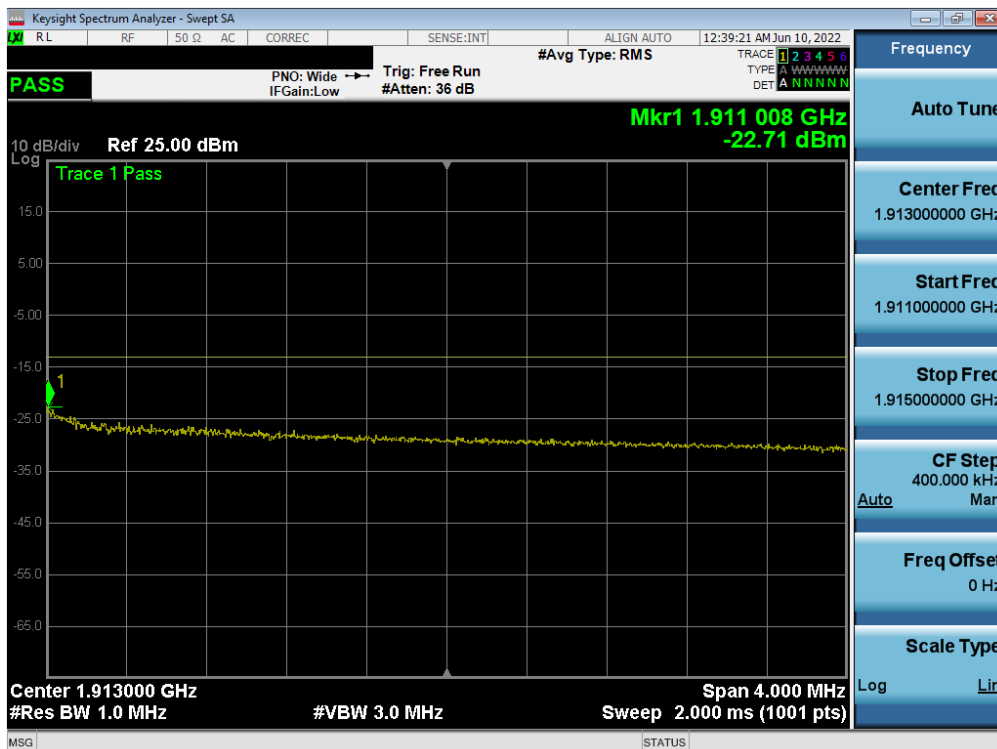
Plot 7-113. Upper Extended Band Edge Plot (NR Band n2 – 15.0MHz - Full RB)
