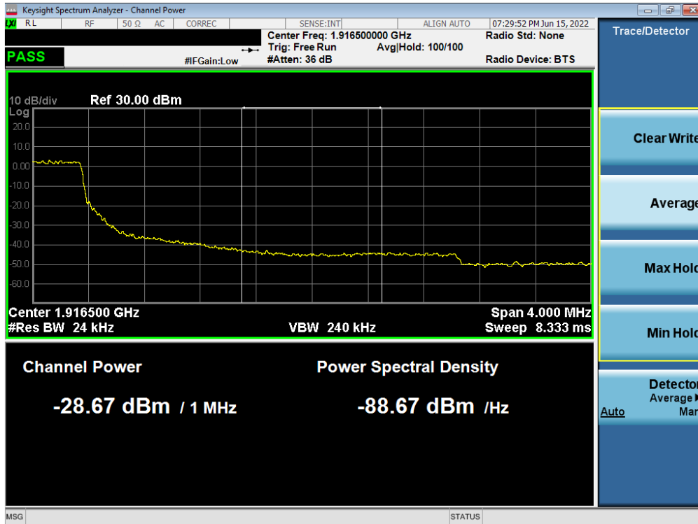
Plot 7-99. Extended Upper Band Edge Plot (LTE Band 25 - 3MHz QPSK – Full RB)
