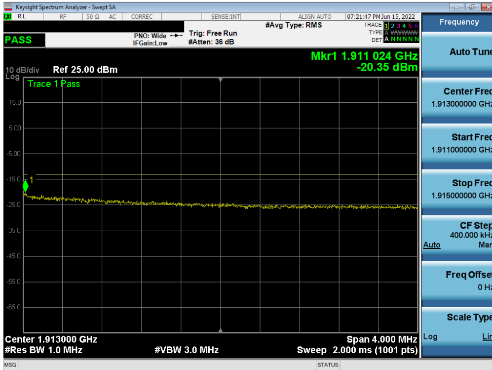
Plot 7-85. Extended Upper Band Edge Plot (LTE Band 2 - 10MHz QPSK – Full RB)
