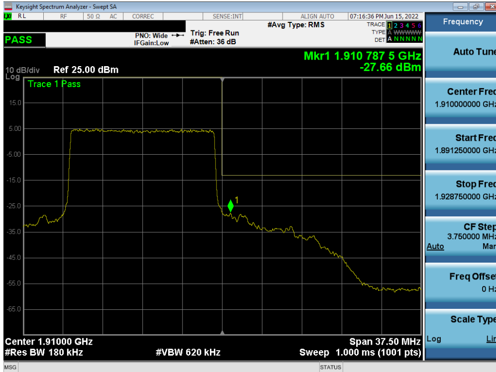
Plot 7-78. Upper Band Edge Plot (LTE Band 2 - 15MHz QPSK – Full RB)
