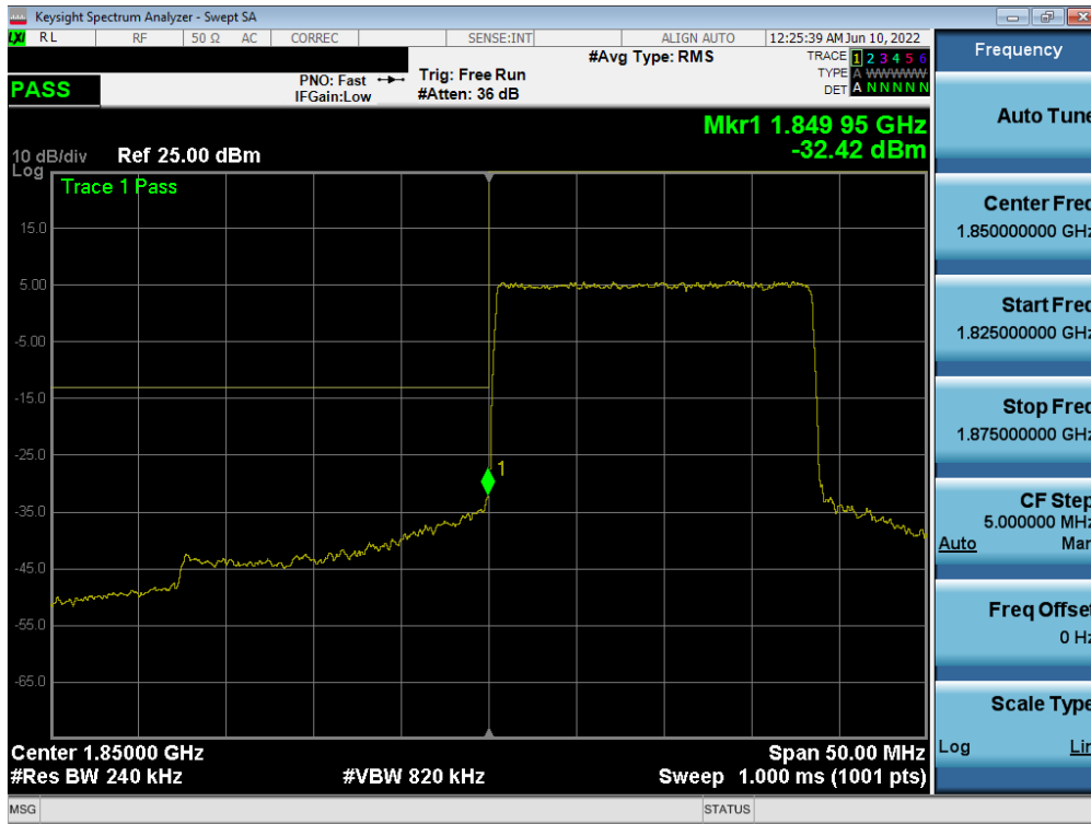
Plot 7-106. Lower Band Edge Plot (NR Band n2 – 20.0MHz - Full RB)
