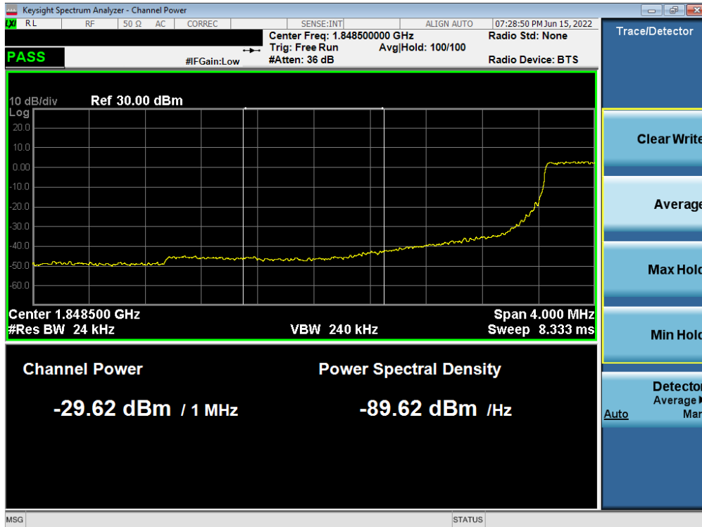
Plot 7-95. Extended Lower Band Edge Plot (LTE Band 25/2 - 3MHz QPSK – Full RB)
