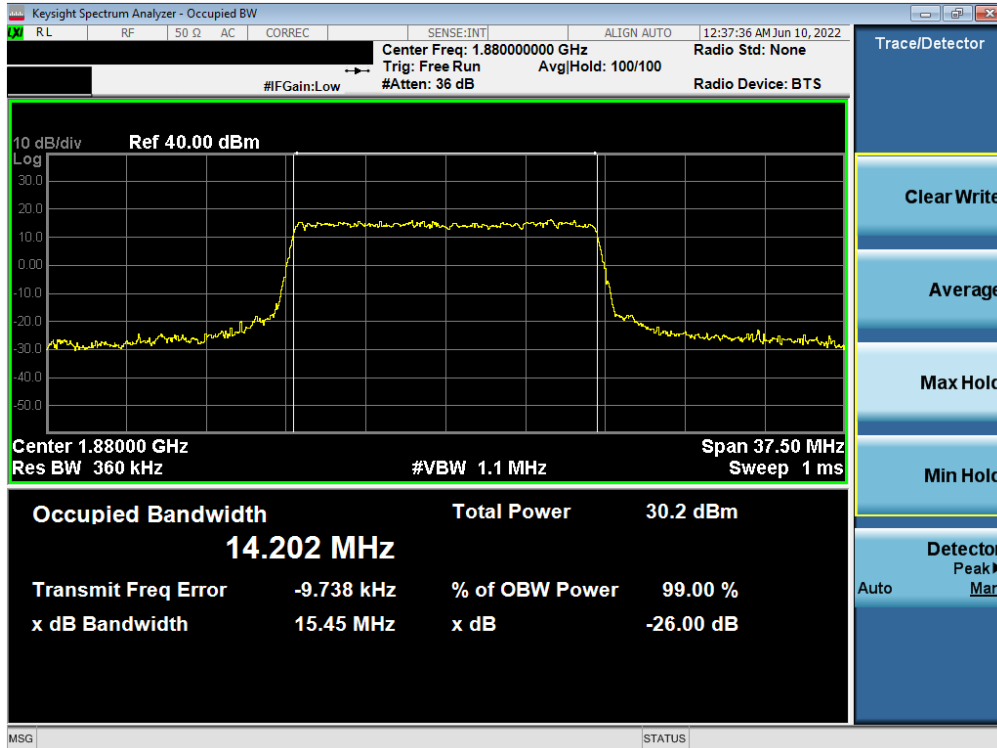
Plot 7-20. Occupied Bandwidth Plot (NR Band n2 - 15.0MHz CP-OFDM QPSK - Full RB)
