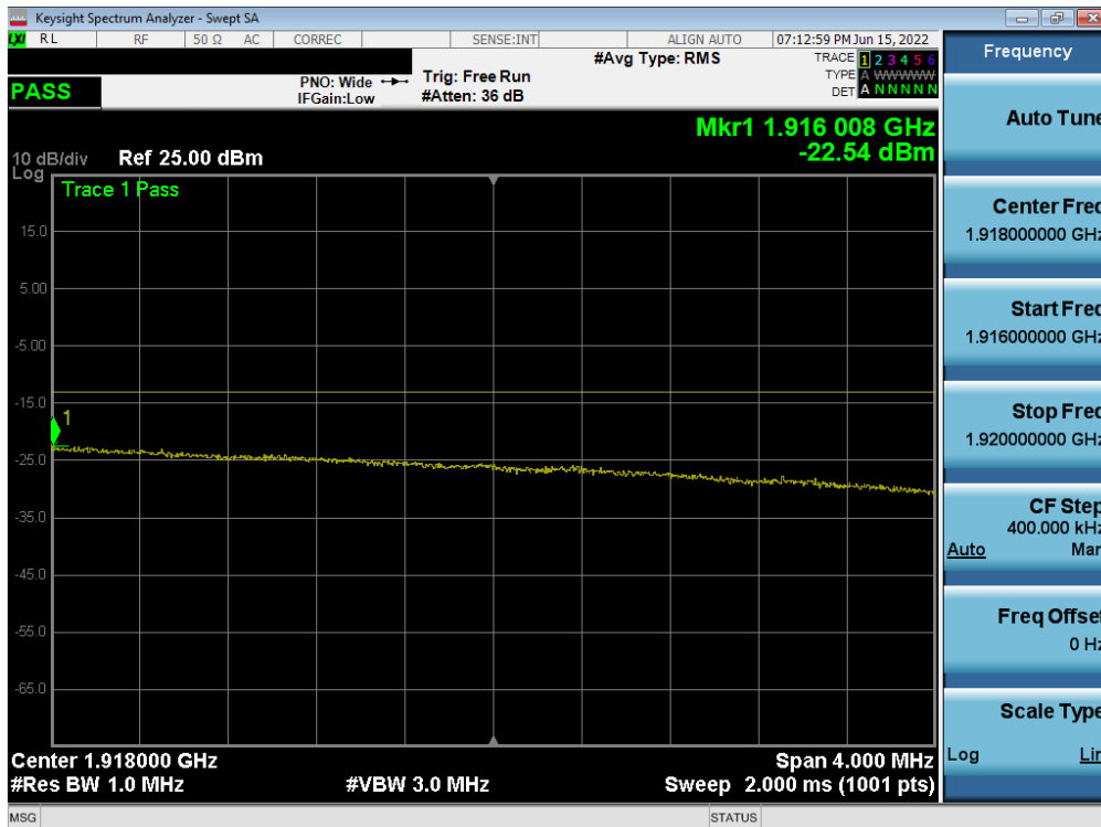
Plot 7-75. Extended Upper Band Edge Plot (LTE Band 25 - 20MHz QPSK – Full RB)
