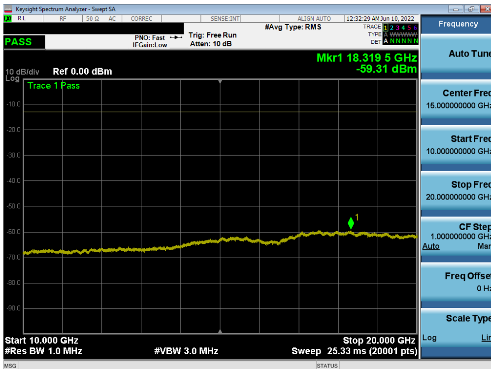
Plot 7-60. Conducted Spurious Plot (NR Band n2 - 20.0MHz - 1RB - Mid Channel)
