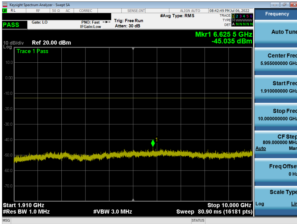
Plot 7-29. Conducted Spurious Plot (GPRS Ch. 512)
