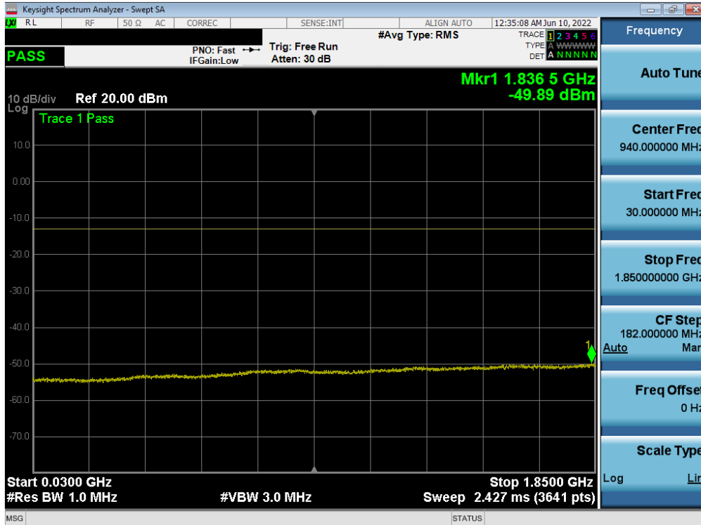
Plot 7-61. Conducted Spurious Plot (NR Band n2 - 20.0MHz - 1RB - High Channel)
