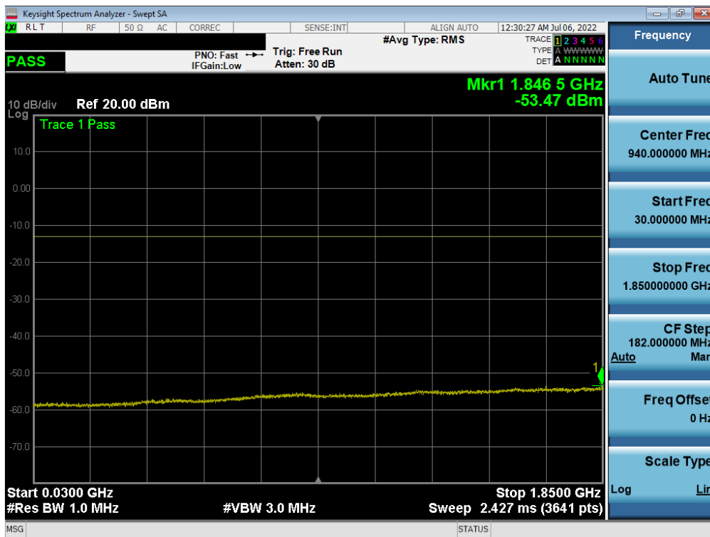
Plot 7-40. Conducted Spurious Plot (WCDMA Ch. 9400)
