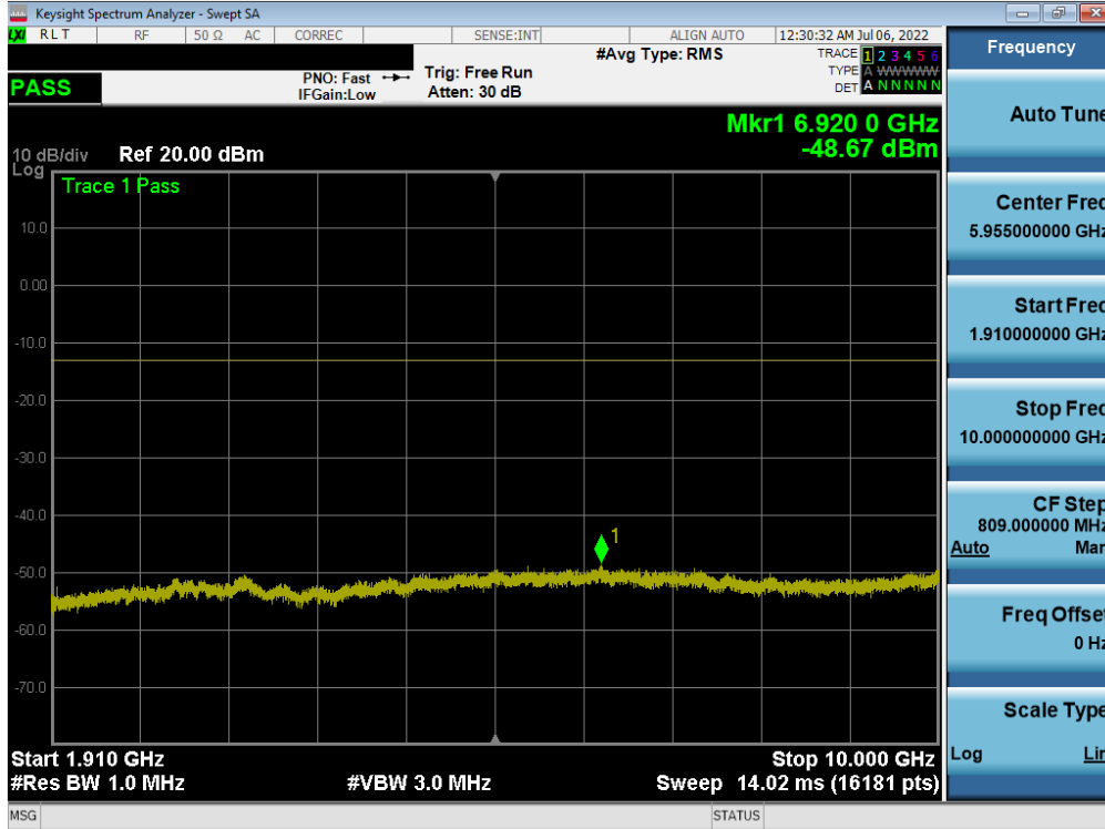
Plot 7-41. Conducted Spurious Plot (WCDMA Ch. 9400)
