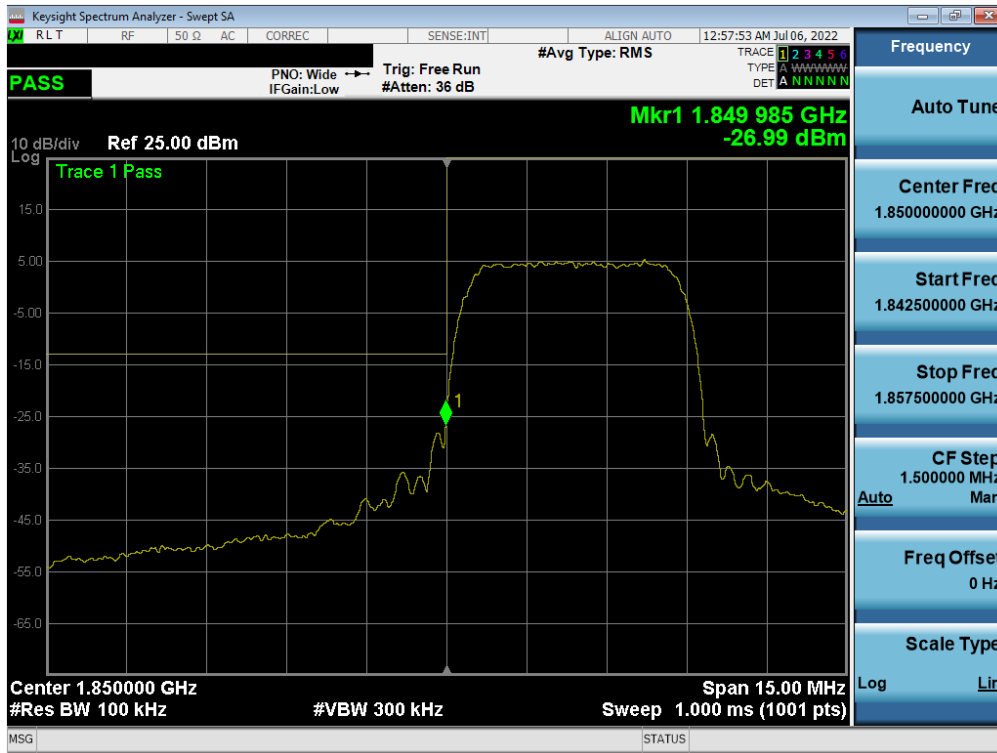
Plot 7-66. Lower Band Edge Plot (WCDMA PCS – Ch. 9262)
