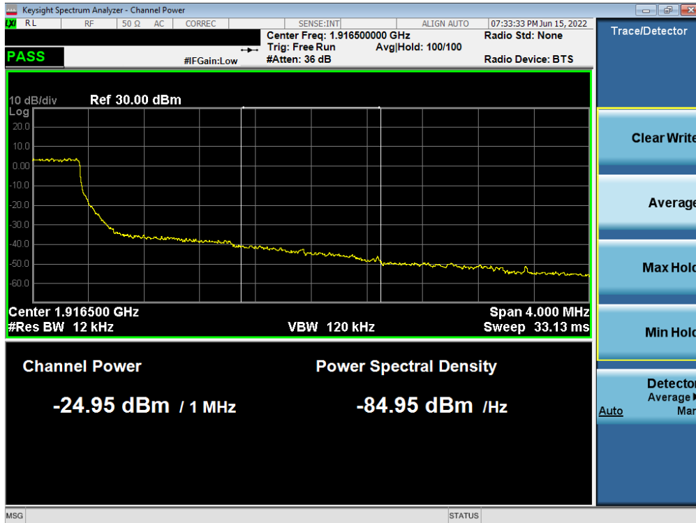
Plot 7-105. Extended Upper Band Edge Plot (LTE Band 25 – 1.4MHz QPSK – Full RB)
