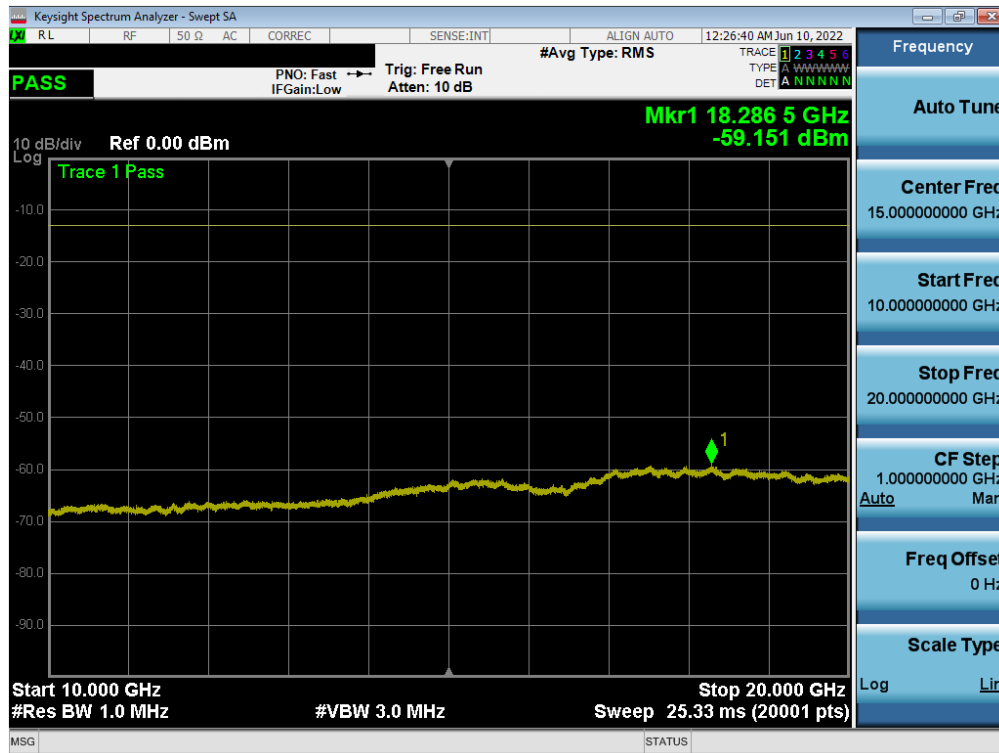
Plot 7-57. Conducted Spurious Plot (NR Band n2 - 20.0MHz - 1RB - Low Channel)
