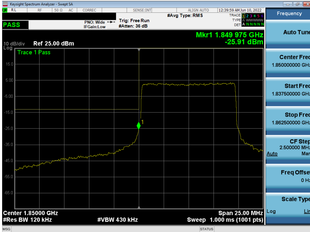
Plot 7-114. Lower Band Edge Plot (NR Band n2 – 10.0MHz - Full RB)
