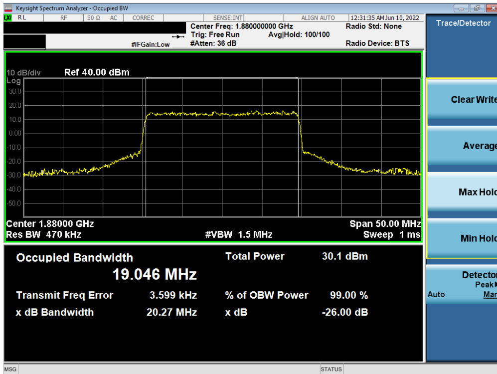
Plot 7-18. Occupied Bandwidth Plot (NR Band n2 - 20.0MHz CP-OFDM 16QAM - Full RB)
