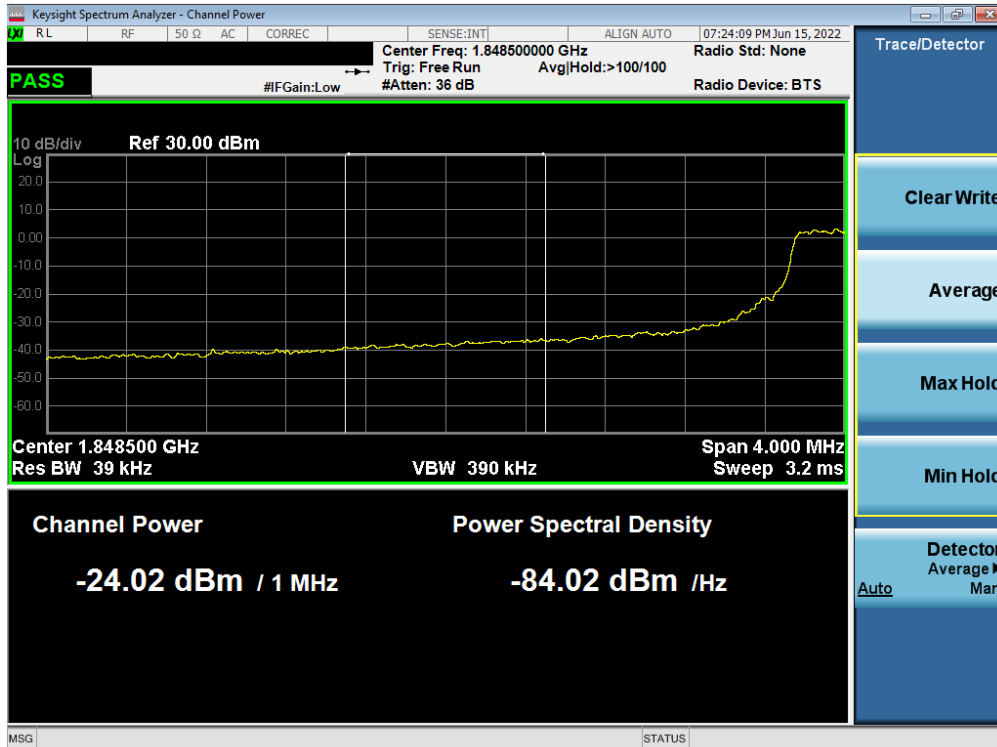
Plot 7-89. Extended Lower Band Edge Plot (LTE Band 25/2 - 5MHz QPSK – Full RB)
