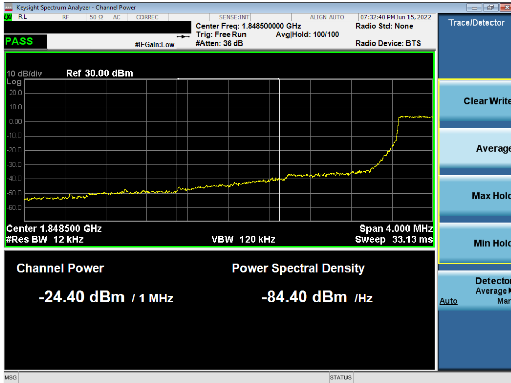
Plot 7-101. Extended Lower Band Edge Plot (LTE Band 25/2 – 1.4MHz QPSK – Full RB)
