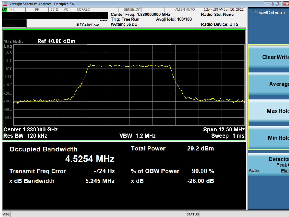
Plot 7-26. Occupied Bandwidth Plot (NR Band n2 - 5.0MHz CP-OFDM QPSK - Full RB)
