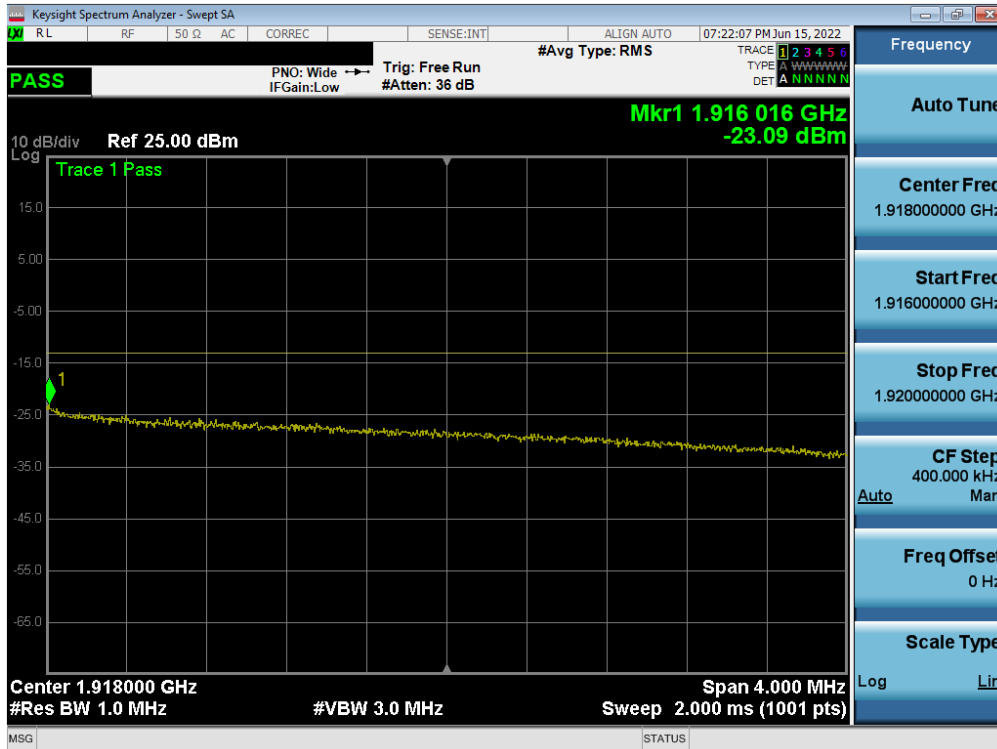
Plot 7-87. Extended Upper Band Edge Plot (LTE Band 25 - 10MHz QPSK – Full RB)
