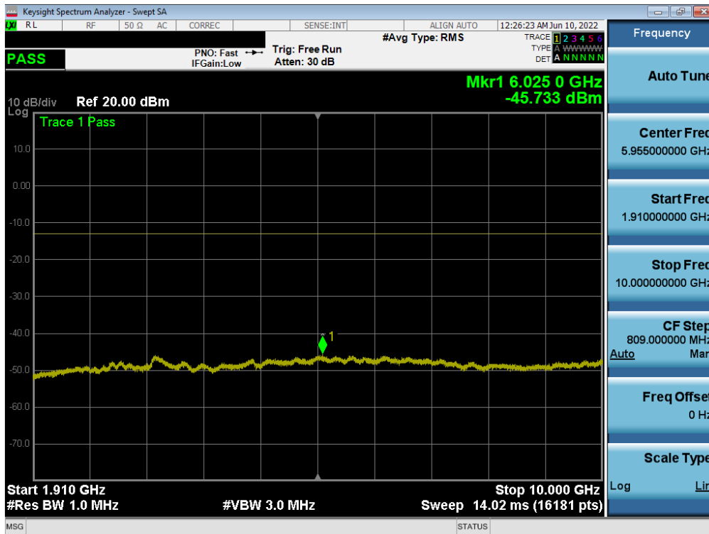
Plot 7-56. Conducted Spurious Plot (NR Band n2 - 20.0MHz - 1RB - Low Channel)
