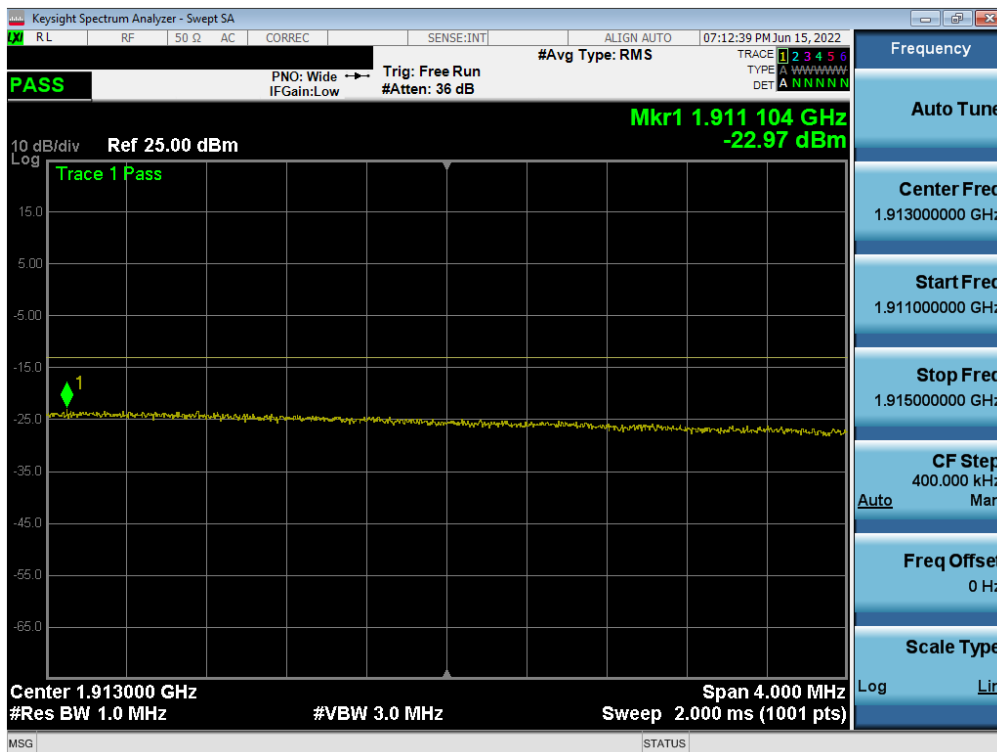
Plot 7-73. Extended Upper Band Edge Plot (LTE Band 2 - 20MHz QPSK – Full RB)
