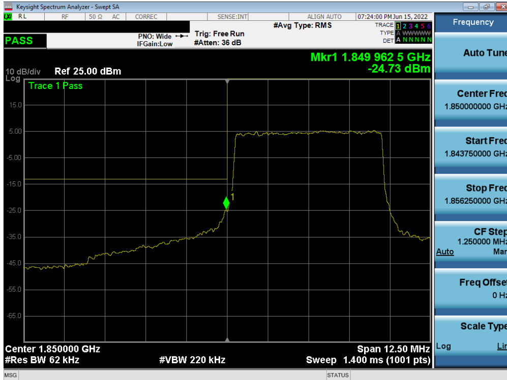
Plot 7-88. Lower Band Edge Plot (LTE Band 25/2 - 5MHz QPSK – Full RB)
