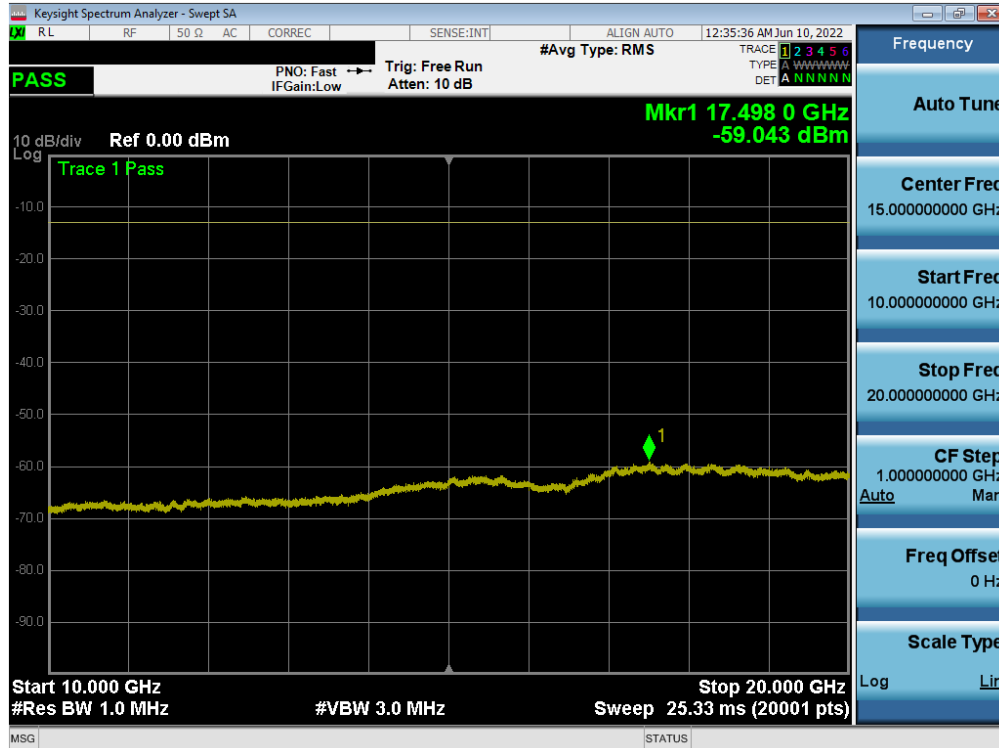
Plot 7-63. Conducted Spurious Plot (NR Band n2 - 20.0MHz - 1RB - High Channel)
