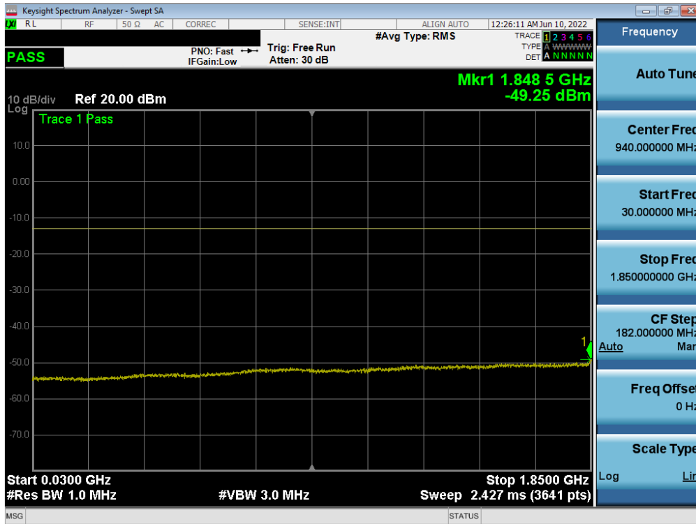
Plot 7-55. Conducted Spurious Plot (NR Band n2 -20.0MHz - 1RB - Low Channel)
