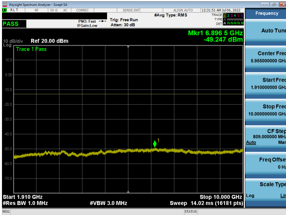
Plot 7-38. Conducted Spurious Plot (WCDMA Ch. 9262)
