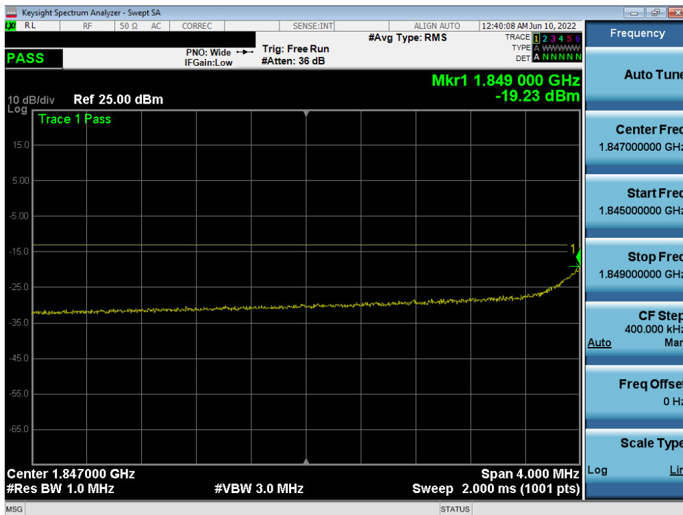
Plot 7-115. Lower Extended Band Edge Plot (NR Band n2 – 10.0MHz - Full RB)
