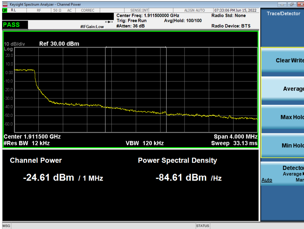
Plot 7-103. Extended Upper Band Edge Plot (LTE Band 2 – 1.4MHz QPSK – Full RB)
