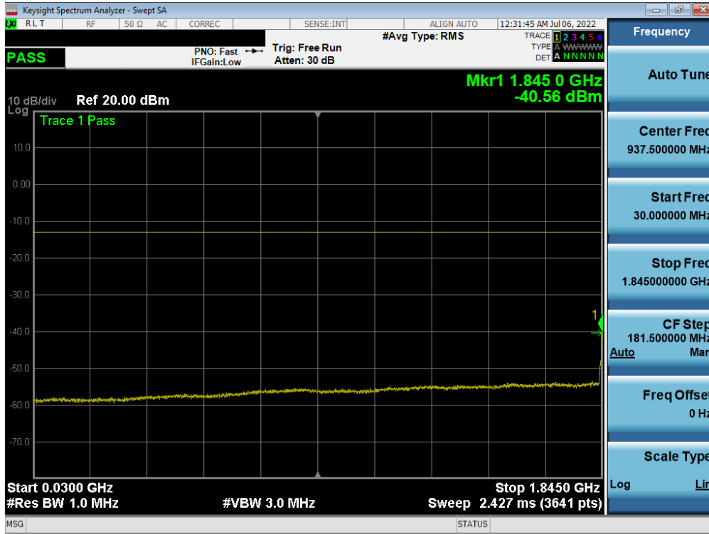
Plot 7-37. Conducted Spurious Plot (WCDMA Ch. 9262)
