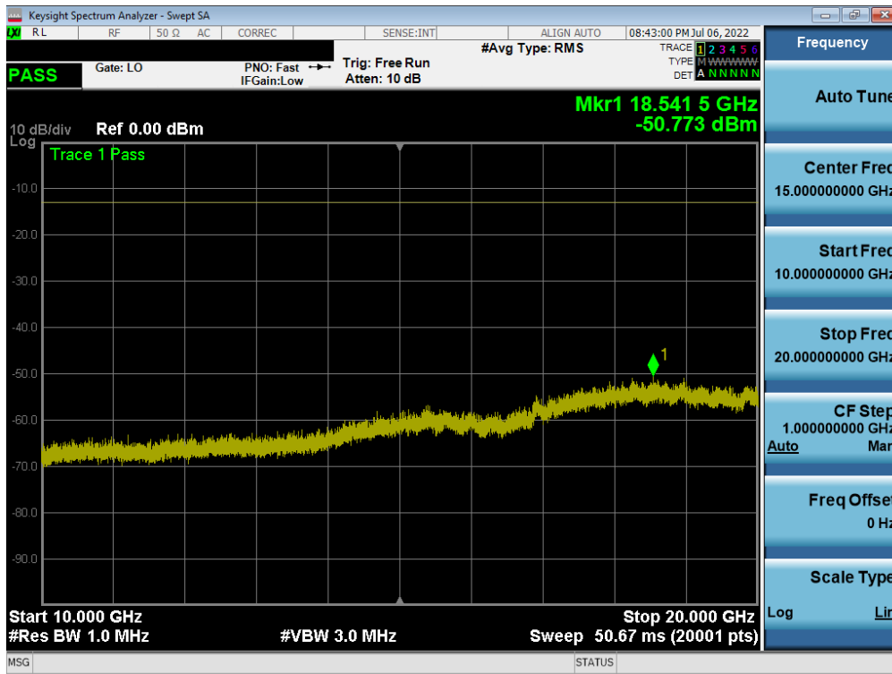
Plot 7-30. Conducted Spurious Plot (GPRS Ch. 512)
