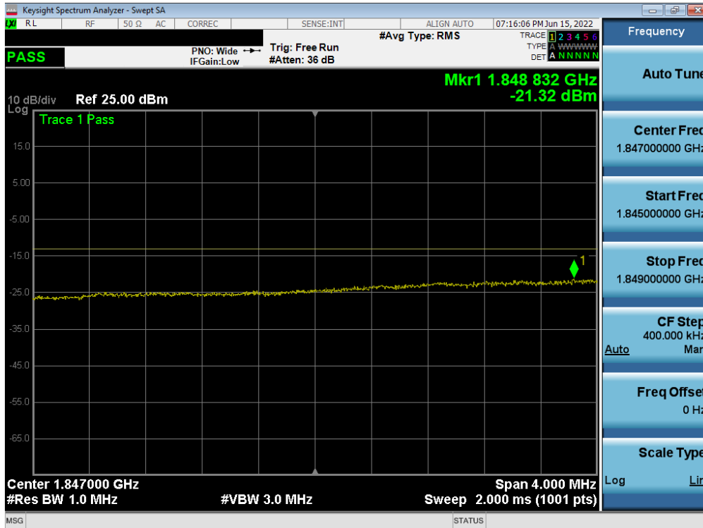
Plot 7-77. Extended Lower Band Edge Plot (LTE Band 25/2 - 15MHz QPSK – Full RB)
