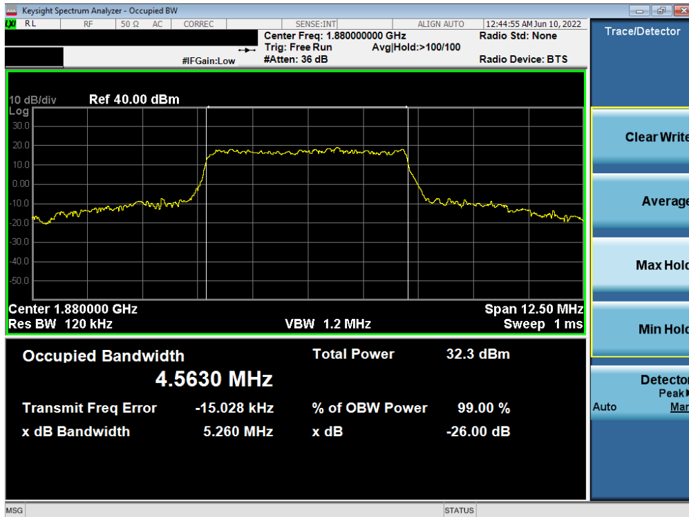
Plot 7-25. Occupied Bandwidth Plot (NR Band n2 - 5.0MHz DFT-s-OFDM BPSK - Full RB)
