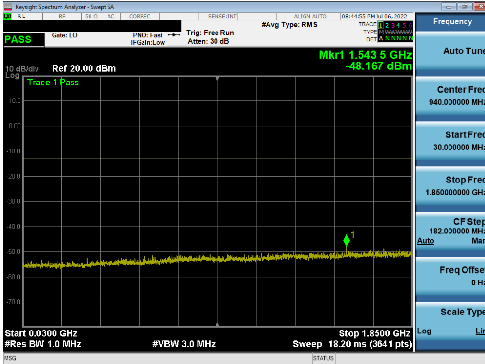
Plot 7-34. Conducted Spurious Plot (GPRS Ch. 810)
