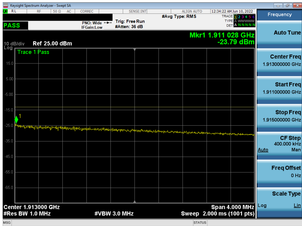
Plot 7-109. Upper Extended Band Edge Plot (NR Band n2 – 20.0MHz - Full RB)
