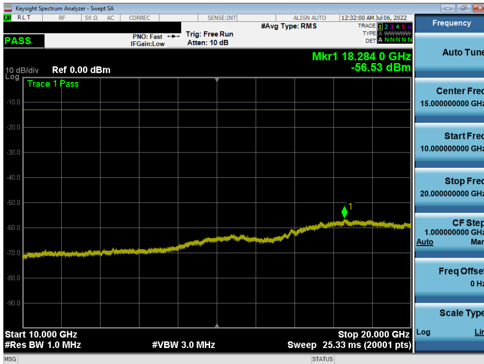
Plot 7-39. Conducted Spurious Plot (WCDMA Ch. 9262)
