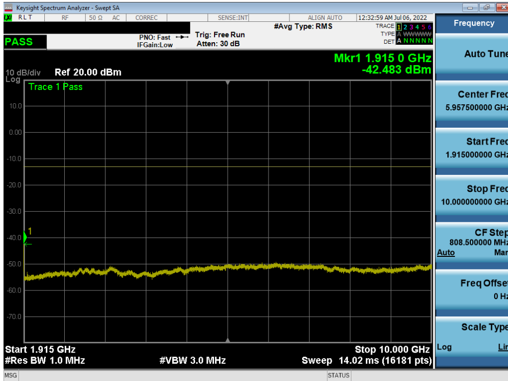
Plot 7-44. Conducted Spurious Plot (WCDMA Ch. 9538)
