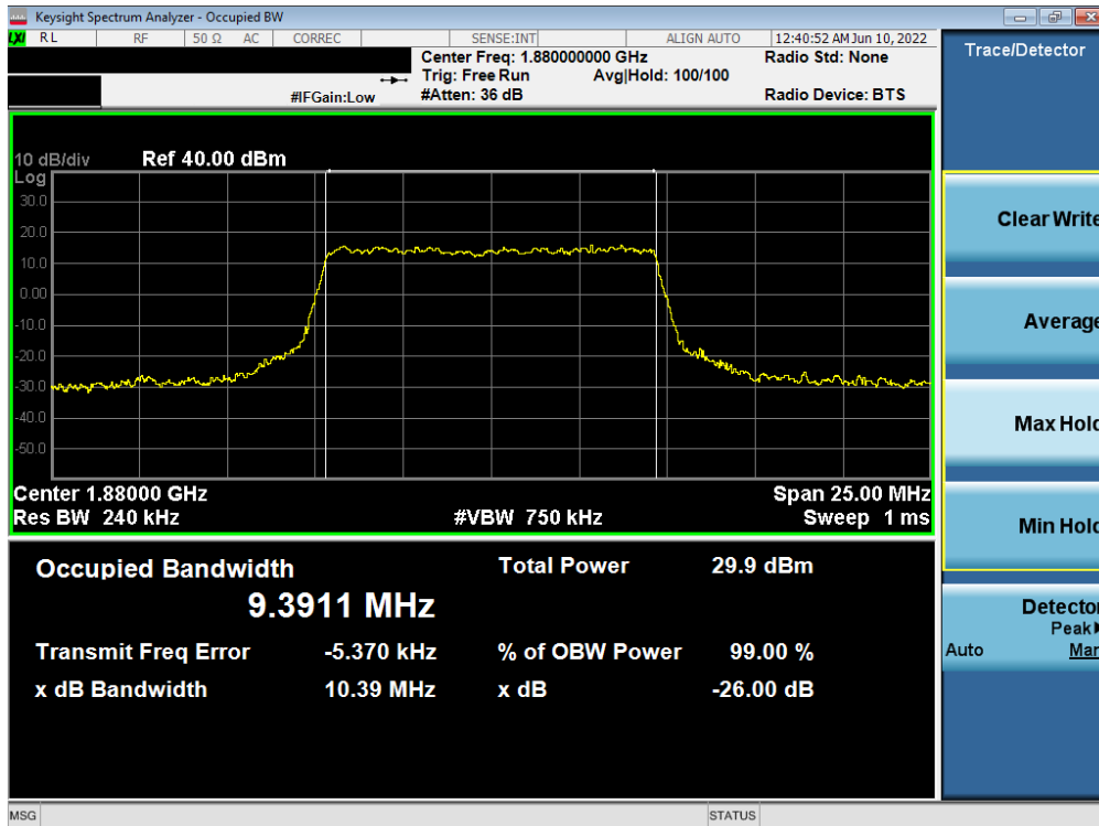
Plot 7-23. Occupied Bandwidth Plot (NR Band n2 - 10.0MHz CP-OFDM QPSK - Full RB)
