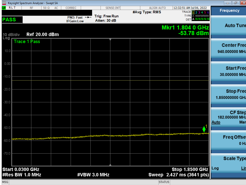
Plot 7-43. Conducted Spurious Plot (WCDMA Ch. 9538)
