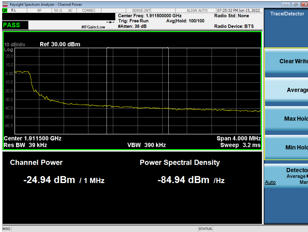
Plot 7-91. Extended Upper Band Edge Plot (LTE Band 2 - 5MHz QPSK – Full RB)
