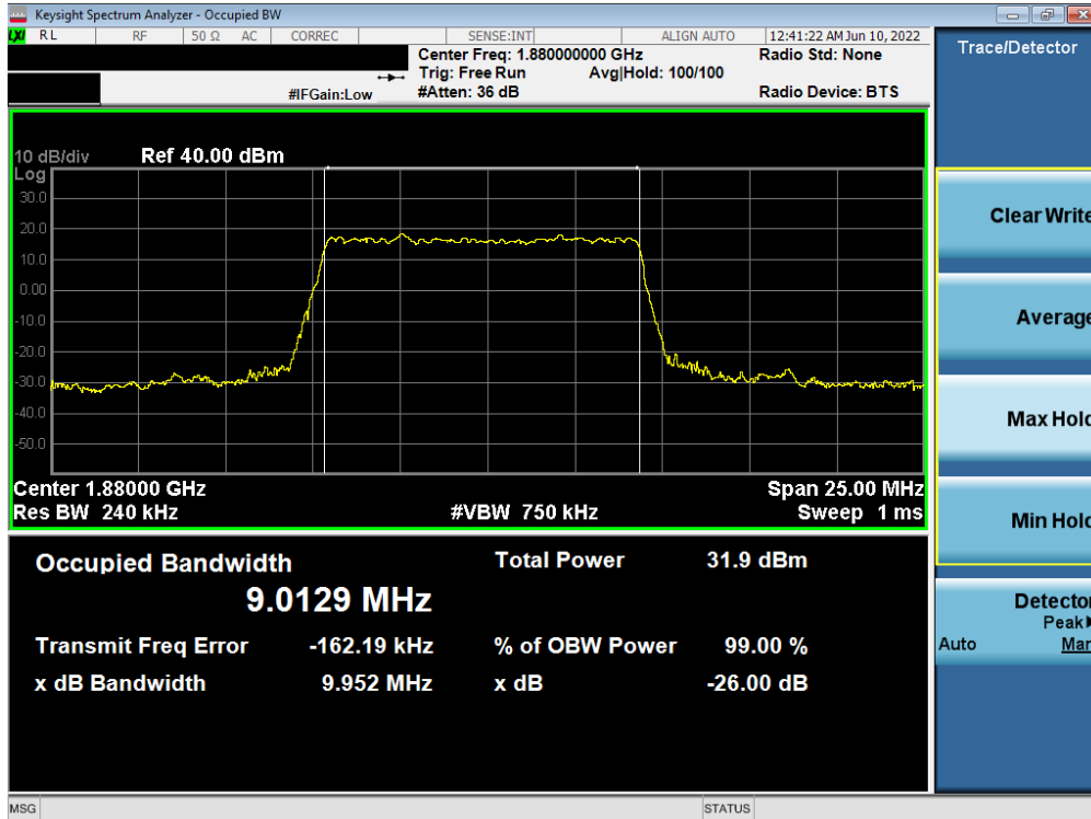
Plot 7-22. Occupied Bandwidth Plot (NR Band n2 - 10.0MHz DFT-s-OFDM BPSK - Full RB)
