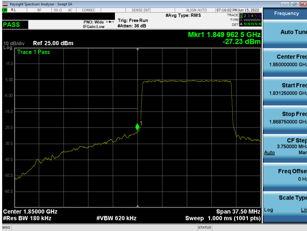
Plot 7-76. Lower Band Edge Plot (LTE Band 25/2 - 15MHz QPSK – Full RB)
