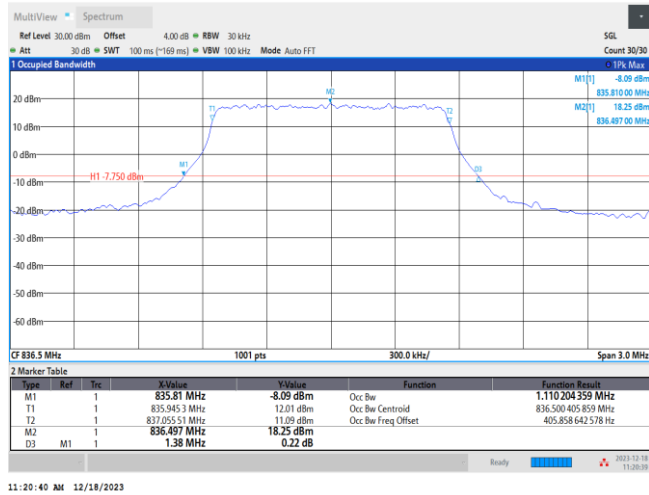
Band5-1.4MHz-16QAM-20525-6RB#0
