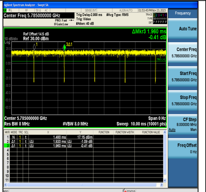
NTVN-11N20MIMO-Ant7-5785
