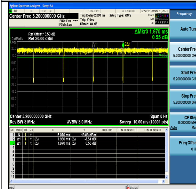
NTNV-11AC20MIMO-Ant6-5200
