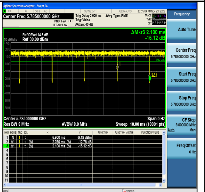
NTNV-11A-CDD-Ant7-5785
