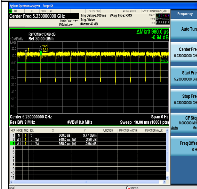
NTVN-11N40MIMO-Ant6-5230
