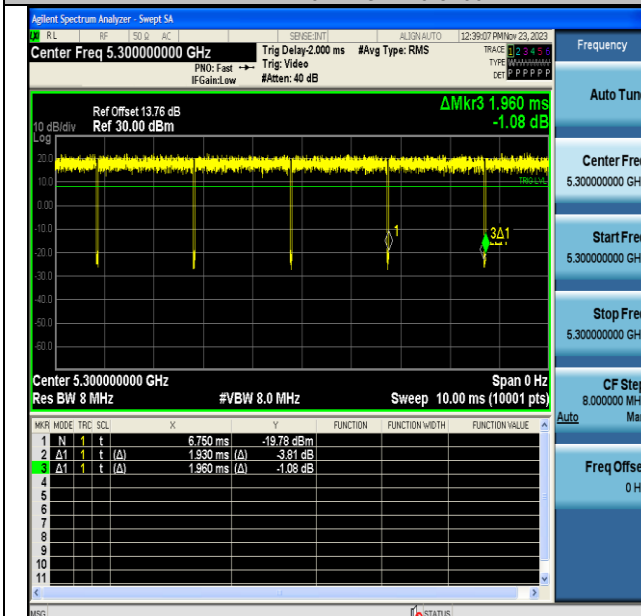
NTVN-11N20MIMO-Ant6-5300
