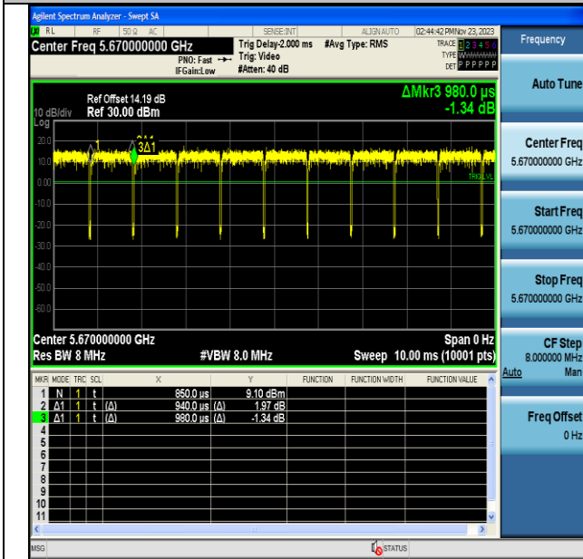
NTVN-11N40MIMO-Ant6-5670
