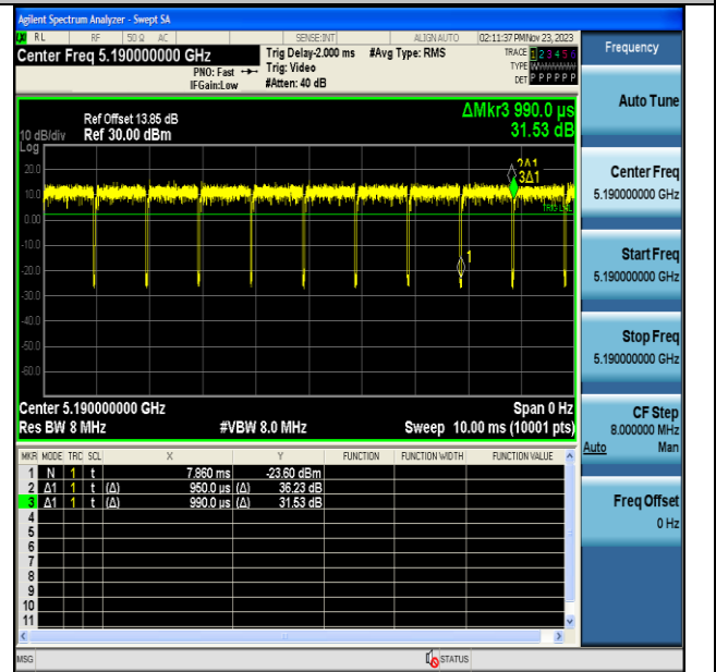
NTVN-11N40MIMO-Ant7-5190
