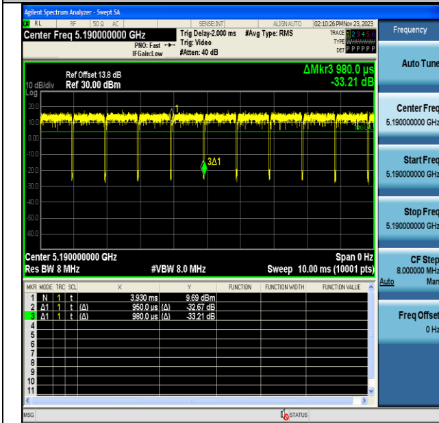
NTVN-11N40MIMO-Ant6-5190
