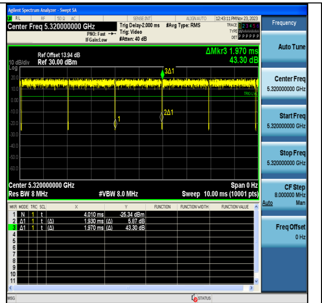
NTVN-11N20MIMO-Ant7-5320
