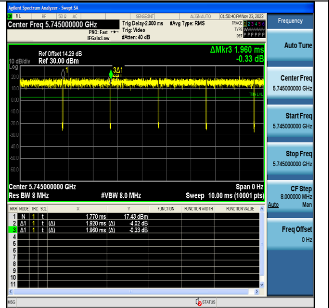
NTVN-11N20MIMO-Ant7-5745
