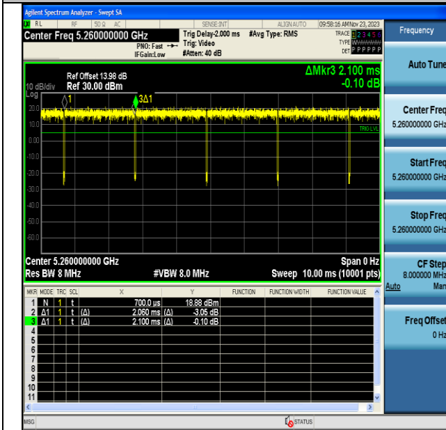
NTVN-11A-CDD-Ant6-5260
