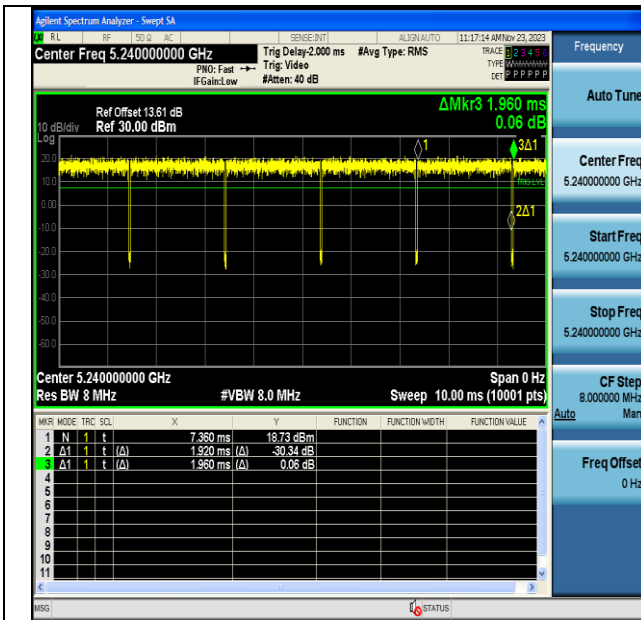
NTVN-11N20MIMO-Ant6-5240
