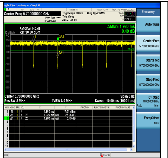
NTVN-11N20MIMO-Ant7-5700
