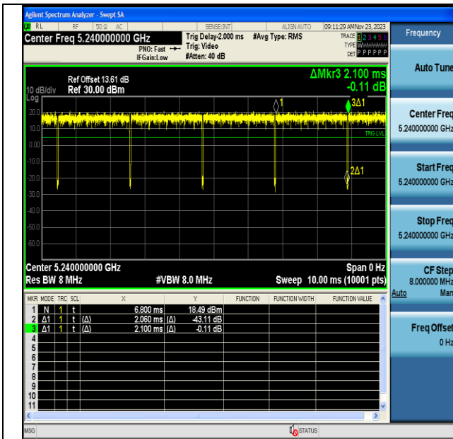
NTVN-11A-CDD-Ant6-5240
