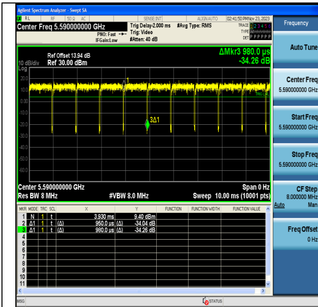
NTVN-11N40MIMO-Ant6-5590
