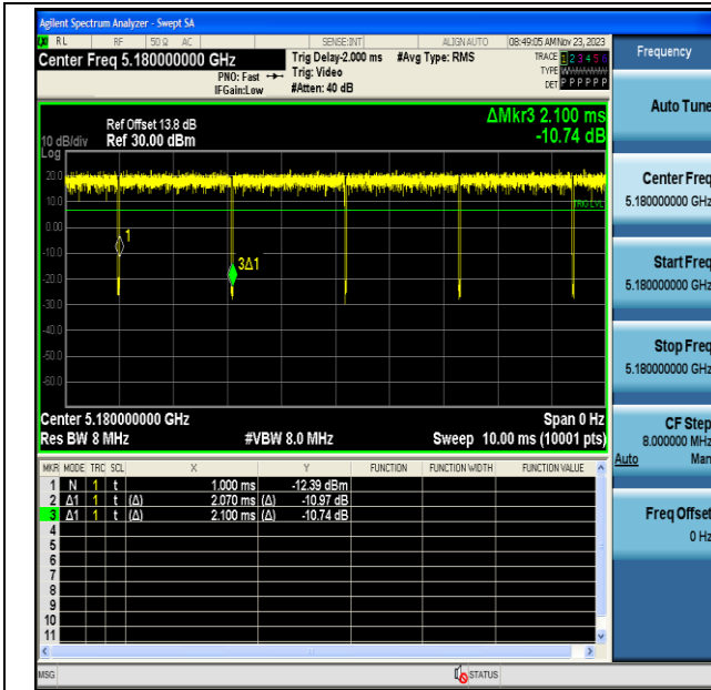
NTVN-11A-CDD-Ant6-5180
