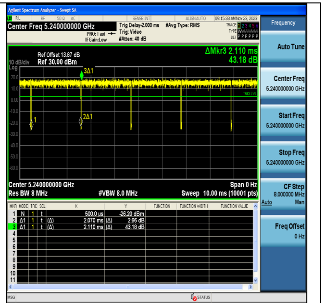
NTVN-11A-CDD-Ant7-5240
