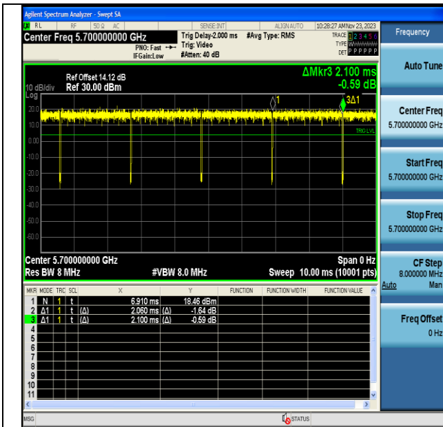
NTNV-11A-CDD-Ant6-5700
