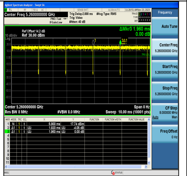
NTVN-11N20MIMO-Ant7-5260
