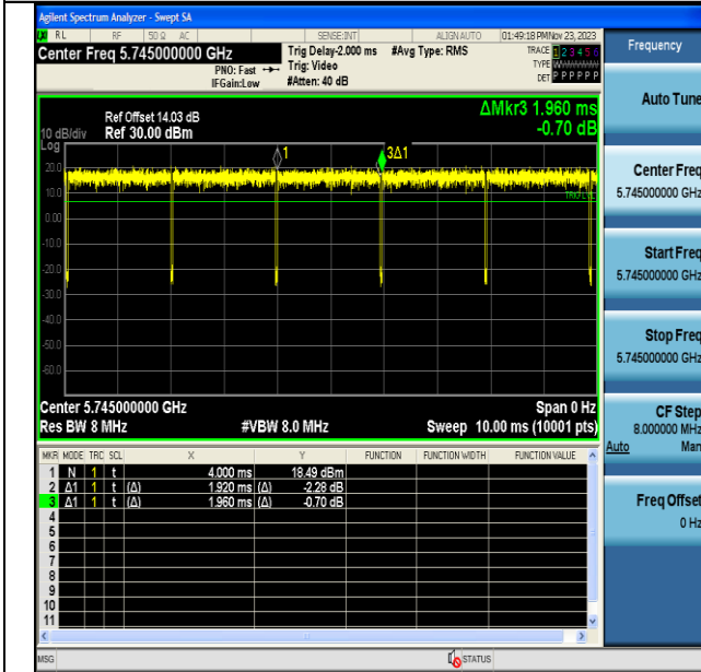
NTVN-11N20MIMO-Ant6-5745
