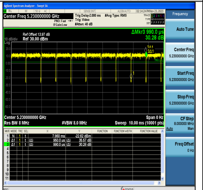
NTVN-11N40MIMO-Ant7-5230
