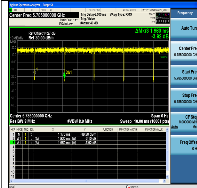
NTVN-11N20MIMO-Ant6-5785
