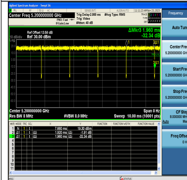
NTVN-11N20MIMO-Ant6-5200
