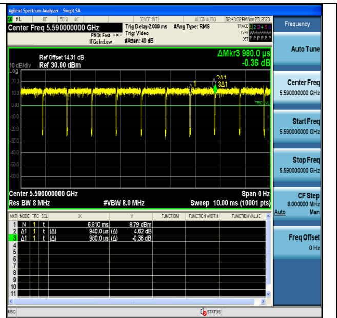
NTVN-11N40MIMO-Ant7-5590
