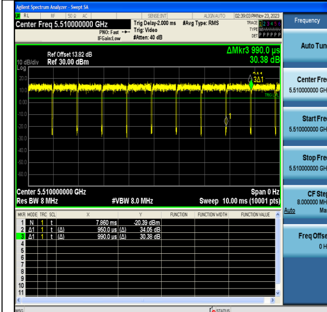
NTVN-11N40MIMO-Ant6-5510
