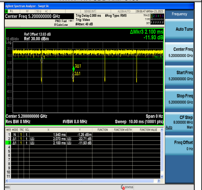
NTVN-11A-CDD-Ant7-5200
