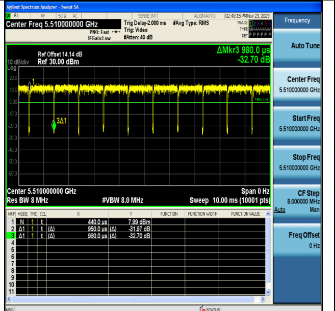
NTVN-11N40MIMO-Ant7-5510
