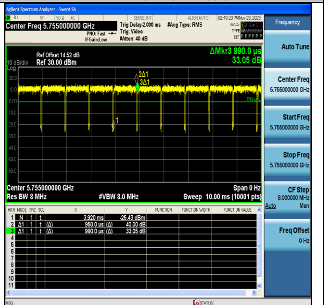
NTVN-11N40MIMO-Ant7-5755
