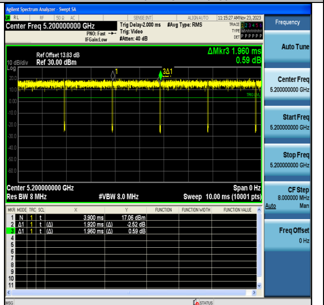
NTVN-11N20MIMO-Ant7-5200
