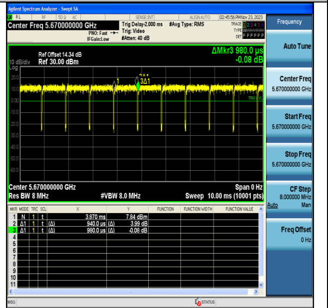
NTVN-11N40MIMO-Ant7-5670
