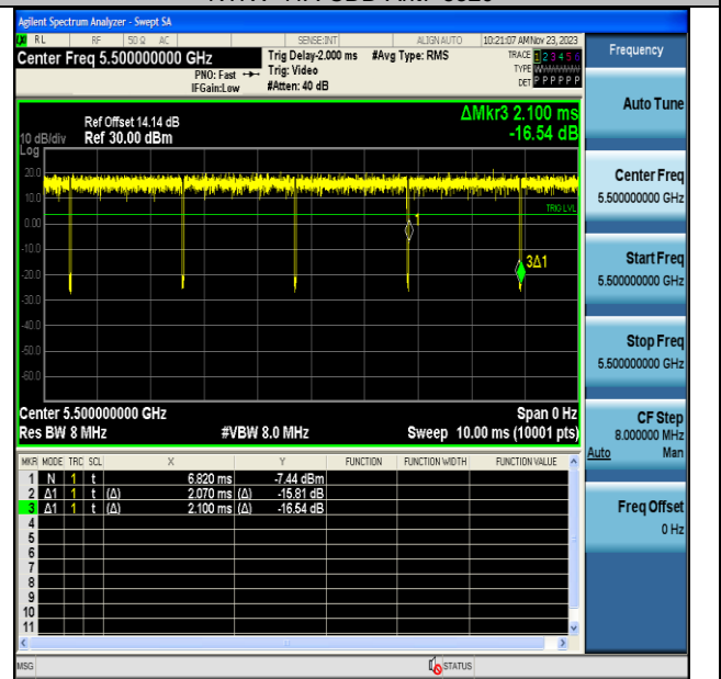
NTVN-11A-CDD-Ant7-5500
