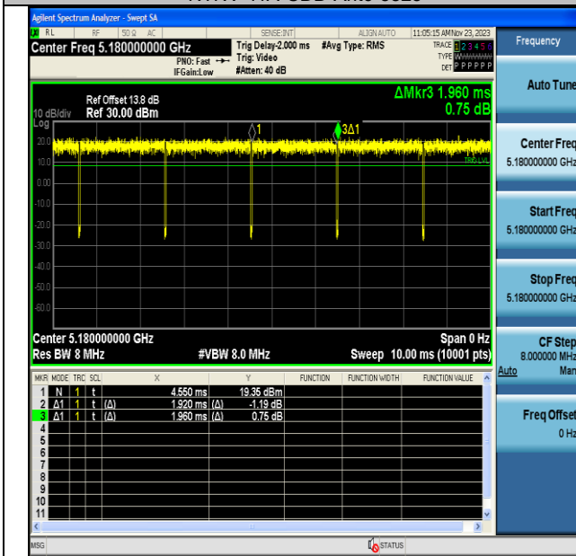
NTVN-11N20MIMO-Ant6-5180
