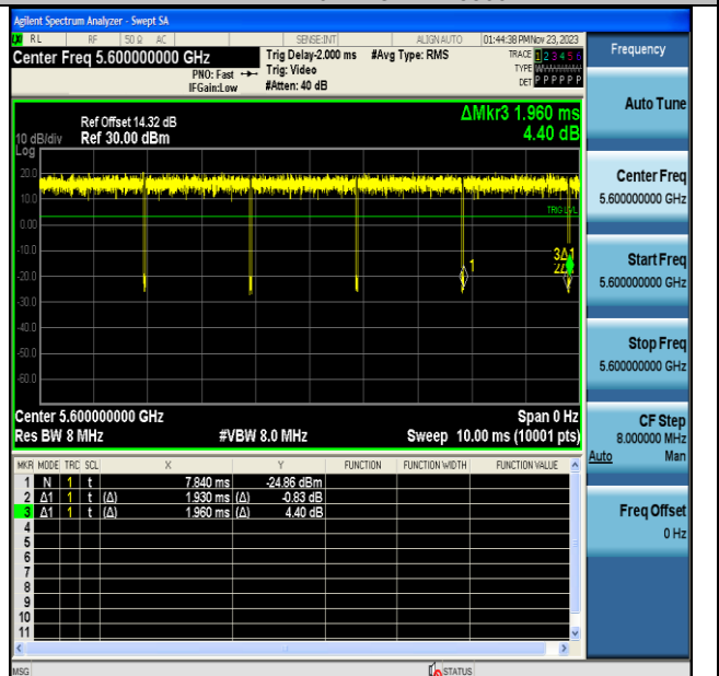
NTVN-11N20MIMO-Ant7-5600
