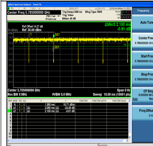
NTNV-11A-CDD-Ant6-5785
