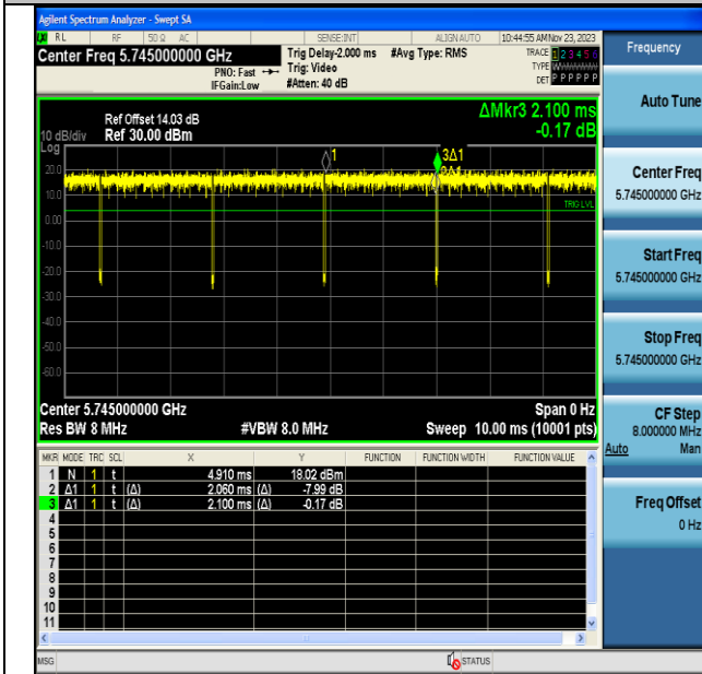
NTNV-11A-CDD-Ant6-5745
