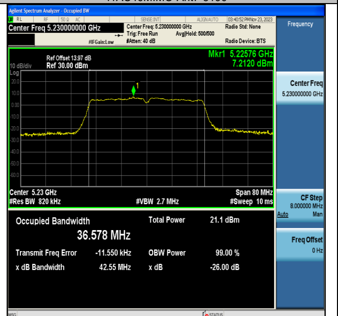
11AC40MIMO-Ant7-5230
