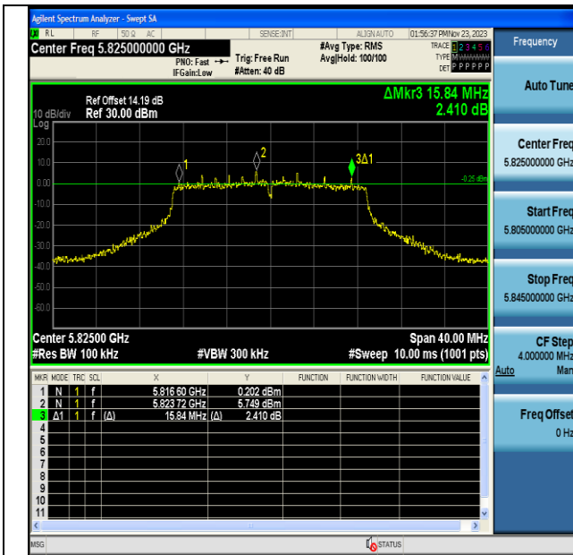
11N20MIMO-Ant6-5825-PASS
