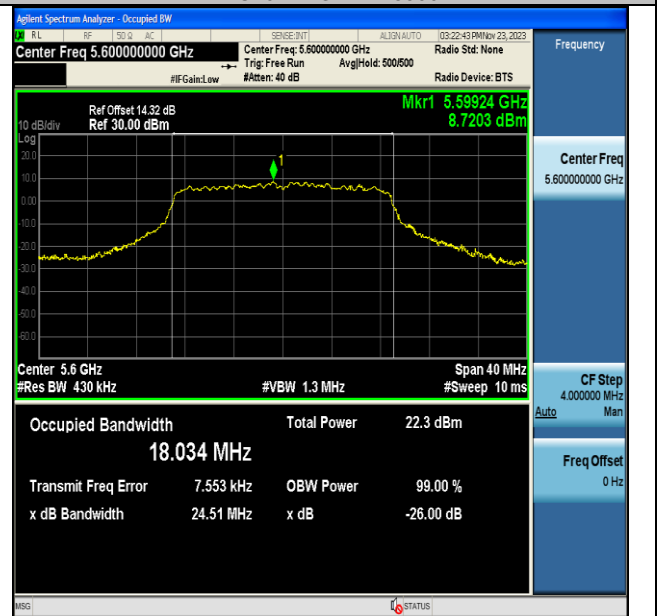
11AC20MIMO-Ant7-5600
