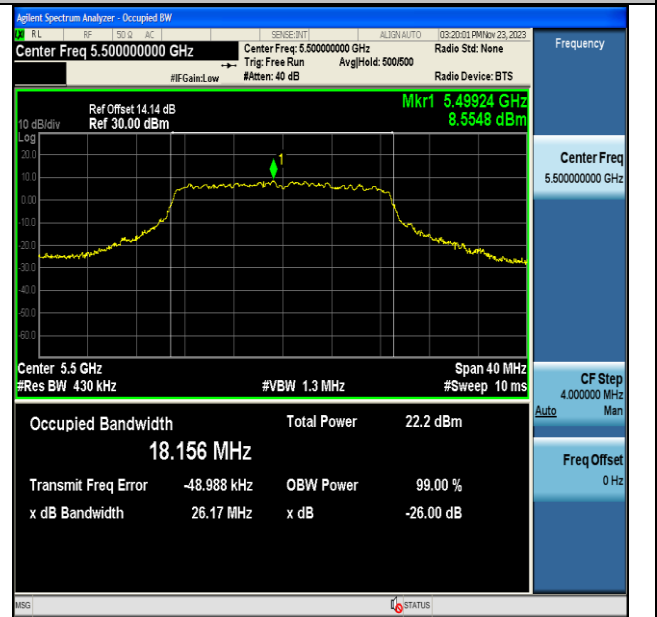
11AC20MIMO-Ant7-5500
