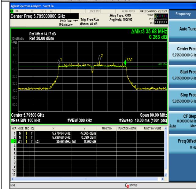
11AC40MIMO-Ant6-5795-PASS
