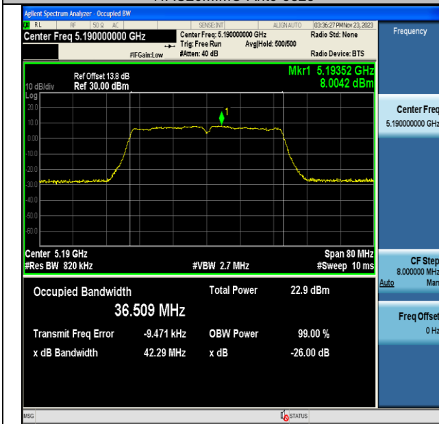
11AC40MIMO-Ant6-5190
