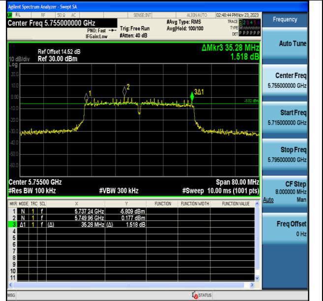
11N40MIMO-Ant7-5755-PASS
