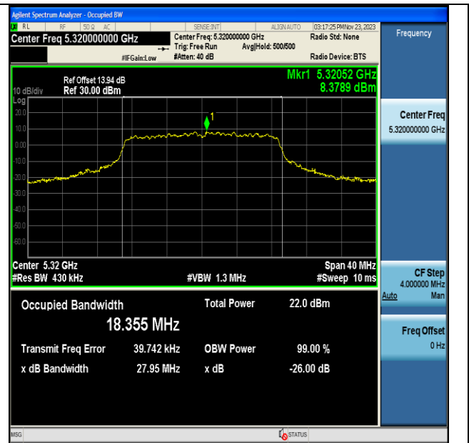
11AC20MIMO-Ant7-5320
