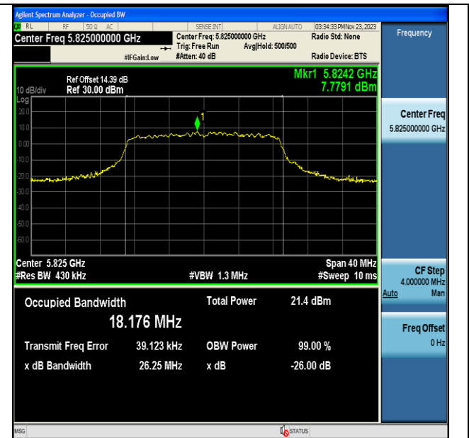
11AC20MIMO-Ant7-5825
