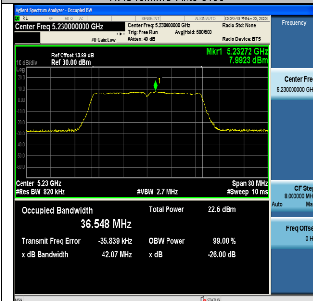
11AC40MIMO-Ant6-5230
