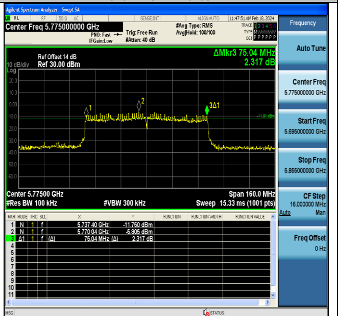
11AC80MIMO-Ant7-5775-PASS
