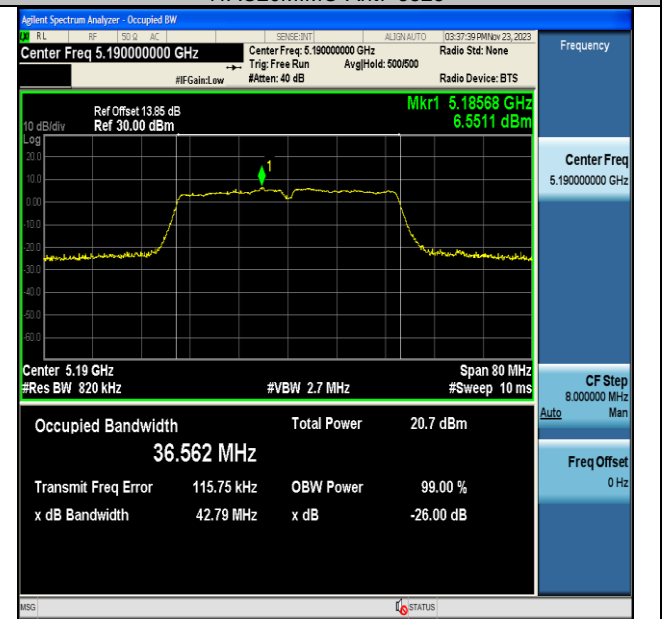
11AC40MIMO-Ant7-5190
