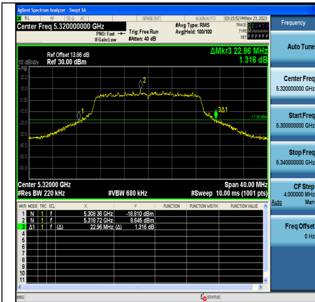
11AC20MIMO-Ant6-5320
