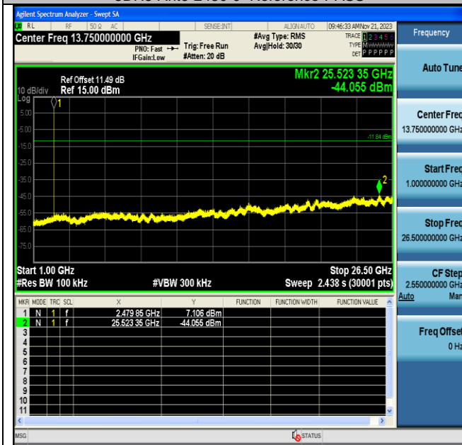
3DH5-Ant6-2480-1000~26500-PASS
