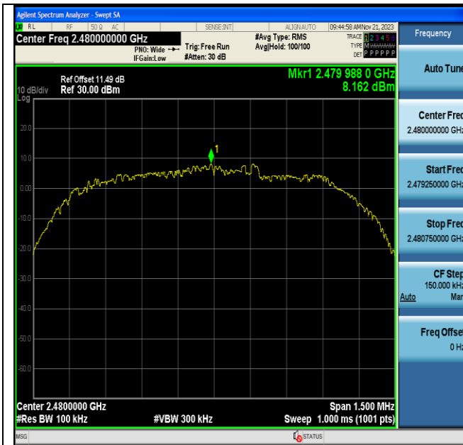
3DH5-Ant6-2480-0~Reference-PASS
