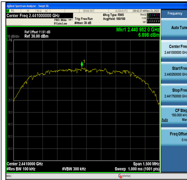
3DH5-Ant6-2441-0~Reference-PASS
