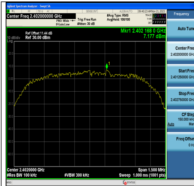
3DH5-Ant6-2402-0~Reference-PASS
