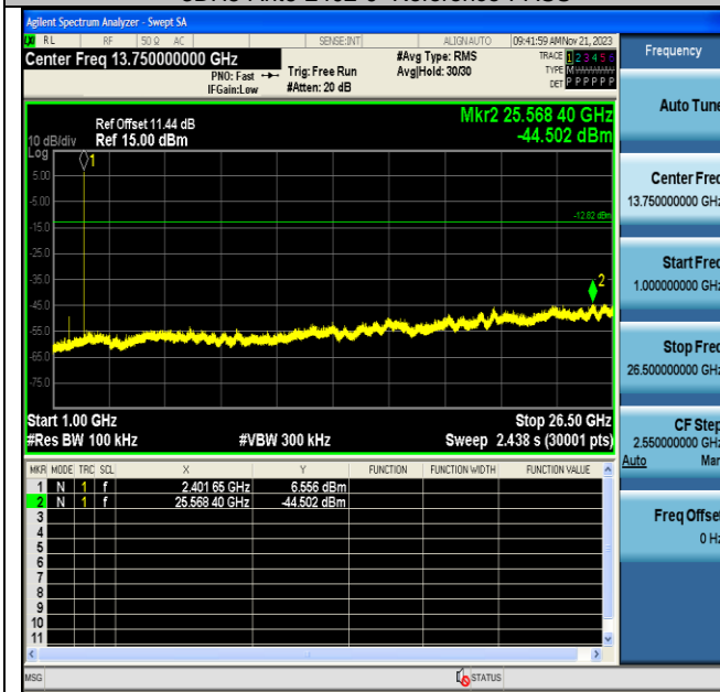
3DH5-Ant6-2402-1000~26500-PASS
