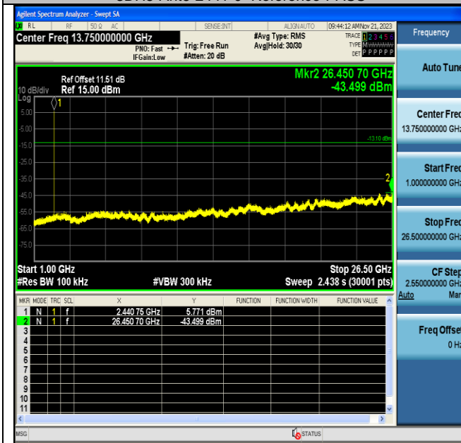
3DH5-Ant6-2441-1000~26500-PASS
