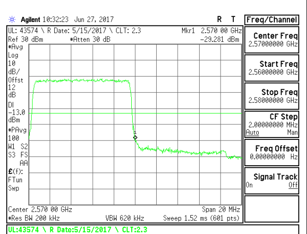
LTE B7 10MHz QPSK High Channel FRB
