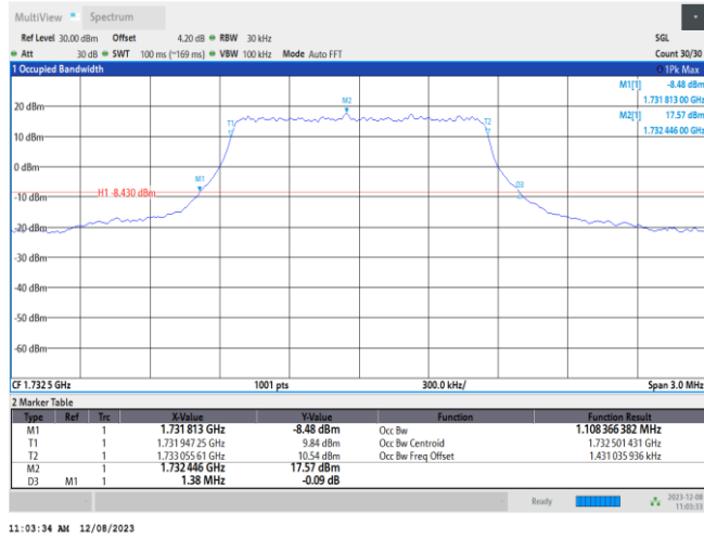
Band4-1.4MHz-16QAM-20175-6RB#0
