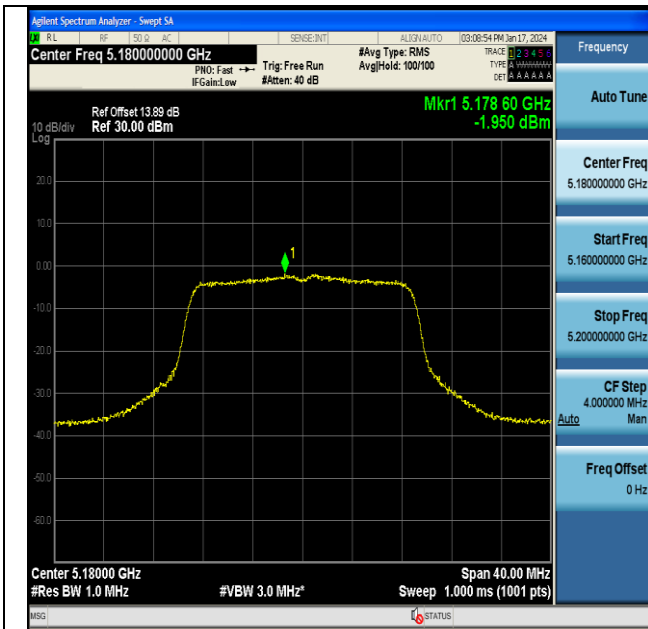
11N20MIMO-Ant6-5180-PASS
