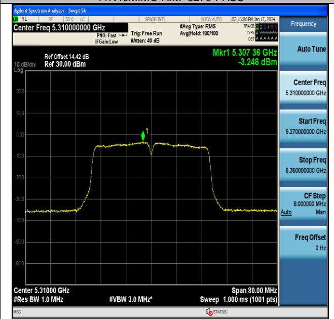
11N40MIMO-Ant7-5310-PASS
