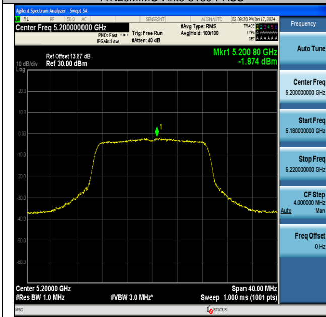
11N20MIMO-Ant6-5200-PASS
