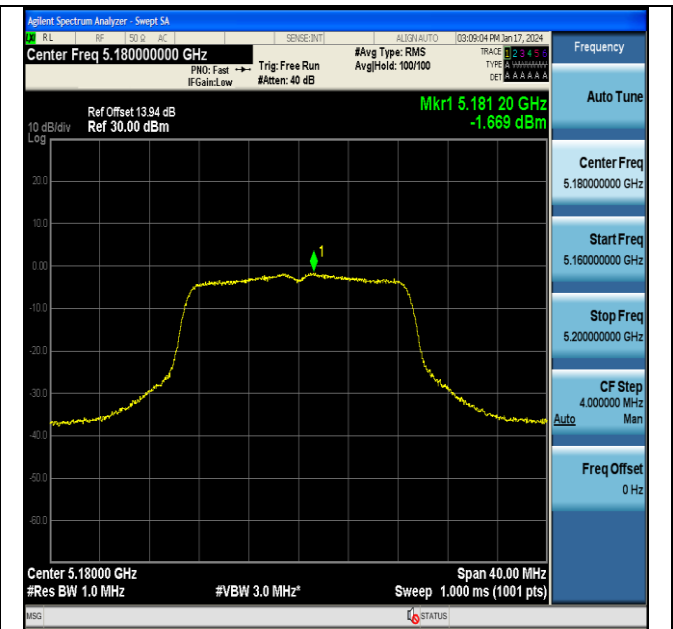
11N20MIMO-Ant7-5180-PASS
