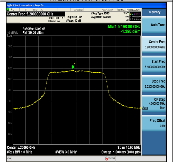
11N20MIMO-Ant7-5200-PASS
