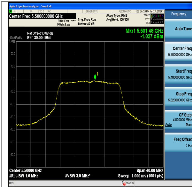
11A-CDD-Ant6-5500-PASS
