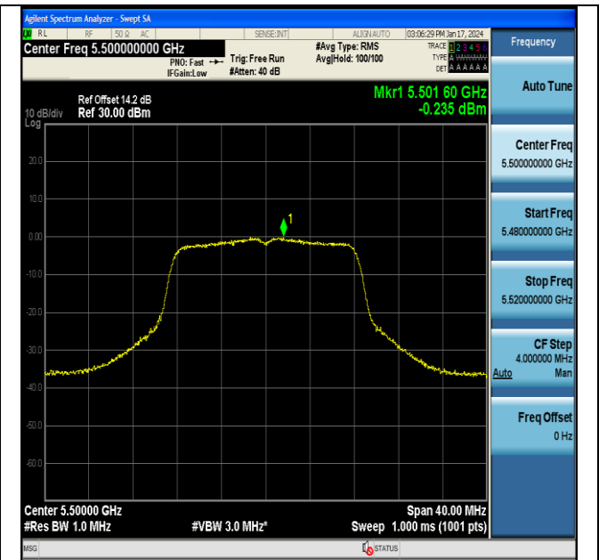
11A-CDD-Ant7-5500-PASS
