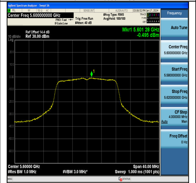
11A-CDD-Ant7-5600-PASS
