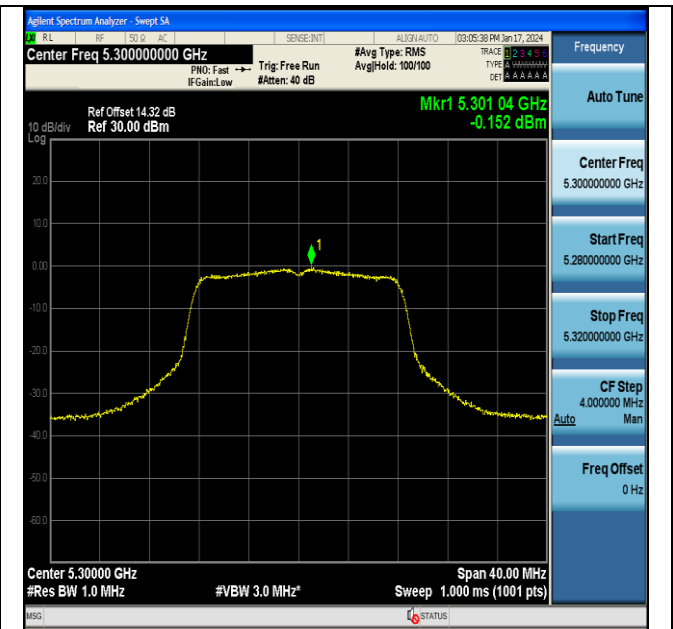
11A-CDD-Ant7-5300-PASS
