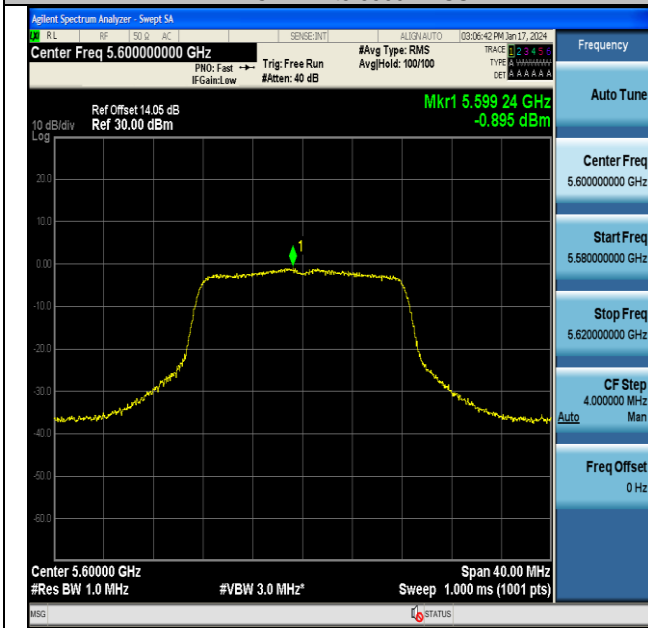
11A-CDD-Ant6-5600-PASS
