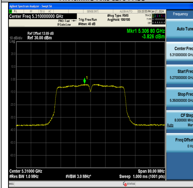
11N40MIMO-Ant6-5310-PASS
