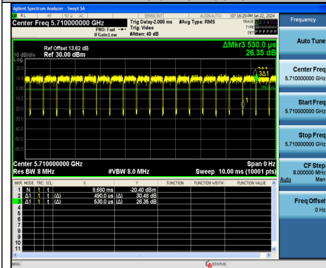
NTNV-11AC40MIMO-Ant6-5710
