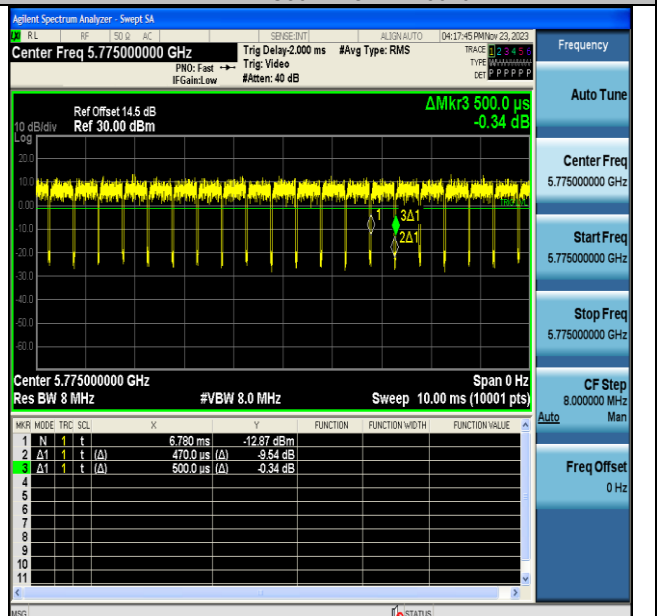
NTNV-11AC80MIMO-Ant7-5775
