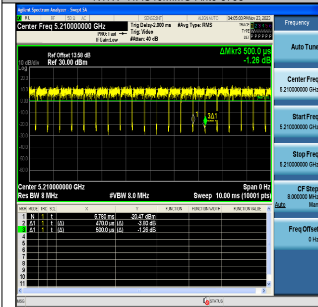
NTNV-11AC80MIMO-Ant6-5210
