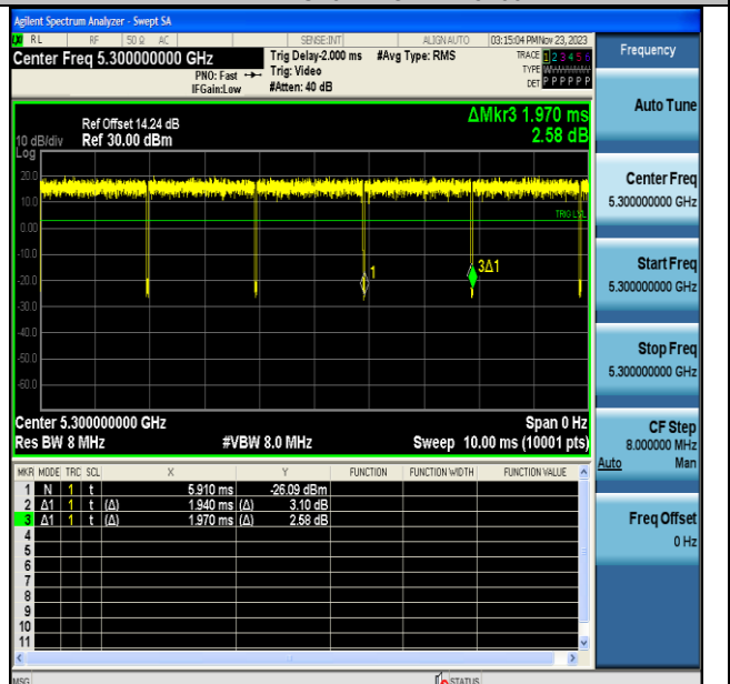
NTNV-11AC20MIMO-Ant7-5300
