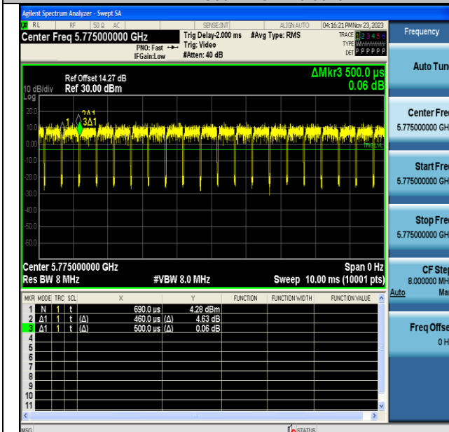
NTNV-11AC80MIMO-Ant6-5775
