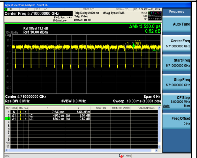
NTNV-11AC40MIMO-Ant7-5710
