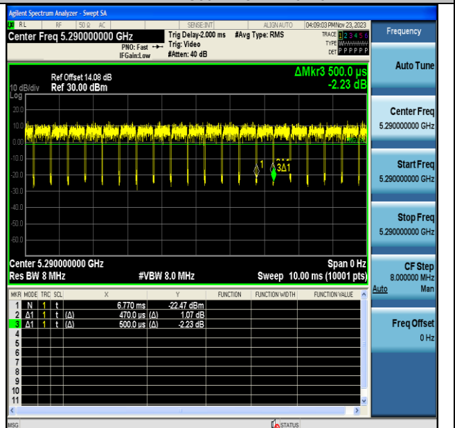
NTNV-11AC80MIMO-Ant7-5290
