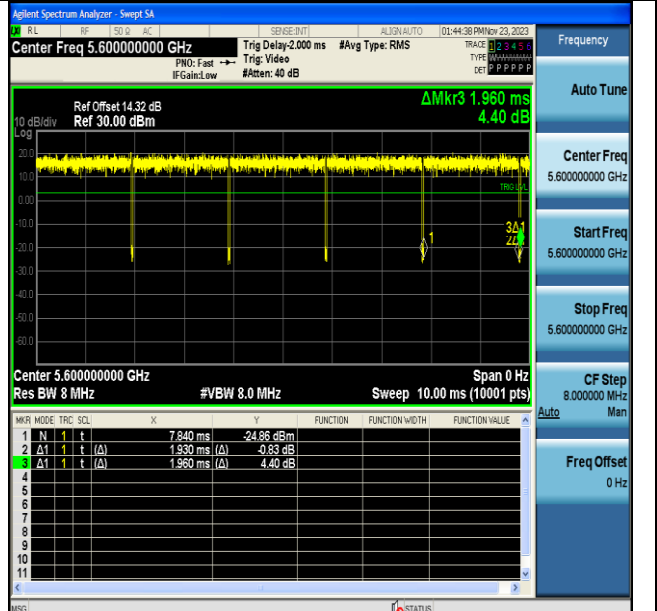
NTV-11N20MIMO-Ant7-5600
