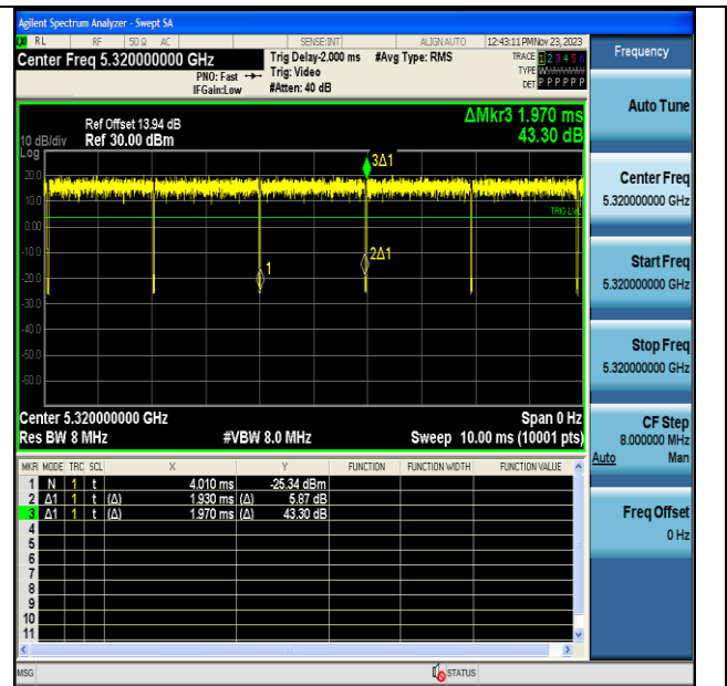
NTV-11N20MIMO-Ant7-5320
