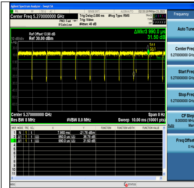
NTVN-11N40MIMO-Ant6-5270
