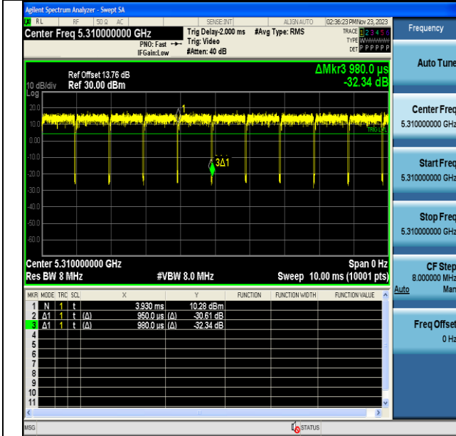
NTVN-11N40MIMO-Ant6-5310
