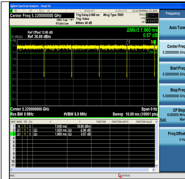
NTV-11N20MIMO-Ant6-5320
