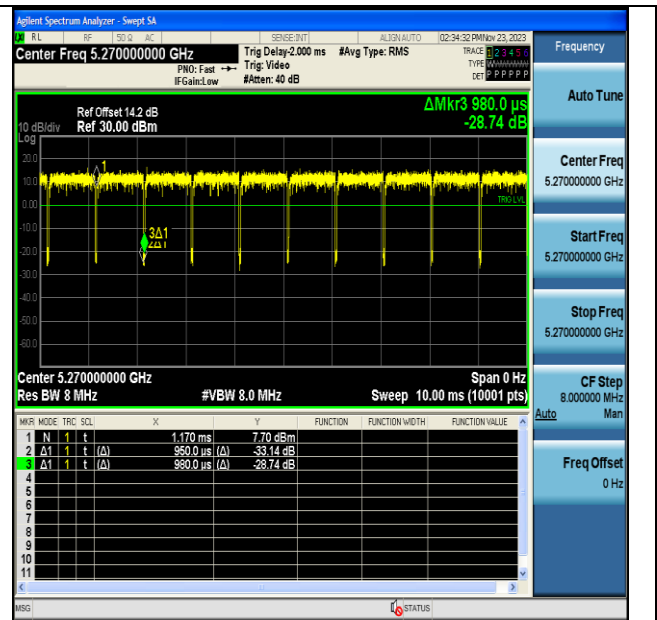
NTVN-11N40MIMO-Ant7-5270
