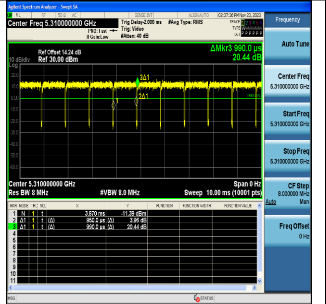
NTVN-11N40MIMO-Ant7-5310
