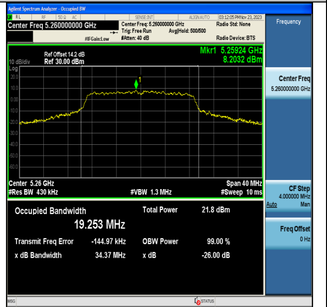
11AC20MIMO-Ant7-5260
