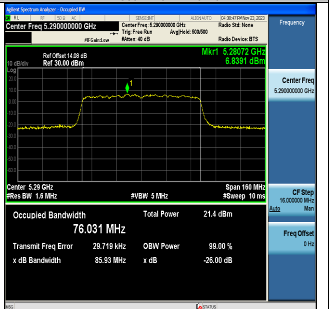
11AC80MIMO-Ant7-5290
