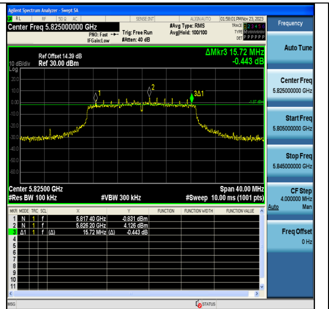
11N20MIMO-Ant7-5825-PASS
