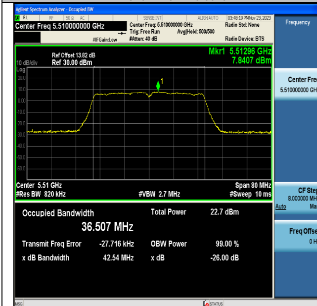
11AC40MIMO-Ant6-5510
