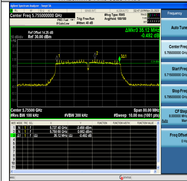
11N40MIMO-Ant6-5755-PASS
