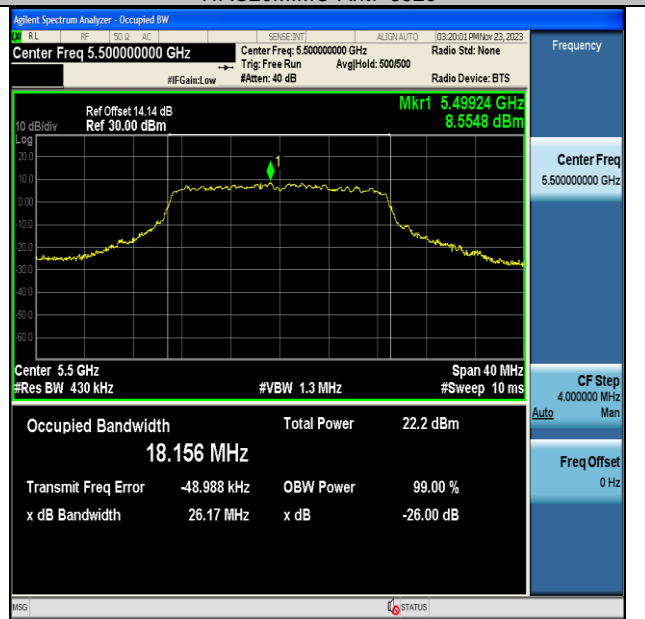
11AC20MIMO-Ant7-5500
