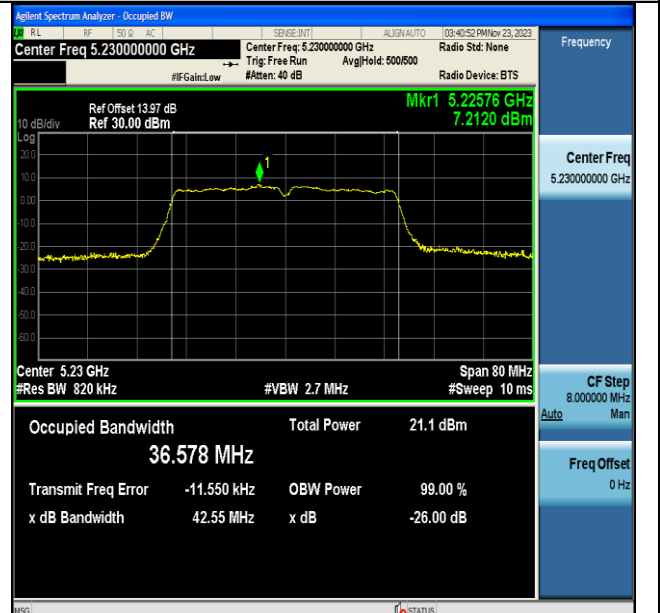
11AC40MIMO-Ant7-5230
