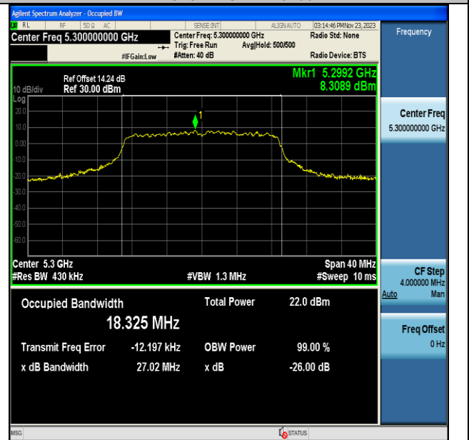
11AC20MIMO-Ant7-5300
