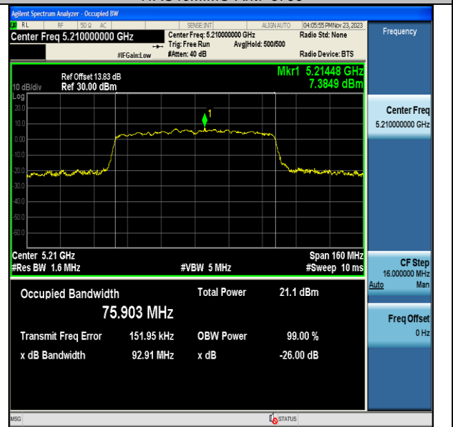
11AC80MIMO-Ant7-5210
