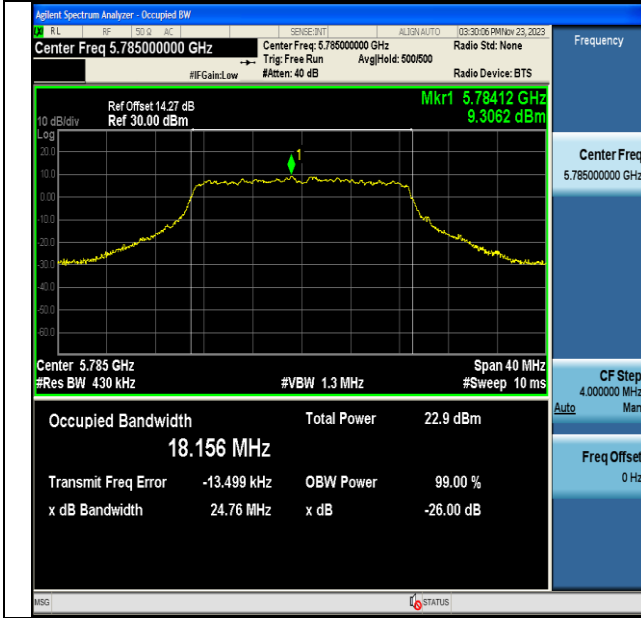
11AC20MIMO-Ant6-5785
