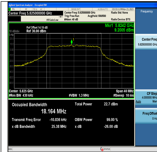
11AC20MIMO-Ant6-5825
