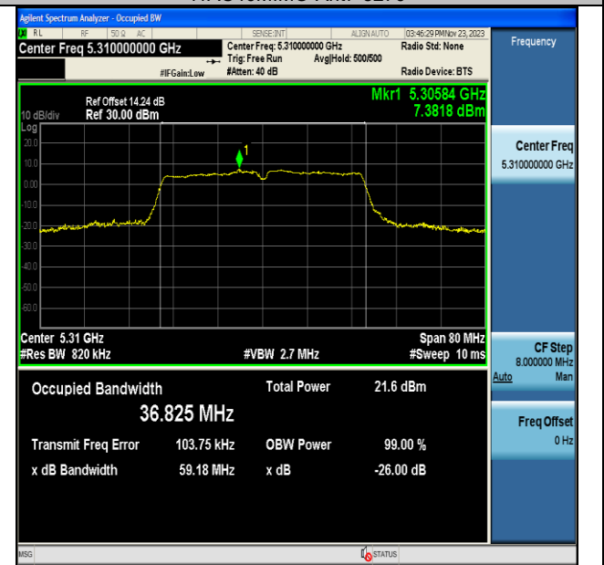
11AC40MIMO-Ant7-5310
