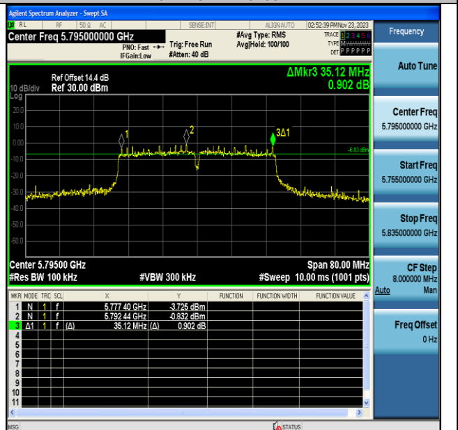
11N40MIMO-Ant7-5795-PASS
