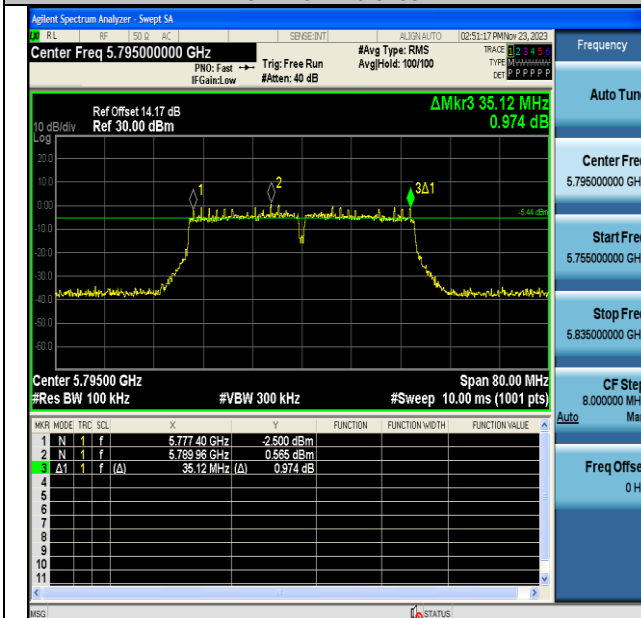
11N40MIMO-Ant6-5795-PASS
