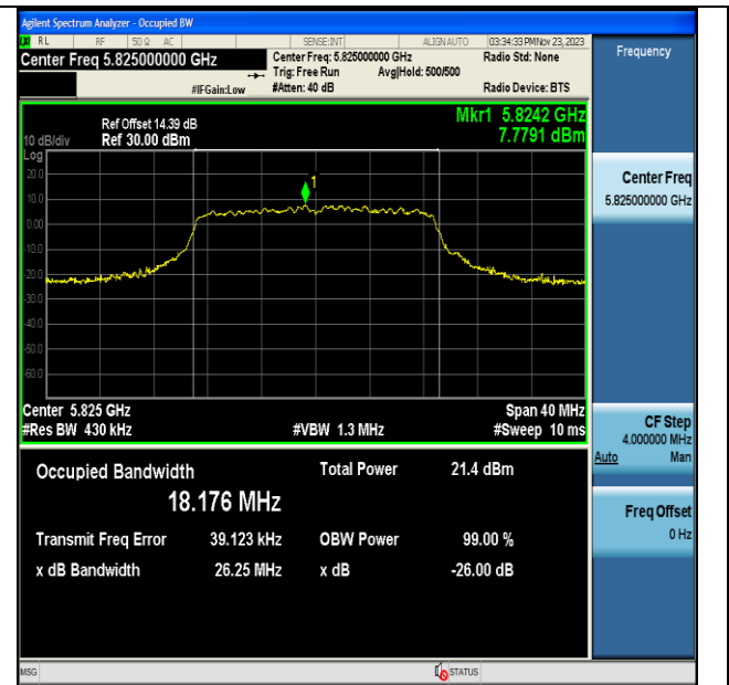
11AC20MIMO-Ant7-5825
