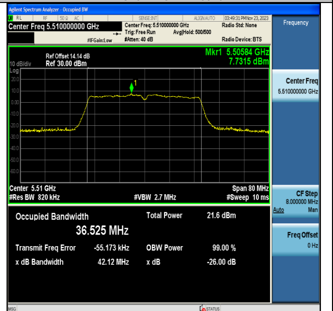
11AC40MIMO-Ant7-5510
