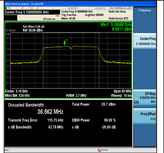
11AC40MIMO-Ant7-5190
