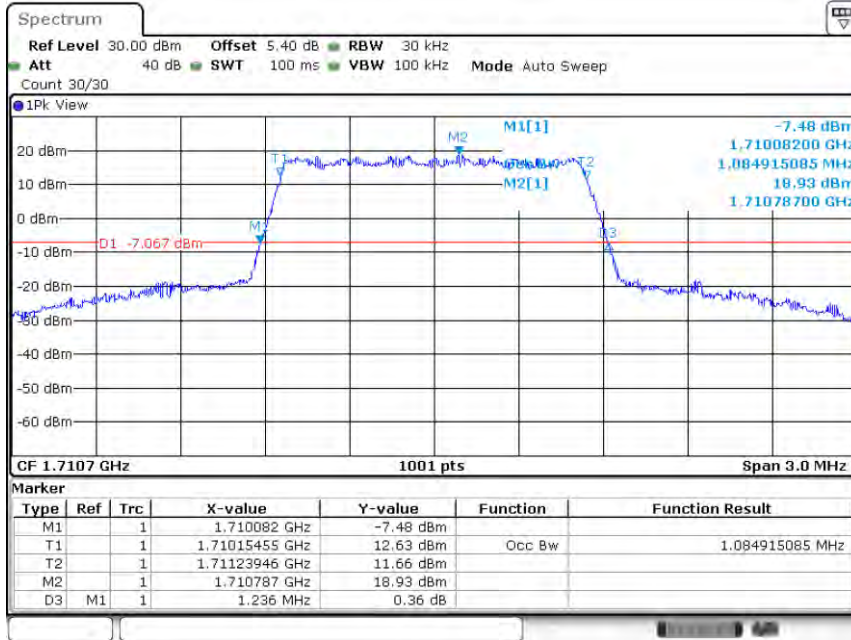
Band4-1.4MHz-QPSK-19957-6RB#0-1.085
