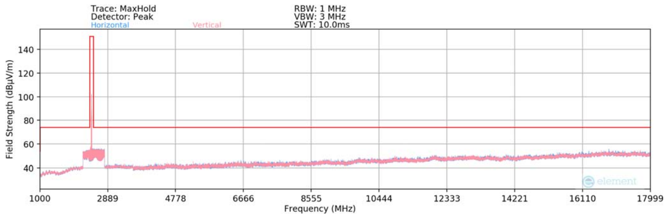
Plot 7-78. Radiated Spurious Plot above 1GHz SISO ANT1 (802.11b – Ch. 6)
