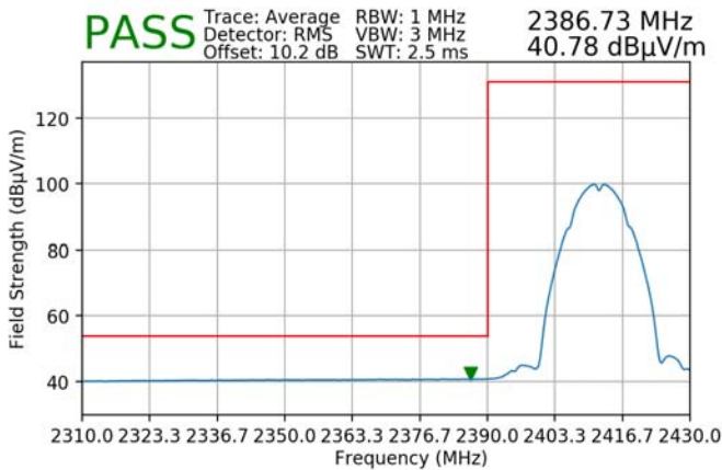
Plot 7-89. Radiated Restricted Lower Band Edge Measurement SISO ANT1 (Average)
