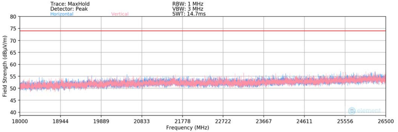
Plot 7-80. Radiated Spurious Plot above 18GHz SISO ANT1
