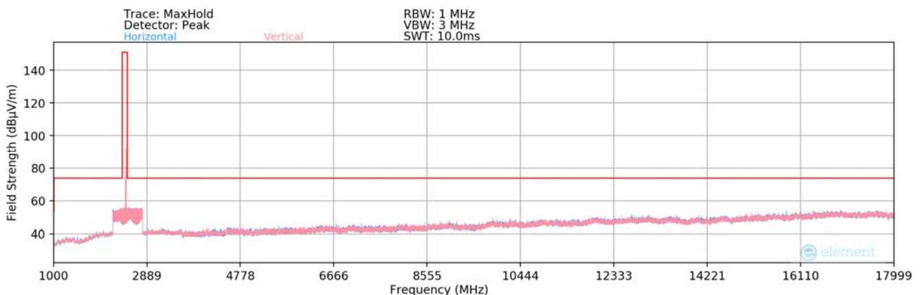
Plot 7-83. Radiated Spurious Plot above 1GHz SISO ANT2 (802.11b – Ch. 11)
