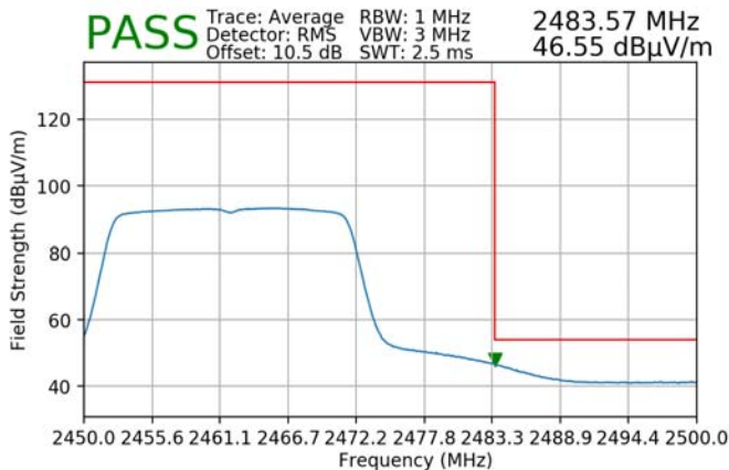
Plot 7-99. Radiated Restricted Upper Band Edge Measurement MIMO (Average)
