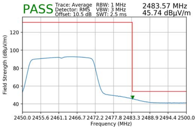
Plot 7-101. Radiated Restricted Band Edge Measurement MIMO with WCP (Average)
