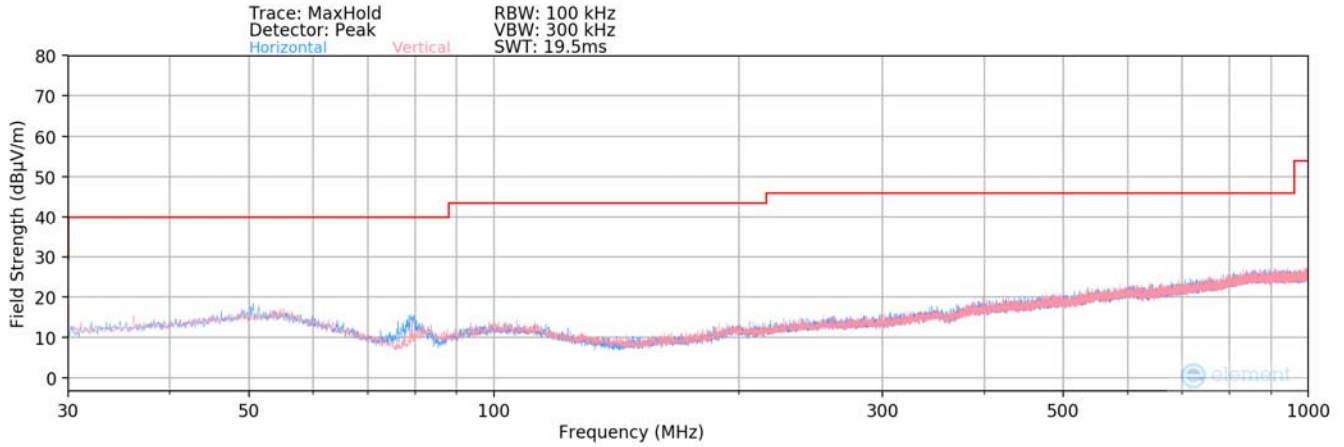
Plot 7-103. Radiated Spurious Plot below 1GHz SISO ANT1
