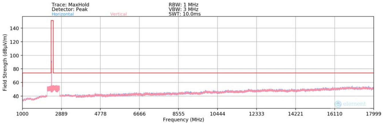
Plot 7-81. Radiated Spurious Plot above 1GHz SISO ANT2 (802.11b – Ch. 1)
