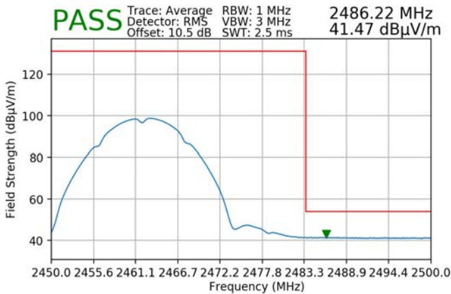
Plot 7-91. Radiated Restricted Upper Band Edge Measurement SISO ANT1 (Average)
