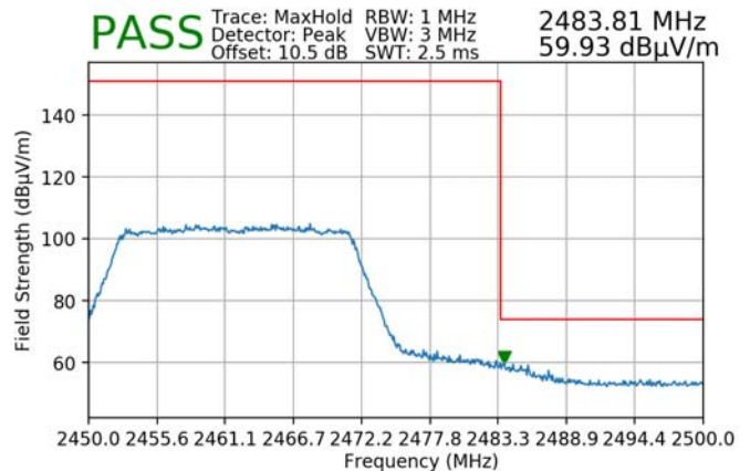
Plot 7-100. Radiated Restricted Upper Band Edge Measurement MIMO (Peak)
