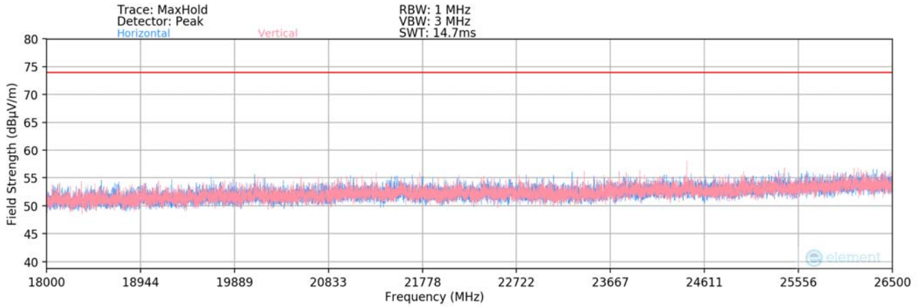
Plot 7-84. Radiated Spurious Plot above 18GHz SISO ANT2
