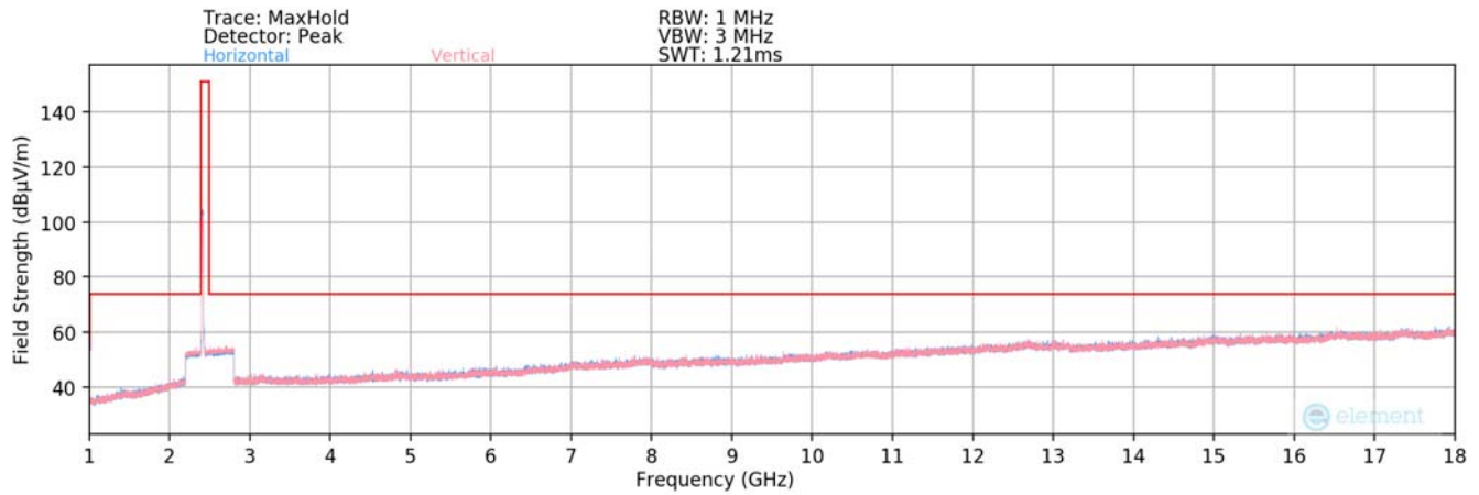
Plot 7-85. Radiated Spurious Plot above 1GHz MIMO/CDD (802.11g – Ch. 1)
