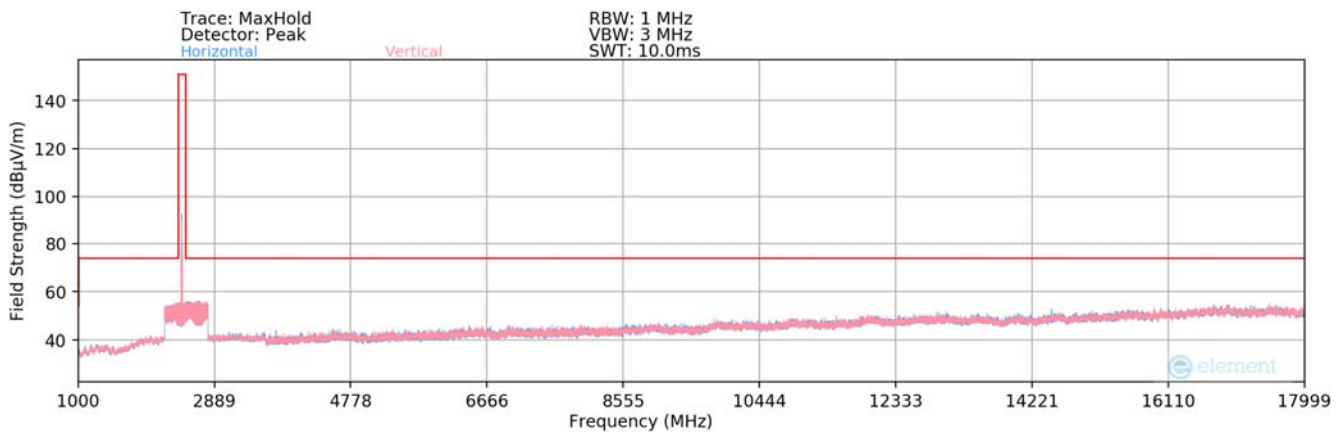
Plot 7-82. Radiated Spurious Plot above 1GHz SISO ANT2 (802.11b – Ch. 6)
