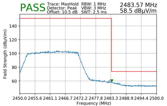
Plot 7-102. Radiated Restricted Band Edge Measurement MIMO with WCP (Peak)
