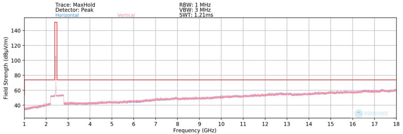
Plot 7-86. Radiated Spurious Plot above 1GHz MIMO/CDD (802.11g – Ch. 6)
