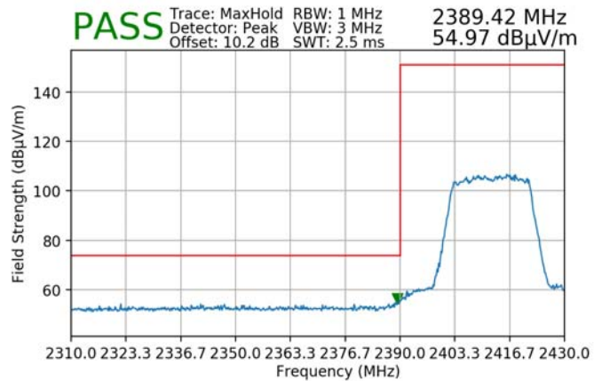
Plot 7-98. Radiated Restricted Lower Band Edge Measurement MIMO (Peak)
