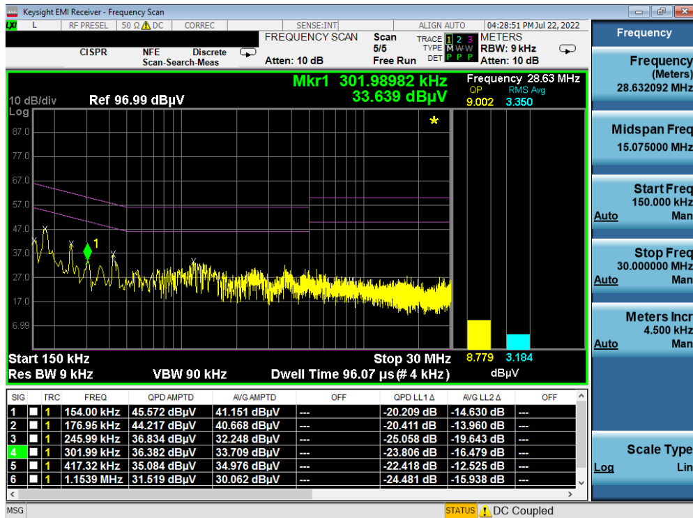
Plot 7-109. Line Conducted Plot with 802.11b (N) _WCP
