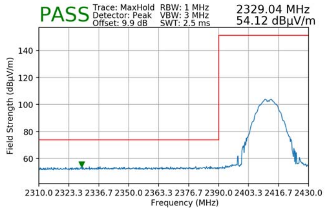
Plot 7-90. Radiated Restricted Lower Band Edge Measurement SISO ANT1 (Peak)
