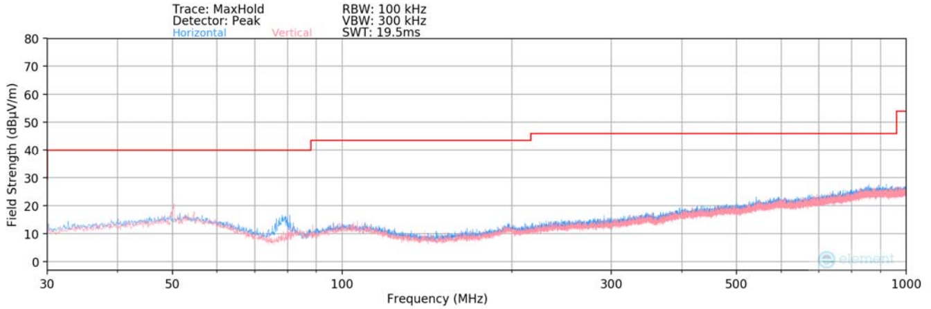
Plot 7-104. Radiated Spurious Plot below 1GHz SISO ANT2
