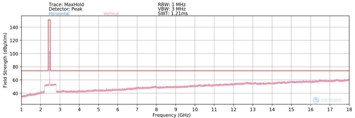
Plot 7-87. Radiated Spurious Plot above 1GHz MIMO/CDD (802.11g – Ch. 11)
