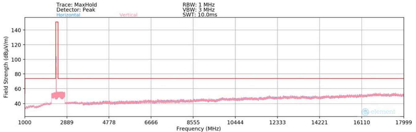
Plot 7-77. Radiated Spurious Plot above 1GHz SISO ANT1 (802.11b – Ch. 1)
