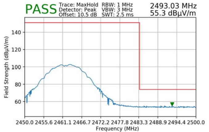
Plot 7-92. Radiated Restricted Upper Band Edge Measurement SISO ANT1 (Peak)
