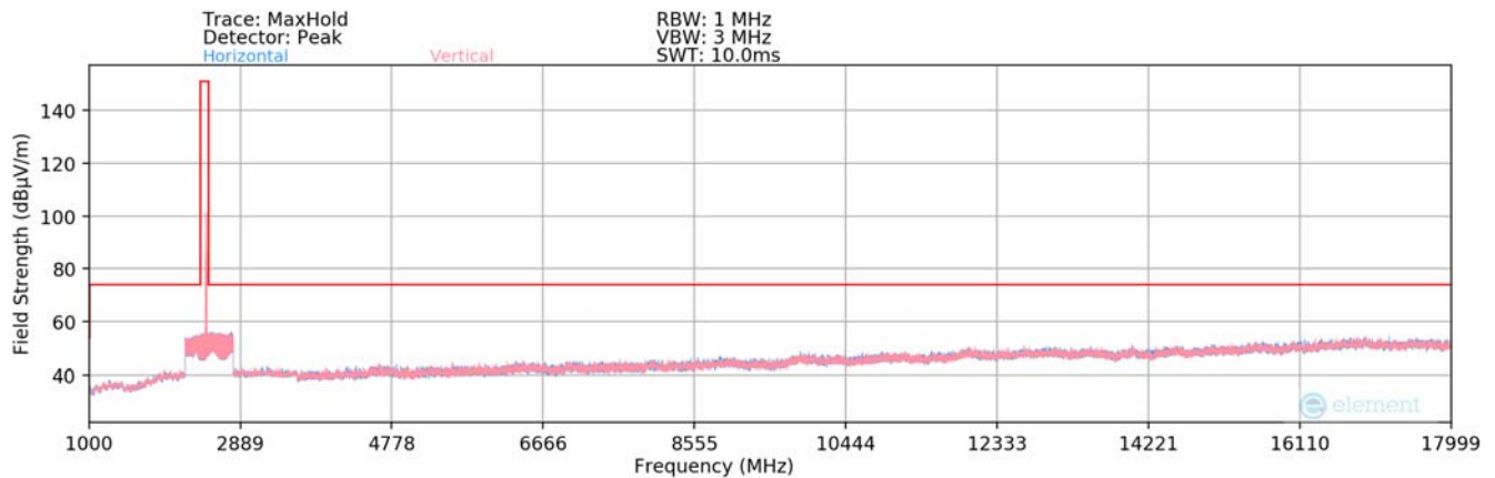
Plot 7-79. Radiated Spurious Plot above 1GHz SISO ANT1 (802.11b – Ch. 11)
