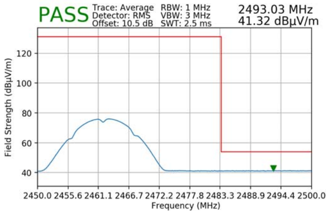
Plot 7-95. Radiated Restricted Upper Band Edge Measurement SISO ANT2 (Average)
