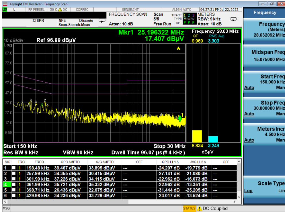
Plot 7-108. Line Conducted Plot with 802.11b (L1) _WCP
