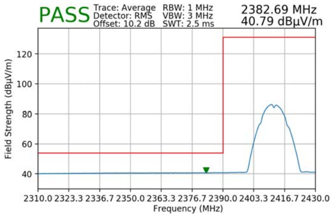
Plot 7-93. Radiated Restricted Lower Band Edge Measurement SISO ANT2 (Average)
