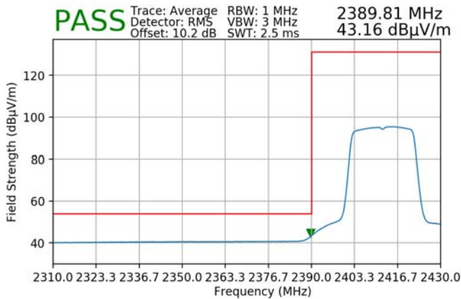
Plot 7-97. Radiated Restricted Lower Band Edge Measurement MIMO (Average)
