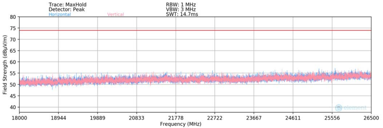
Plot 7-88. Radiated Spurious Plot above 18GHz MIMO/CDD
