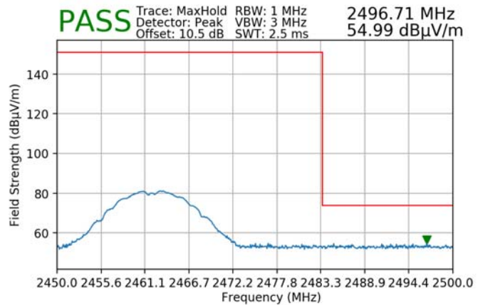
Plot 7-96. Radiated Restricted Upper Band Edge Measurement SISO ANT2 (Peak)
