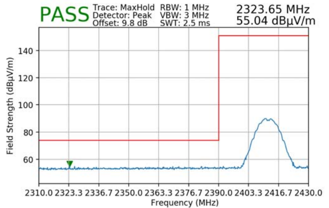
Plot 7-94. Radiated Restricted Lower Band Edge Measurement SISO ANT2 (Peak)
