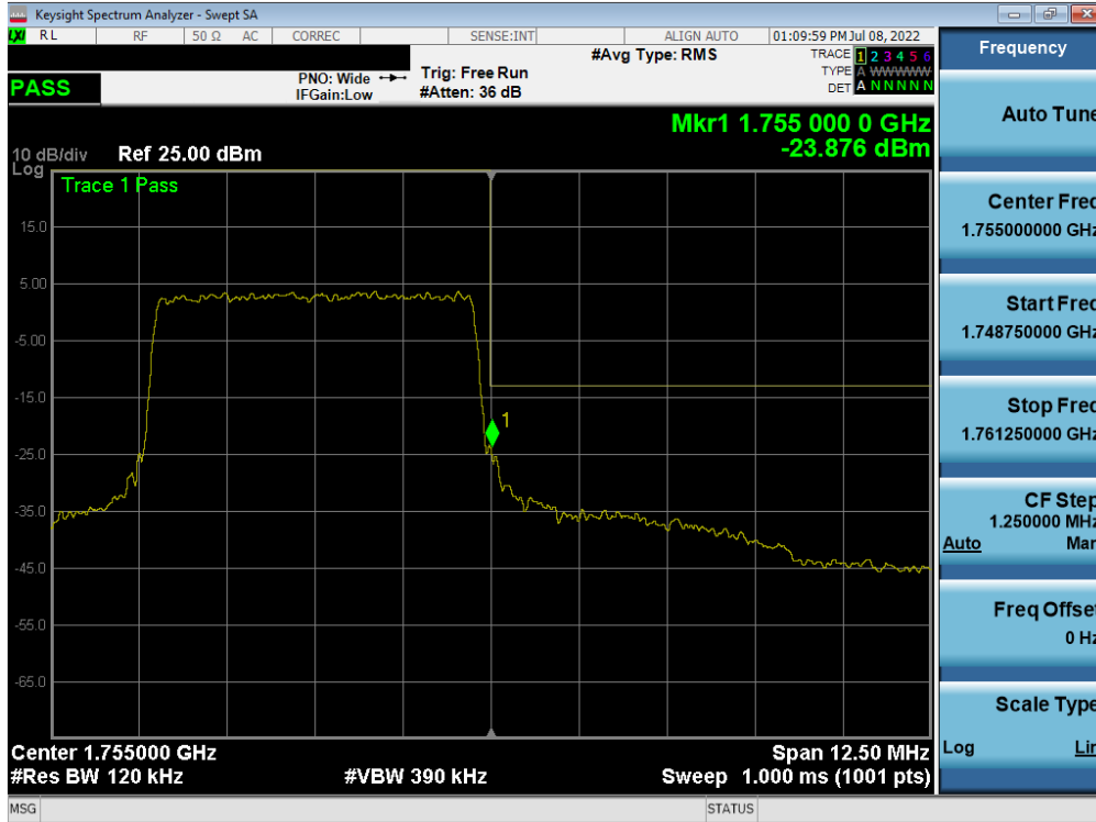
Plot 7-110. Upper Band Edge Plot (LTE Band 4 - 5MHz QPSK – Full RB)
