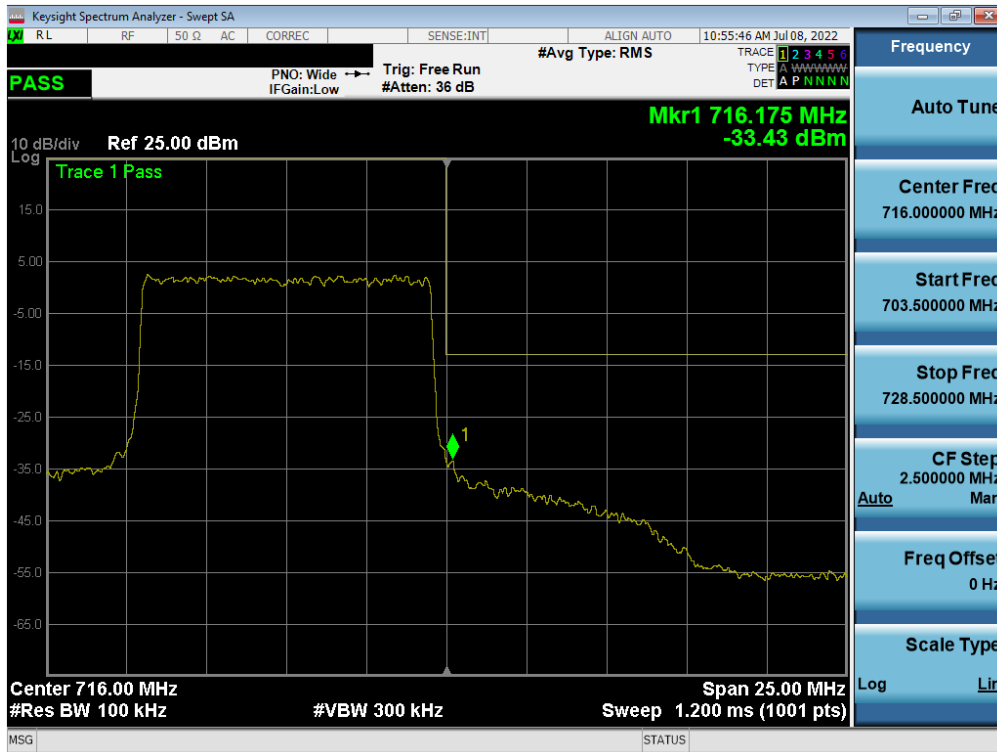
Plot 7-70. Upper Band Edge Plot (LTE Band 12/17 - 10MHz QPSK – Full RB)
