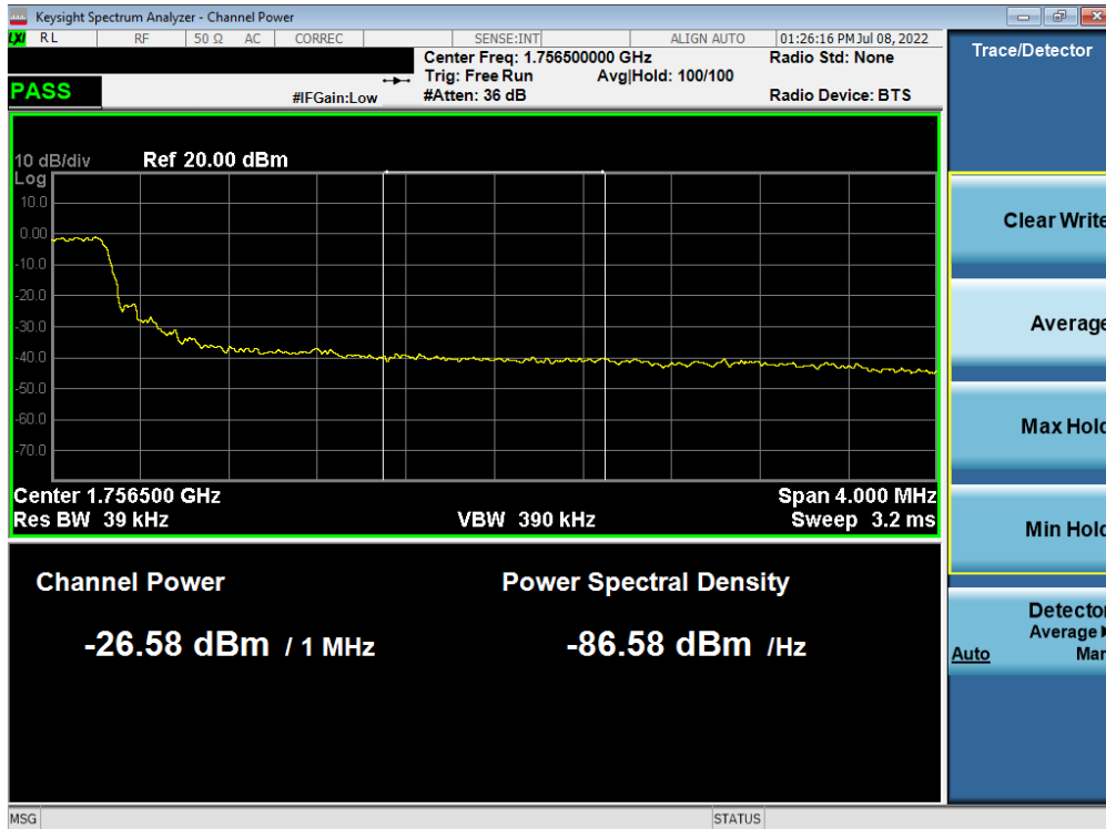
Plot 7-111. Upper Extended Band Edge Plot (LTE Band 4 - 5MHz QPSK – Full RB)
