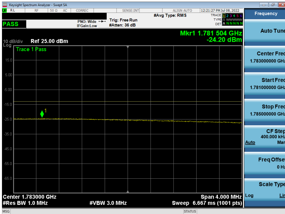
Plot 7-95. Channel Edge Plot (LTE Band 66 - 20MHz QPSK – Full RB)
