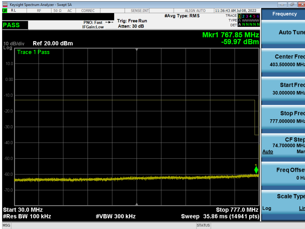
Plot 7-47. Conducted Spurious Plot (LTE Band 13 - 10MHz QPSK - 1 RB)
