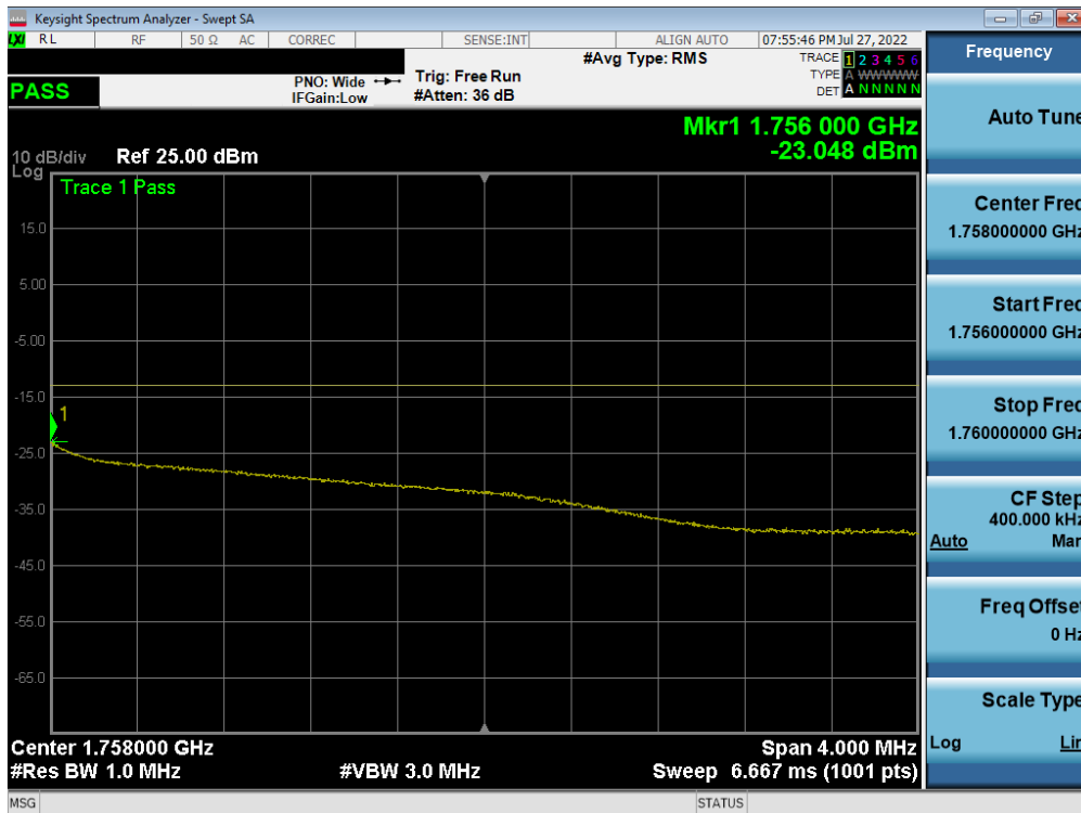
Plot 7-89. Upper Extended Band Edge Plot (WCDMA AWS – Ch. 1513)
