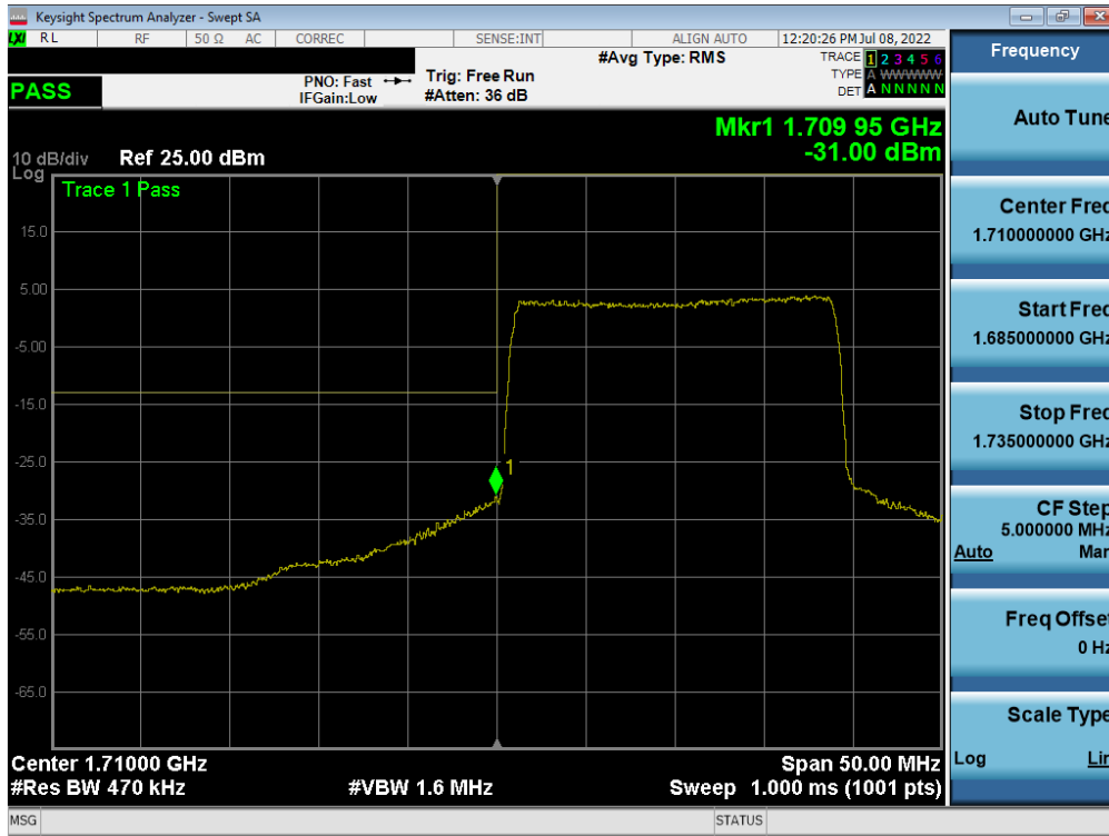
Plot 7-90. Lower Band Edge Plot (LTE Band 66/4 - 20MHz QPSK – Full RB)
