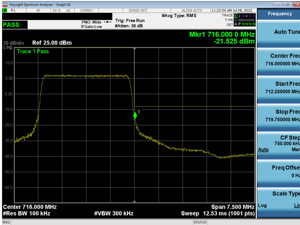
Plot 7-75. Upper Band Edge Plot (LTE Band 12 - 3MHz QPSK – Full RB)
