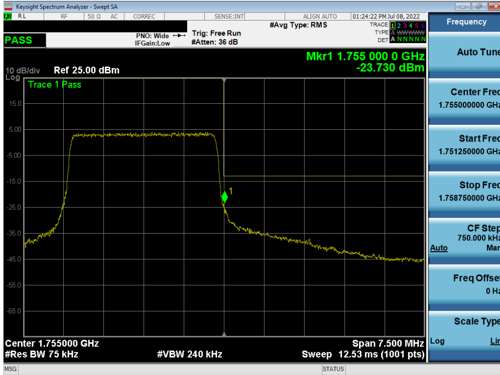
Plot 7-116. Upper Band Edge Plot (LTE Band 4 - 3MHz QPSK – Full RB)
