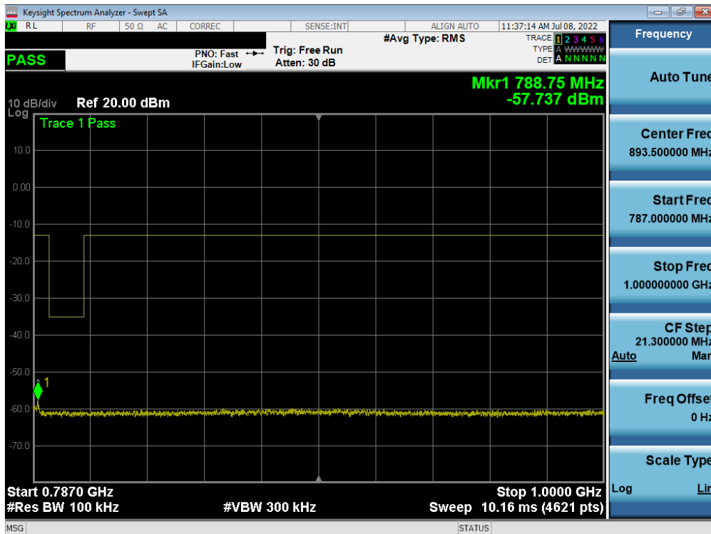
Plot 7-48. Conducted Spurious Plot (LTE Band 13 - 10MHz QPSK - 1 RB)
