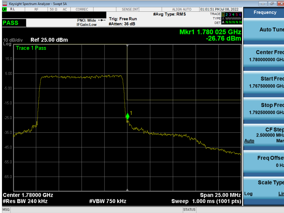
Plot 7-106. Upper Band Edge Plot (LTE Band 66 - 10MHz QPSK – Full RB)
