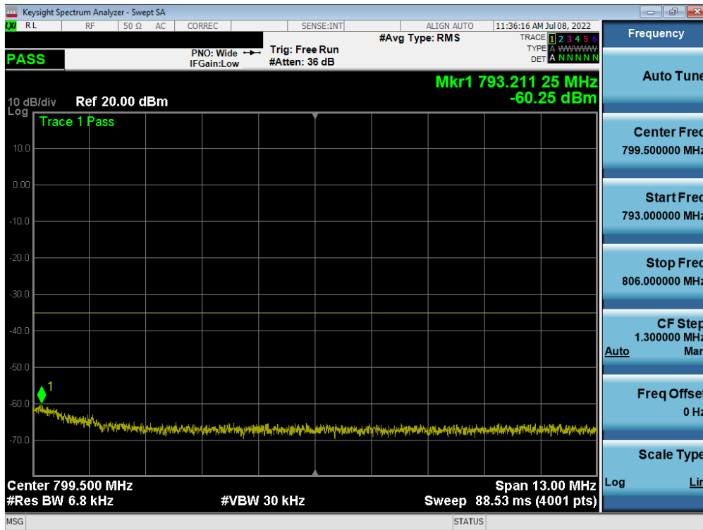
Plot 7-81. Upper Emission Mask Plot (LTE Band 13 - 10MHz QPSK – Full RB)
