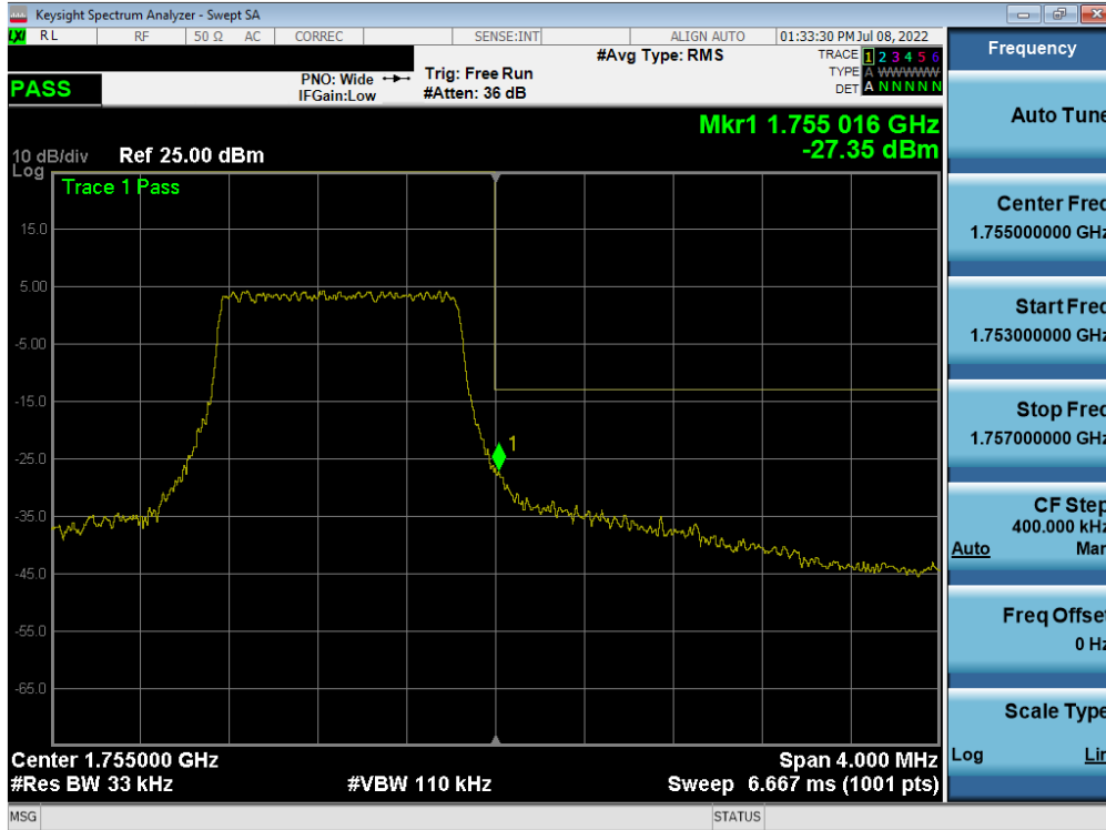
Plot 7-122. Upper Band Edge Plot (LTE Band 4 – 1.4MHz QPSK – Full RB)
