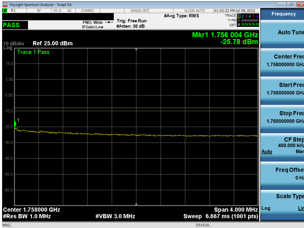
Plot 7-105. Upper Extended Band Edge Plot (LTE Band 4 - 10MHz QPSK – Full RB)
