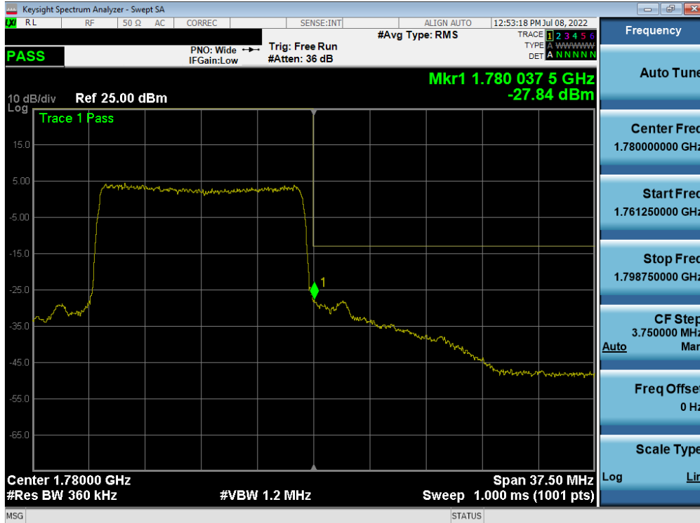
Plot 7-100. Upper Band Edge Plot (LTE Band 66 - 15MHz QPSK - Full RB)
