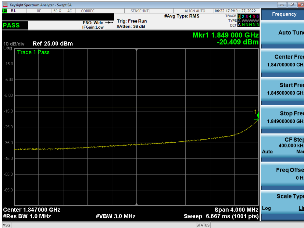
Plot 7-88. Extended Lower Band Edge Plot (WCDMA PCS – Ch. 9262)
