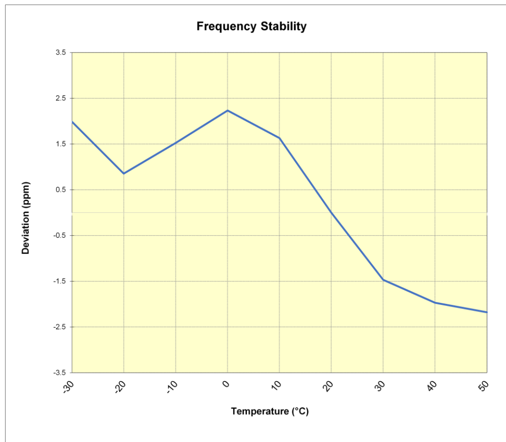
Plot 7-113. GSM/GPRS PCS Frequency Stability Chart
