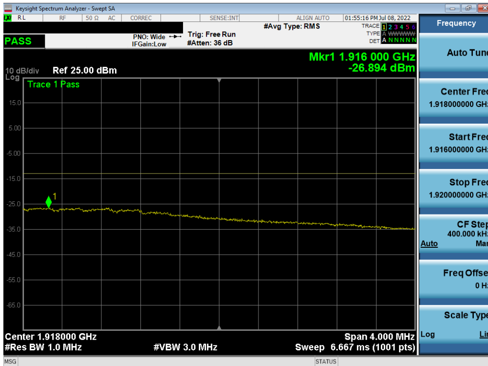
Plot 7-60. Extended Upper Band Edge Plot (LTE Band 25 - 15MHz QPSK – Full RB)
