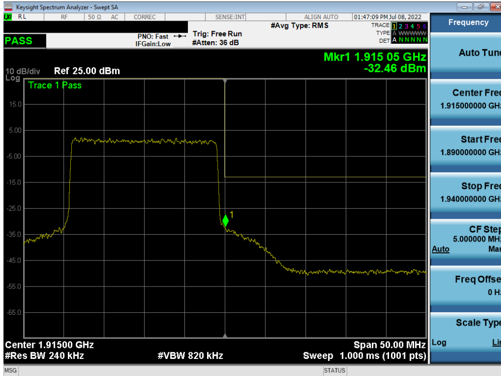
Plot 7-53. Upper Band Edge Plot (LTE Band 25 - 20MHz QPSK – Full RB)
