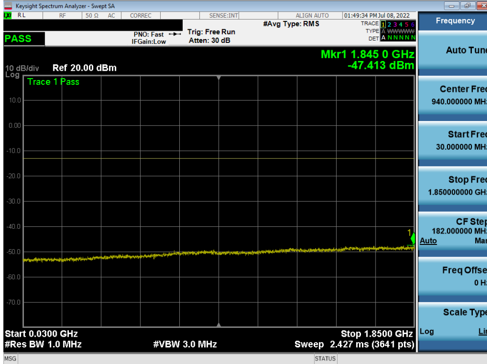
Plot 7-28. Conducted Spurious Plot (LTE Band 25/2 - 20MHz QPSK - 1RB - High Channel)
