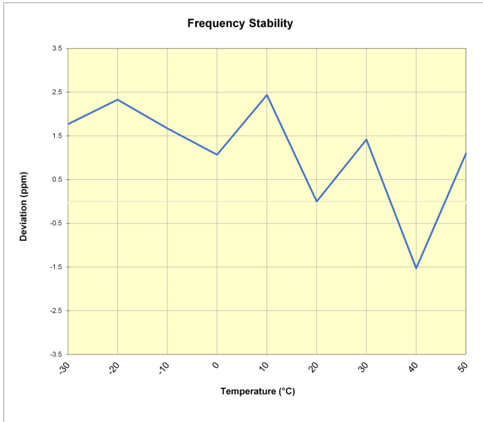
Plot 7-112. LTE Band 25/2 Frequency Stability Chart
