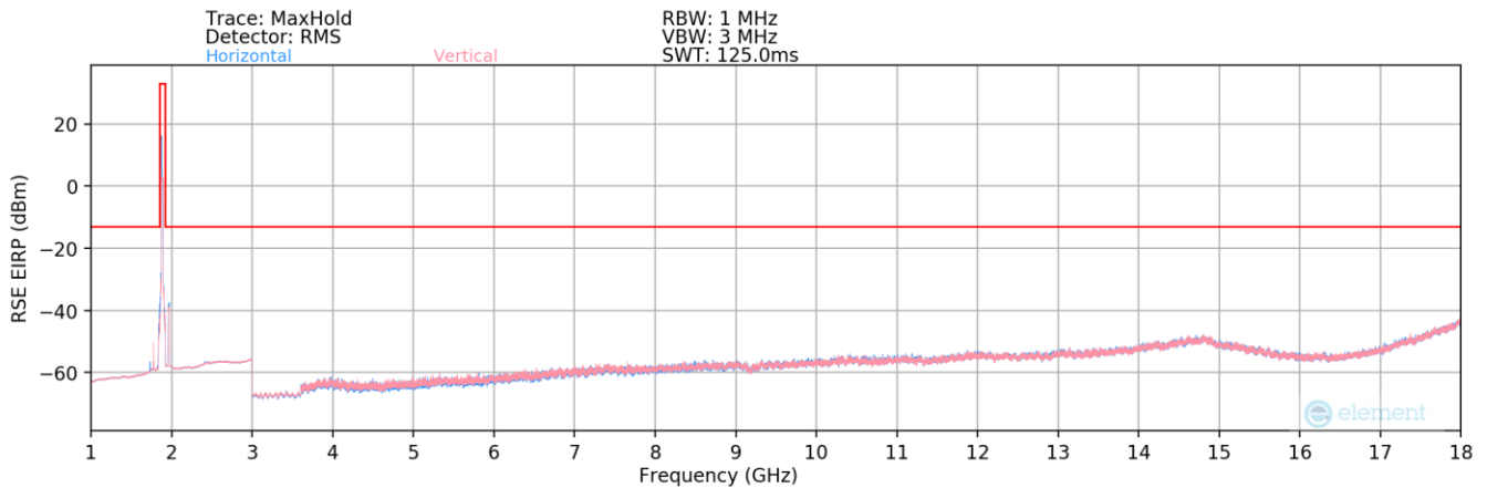
Plot 7-107. Radiated Spurious Plot (LTE Band 25/2)
