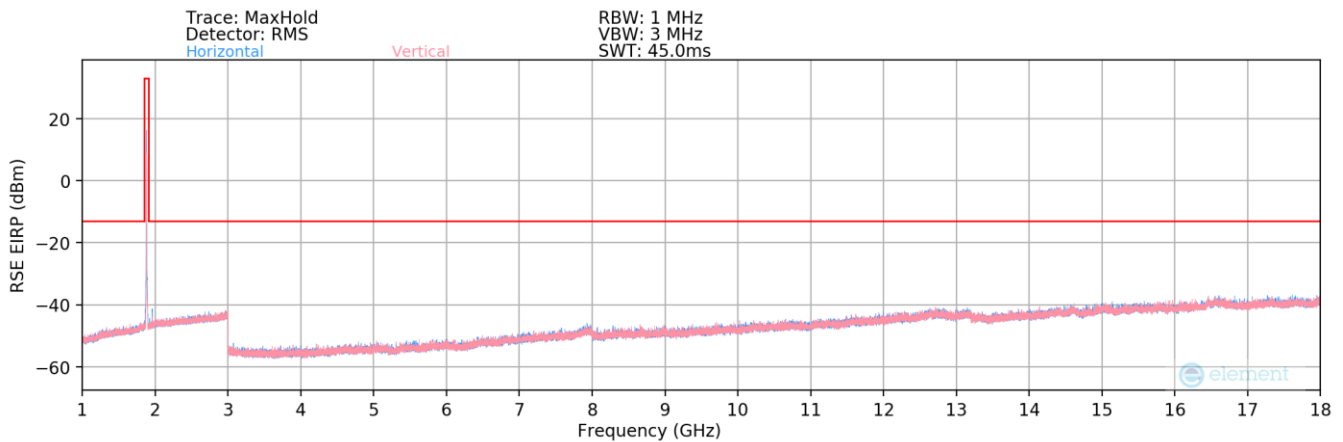
Plot 7-111. Radiated Spurious Plot (WCDMA PCS)
