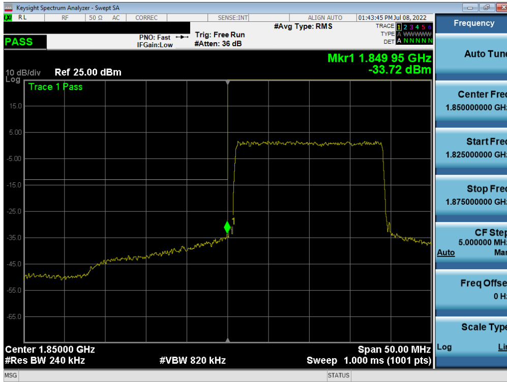
Plot 7-49. Lower Band Edge Plot (LTE Band 25/2 - 20MHz QPSK – Full RB)
