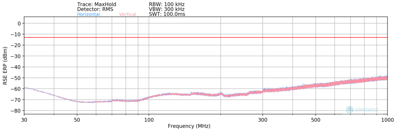
Plot 7-106. Radiated Spurious Plot Below 1GHz (LTE Band 25/2)
