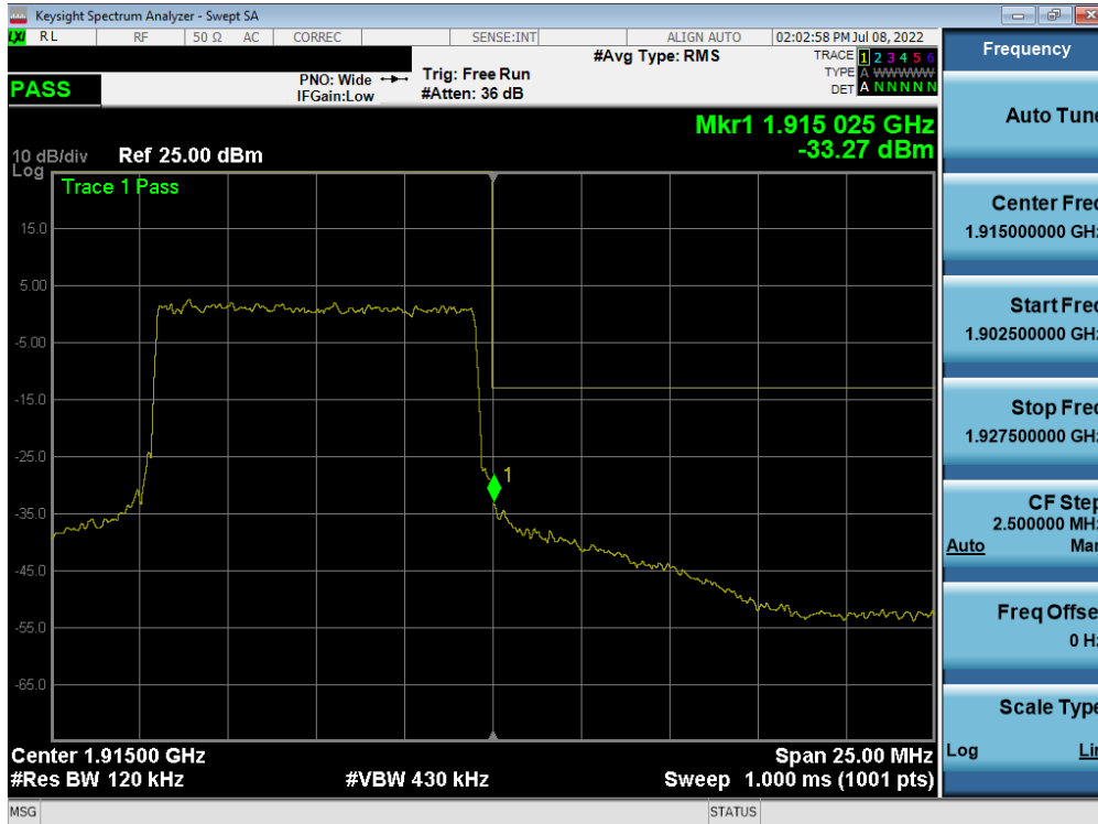
Plot 7-65. Upper Band Edge Plot (LTE Band 25 - 10MHz QPSK – Full RB)
