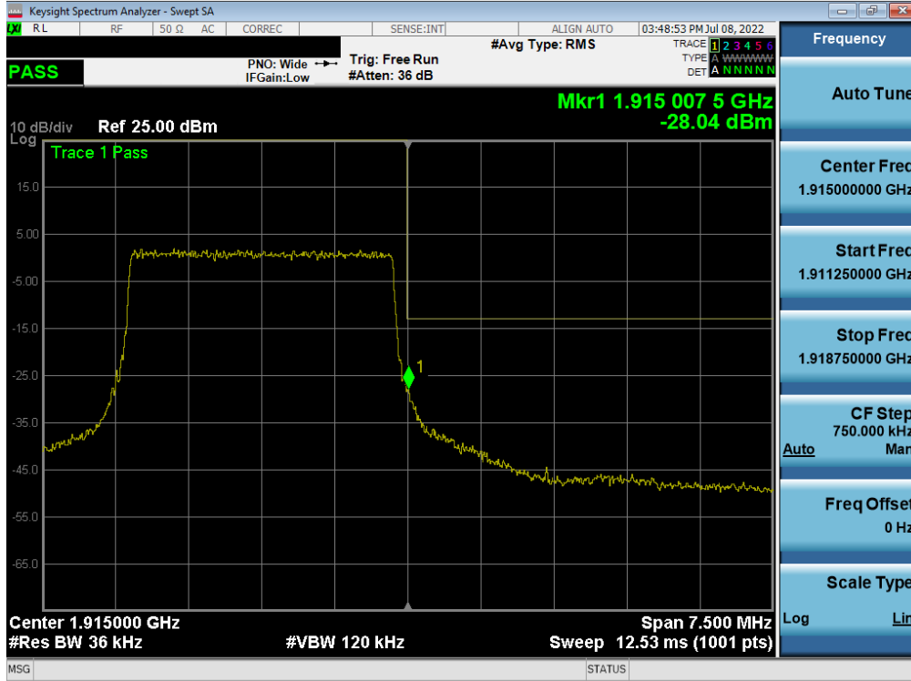
Plot 7-77. Upper Band Edge Plot (LTE Band 25 - 3MHz QPSK – Full RB)
