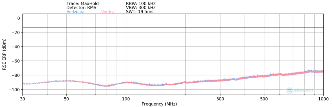
Plot 7-110. Radiated Spurious Plot Below 1GHz (WCDMA PCS)
