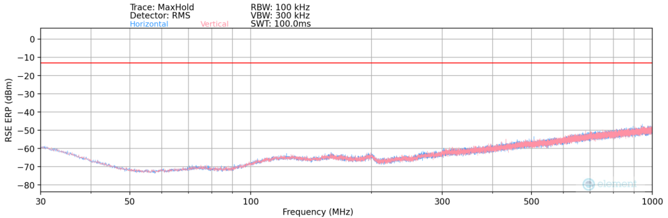
Plot 7-108. Radiated Spurious Plot Below 1GHz (GPRS PCS)
