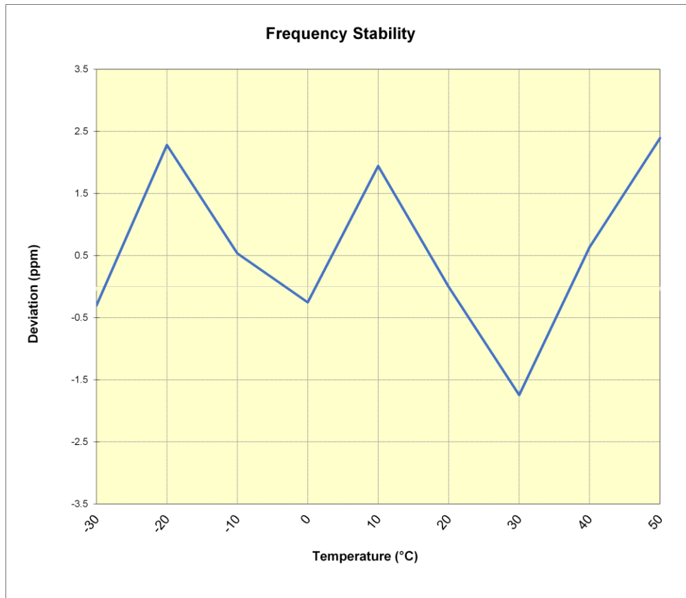
Plot 7-114. WCDMA PCS Frequency Stability Chart
