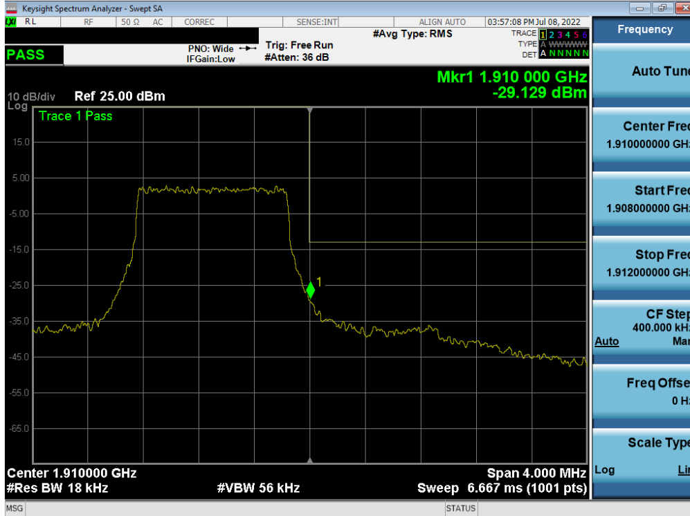
Plot 7-81. Upper Band Edge Plot (LTE Band 2 – 1.4MHz QPSK – Full RB)
