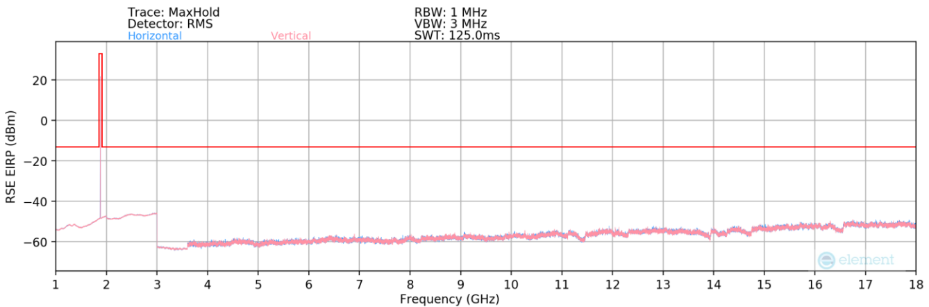
Plot 7-109. Radiated Spurious Plot (GPRS PCS)
