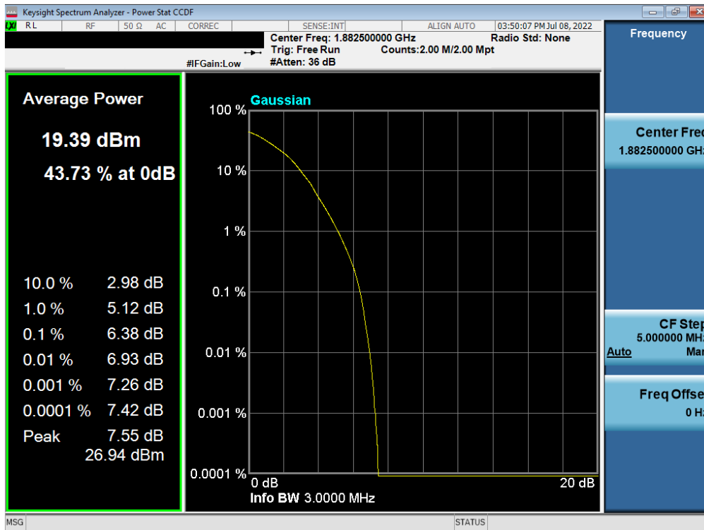
Plot 7-100. PAR Plot (LTE Band 25/2 - 3MHz 64-QAM - Full RB)
