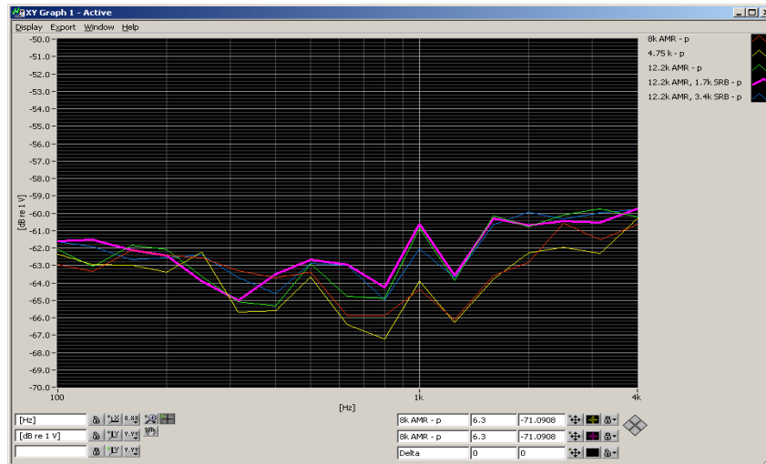
Figure 7-1 UMTS Audio Band Magnetic Noise
