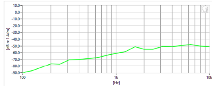
Frequency Response
