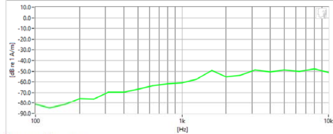
Frequency Response
