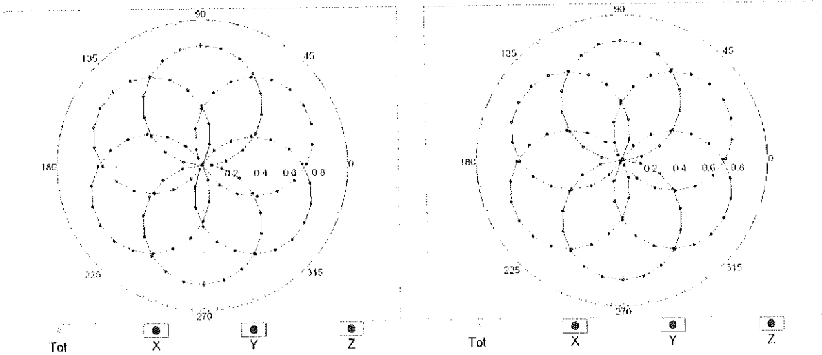
f=600 MHz,TEM
