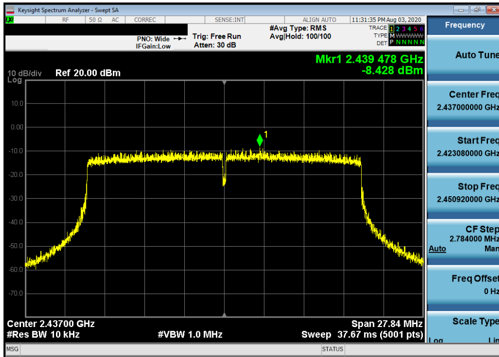
Plot 7-35. Power Spectral Density Plot SISO ANT1 (802.11ax (2.4GHz) – Ch. 6)
