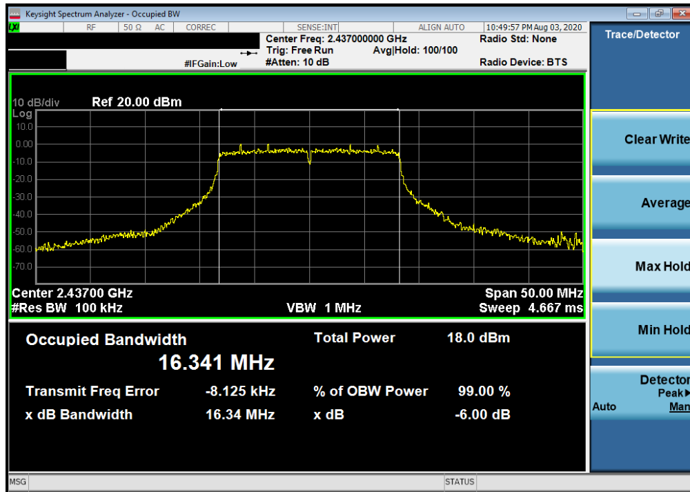
Plot 7-5. 6dB Bandwidth Plot SISO ANT1 (802.11g – Ch. 6)
