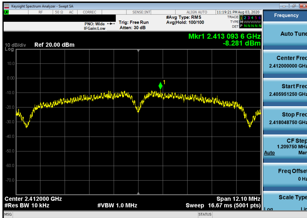
Plot 7-25. Power Spectral Density Plot SISO ANT1 (802.11b - Ch. 1)
