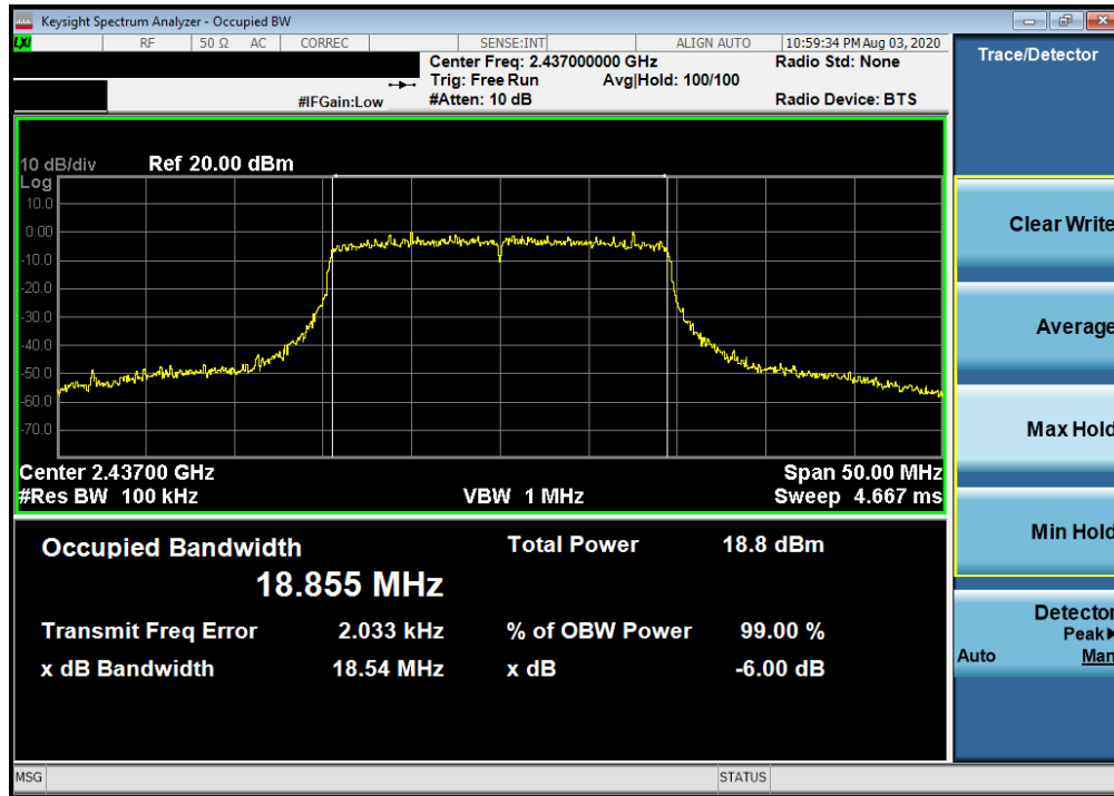
Plot 7-11. 6dB Bandwidth Plot SISO ANT1 (802.11ax (2.4GHz) – Ch. 6)
