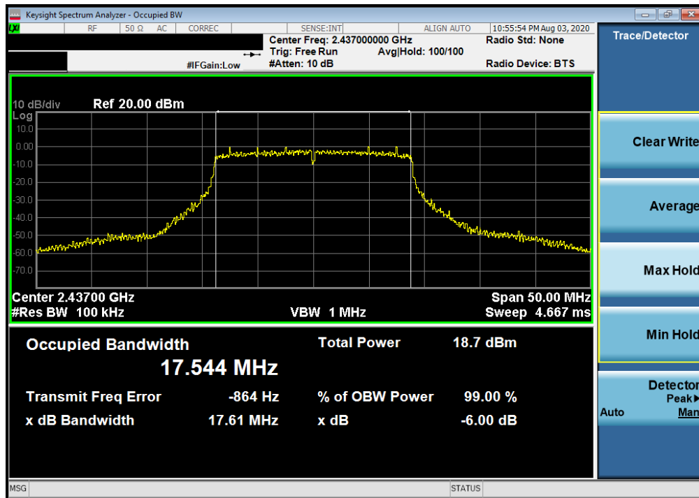
Plot 7-8. 6dB Bandwidth Plot SISO ANT1 (802.11n (2.4GHz) – Ch. 6)
