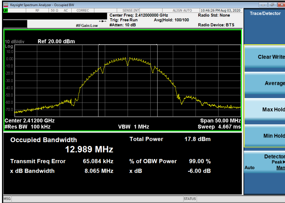
Plot 7-1. 6dB Bandwidth Plot SISO ANT1 (802.11b – Ch. 1)
