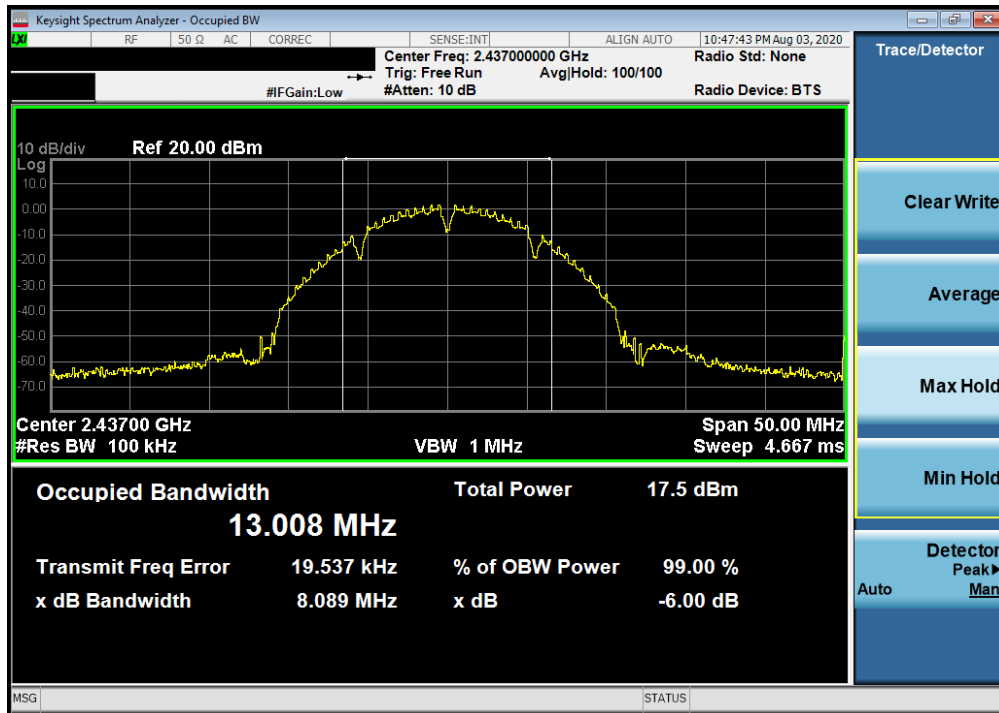
Plot 7-2. 6dB Bandwidth Plot SISO ANT1 (802.11b – Ch. 6)
