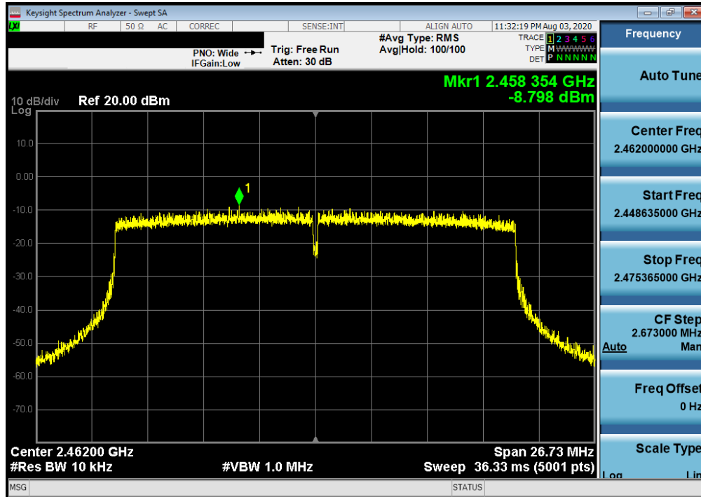
Plot 7-36. Power Spectral Density Plot SISO ANT1 (802.11ax (2.4GHz) – Ch. 11)
