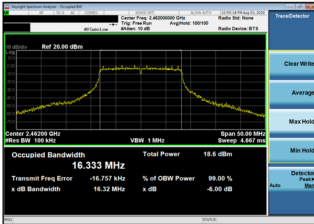
Plot 7-6. 6dB Bandwidth Plot SISO ANT1 (802.11g – Ch. 11)
