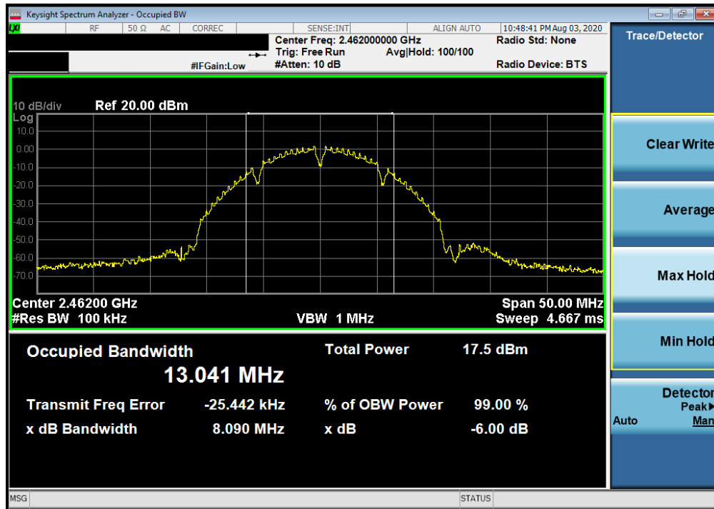
Plot 7-3. 6dB Bandwidth Plot SISO ANT1 (802.11b – Ch. 11)
