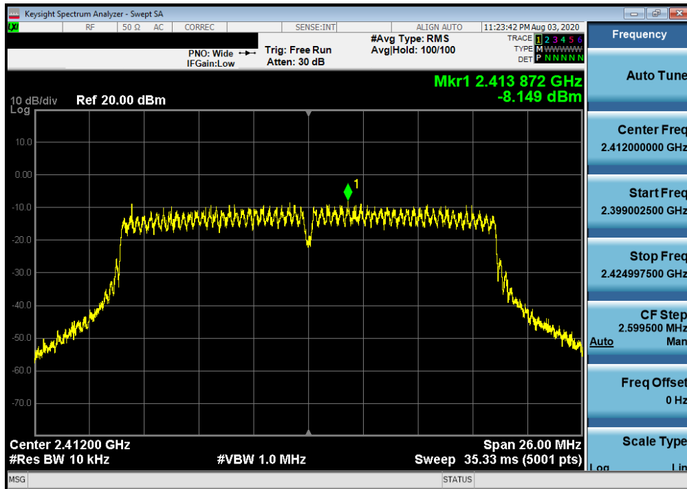
Plot 7-31. Power Spectral Density Plot SISO ANT1 (802.11n (2.4GHz) – Ch. 1)
