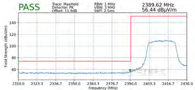
Plot 7-98. Radiated Restricted Lower Band Edge Measurement MIMO (Peak)
