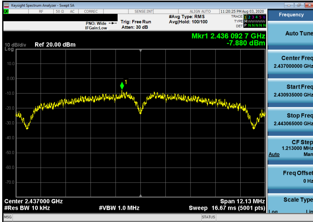
Plot 7-26. Power Spectral Density Plot SISO ANT1 (802.11b – Ch. 6)
