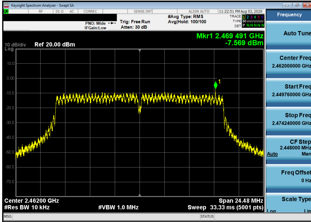
Plot 7-30. Power Spectral Density Plot SISO ANT1 (802.11g – Ch. 11)
