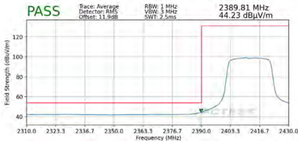
Plot 7-97. Radiated Restricted Lower Band Edge Measurement MIMO (Average)
