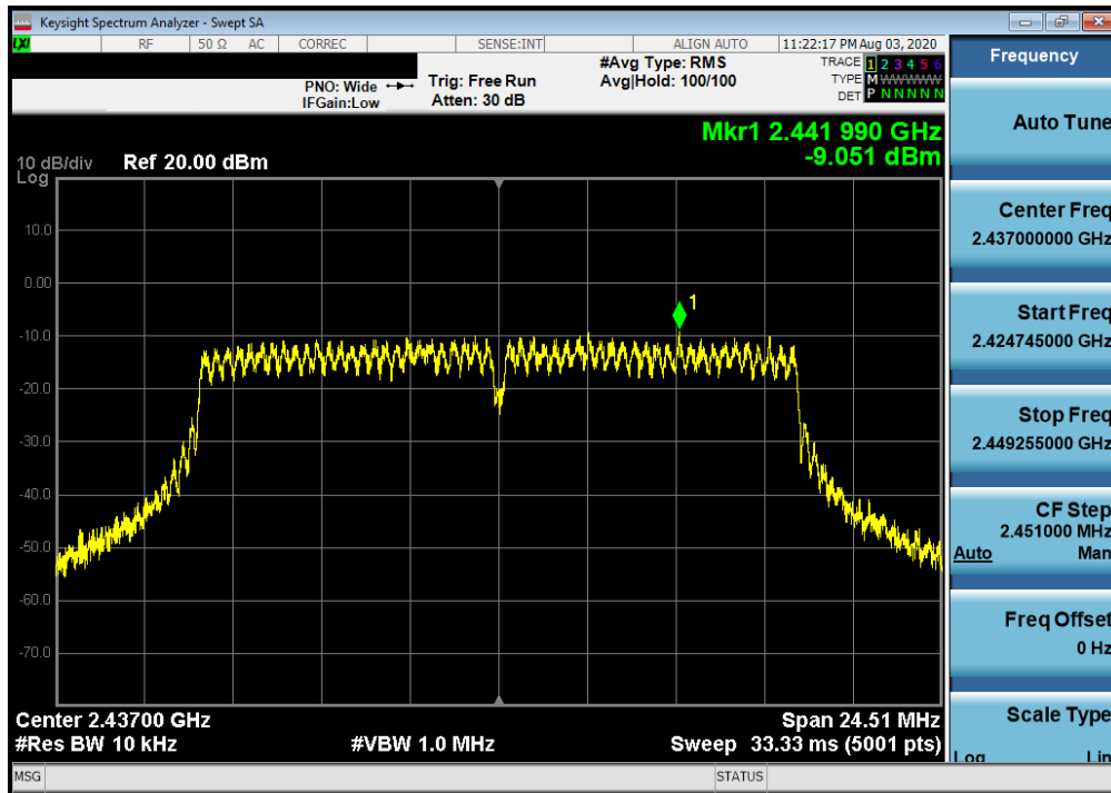
Plot 7-29. Power Spectral Density Plot SISO ANT1 (802.11g – Ch. 6)
