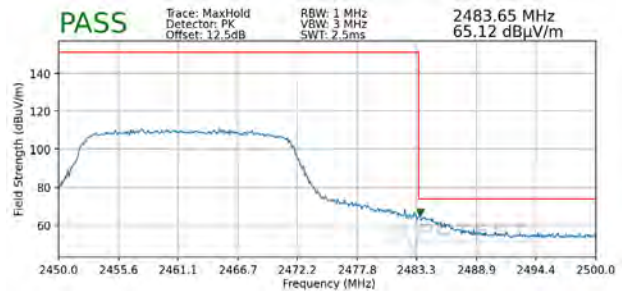
Plot 7-100. Radiated Restricted Upper Band Edge Measurement MIMO (Peak)
