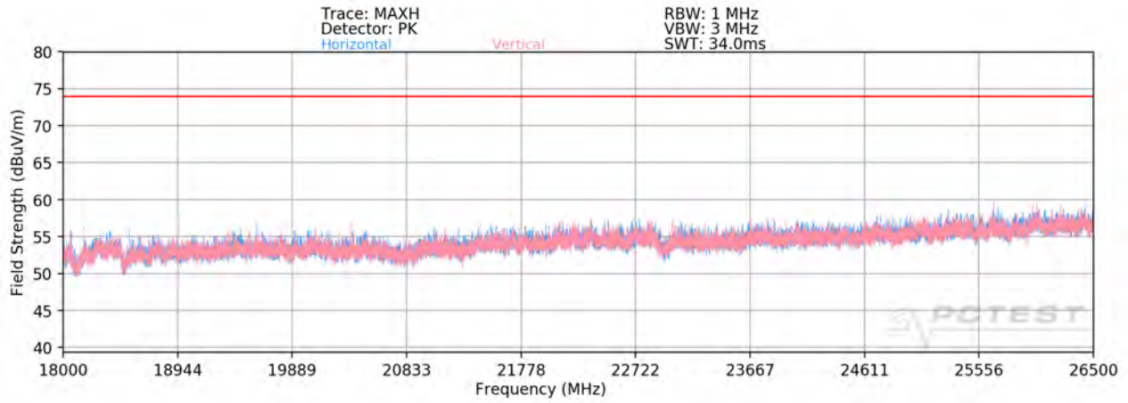
Plot 7-88. Radiated Spurious Plot above 18GHz MIMO/CDD
