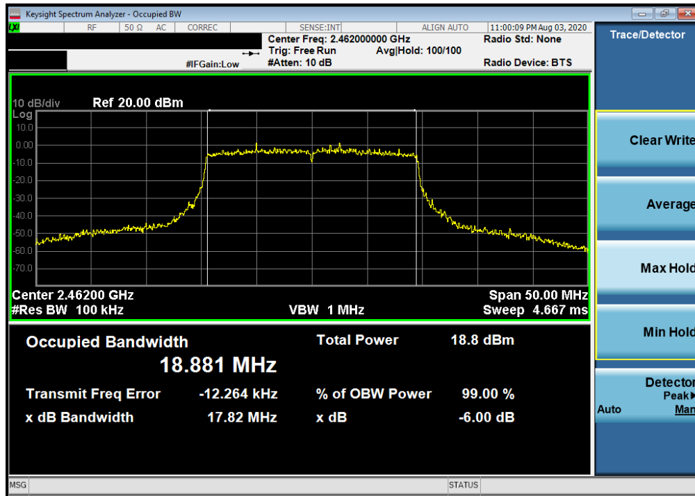
Plot 7-12. 6dB Bandwidth Plot SISO ANT1 (802.11ax (2.4GHz) – Ch. 11)
