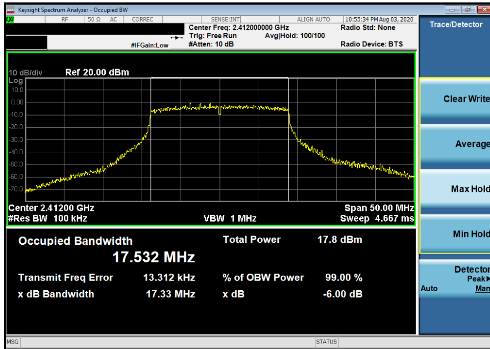
Plot 7-7. 6dB Bandwidth Plot SISO ANT1 (802.11n (2.4GHz) – Ch. 1)
