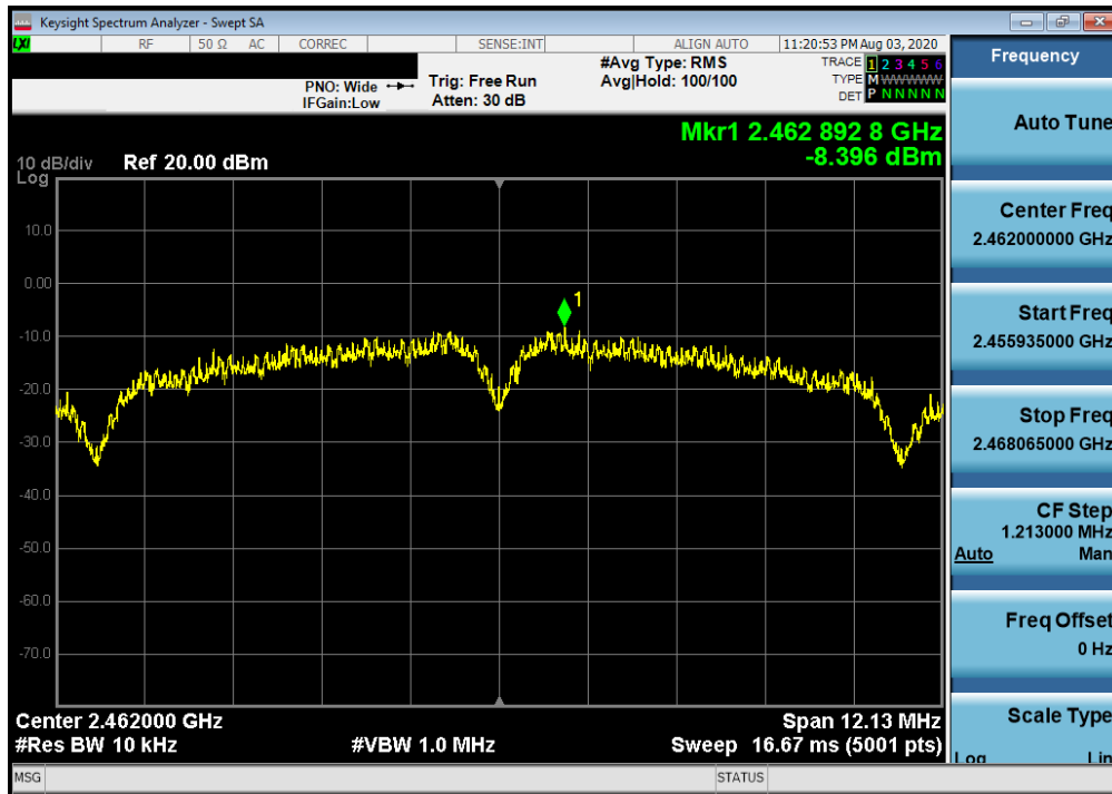
Plot 7-27. Power Spectral Density Plot SISO ANT1 (802.11b – Ch. 11)
