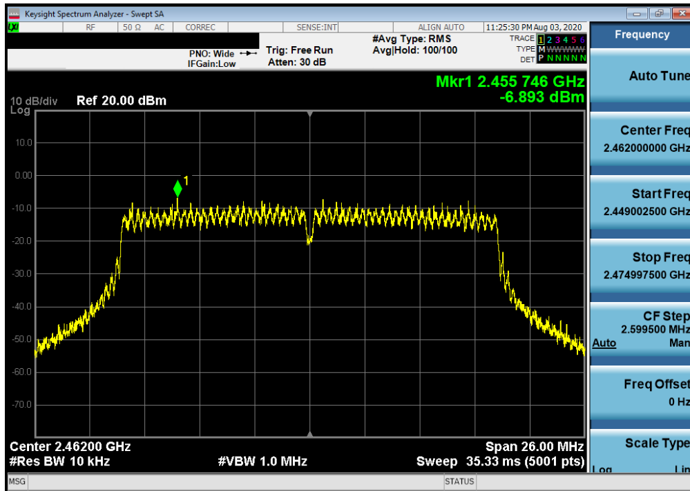
Plot 7-33. Power Spectral Density Plot SISO ANT1 (802.11n (2.4GHz) – Ch. 11)
