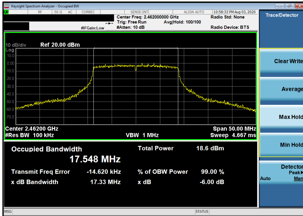
Plot 7-9. 6dB Bandwidth Plot SISO ANT1 (802.11n (2.4GHz) – Ch. 11)
