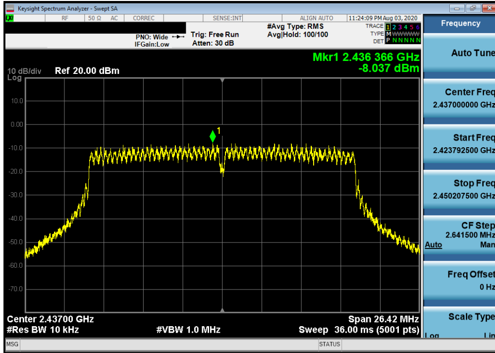
Plot 7-32. Power Spectral Density Plot SISO ANT1 (802.11n (2.4GHz) – Ch. 6)
