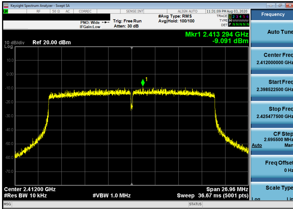
Plot 7-34. Power Spectral Density Plot SISO ANT1 (802.11ax (2.4GHz) – Ch. 1)
