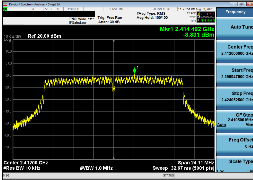
Plot 7-28. Power Spectral Density Plot SISO ANT1 (802.11g – Ch. 1)
