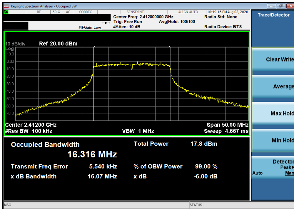
Plot 7-4. 6dB Bandwidth Plot SISO ANT1 (802.11g – Ch. 1)
