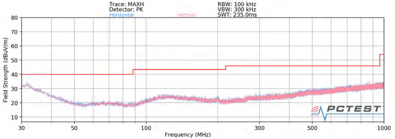
Plot 7-101. Radiated Spurious Plot below 1GHz
