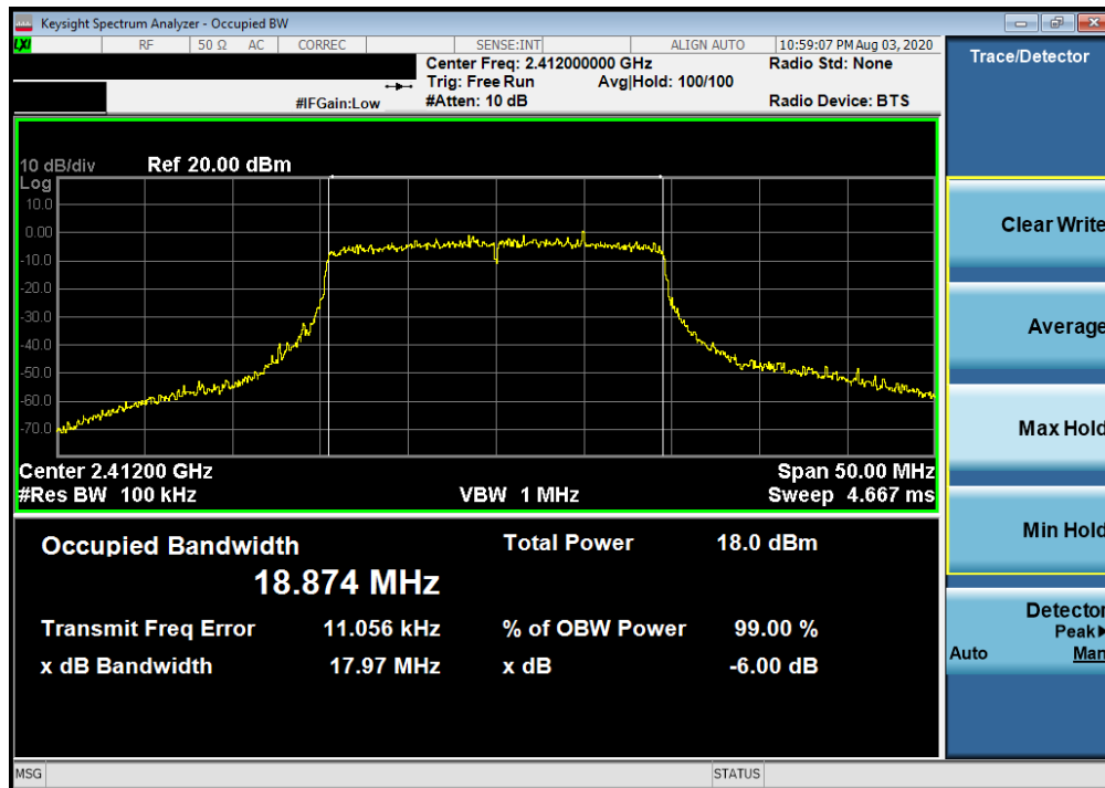
Plot 7-10. 6dB Bandwidth Plot SISO ANT1 (802.11ax (2.4GHz) – Ch. 1)
