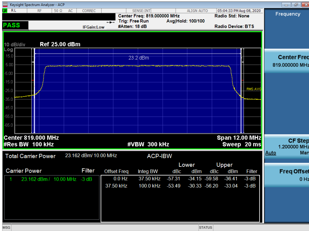
Plot 7-23. Channel Edge Plot (LTE Band 26 - 10MHz QPSK)
