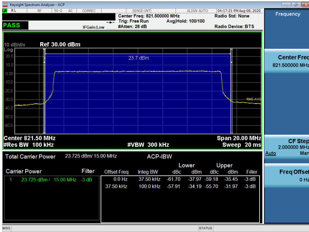
Plot 7-22. Channel Edge Plot (LTE Band 26 - 15MHz QPSK)
