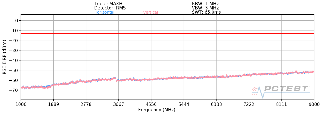
Plot 7-31. Radiated Spurious Plot (Band 26)
