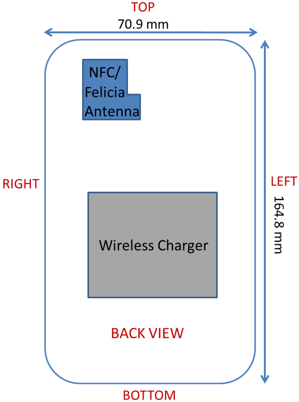
Figure G-2 NFC Antenna Locations
