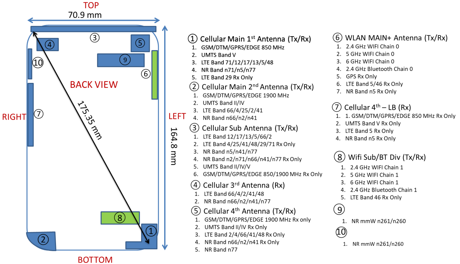
Figure G-1 DUT Antenna Locations
