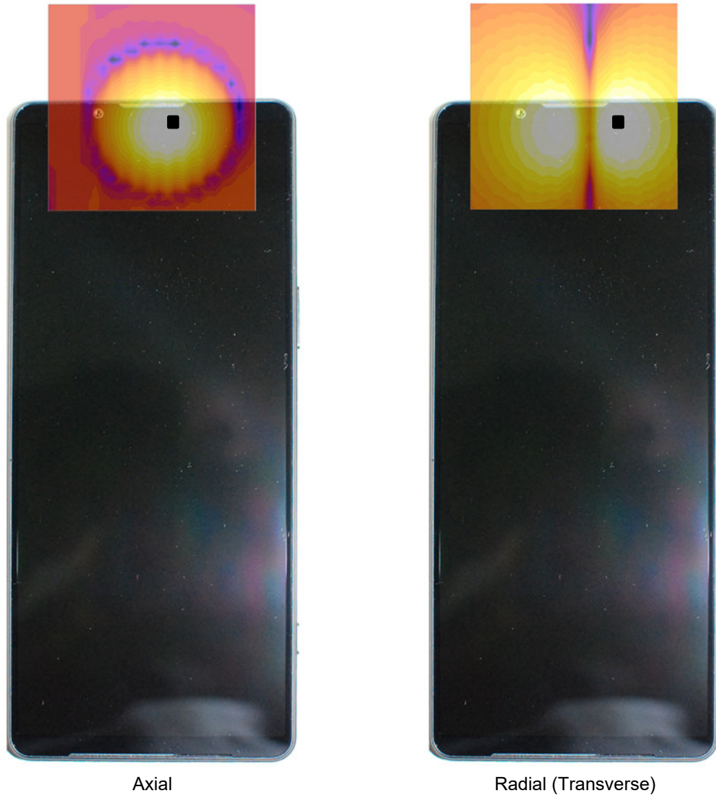
Figure 15-3 T-Coil Scan Overlay Magnetic Field Distributions
