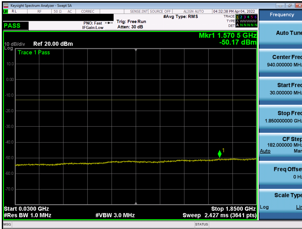
Plot 7-43. Conducted Spurious Plot (NR Band n2 - 20.0MHz - 1RB - High Channel)
