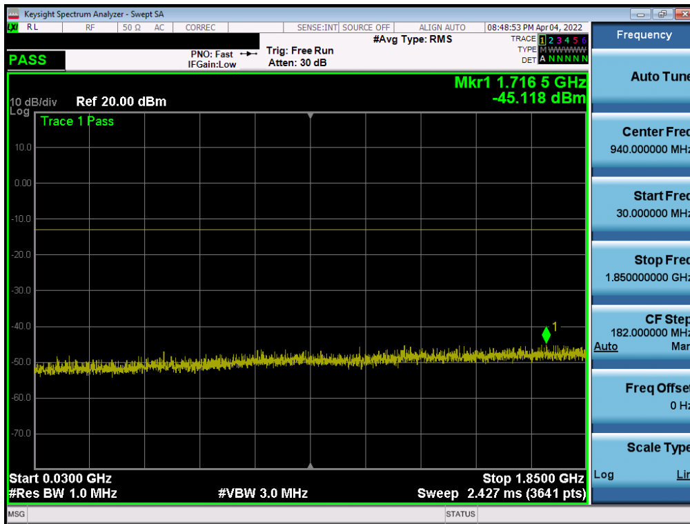
Plot 7-49. Conducted Spurious Plot (GPRS Ch. 661)
