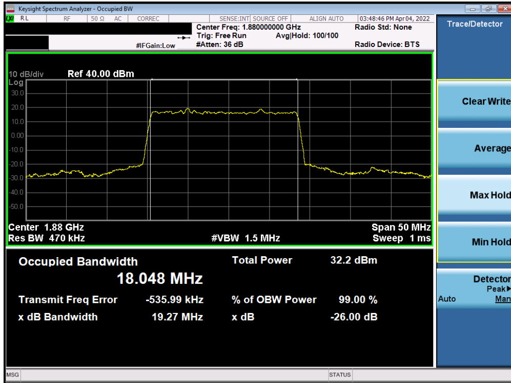
Plot 7-13. Occupied Bandwidth Plot (NR Band n2 - 20.0MHz DFT-S-OFDM BPSK - Full RB)
