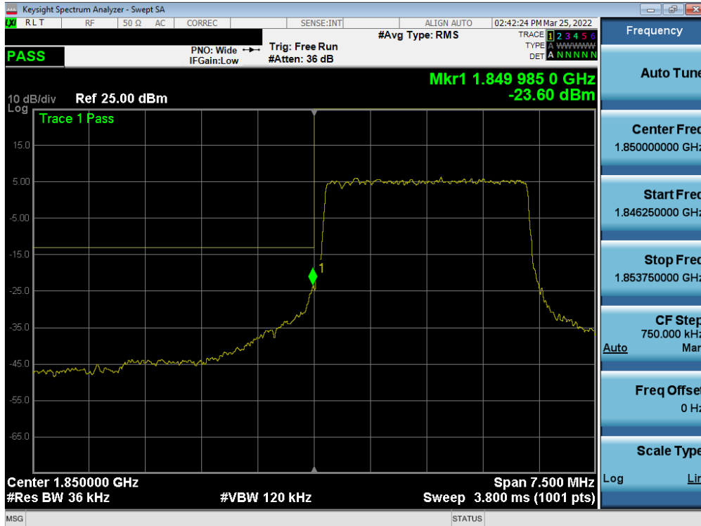
Plot 7-88. Lower Band Edge Plot (LTE Band 25/2 - 3MHz QPSK – Full RB)
