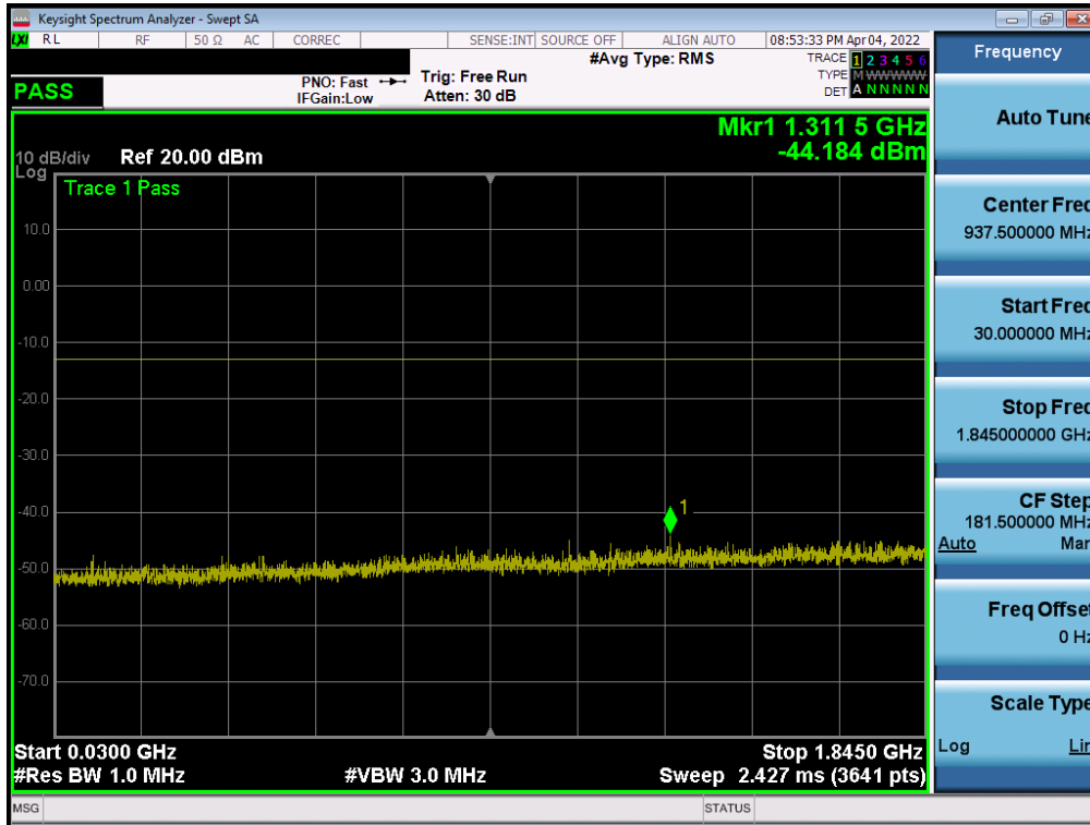
Plot 7-46. Conducted Spurious Plot (GPRS Ch. 512)
