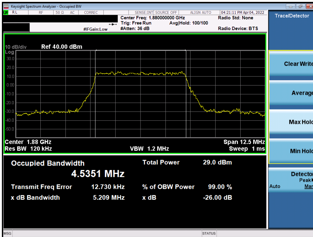
Plot 7-24. Occupied Bandwidth Plot (NR Band n2 - 5.0MHz CP-OFDM 16QAM - Full RB)
