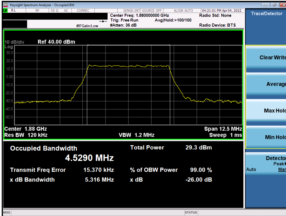
Plot 7-23. Occupied Bandwidth Plot (NR Band n2 - 5.0MHz CP-OFDM QPSK - Full RB)
