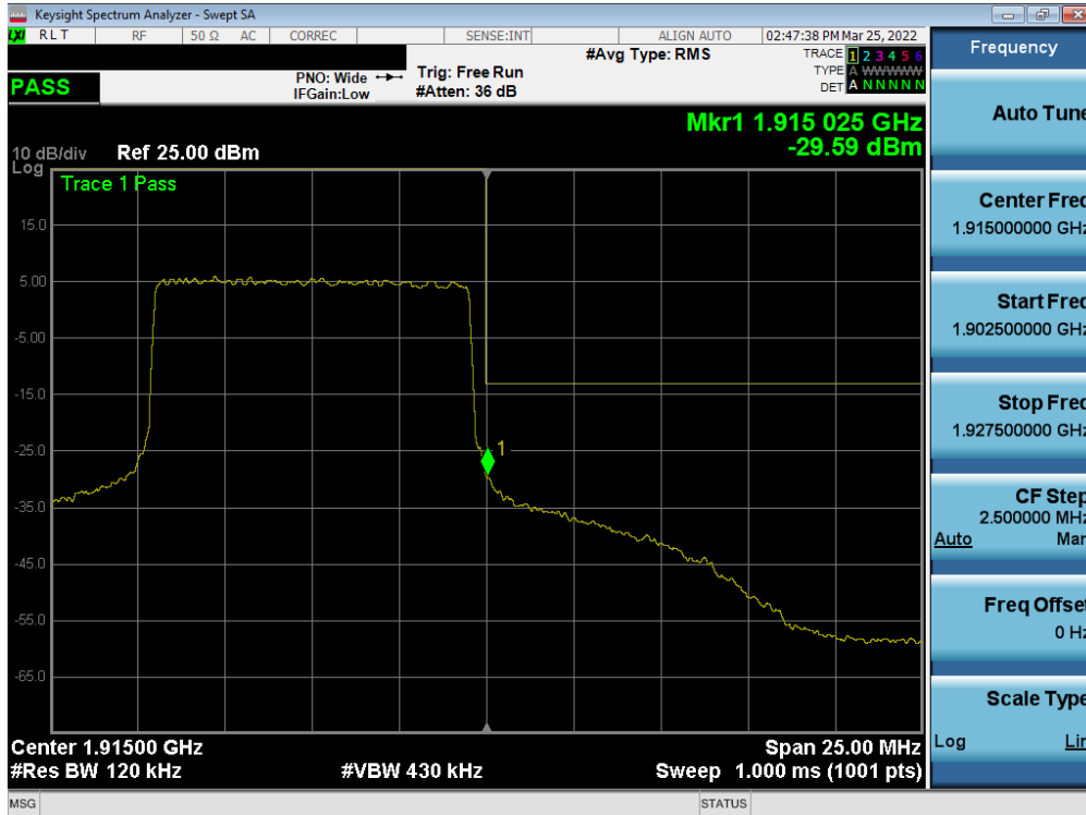
Plot 7-80. Upper Band Edge Plot (LTE Band 25 - 10MHz QPSK – Full RB)
