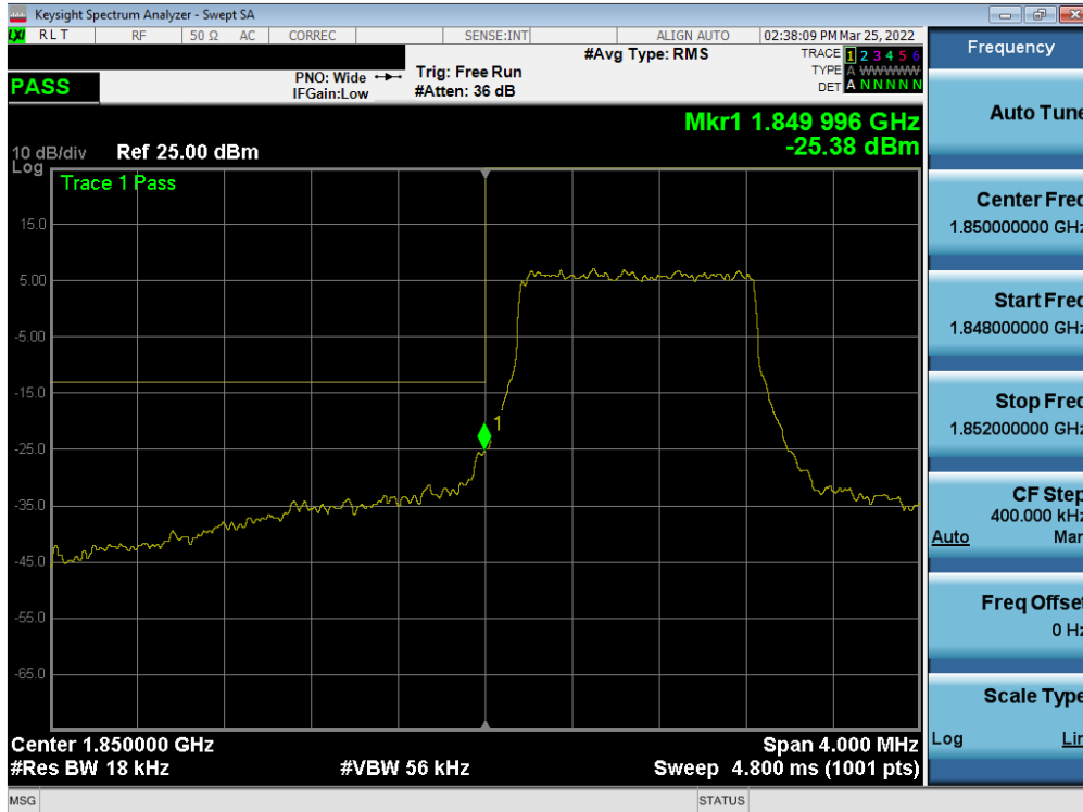
Plot 7-94. Lower Band Edge Plot (LTE Band 25/2 – 1.4MHz QPSK – Full RB)
