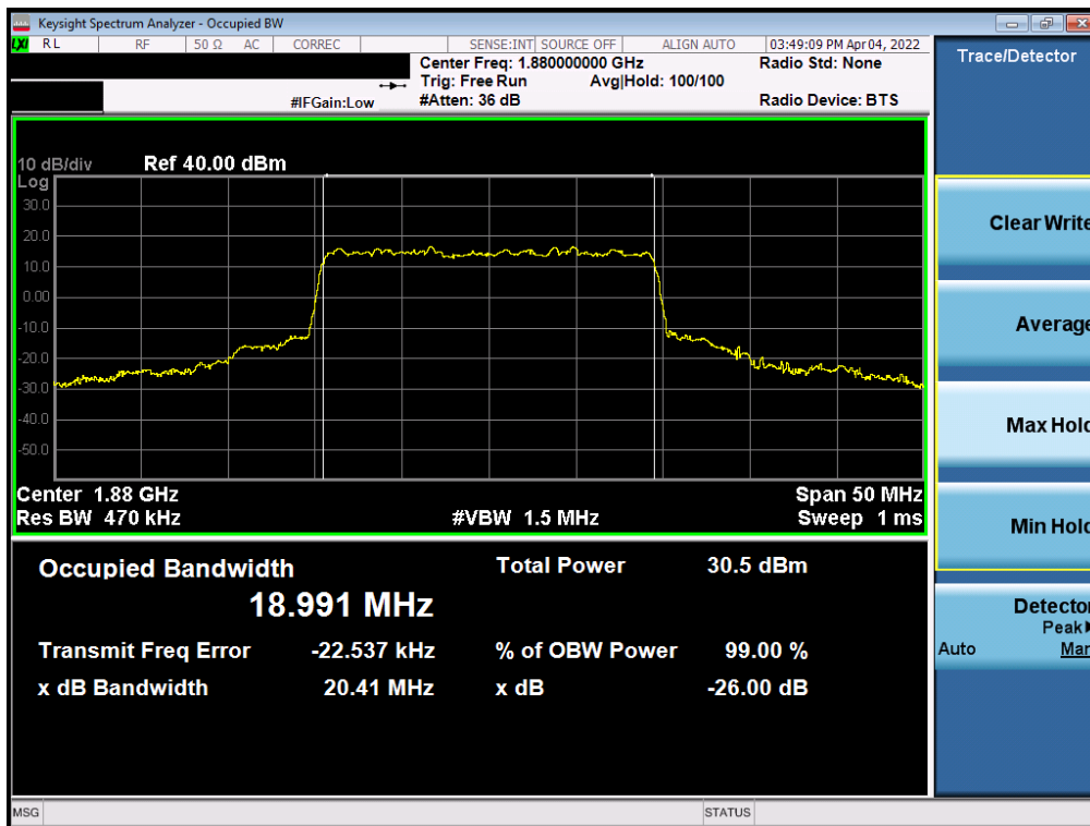
Plot 7-14. Occupied Bandwidth Plot (NR Band n2 - 20.0MHz CP-OFDM QPSK - Full RB)
