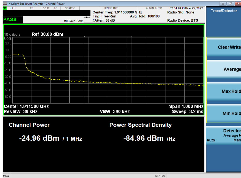
Plot 7-85. Extended Upper Band Edge Plot (LTE Band 2 - 5MHz QPSK – Full RB)
