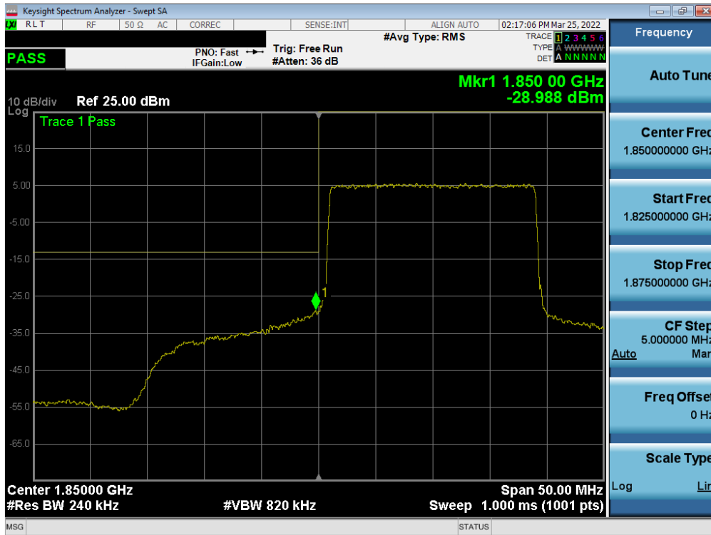
Plot 7-64. Lower Band Edge Plot (LTE Band 25/2 - 20MHz QPSK – Full RB)
