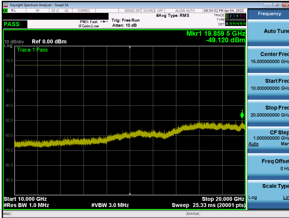
Plot 7-54. Conducted Spurious Plot (GPRS Ch. 810)
