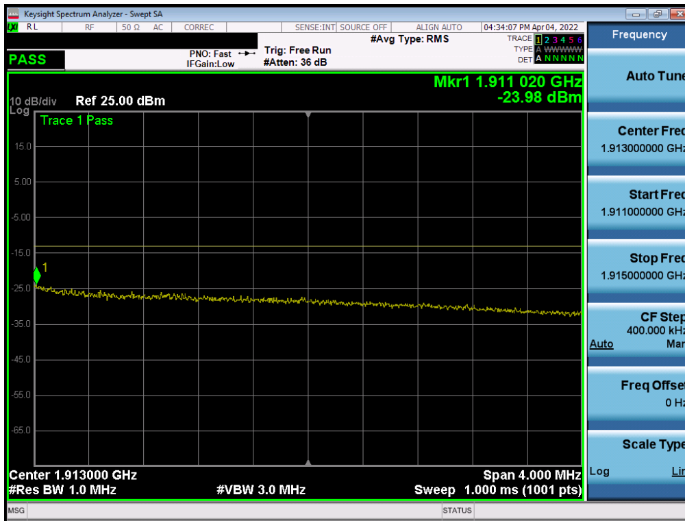
Plot 7-103. Upper Extended Band Edge Plot (NR Band n2 – 20.0MHz - Full RB)
