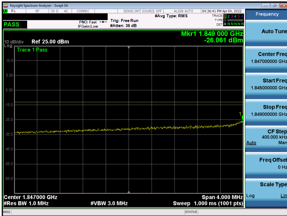
Plot 7-101. Lower Extended Band Edge Plot (NR Band n2 – 20.0MHz - Full RB)
