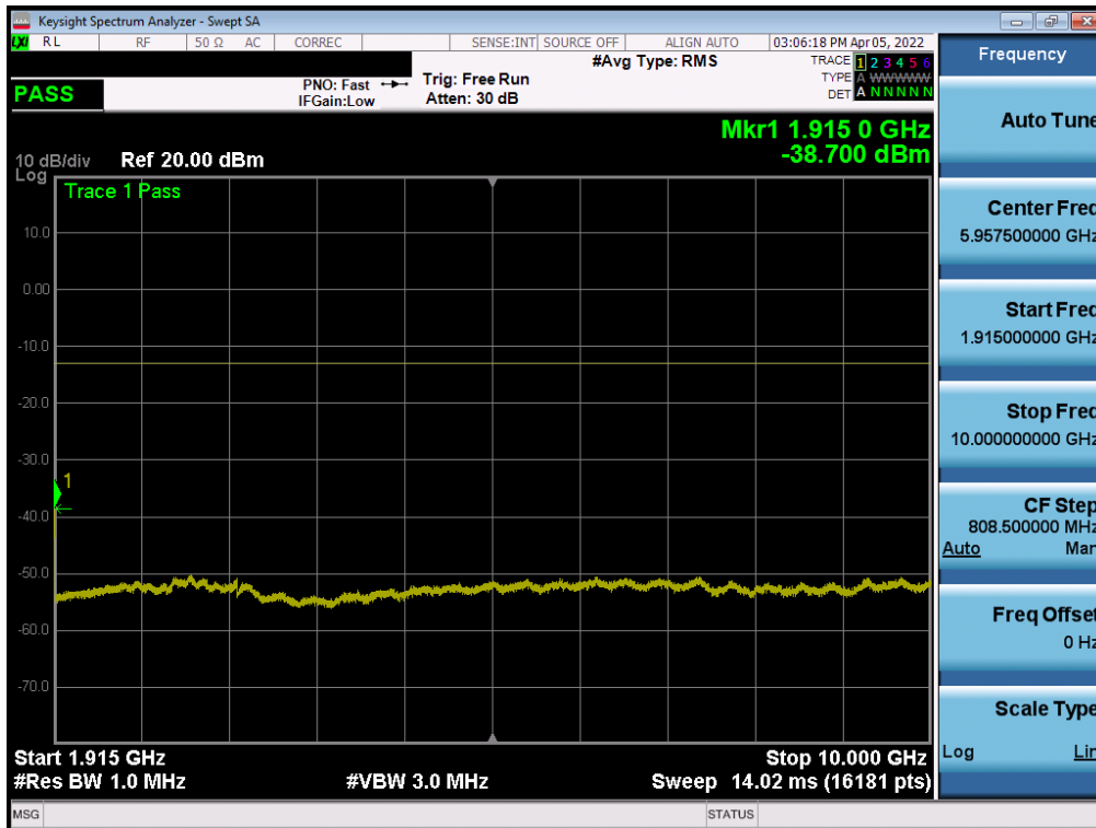
Plot 7-62. Conducted Spurious Plot (WCDMA Ch. 9538)
