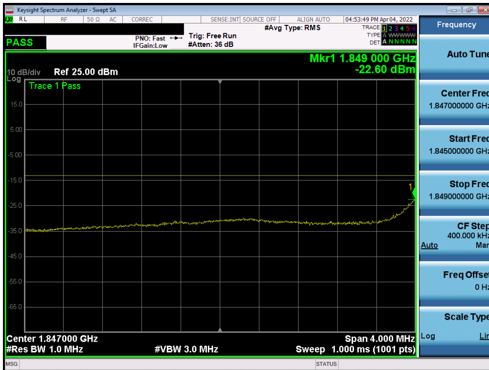
Plot 7-105. Lower Extended Band Edge Plot (NR Band n2 – 15.0MHz - Full RB)
