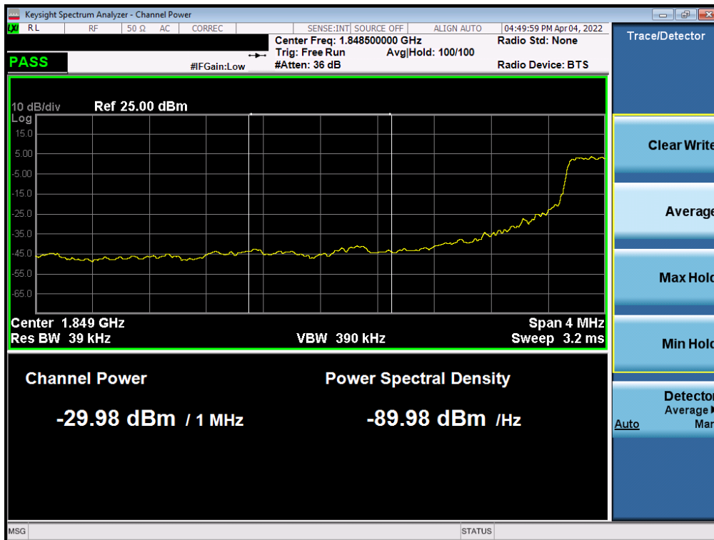
Plot 7-113. Lower Extended Band Edge Plot (NR Band n2 – 5.0MHz - Full RB)
