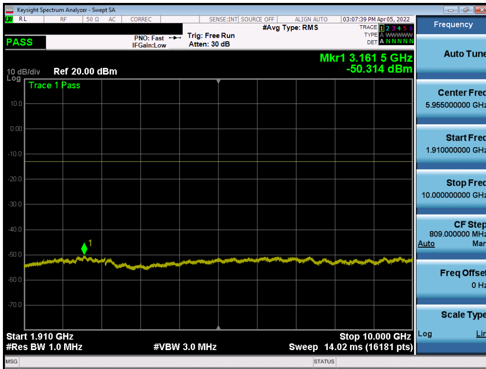
Plot 7-56. Conducted Spurious Plot (WCDMA Ch. 9262)
