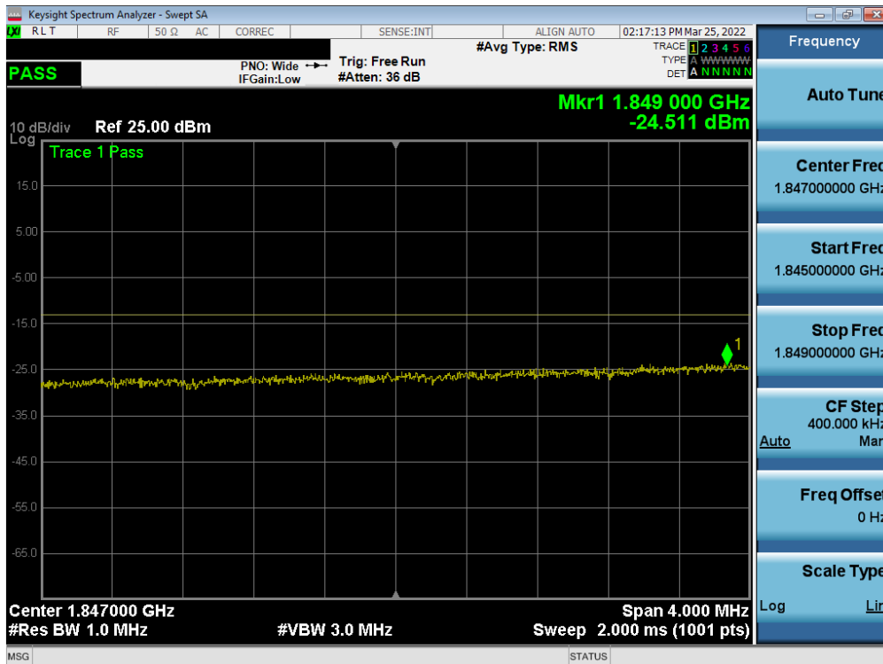
Plot 7-65. Extended Lower Band Edge Plot (LTE Band 25/2 - 20MHz QPSK – Full RB)
