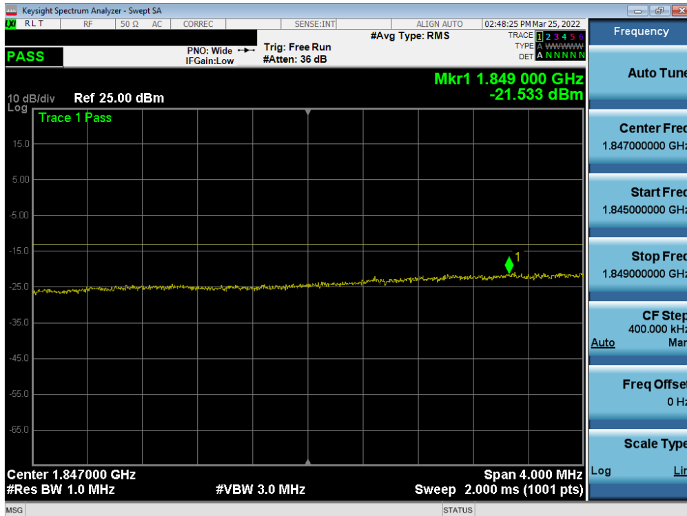
Plot 7-71. Extended Lower Band Edge Plot (LTE Band 25/2 - 15MHz QPSK – Full RB)
