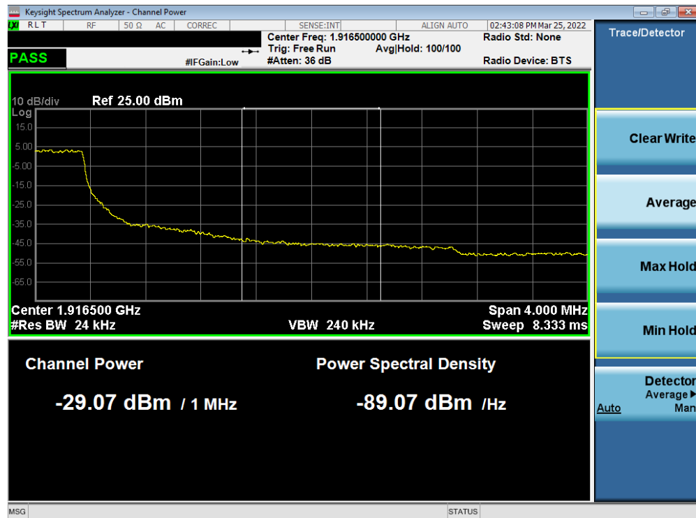
Plot 7-93. Extended Upper Band Edge Plot (LTE Band 25 - 3MHz QPSK – Full RB)
