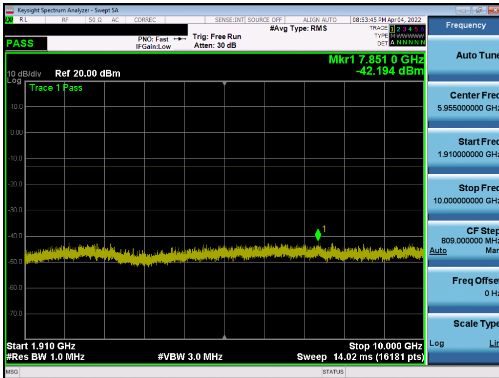
Plot 7-47. Conducted Spurious Plot (GPRS Ch. 512)
