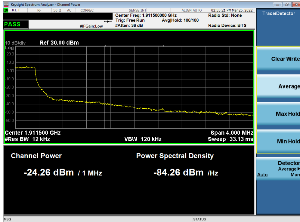
Plot 7-97. Extended Upper Band Edge Plot (LTE Band 2 – 1.4MHz QPSK – Full RB)
