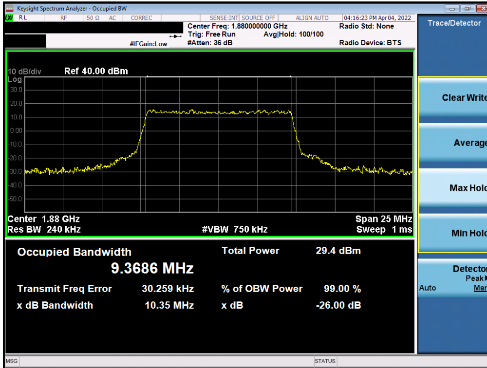
Plot 7-21. Occupied Bandwidth Plot (NR Band n2 - 10.0MHz CP-OFDM 16QAM - Full RB)
