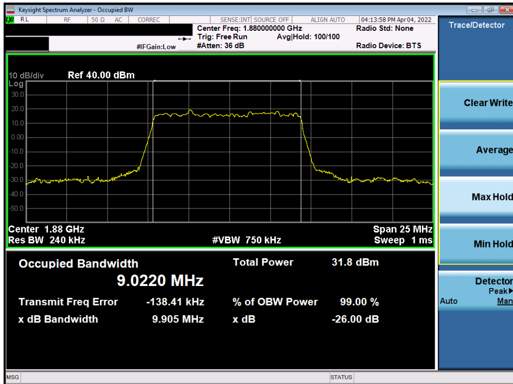
Plot 7-19. Occupied Bandwidth Plot (NR Band n2 - 10.0MHz DFT-S-OFDM BPSK - Full RB)
