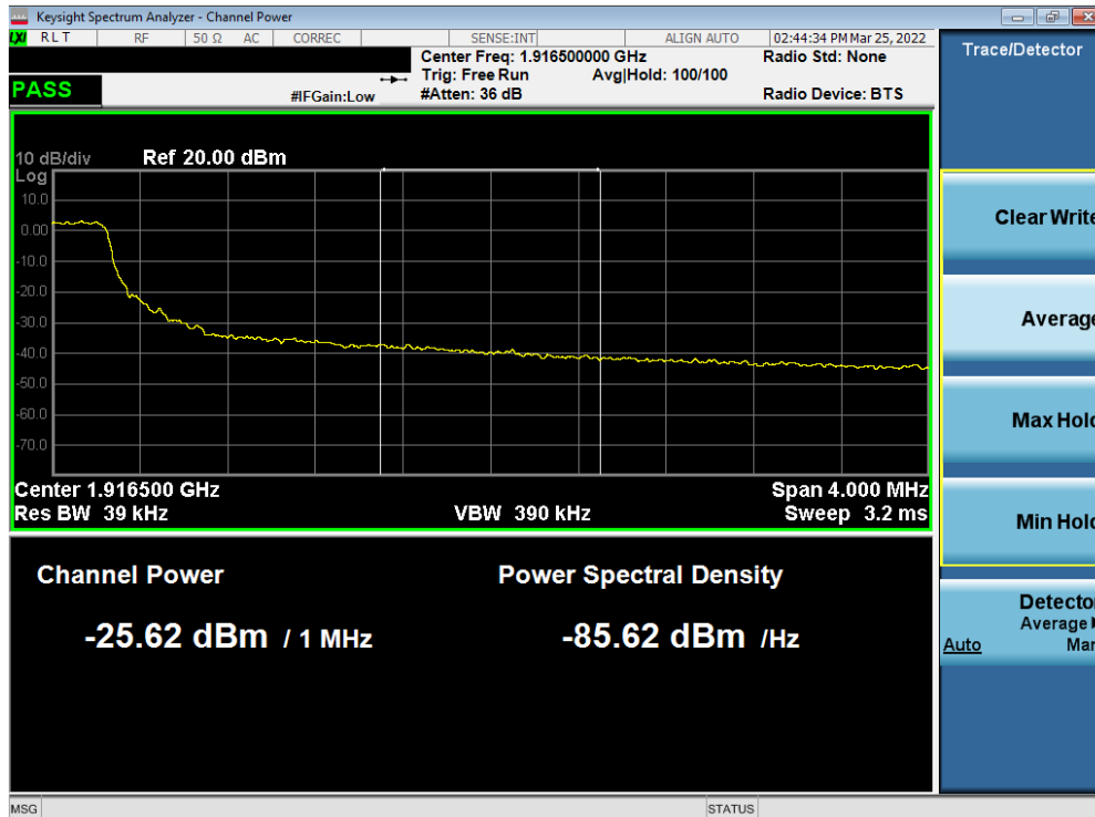
Plot 7-87. Extended Upper Band Edge Plot (LTE Band 25 - 5MHz QPSK – Full RB)
