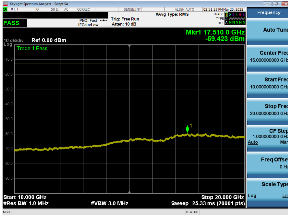
Plot 7-36. Conducted Spurious Plot (LTE Band 25/2 - 20MHz QPSK - 1RB - High Channel)
