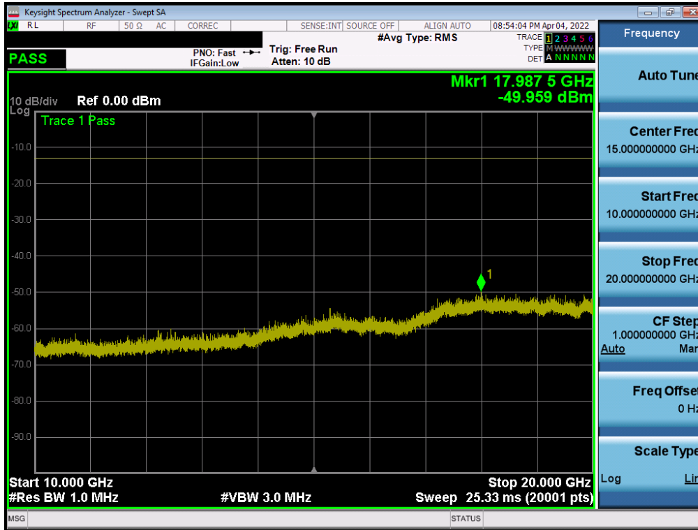
Plot 7-48. Conducted Spurious Plot (GPRS Ch. 512)
