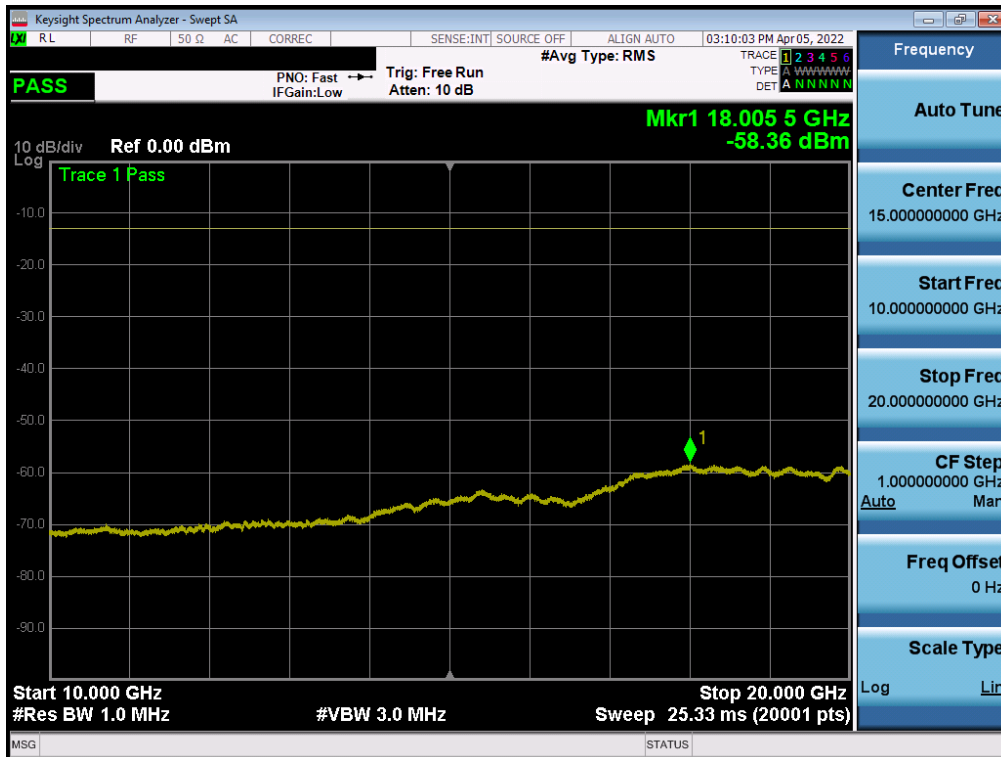
Plot 7-60. Conducted Spurious Plot (WCDMA Ch. 9400)
