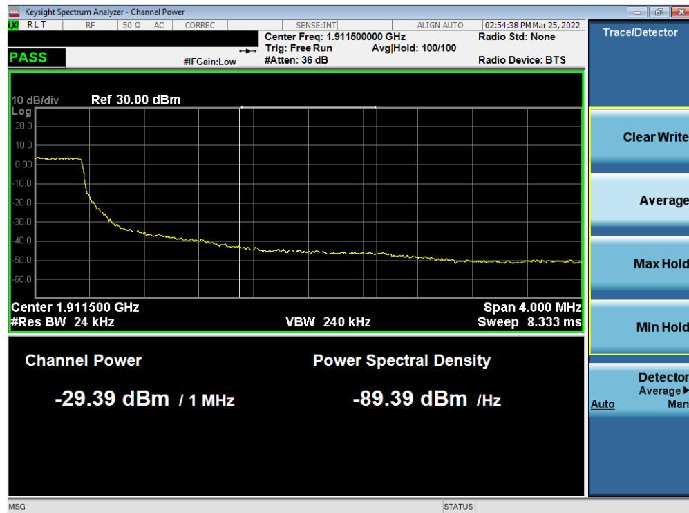
Plot 7-91. Extended Upper Band Edge Plot (LTE Band 2 - 3MHz QPSK – Full RB)
