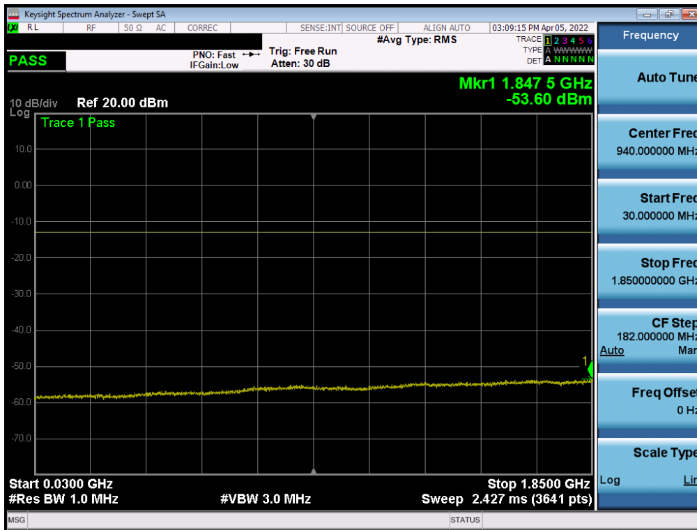
Plot 7-58. Conducted Spurious Plot (WCDMA Ch. 9400)
