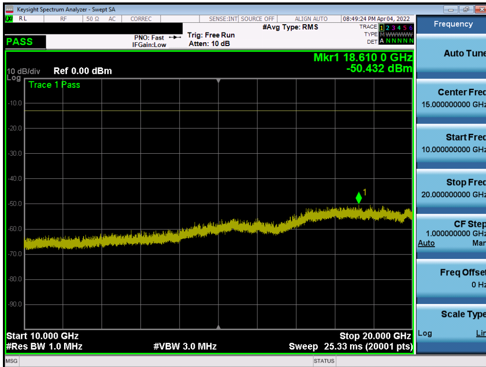
Plot 7-51. Conducted Spurious Plot (GPRS Ch. 661)
