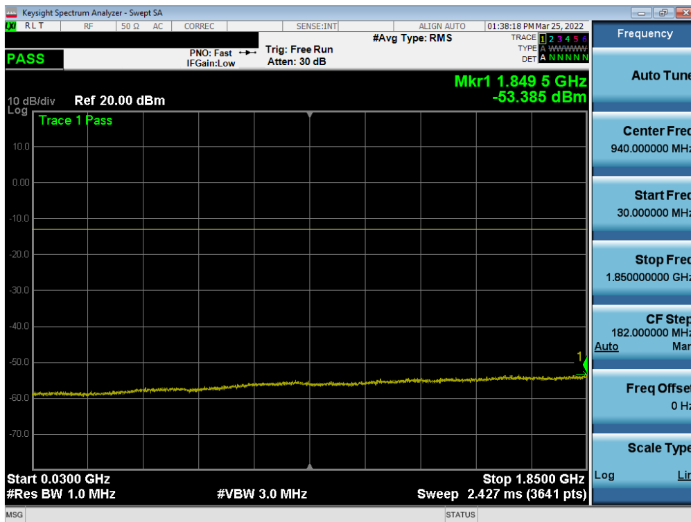
Plot 7-31. Conducted Spurious Plot (LTE Band 25/2 - 20MHz QPSK - 1RB - Mid Channel)
