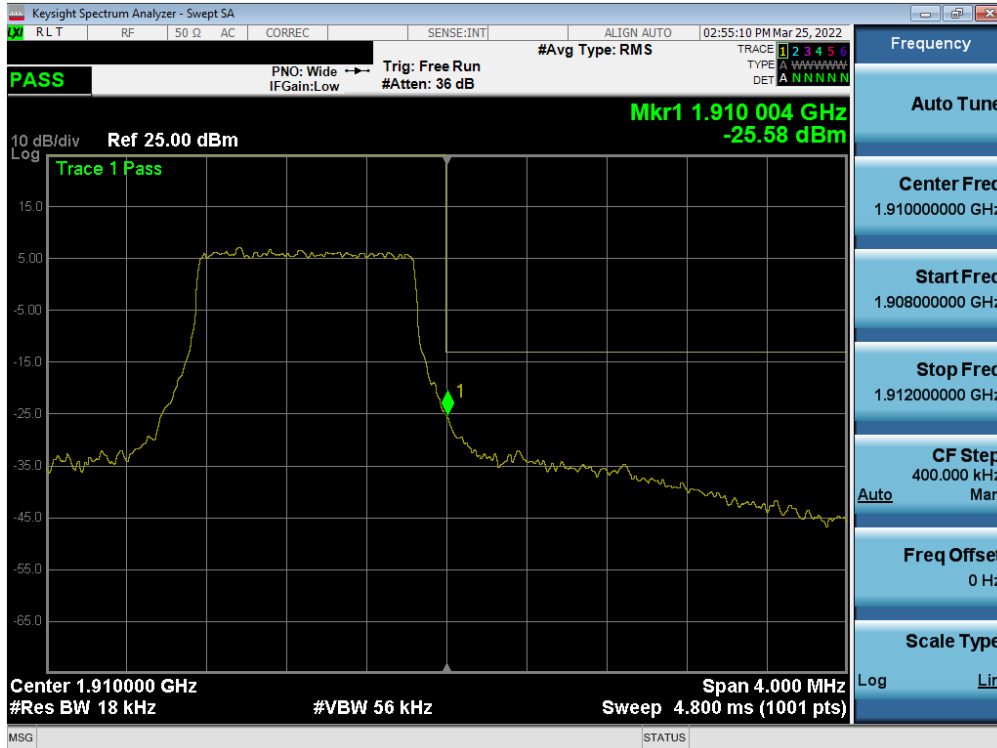
Plot 7-96. Upper Band Edge Plot (LTE Band 2 – 1.4MHz QPSK – Full RB)
