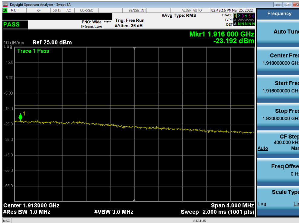
Plot 7-75. Extended Upper Band Edge Plot (LTE Band 25 - 15MHz QPSK – Full RB)
