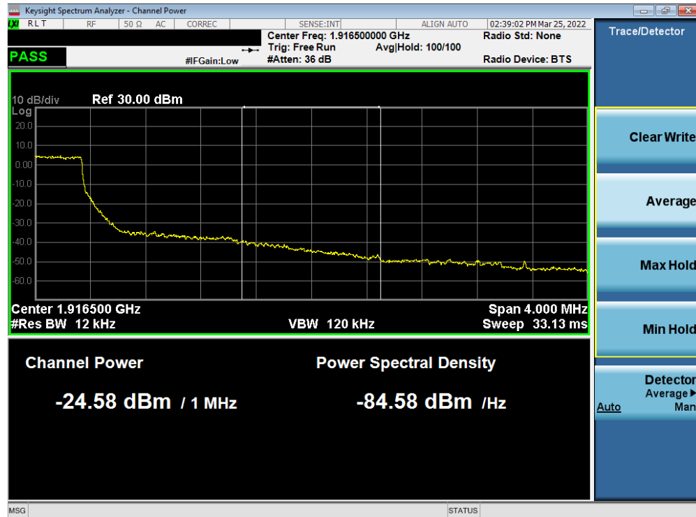
Plot 7-99. Extended Upper Band Edge Plot (LTE Band 25 – 1.4MHz QPSK – Full RB)
