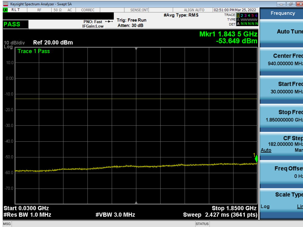
Plot 7-34. Conducted Spurious Plot (LTE Band 25/2 - 20MHz QPSK - 1RB - High Channel)
