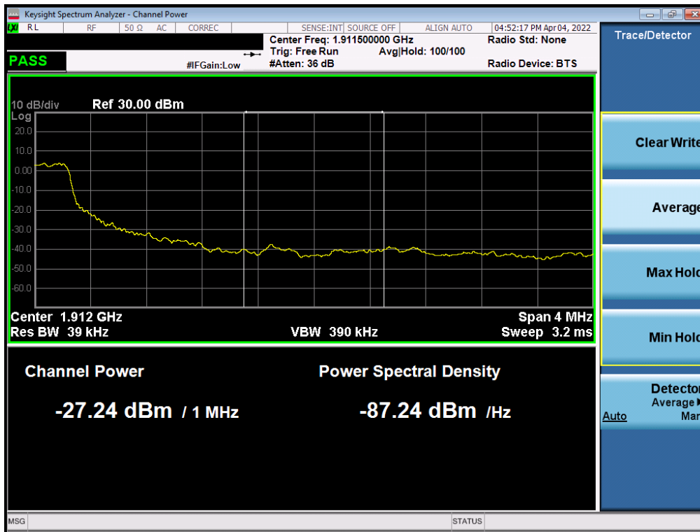
Plot 7-115. Upper Extended Band Edge Plot (NR Band n2 – 5.0MHz - Full RB)
