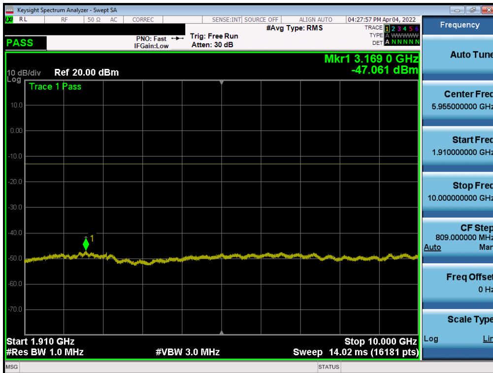
Plot 7-38. Conducted Spurious Plot (NR Band n2 - 20.0MHz - 1RB - Low Channel)
