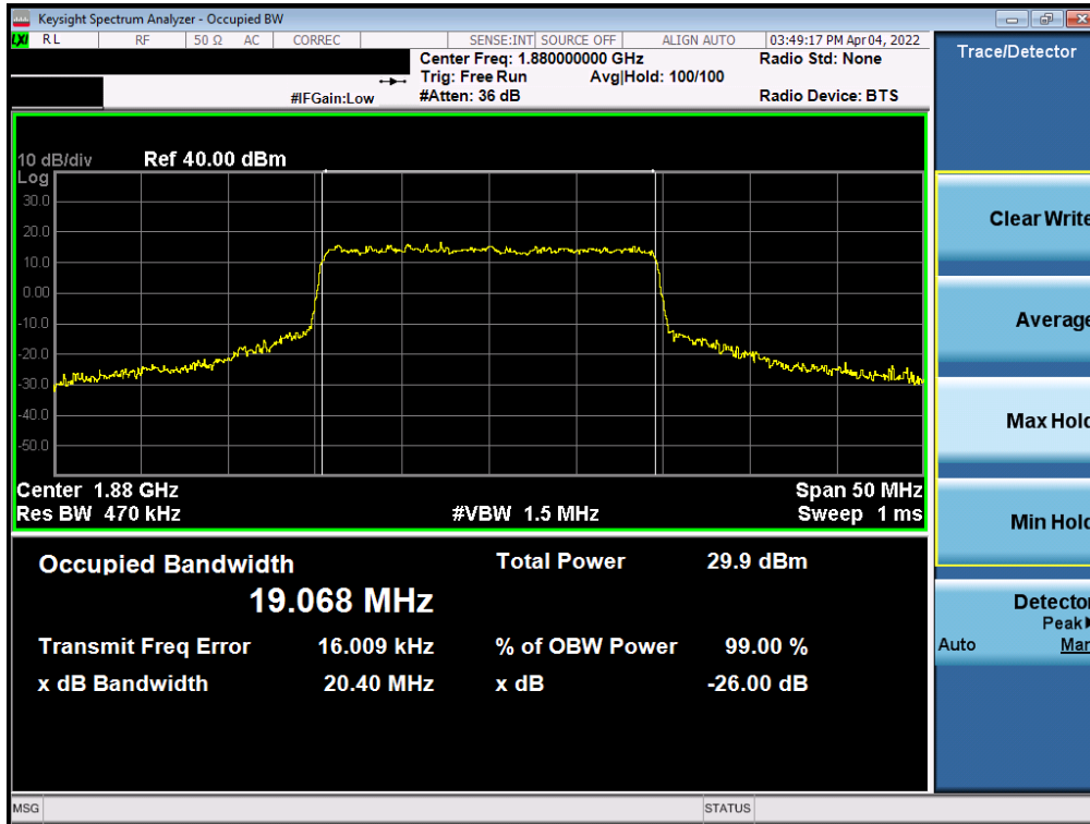
Plot 7-15. Occupied Bandwidth Plot (NR Band n2 - 20.0MHz CP-OFDM 16QAM - Full RB)
