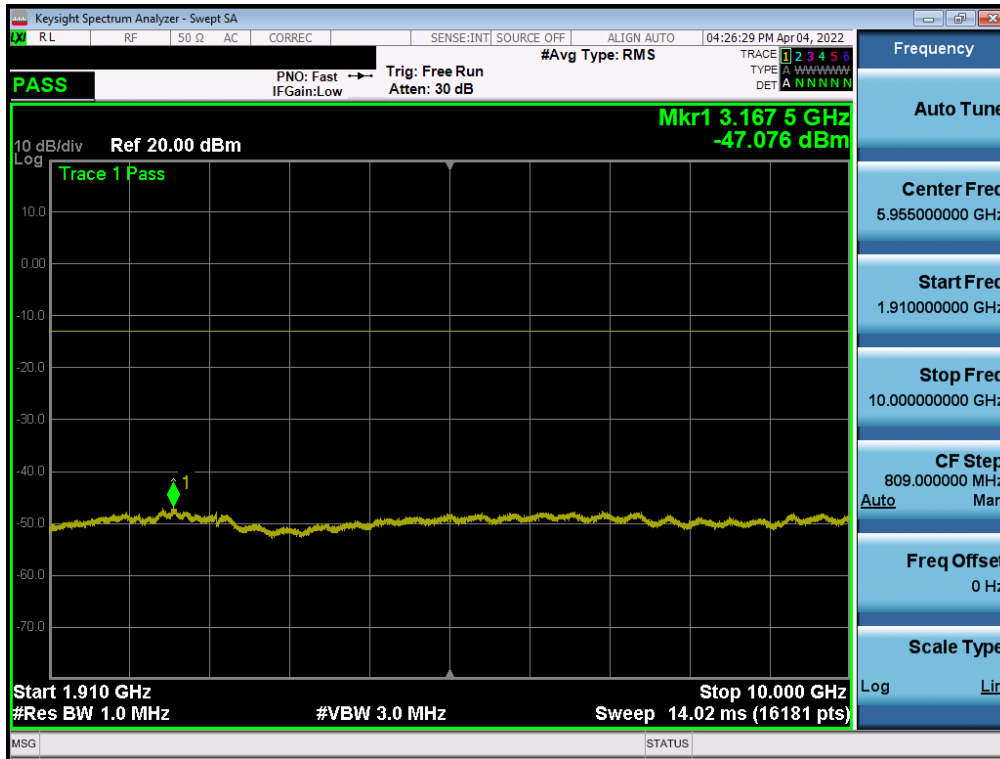
Plot 7-41. Conducted Spurious Plot (NR Band n2 - 20.0MHz - 1RB - Mid Channel)
