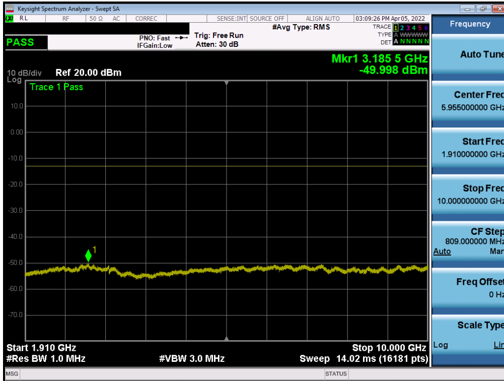
Plot 7-59. Conducted Spurious Plot (WCDMA Ch. 9400)
