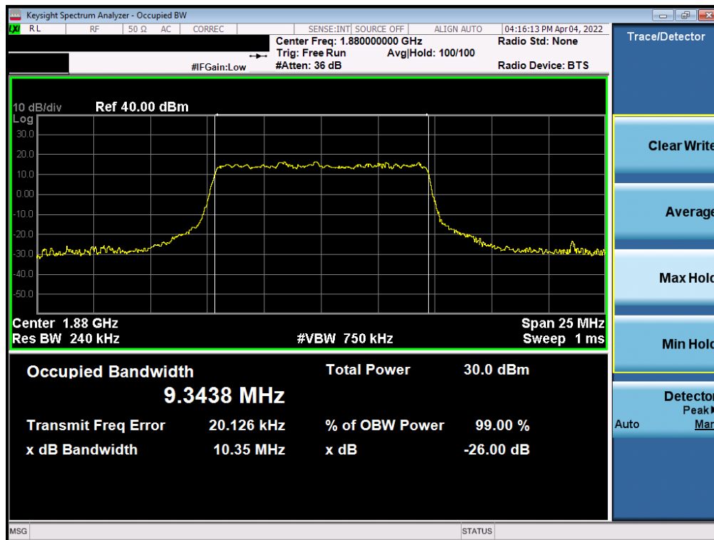
Plot 7-20. Occupied Bandwidth Plot (NR Band n2 - 10.0MHz CP-OFDM QPSK - Full RB)
