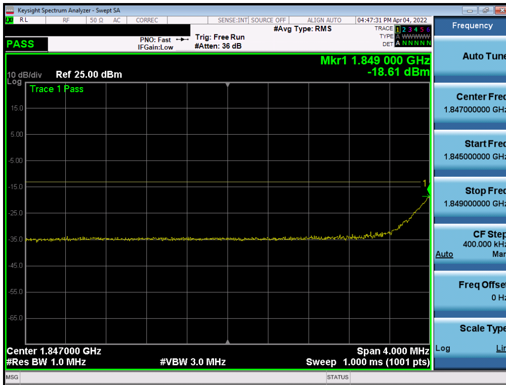
Plot 7-109. Lower Extended Band Edge Plot (NR Band n2 – 10.0MHz - Full RB)
