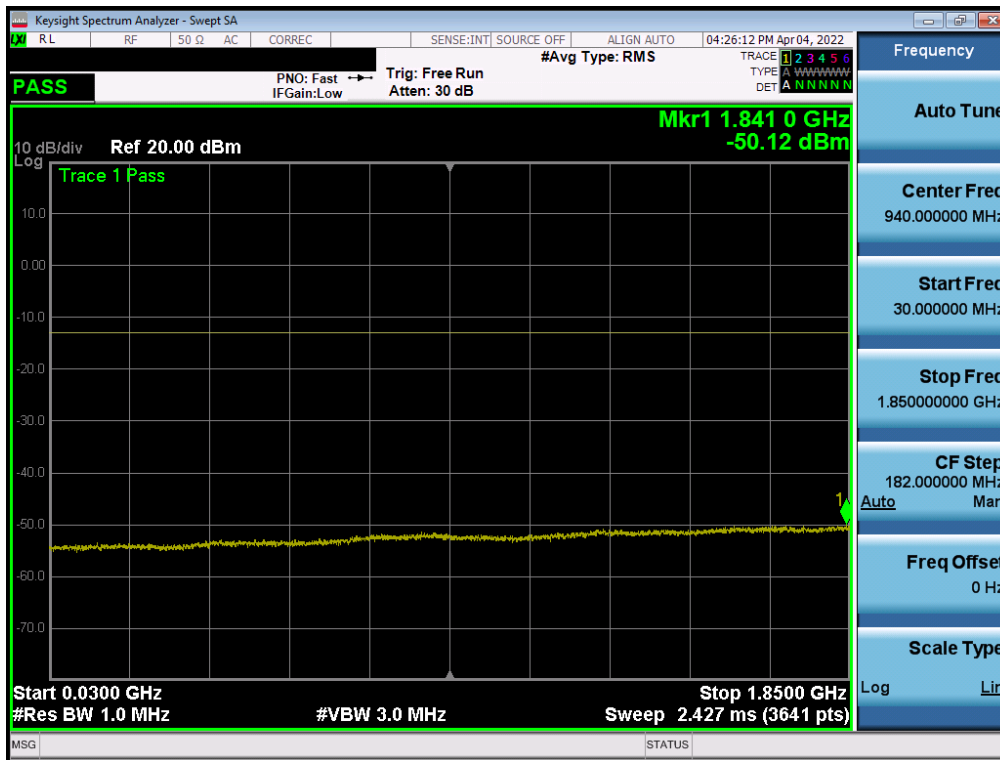
Plot 7-40. Conducted Spurious Plot (NR Band n2 - 20.0MHz - 1RB - Mid Channel)
