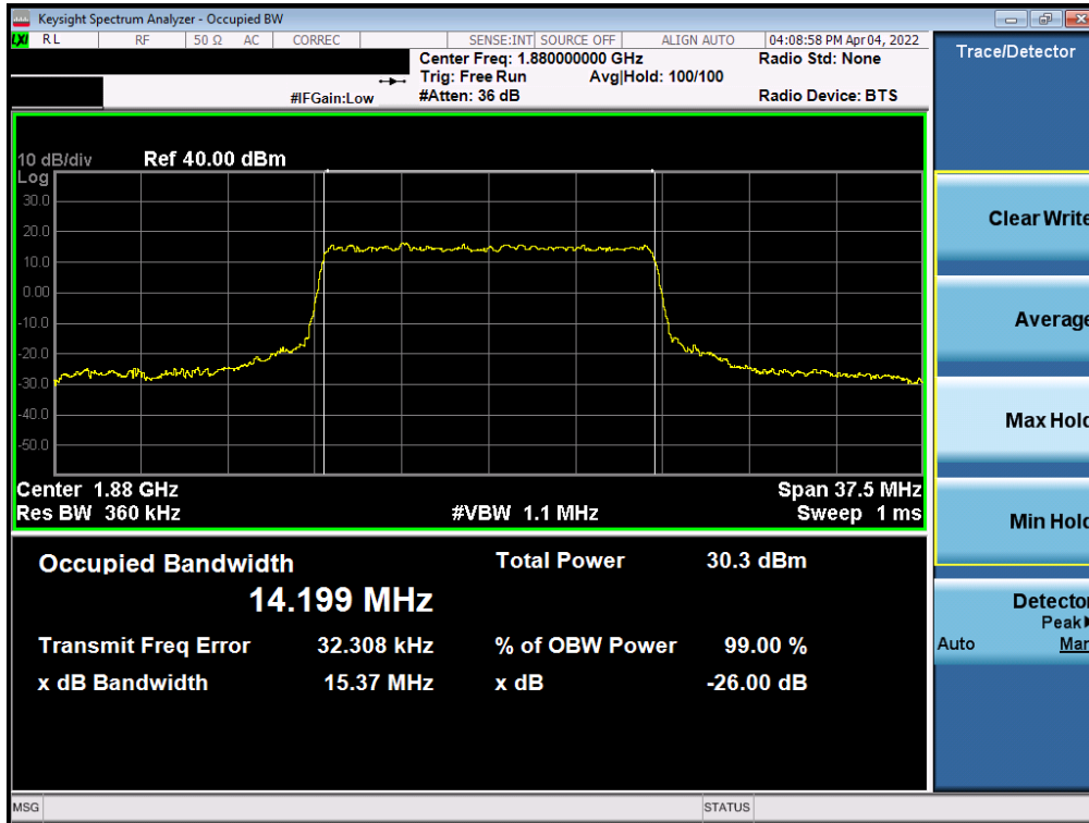
Plot 7-17. Occupied Bandwidth Plot (NR Band n2 - 15.0MHz CP-OFDM QPSK - Full RB)
