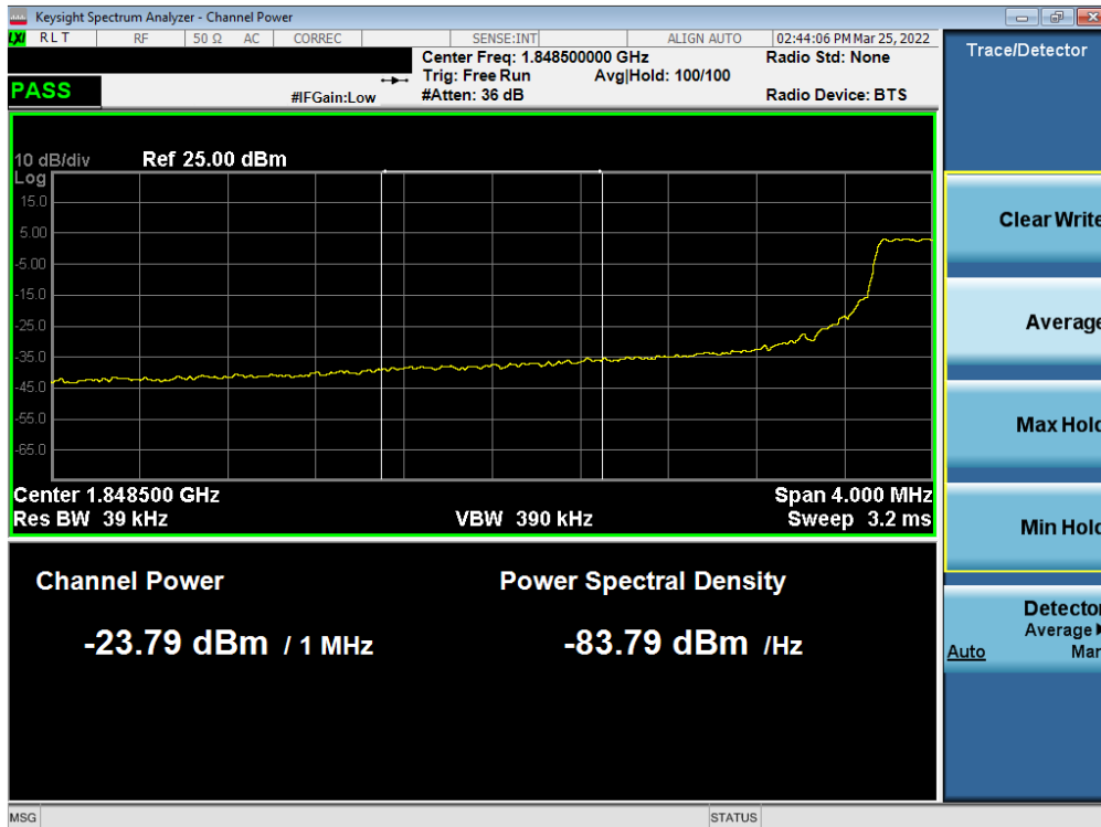
Plot 7-83. Extended Lower Band Edge Plot (LTE Band 25/2 - 5MHz QPSK – Full RB)
