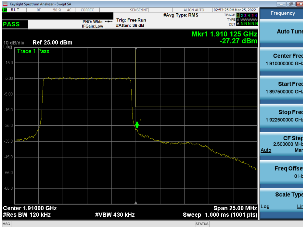
Plot 7-78. Upper Band Edge Plot (LTE Band 2 - 10MHz QPSK – Full RB)
