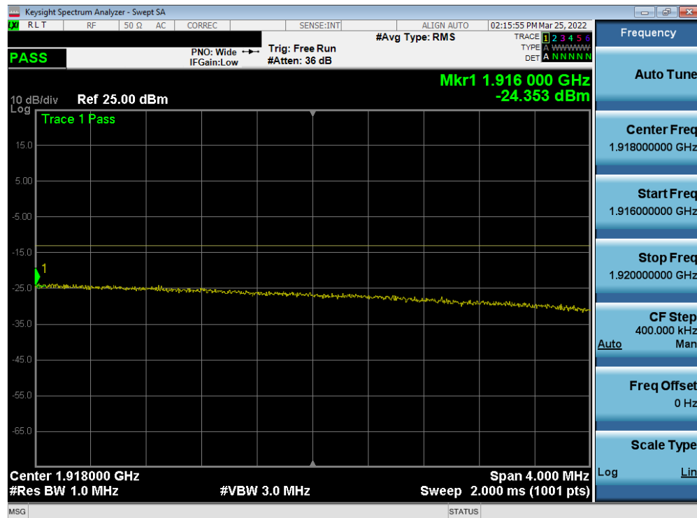
Plot 7-69. Extended Upper Band Edge Plot (LTE Band 25 - 20MHz QPSK – Full RB)
