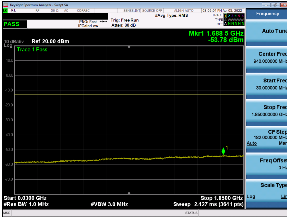
Plot 7-61. Conducted Spurious Plot (WCDMA Ch. 9538)
