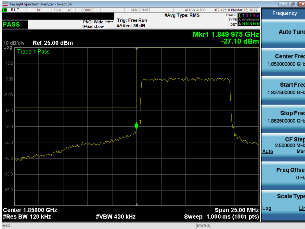
Plot 7-76. Lower Band Edge Plot (LTE Band 25/2 - 10MHz QPSK – Full RB)
