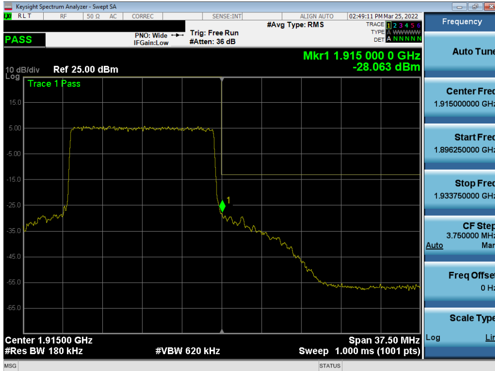
Plot 7-74. Upper Band Edge Plot (LTE Band 25 - 15MHz QPSK – Full RB)
