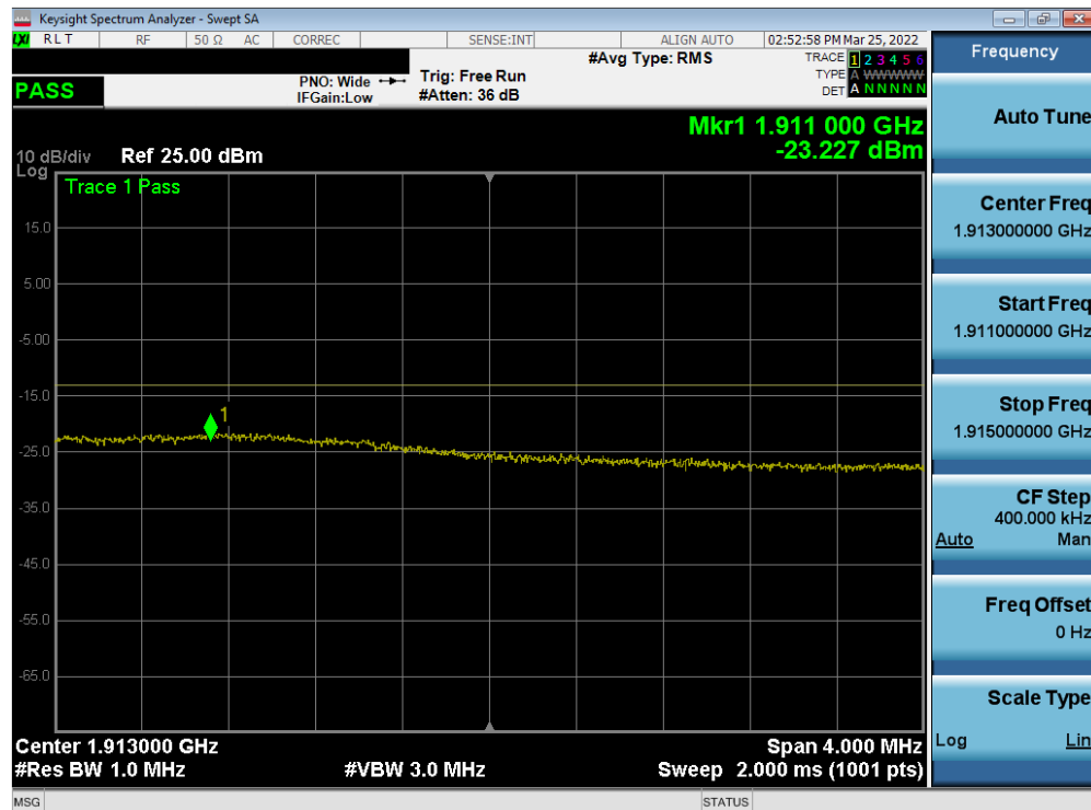
Plot 7-73. Extended Upper Band Edge Plot (LTE Band 2 - 15MHz QPSK – Full RB)
