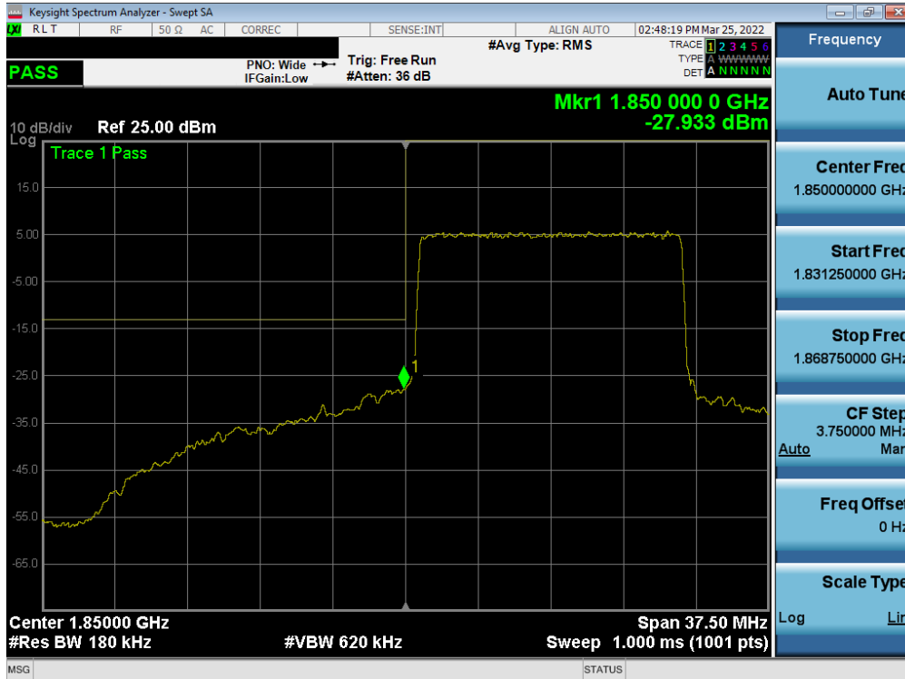
Plot 7-70. Lower Band Edge Plot (LTE Band 25/2 - 15MHz QPSK – Full RB)
