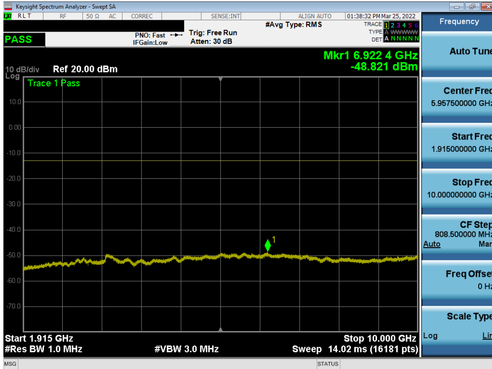
Plot 7-32. Conducted Spurious Plot (LTE Band 25/2 - 20MHz QPSK - 1RB - Mid Channel)
