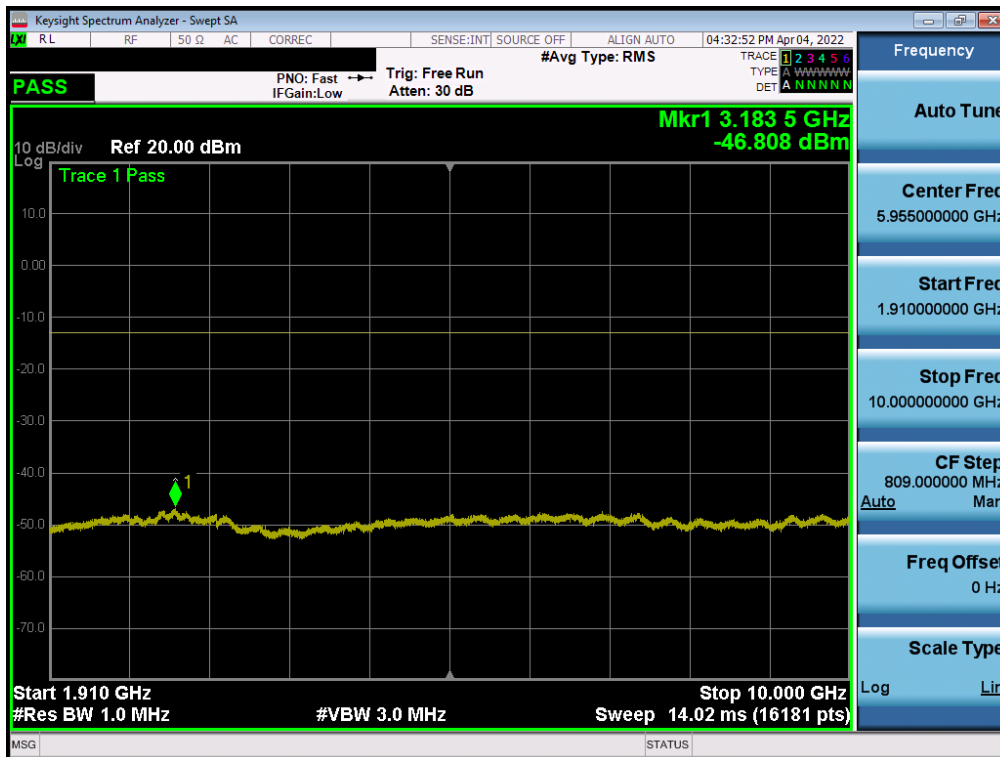
Plot 7-44. Conducted Spurious Plot (NR Band n2 - 20.0MHz - 1RB - High Channel)
