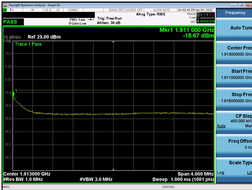
Plot 7-111. Upper Extended Band Edge Plot (NR Band n2 – 10.0MHz - Full RB)
