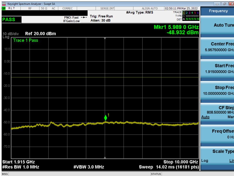
Plot 7-29. Conducted Spurious Plot (LTE Band 25/2 - 20MHz QPSK - 1RB - Low Channel)
