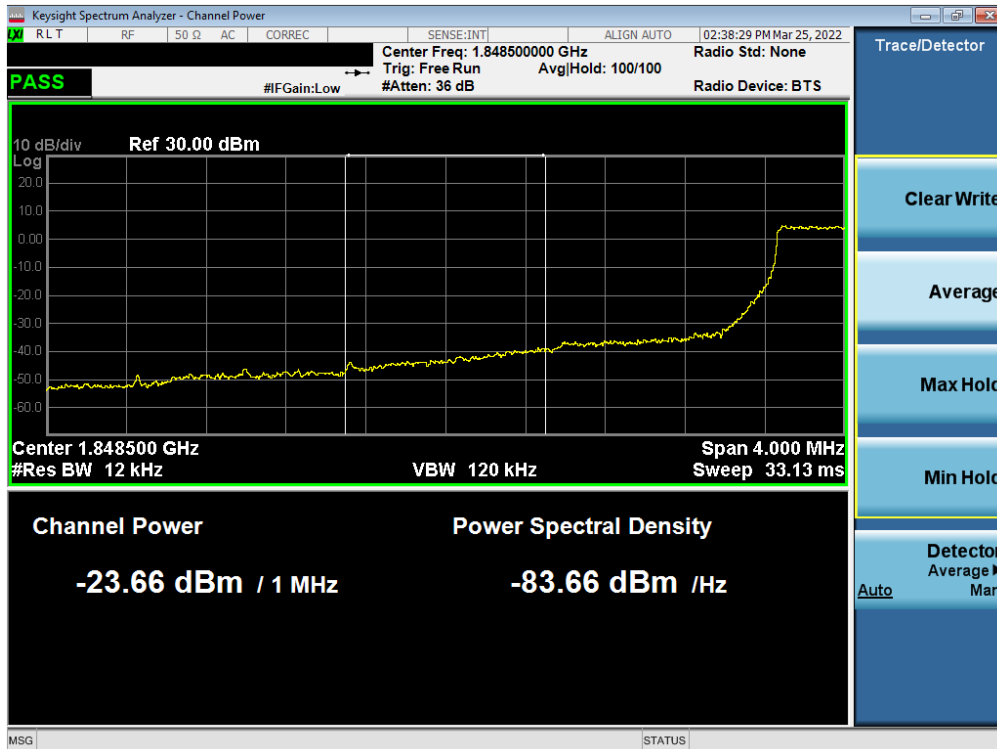
Plot 7-95. Extended Lower Band Edge Plot (LTE Band 25/2 – 1.4MHz QPSK – Full RB)
