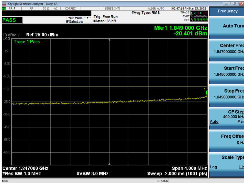
Plot 7-77. Extended Lower Band Edge Plot (LTE Band 25/2 - 10MHz QPSK – Full RB)
