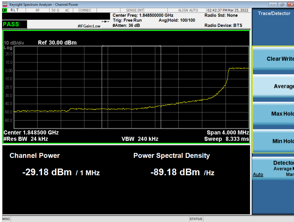
Plot 7-89. Extended Lower Band Edge Plot (LTE Band 25/2 - 3MHz QPSK – Full RB)
