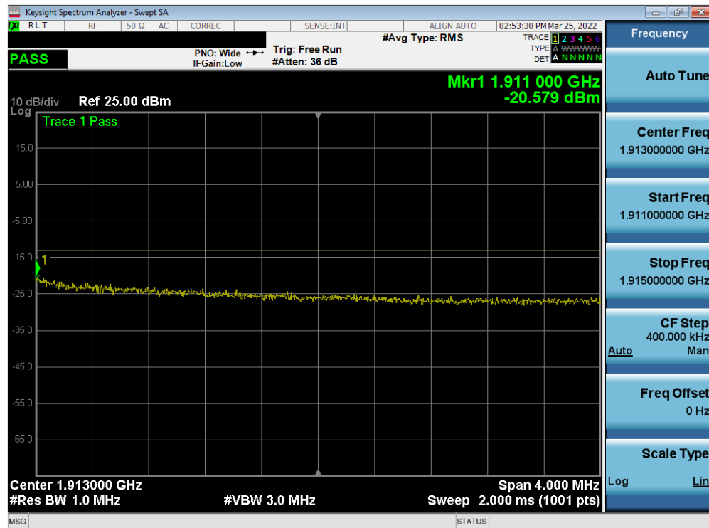
Plot 7-79. Extended Upper Band Edge Plot (LTE Band 2 - 10MHz QPSK – Full RB)
