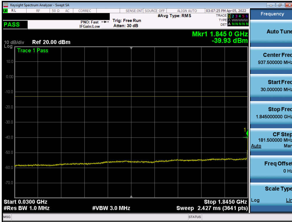
Plot 7-55. Conducted Spurious Plot (WCDMA Ch. 9262)
