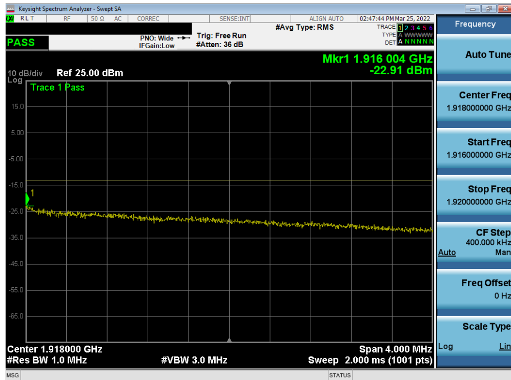
Plot 7-81. Extended Upper Band Edge Plot (LTE Band 25 - 10MHz QPSK – Full RB)
