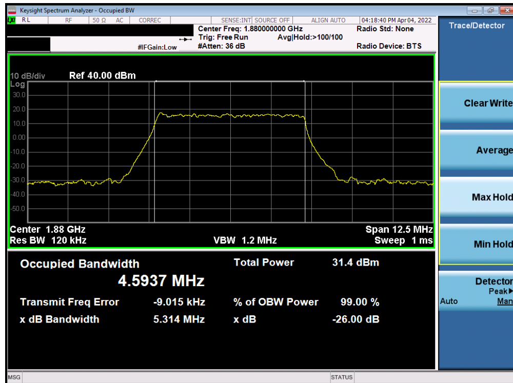
Plot 7-22. Occupied Bandwidth Plot (NR Band n2 - 5.0MHz DFT-S-OFDM BPSK - Full RB)
