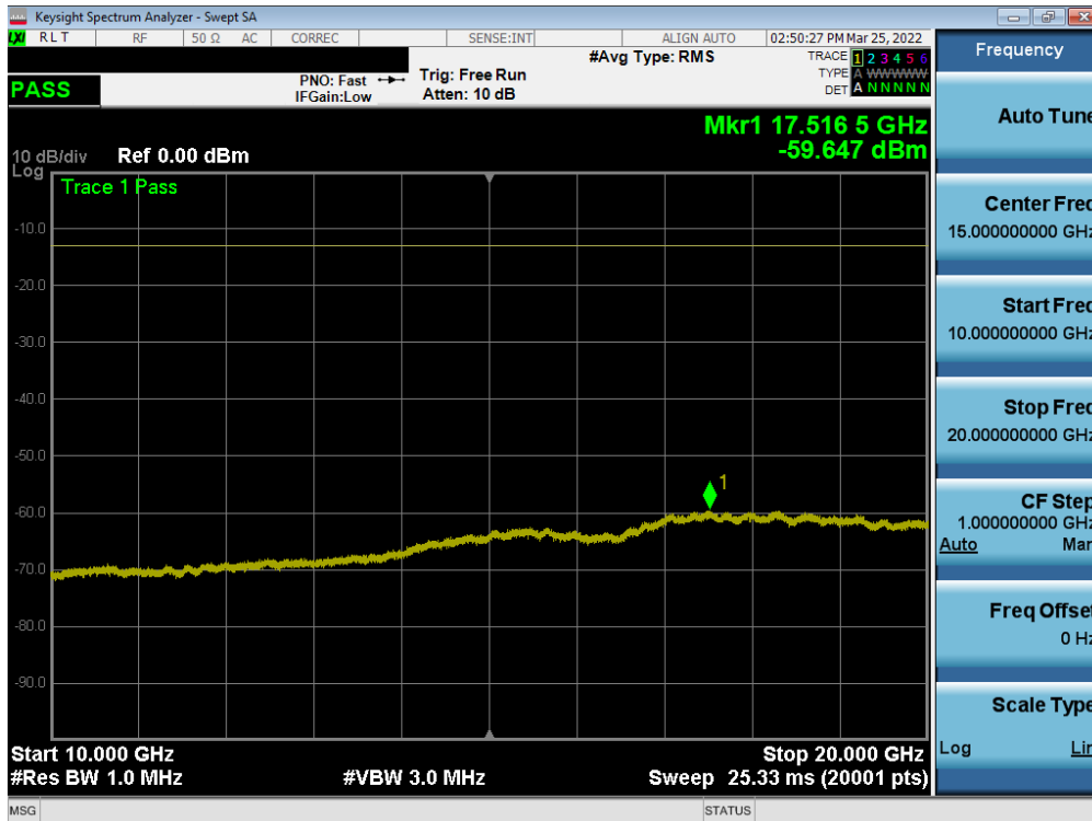
Plot 7-30. Conducted Spurious Plot (LTE Band 25/2 - 20MHz QPSK - 1RB - Low Channel)
