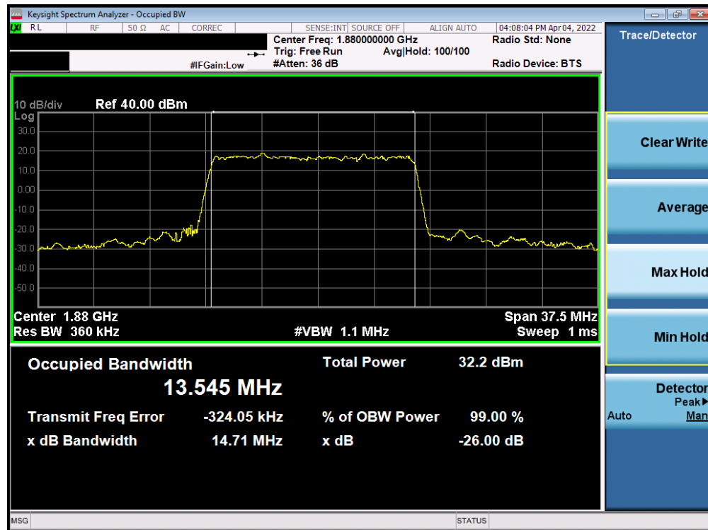
Plot 7-16. Occupied Bandwidth Plot (NR Band n2 - 15.0MHz DFT-S-OFDM BPSK - Full RB)
