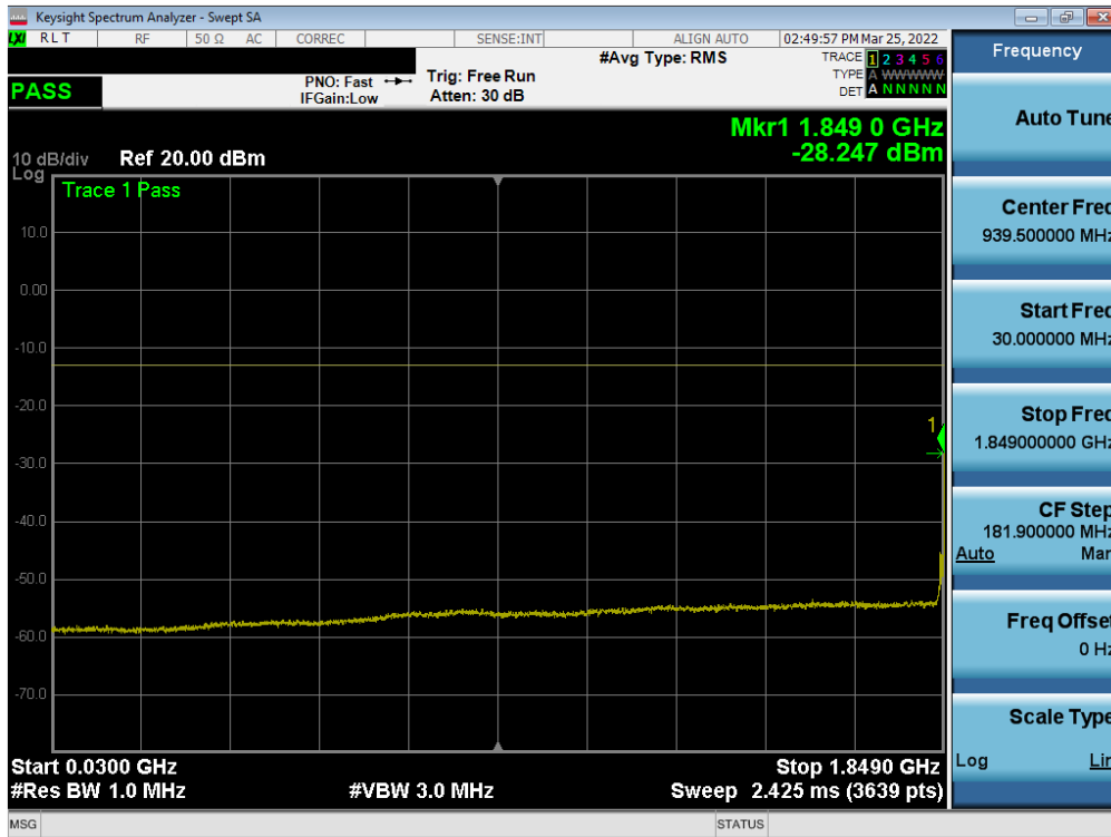
Plot 7-28. Conducted Spurious Plot (LTE Band 25/2 - 20MHz QPSK - 1RB - Low Channel)
