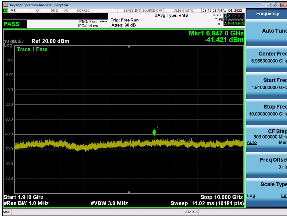
Plot 7-50. Conducted Spurious Plot (GPRS Ch. 661)
