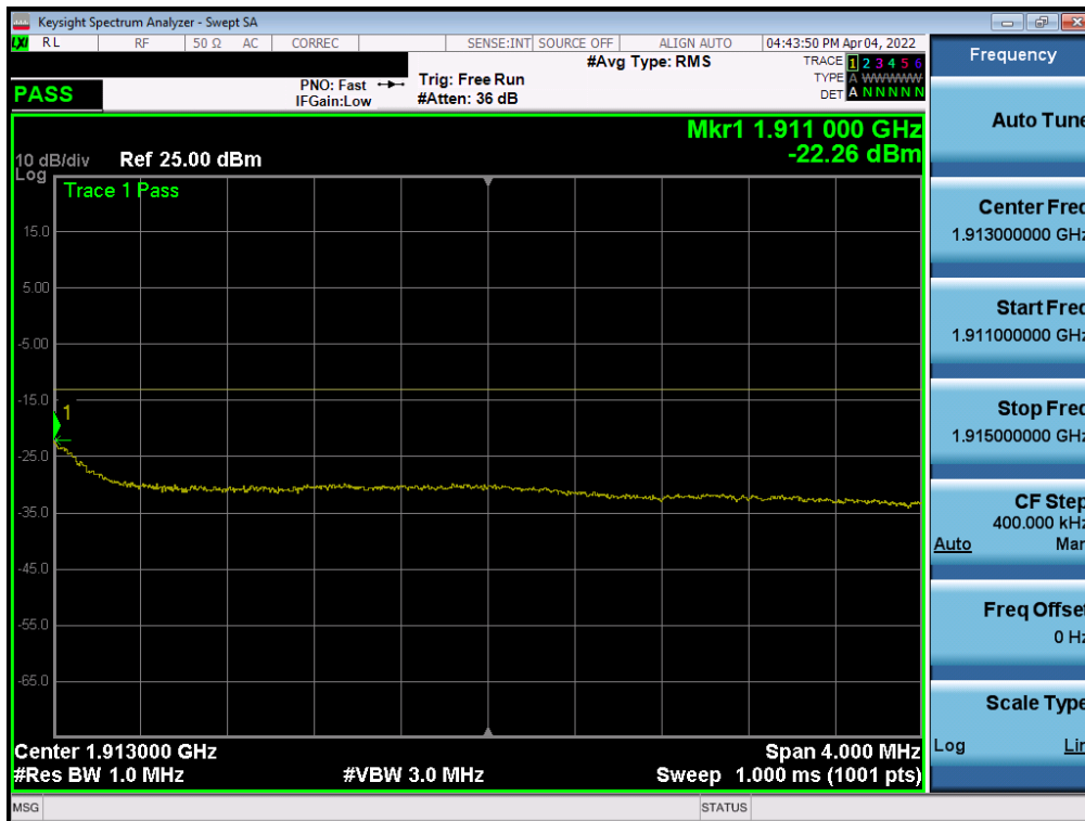
Plot 7-107. Upper Extended Band Edge Plot (NR Band n2 – 15.0MHz - Full RB)
