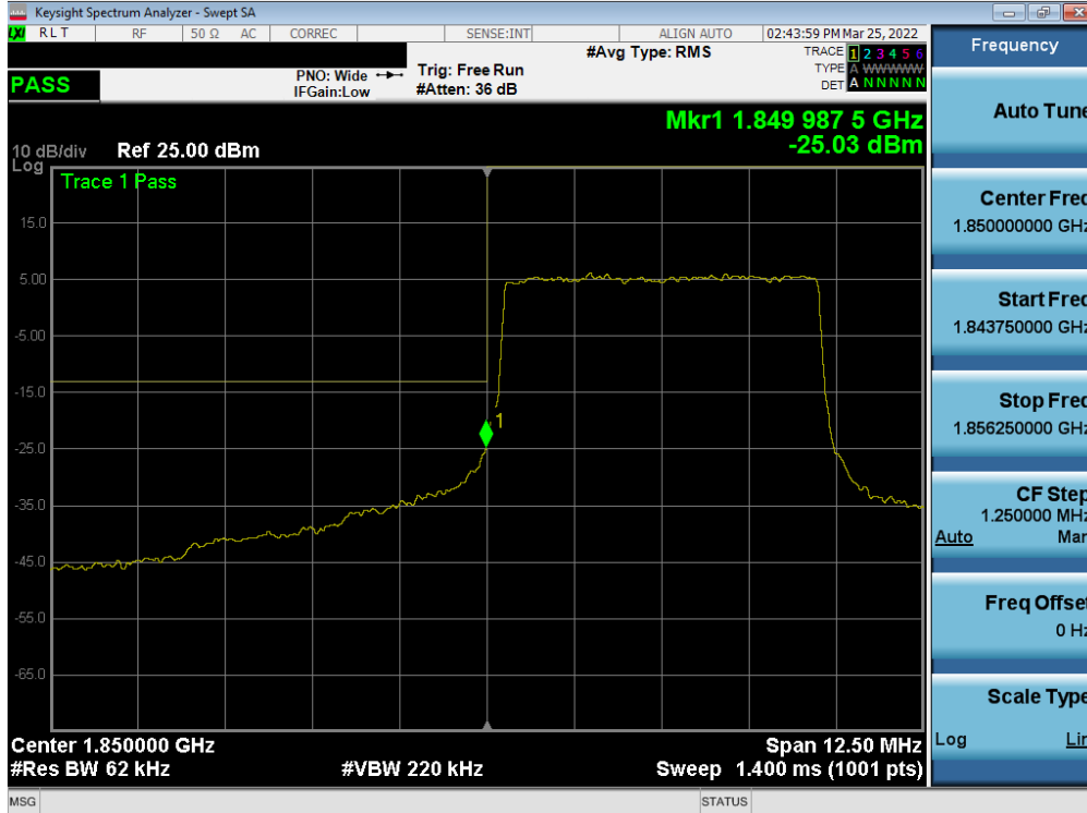
Plot 7-82. Lower Band Edge Plot (LTE Band 25/2 - 5MHz QPSK – Full RB)
