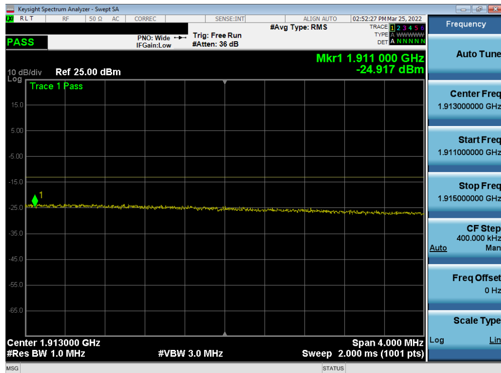
Plot 7-67. Extended Upper Band Edge Plot (LTE Band 2 - 20MHz QPSK – Full RB)
