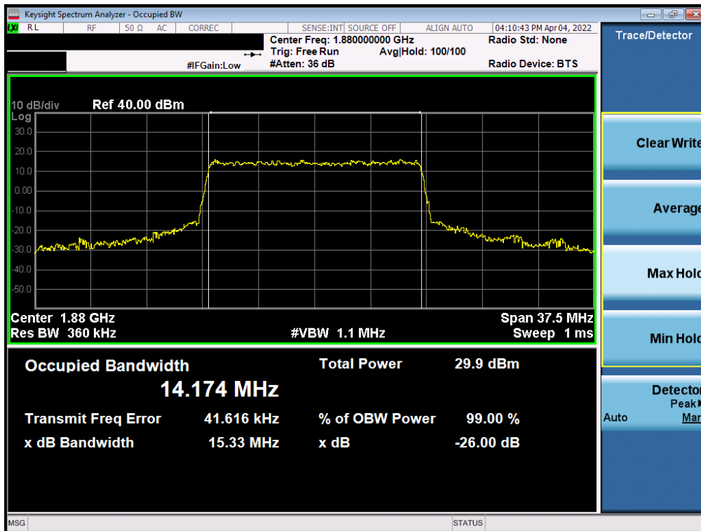
Plot 7-18. Occupied Bandwidth Plot (NR Band n2 - 15.0MHz CP-OFDM 16QAM - Full RB)
