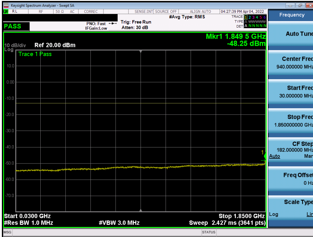
Plot 7-37. Conducted Spurious Plot (NR Band n2 -20.0MHz - 1RB - Low Channel)
