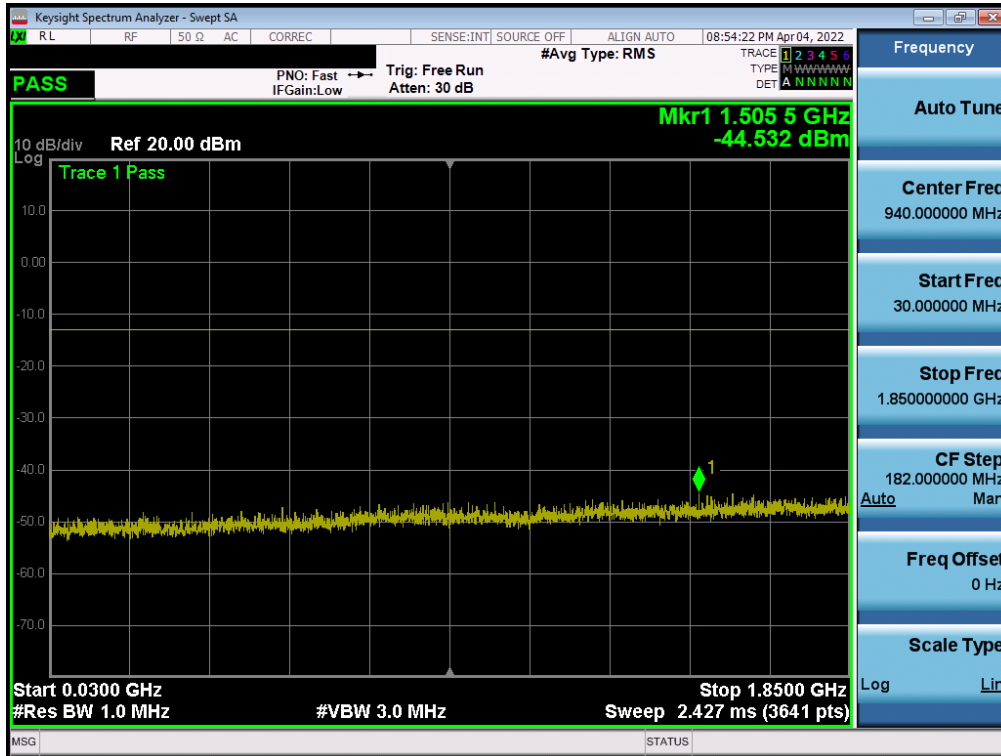
Plot 7-52. Conducted Spurious Plot (GPRS Ch. 810)
