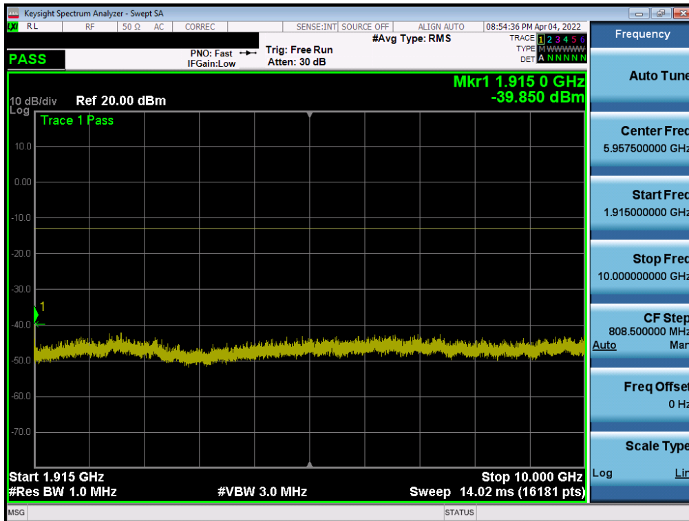
Plot 7-53. Conducted Spurious Plot (GPRS Ch. 810)
