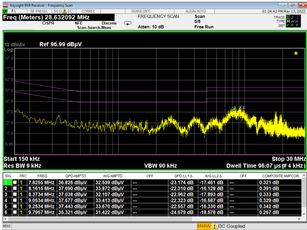
Plot 7-363. Line Conducted Plot with 802.11a UNII Band 5 (N)
