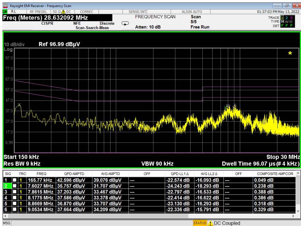
Plot 7-367. Line Conducted Plot with 802.11a UNII Band 7 (N)
