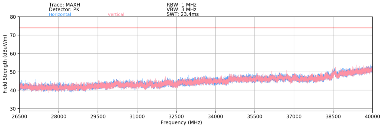
Plot 7-348. Radiated Spurious Plot 26.5GHz - 40GHz – CH 117 - MIMO (802.11ax)
