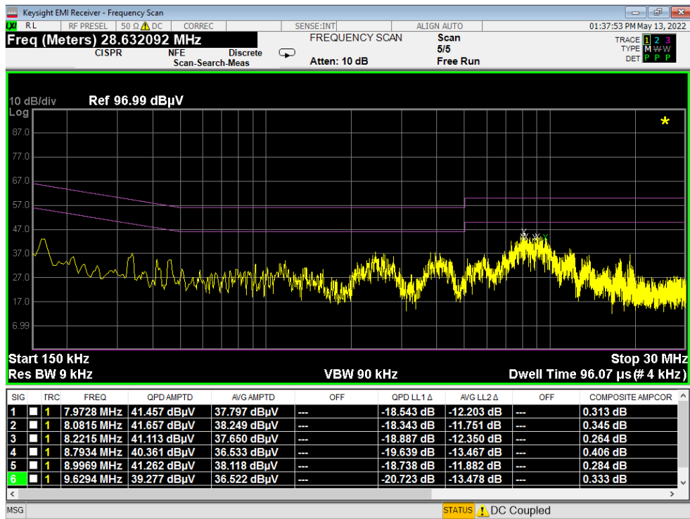
Plot 7-366. Line Conducted Plot with 802.11a UNII Band 7 (L1)
