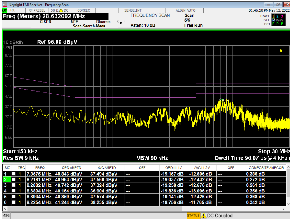
Plot 7-368. Line Conducted Plot with 802.11a UNII Band 8 (L1)
