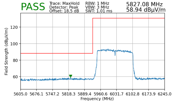
Plot 7-358. Radiated Lower Band Edge Plot MIMO (Peak – UNII Band 5)
