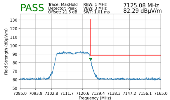
Plot 7-352. Radiated Upper Band Edge Plot MIMO (Peak – UNII Band 8)
