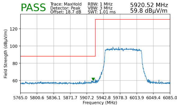
Plot 7-355. Radiated Lower Band Edge Plot MIMO (Peak – UNII Band 5)
