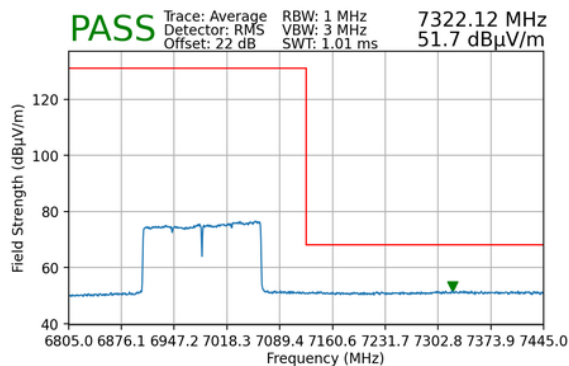
Plot 7-359. Radiated Upper Band Edge Plot MIMO (Average – UNII Band 8)
