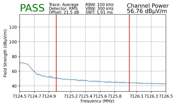
Plot 7-351. Radiated Upper Band Edge Plot MIMO (Average – UNII Band 8)
