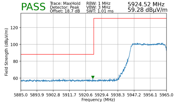
Plot 7-350. Radiated Lower Band Edge Plot MIMO (Peak – UNII Band 5)
