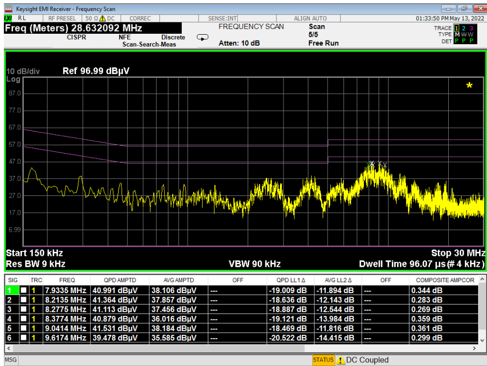
Plot 7-364. Line Conducted Plot with 802.11a UNII Band 6 (L1)
