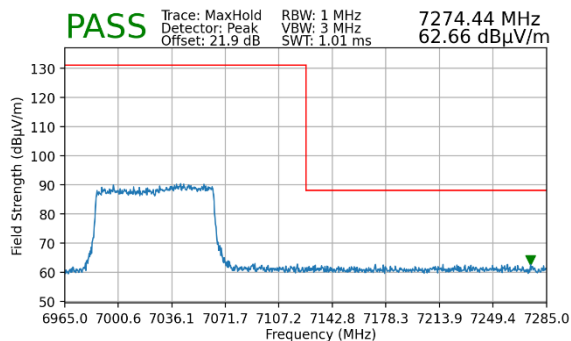
Plot 7-356. Radiated Upper Band Edge Plot MIMO (Peak – UNII Band 8)
