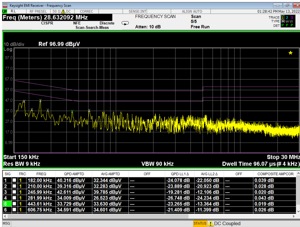
Plot 7-370. Line Conducted Plot with 802.11a UNII Band 5 (L1) with WCP
