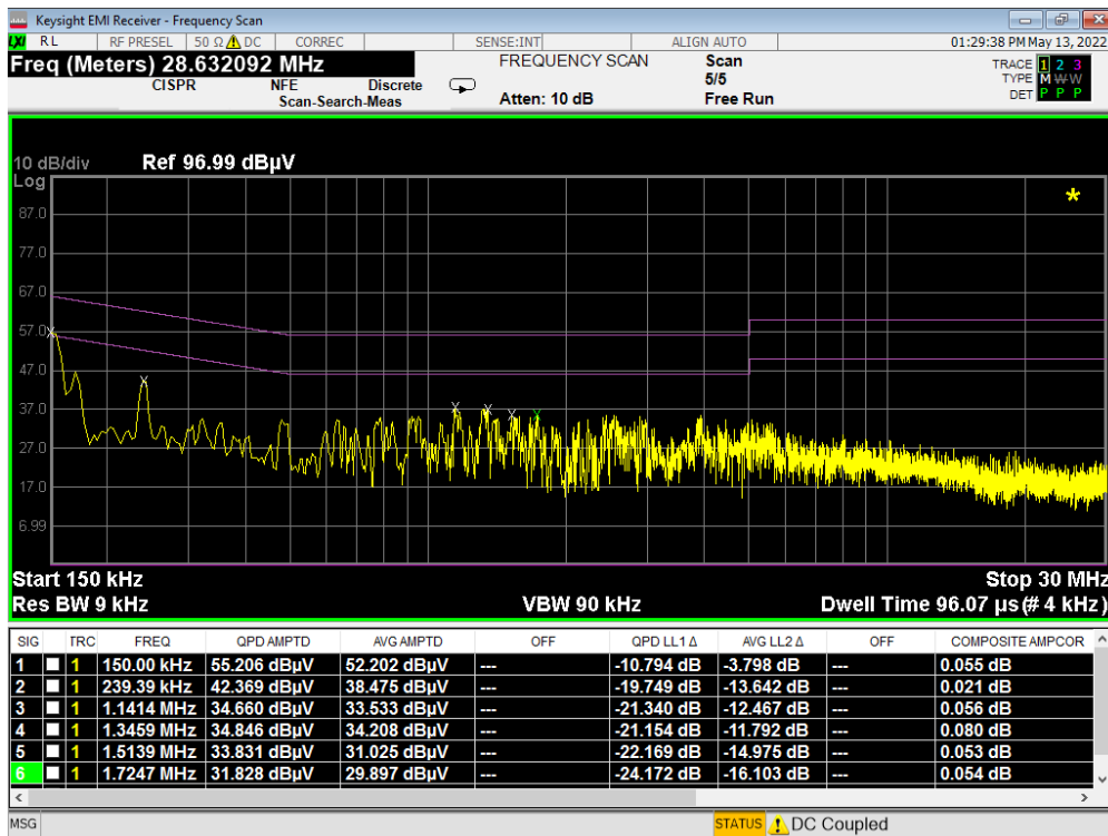
Plot 7-371. Line Conducted Plot with 802.11a UNII Band 5 (N) with WCP
