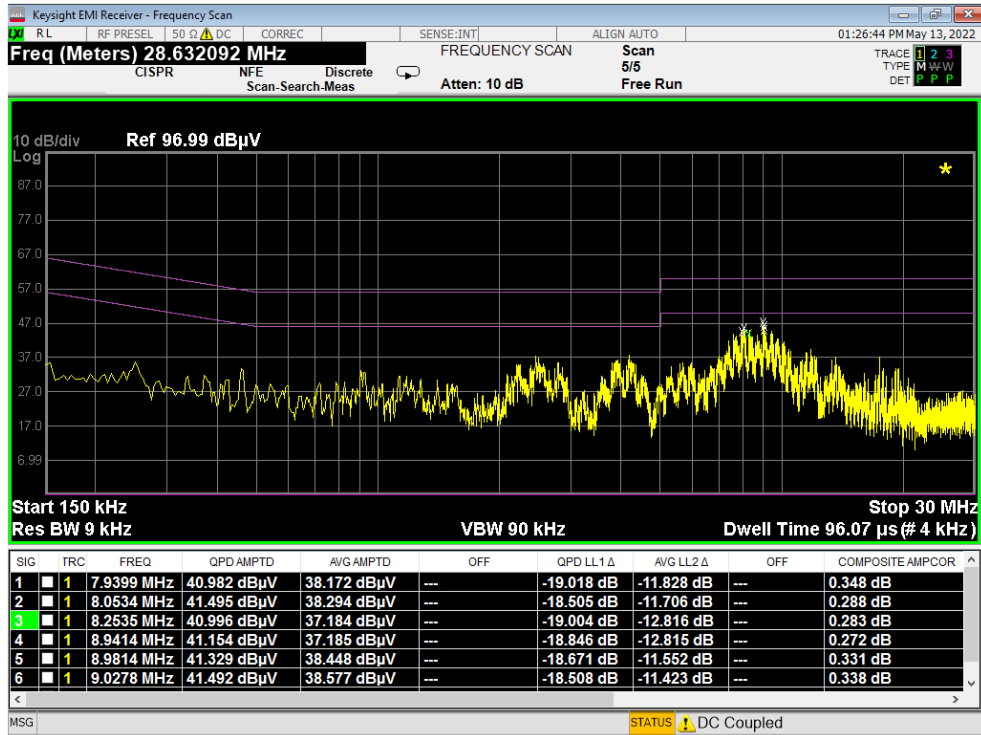
Plot 7-362. Line Conducted Plot with 802.11a UNII Band 5 (L1)
