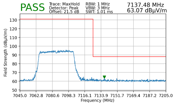
Plot 7-354. Radiated Upper Band Edge Plot MIMO (Peak – UNII Band 8)
