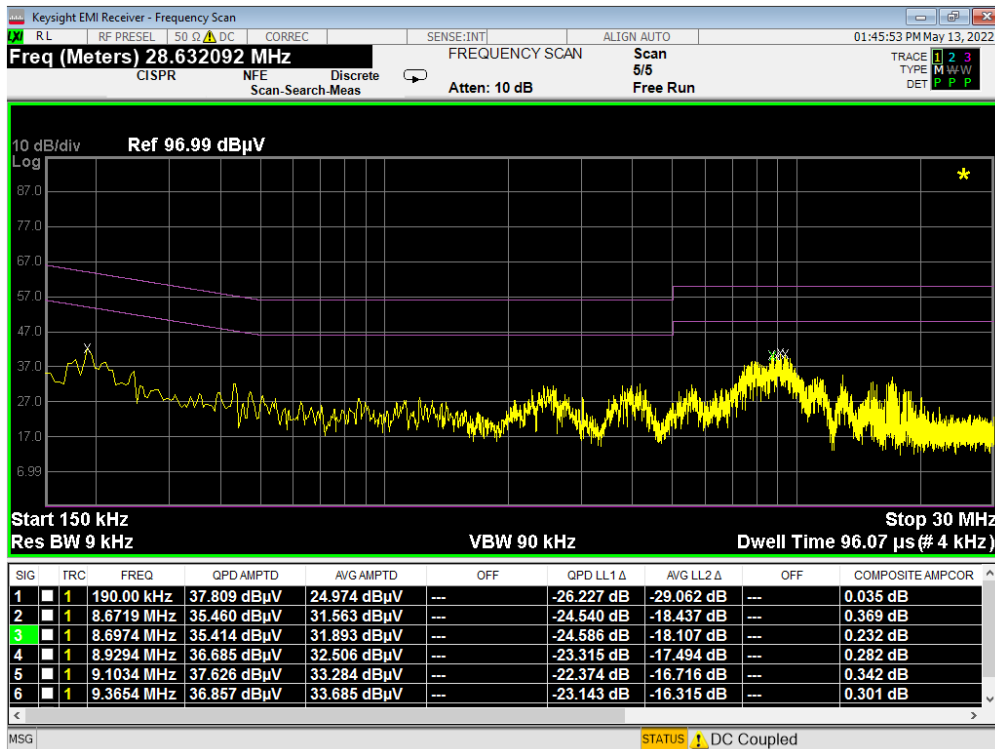
Plot 7-369. Line Conducted Plot with 802.11a UNII Band 8 (N)
