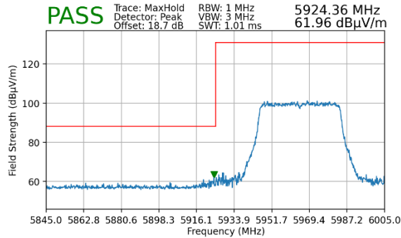
Plot 7-353. Radiated Lower Band Edge Plot MIMO (Peak – UNII Band 5)
