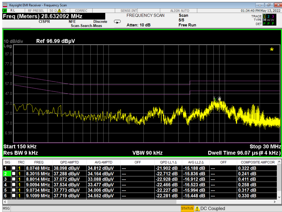
Plot 7-365. Line Conducted Plot with 802.11a UNII Band 6 (N)
