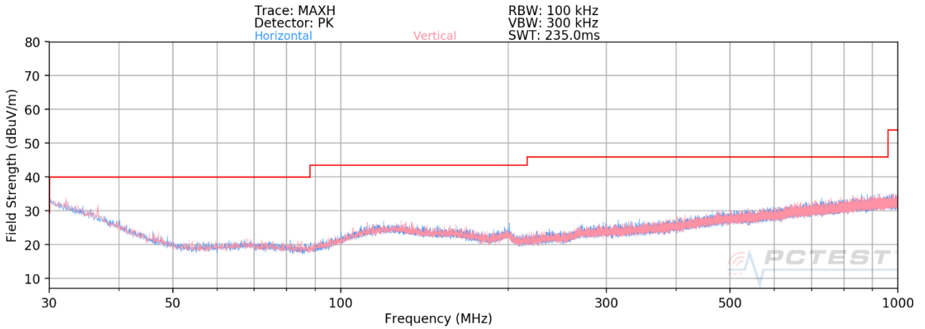
Plot 7-361. Radiated Spurious Plot below 1GHz
