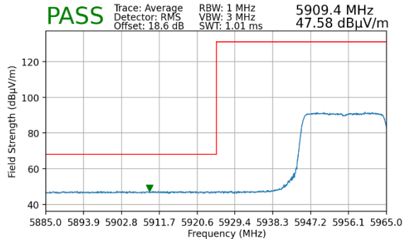
Plot 7-349. Radiated Lower Band Edge Plot MIMO (Average – UNII Band 5)
