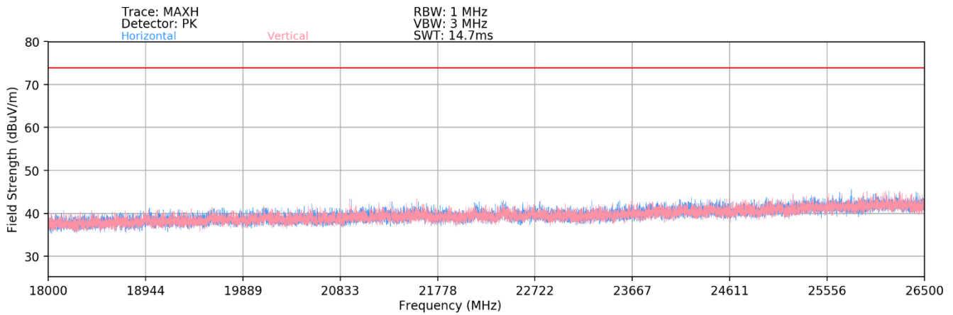
Plot 7-347. Radiated Spurious Plot above 18GHz - 26.5GHz – CH 117 - MIMO (802.11ax)
