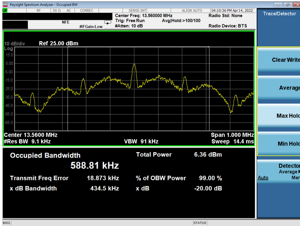
Figure 7-2. Occupied Bandwidth Plot -Type A
