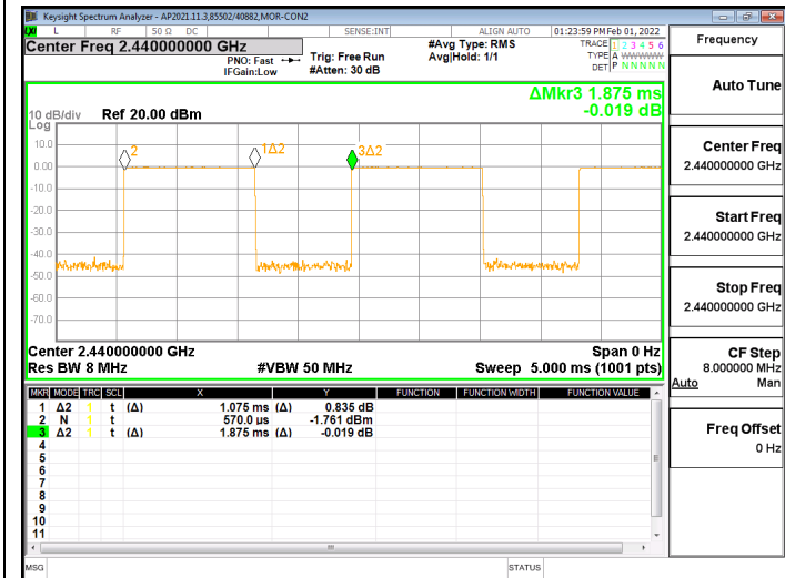
DUTY CYCLE BLE – 2Mbps CHAIN 0
