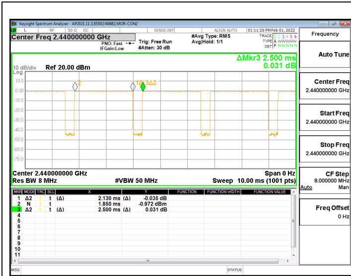
DUTY CYCLE BLE – 1Mbps CHAIN 0
