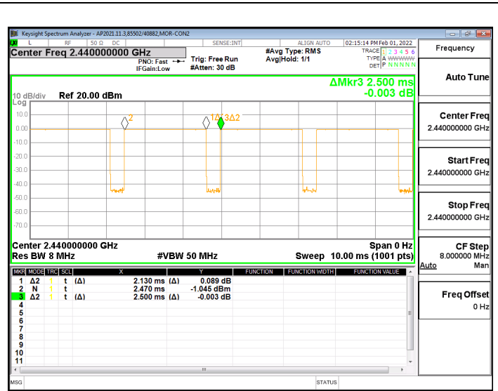
DUTY CYCLE BLE – 1Mbps CHAIN 1
