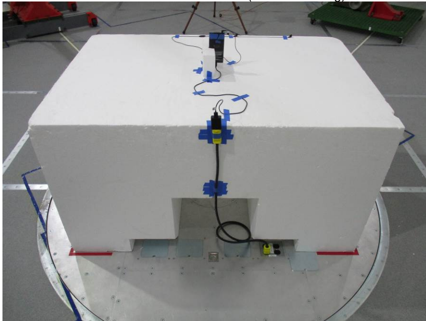
RADIATED EMISSIONS BELOW 30MHz (BACK with Tag)
