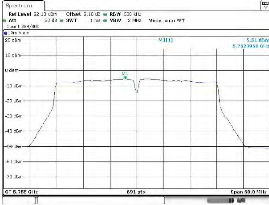
11N40MIMO Ant2_5755
