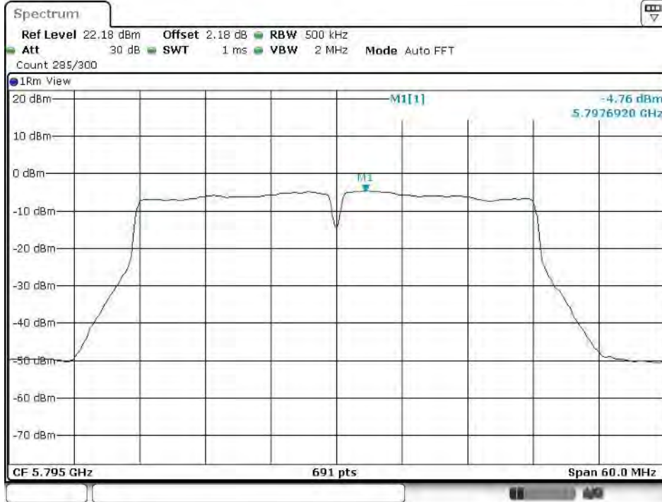
11N40MIMO Ant1_5795
