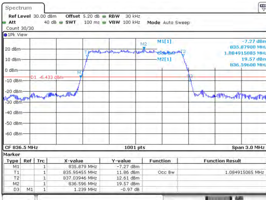
Band5-1.4MHz-QPSK-20525-6RB#0-1.085
