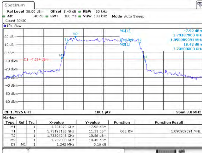
Band4-1.4MHz-QPSK-20175-6RB#0-1.091
