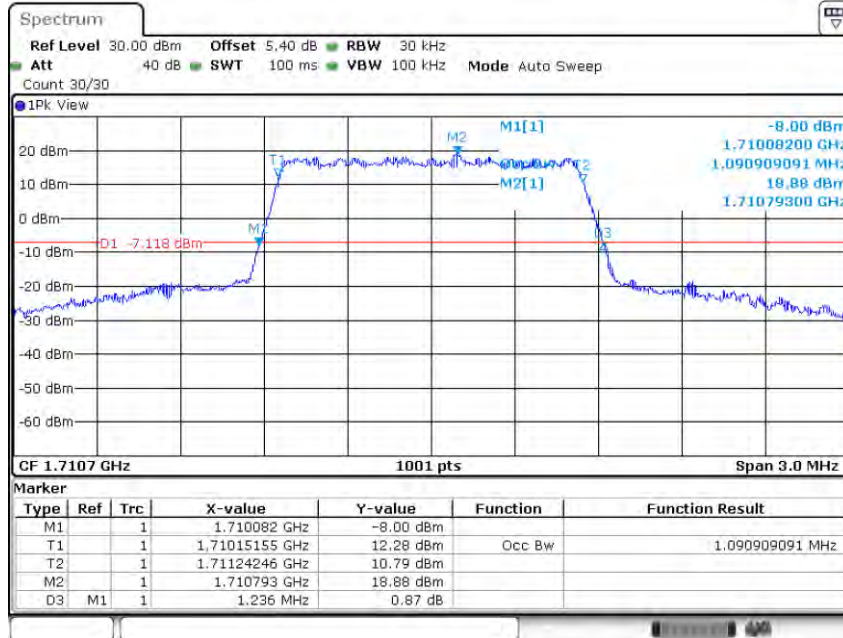
Band4-1.4MHz-QPSK-19957-6RB#0-1.091
