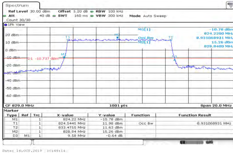
Band5-10MHz-QPSK-20525-50RB#0-8.931
