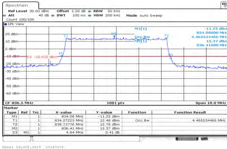
Band5-5MHz-QPSK-20625-25RB#0-4.466
