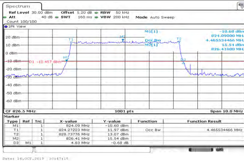
Band5-5MHz-QPSK-20525-25RB#0-4.466
