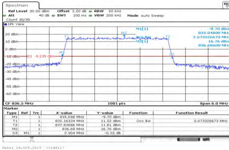
Band5-3MHz-16QAM-20635-15RB#0-2.673
