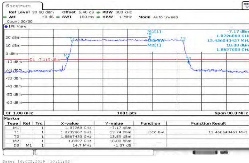
Band2-15MHz-QPSK-19125-75RB#0-13.457
