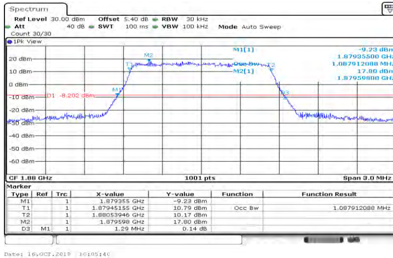
Band2-1.4MHz-16QAM-19193-6RB#0-1.088
