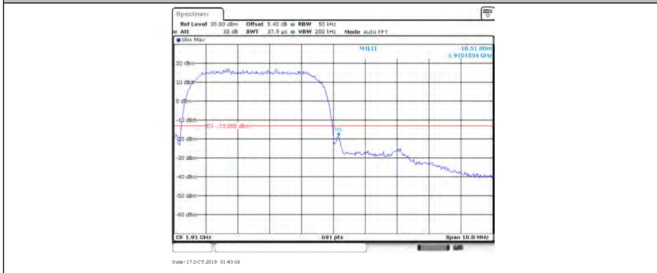
Band II_9538_QPSK
