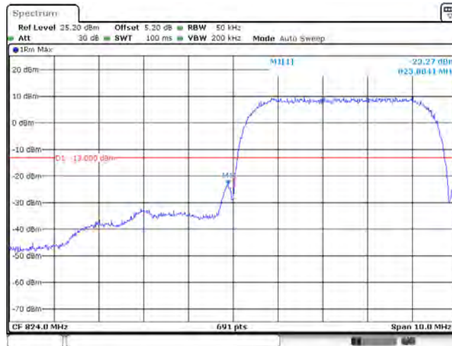
Band V_4132_QPSK
