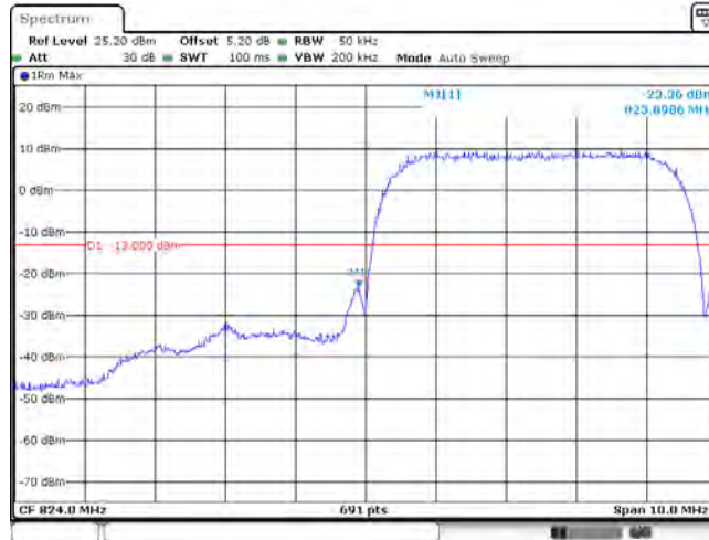
Band V_4132_16QAM
