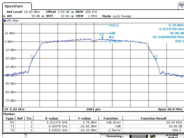
26dB_802.11n_HT20_5320MHz
