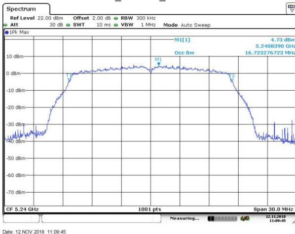
OBW_802.11a_5240MHz
