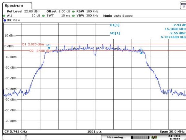
6dB BW_802.11a_5745MHz
