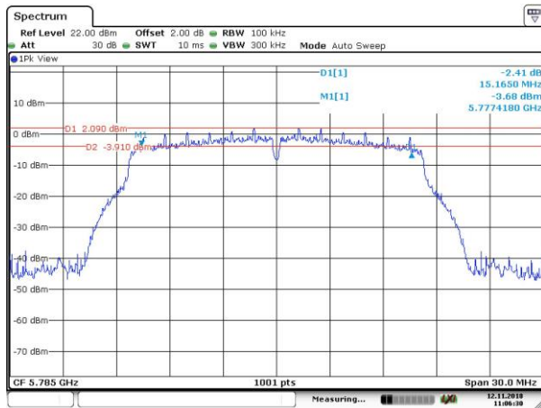
6dB BW_802.11a_5785MHz
