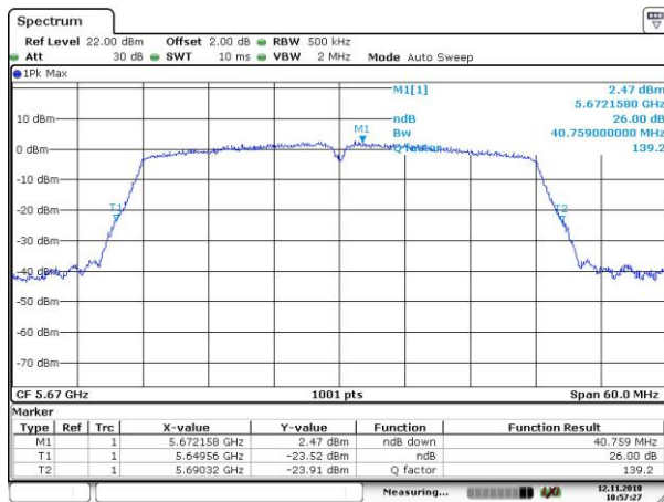
26dB_802.11n_HT40_5670MHz
