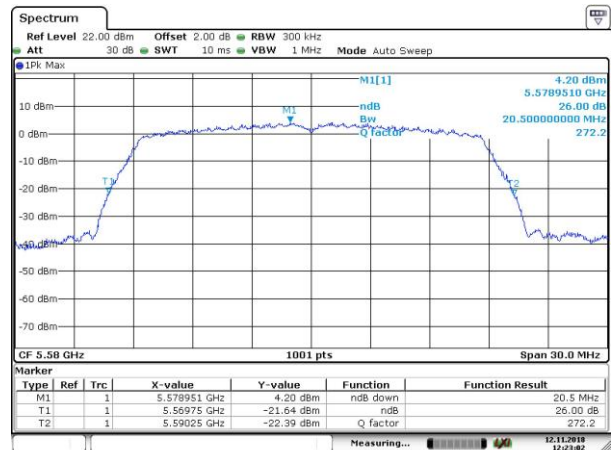
26dB_802.11n_HT20_5580MHz
