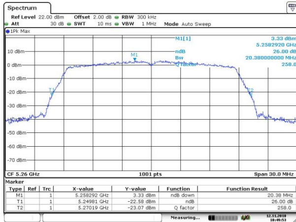
26dB_802.11n_HT20_5260MHz
