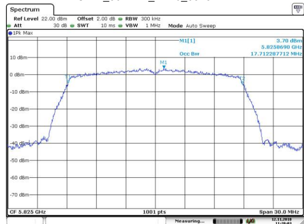
OBW_802.11n_HT20_5825MHz
