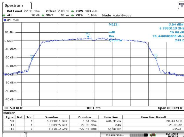
26dB_802.11n_HT20_5300MHz
