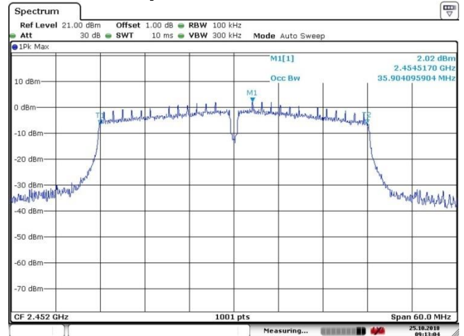
Power Density_802.11n_40MHz_Chain0_2452MHz
