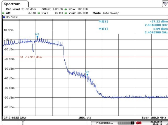
Bandedge_802.11n_40MHz_Chain0_2452MHz
