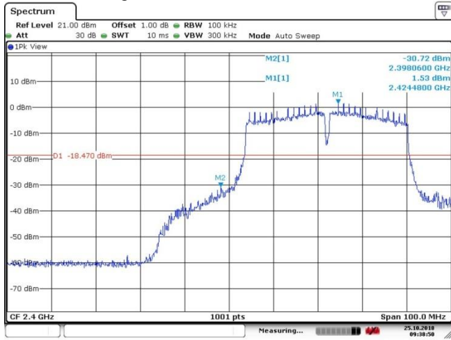
Bandedge_802.11n_40MHz_Chain0_2422MHz
