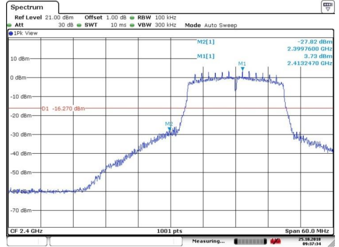
Bandedge_802.11n_20MHz_Chain0_2412MHz
