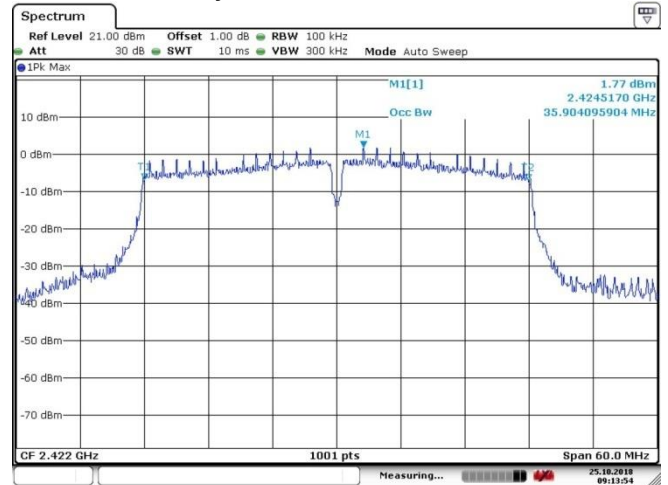
Power Density_802.11n_40MHz_Chain0_2422MHz
