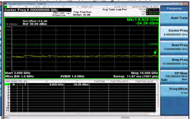
3GHz~10GHz_WCDMA_B5_HighCH4233-846.6
