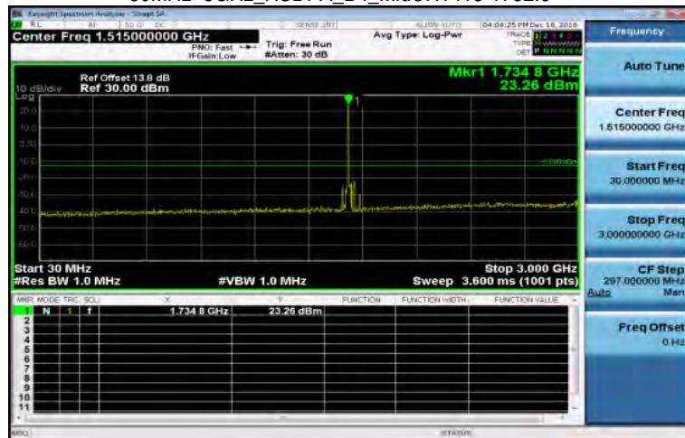
30MHz~3GHz_HSDPA_B4_MidCH1413-1732.6
