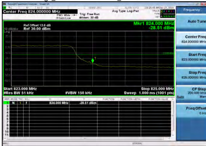
Band Edge_Band 26 for Part 90S_5M-QPSK-25 0-HIGH
