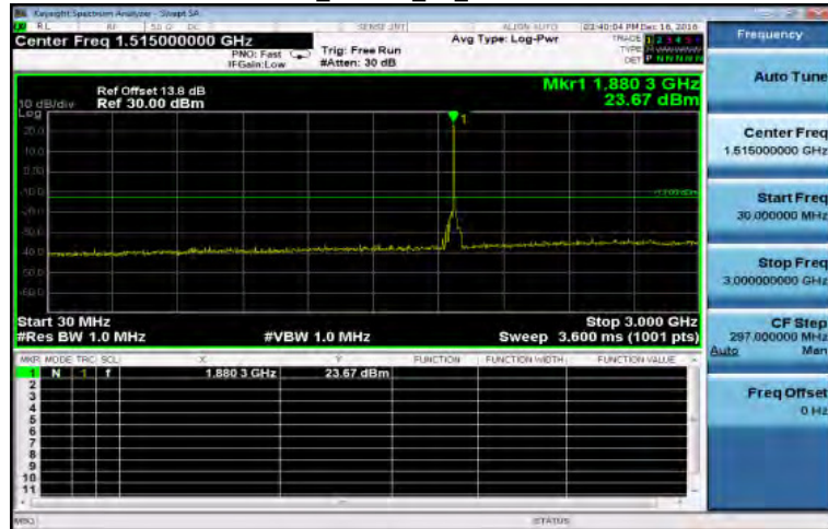
30MHz~3GHz_HSDPA_B2_MidCH9400-1880
