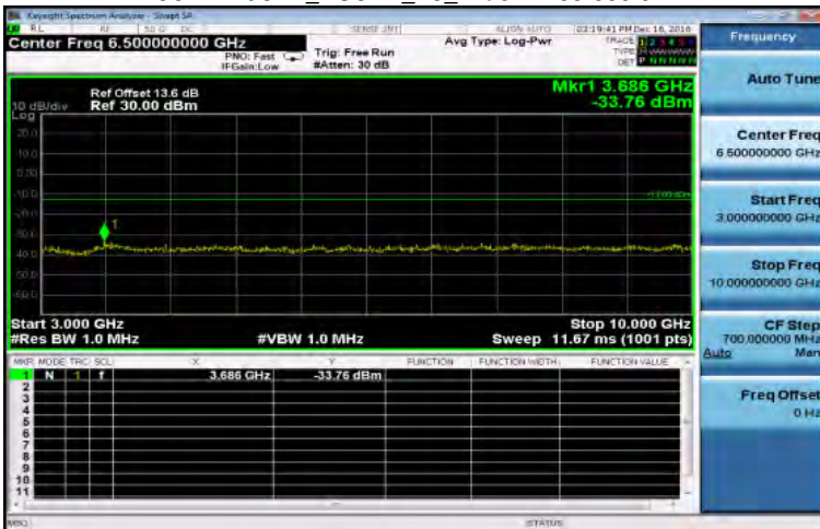
3GHz~10GHz_HSUPA_B5_MidCH4183-836.6
