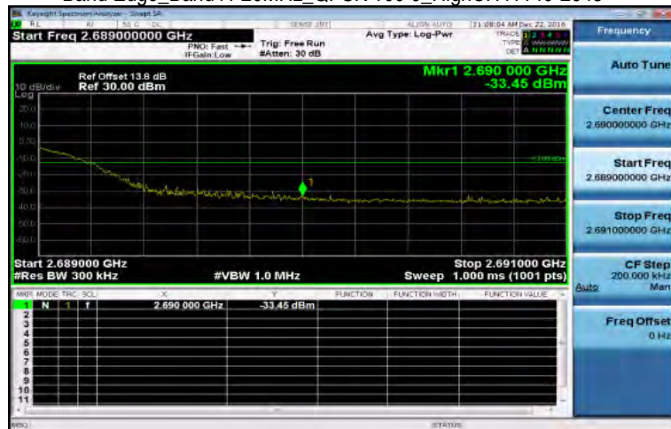
Band Edge_Band41 20MHz_QPSK 100 0_HighCH41140-2645
