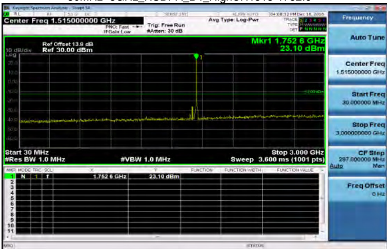
30MHz~3GHz_HSDPA_B4_HighCH1513-1752.6
