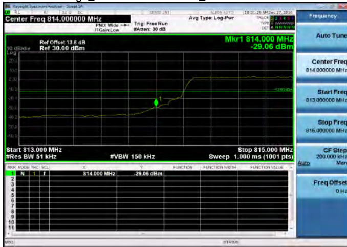
Band Edge_Band 26 for Part 90S_5M-QPSK-25 0-LOW
