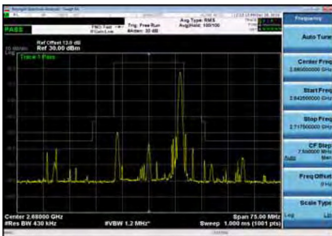
Emission Mask_Band 41_20M_QPSK_HIGH_RB1,99
