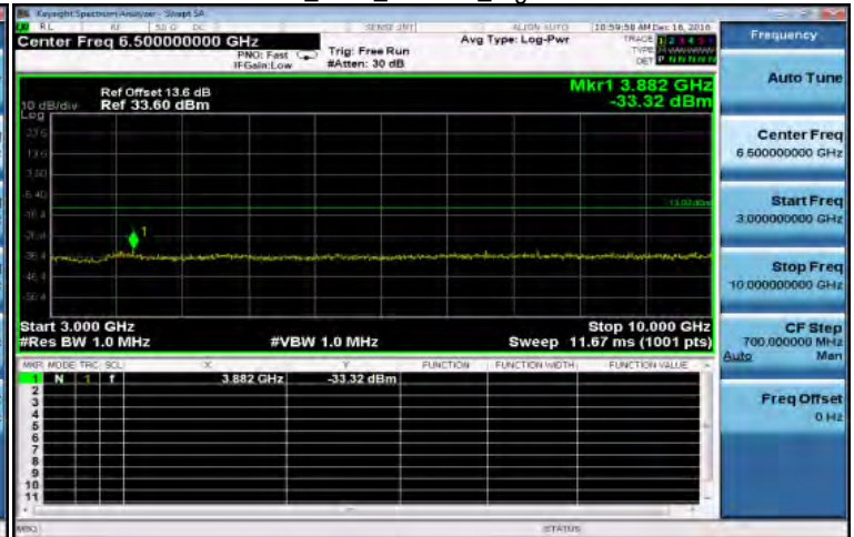
3GHz~10GHz_GSM_850MHz_HighCH251-848.8
