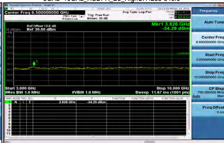
3GHz~10GHz_HSDPA_B5_HighCH4233-846.6
