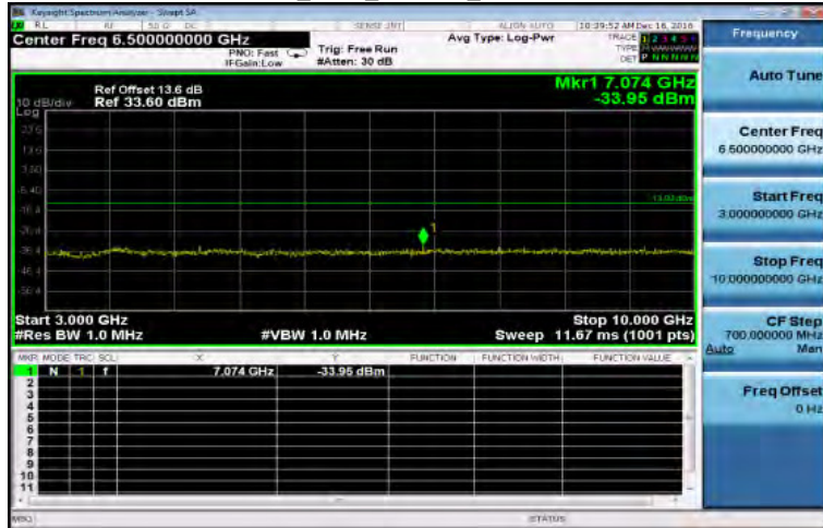
3GHz~10GHz_GSM_850MHz_LowCH128-824.2
