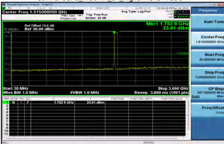
30MHz~3GHz_WCDMA_B4_HighCH1513-1752.6
