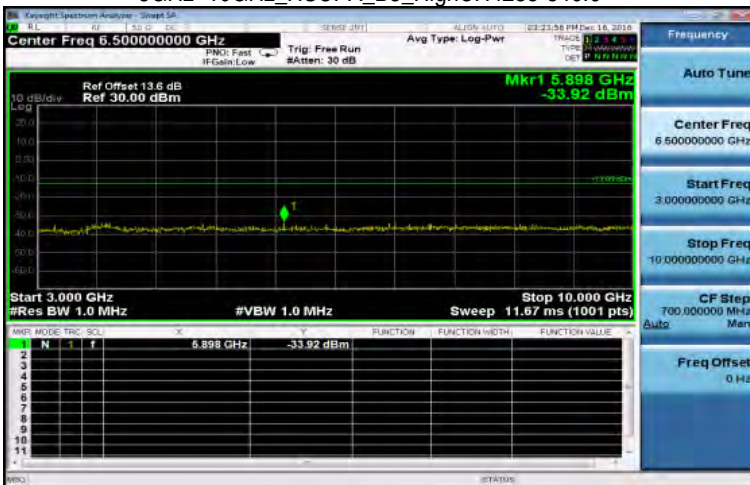
3GHz~10GHz_HSUPA_B5_HighCH4233-846.6
