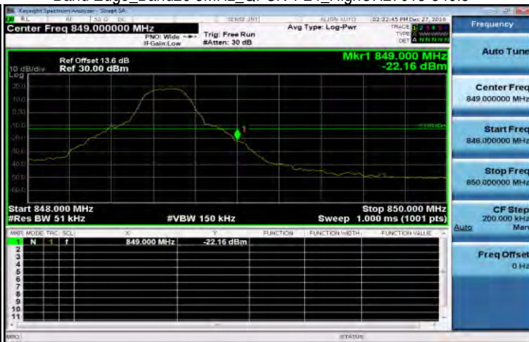
Band Edge_Band26 5MHz_QPSK 1 24_HighCH27015-846.5
