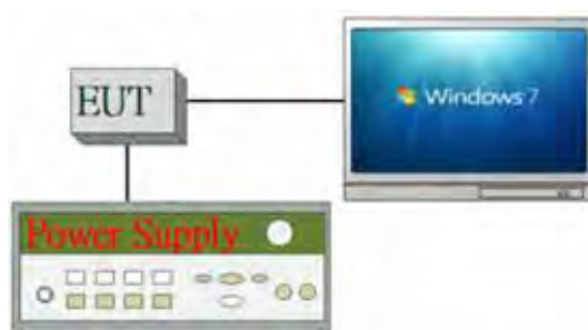
Fig. 2-2 Conducted (Antenna Port) Configuration
