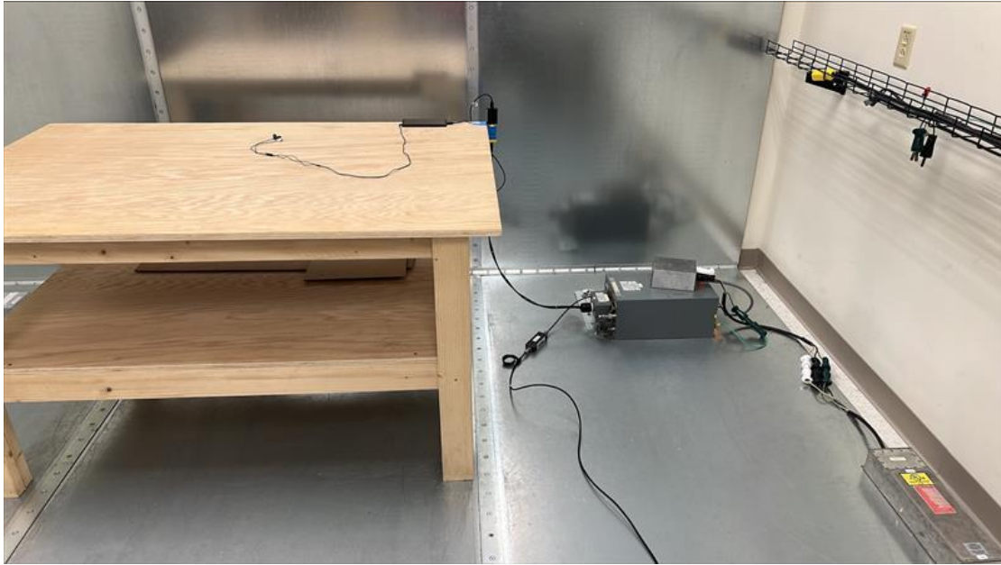
AC Mains Conducted Emissions AC Adaptor Setup
