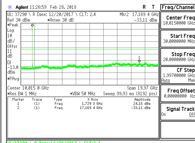
LTE B4 5MHz 16QAM Middle Channel RB1-0
