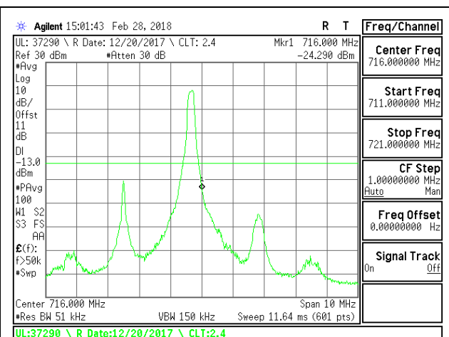
LTE B17 5MHz 16QAM High Channel RB1-0
