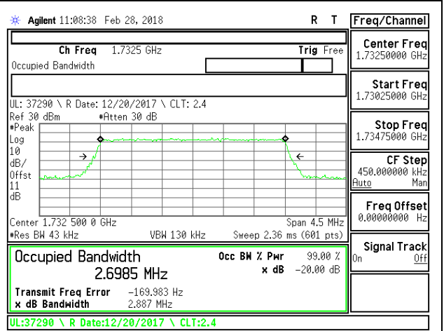
LTE B4 3MHz 16QAM Mid Channel RB15-0
