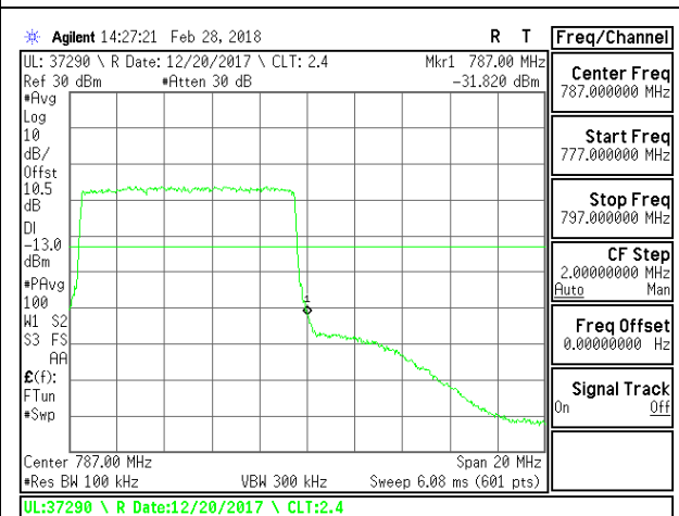
LTE B13 10MHz QPSK High Channel RB50-0
