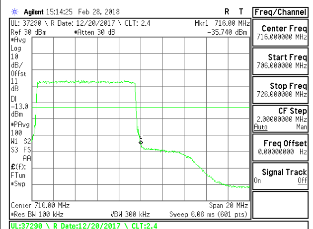
LTE B17 10MHz 16QAM High Channel RB50-0
