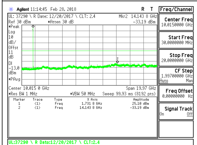
LTE B4 1.4MHz QPSK Middle Channel RB1-0
