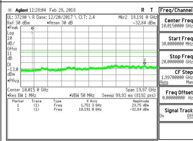
LTE B4 5MHz 16QAM High Channel RB1-0
