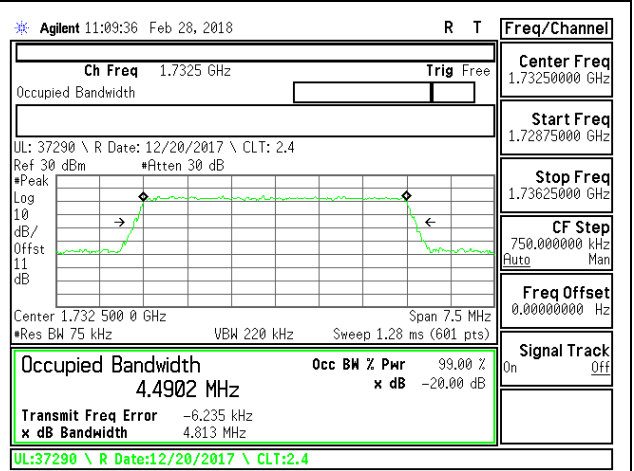
LTE B4 5MHz 16QAM Mid Channel RB25-0
