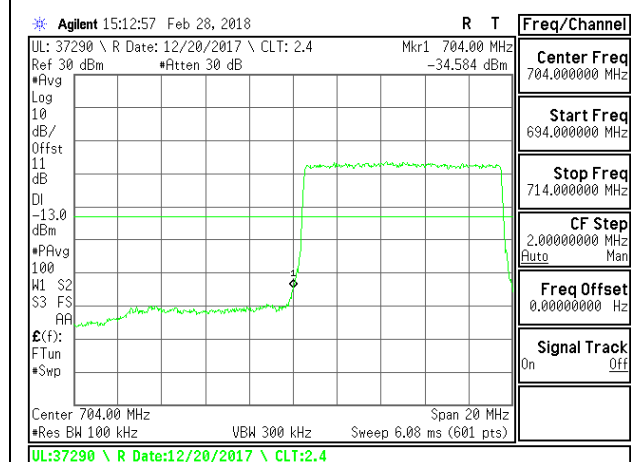
LTE B17 10MHz 16QAM Low Channel RB50-0
