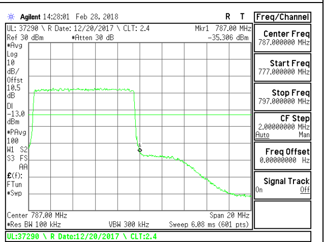
LTE B13 10MHz 16QAM High Channel RB50-0
