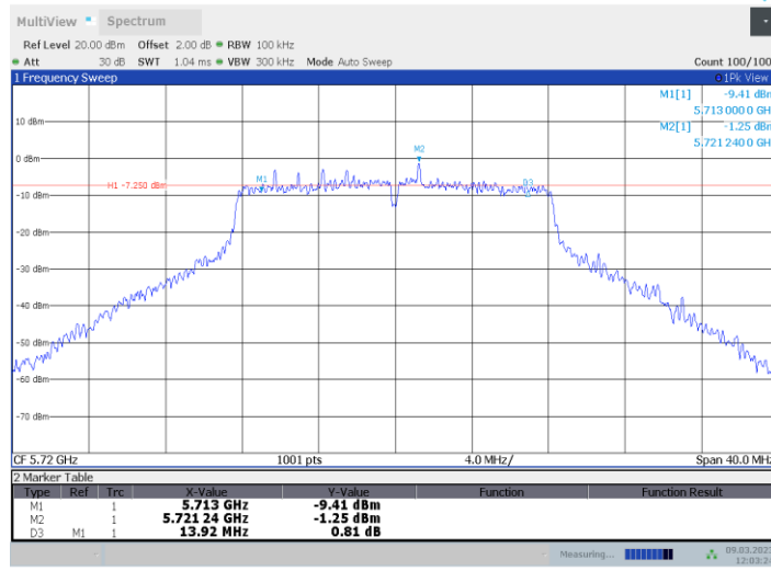
11AC20SISO_Ant1_5720_UNII-3
