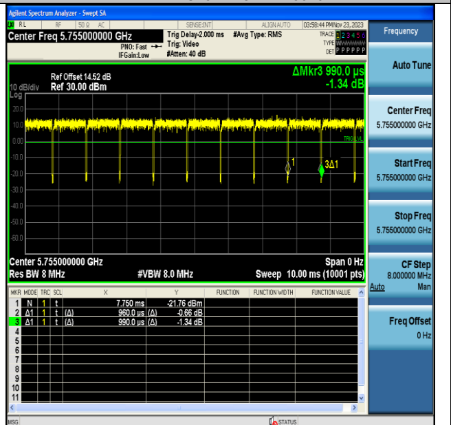
NTNV-11AC40MIMO-Ant7-5755
