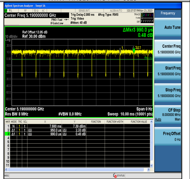
NTNV-11AC20MIMO-Ant7-5190
