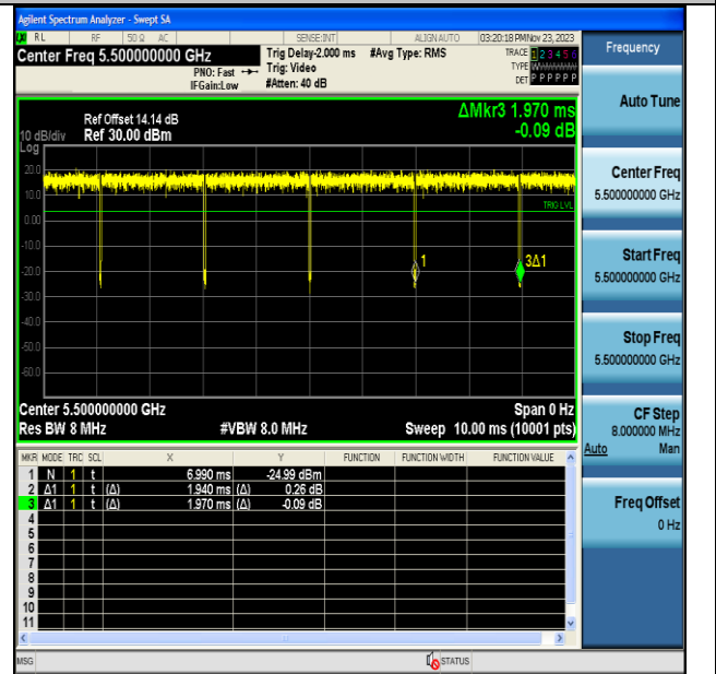
NTNV-11AC20MIMO-Ant7-5500
