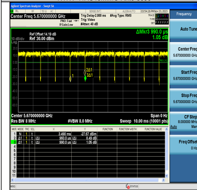
NTNV-11AC40MIMO-Ant6-5670
