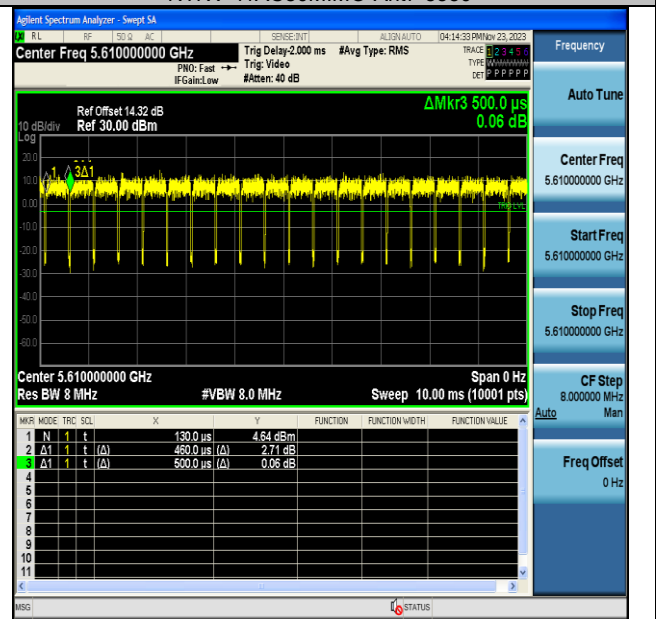
NTNV-11AC80MIMO-Ant7-5610
