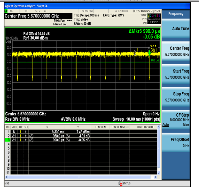
NTNV-11AC40MIMO-Ant7-5670
