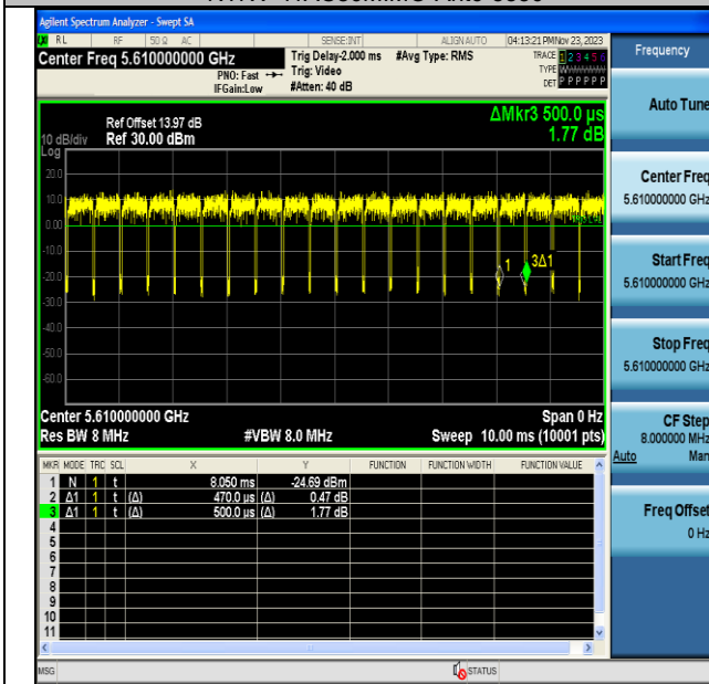
NTNV-11AC80MIMO-Ant6-5610
