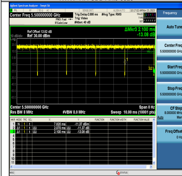
NTNV-11A-CDD-Ant6-5500
