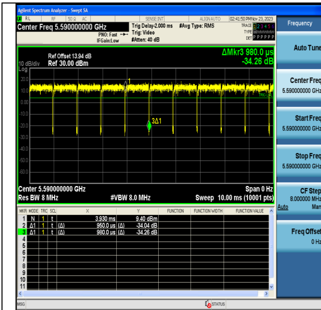
NTVN-11N40MIMO-Ant6-5590
