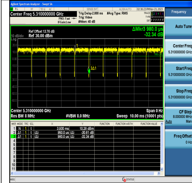
NTVN-11N40MIMO-Ant6-5310
