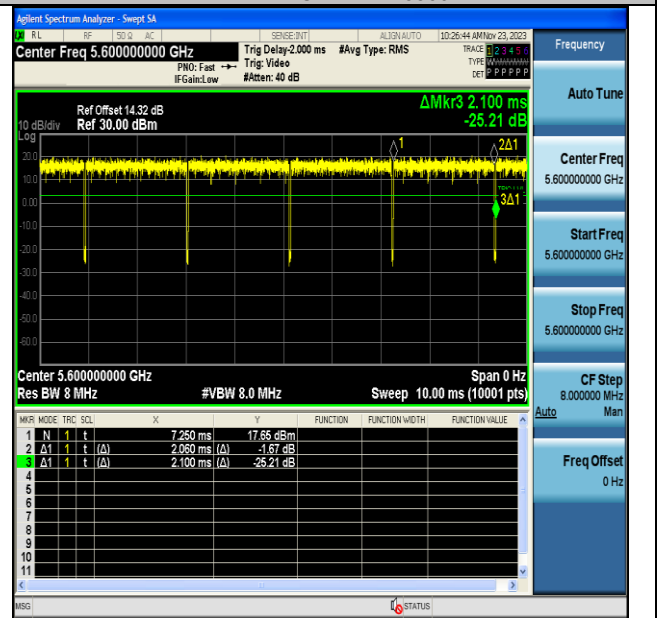
NTNV-11A-CDD-Ant7-5600
