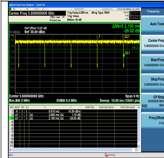
NTNV-11A-CDD-Ant6-5600
