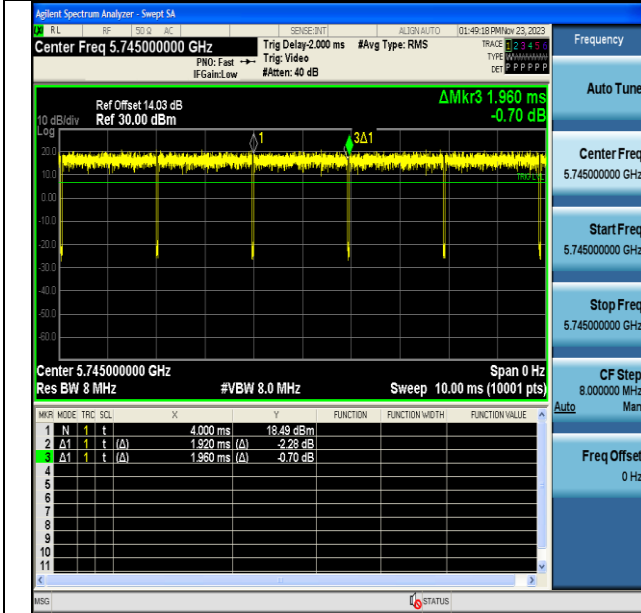
NTVN-11N20MIMO-Ant6-5745
