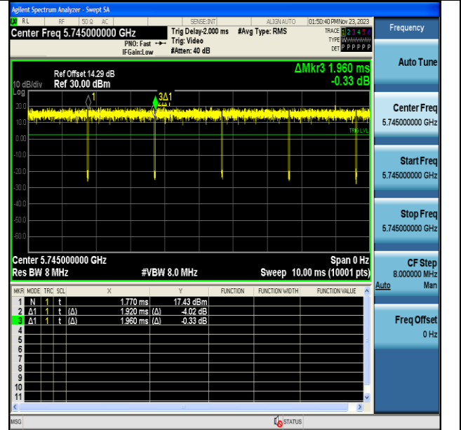
NTVN-11N20MIMO-Ant7-5745
