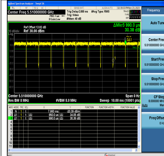
NTVN-11N40MIMO-Ant6-5510
