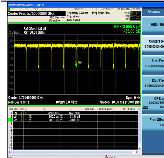
NTVN-11N40MIMO-Ant6-5755
