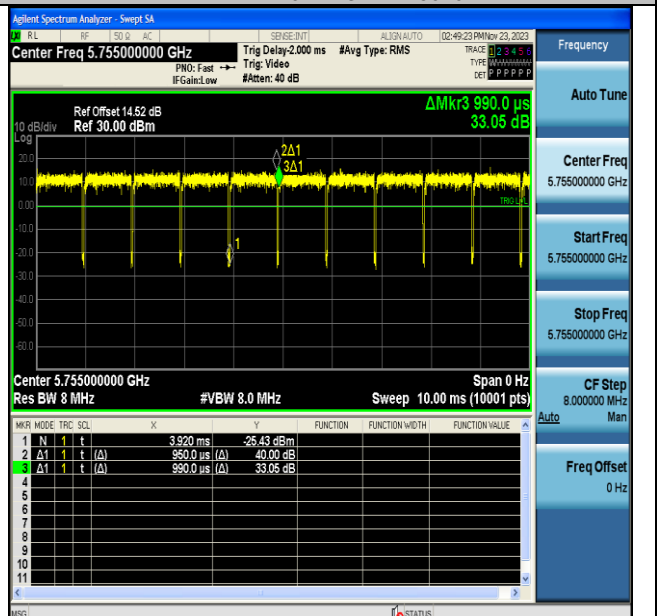
NTVN-11N40MIMO-Ant7-5755
