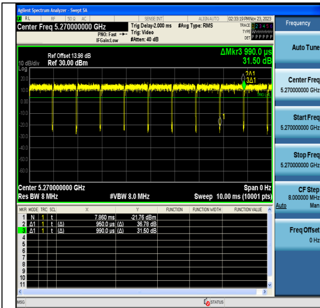
NTVN-11N40MIMO-Ant6-5270
