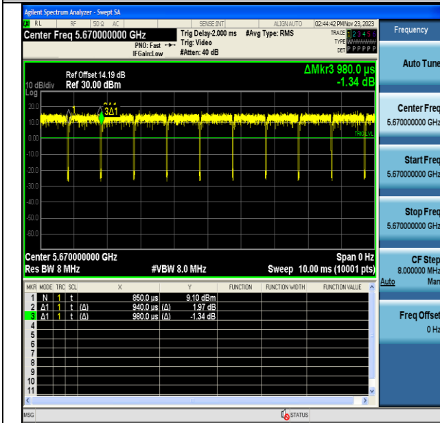
NTVN-11N40MIMO-Ant6-5670
