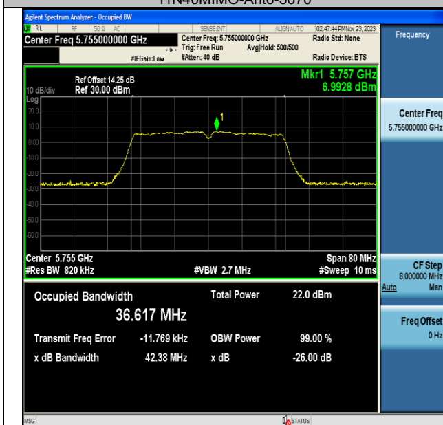
11N40MIMO-Ant6-5755
