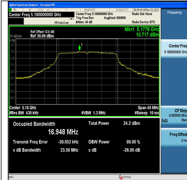
11A-CDD-Ant6-5180
