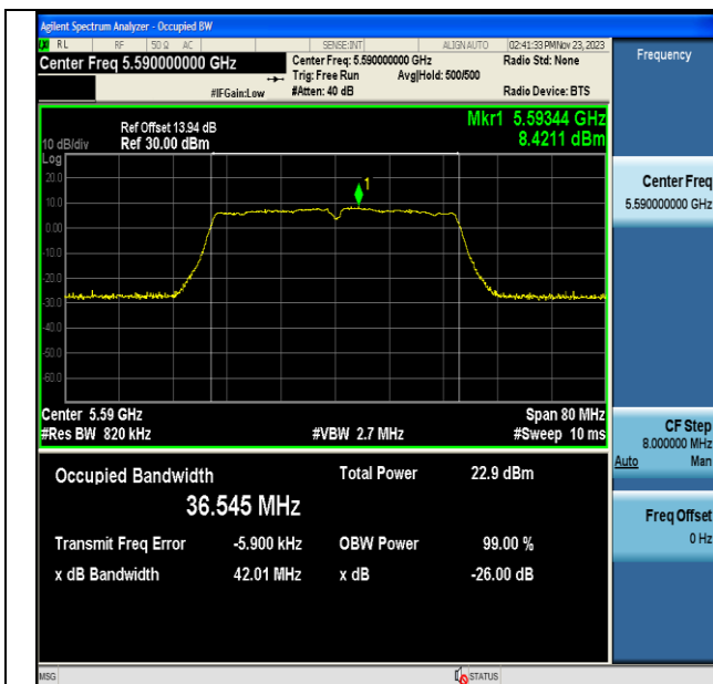
11N40MIMO-Ant6-5590
