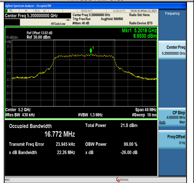
11A-CDD-Ant7-5200
