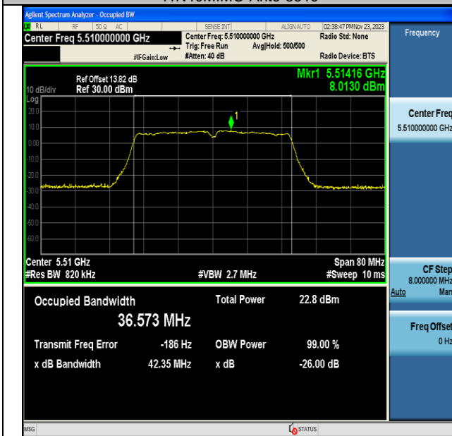
11N40MIMO-Ant6-5510
