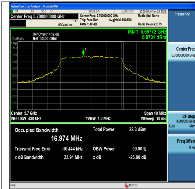
11A-CDD-Ant6-5700
