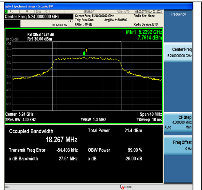
11AC20MIMO-Ant7-5240
