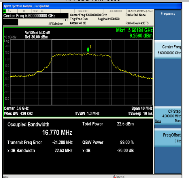
11A-CDD-Ant7-5600
