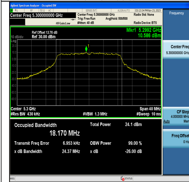
11AC20MIMO-Ant6-5300
