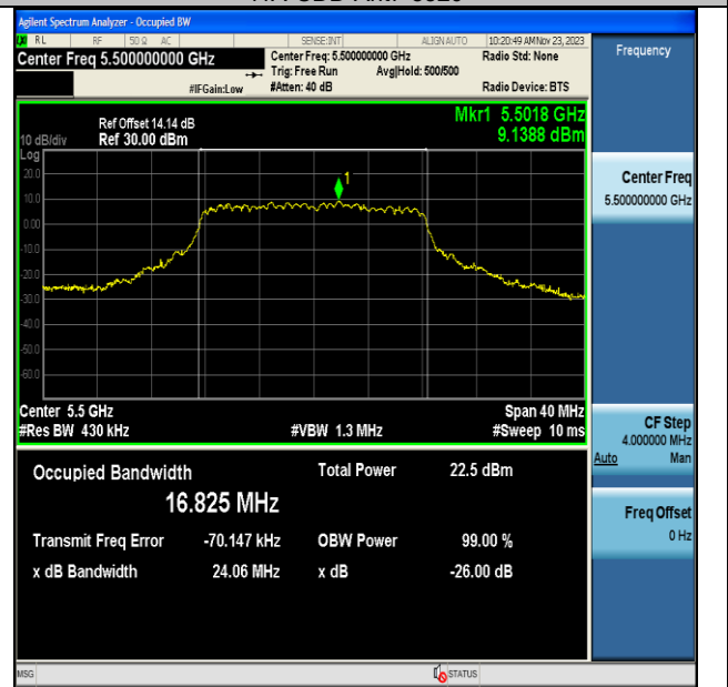
11A-CDD-Ant7-5500
