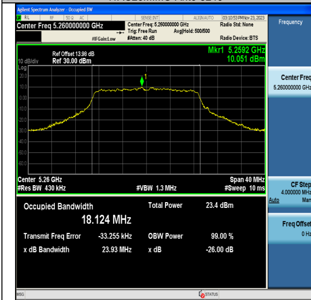
11AC20MIMO-Ant6-5260
