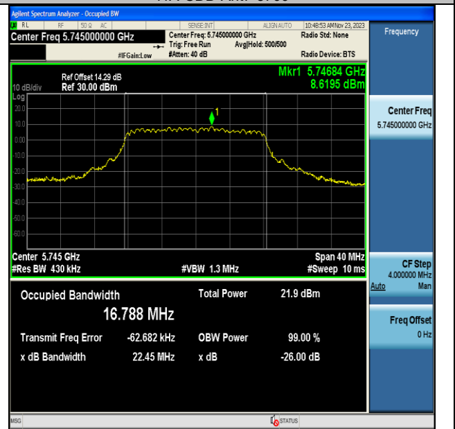
11A-CDD-Ant7-5745
