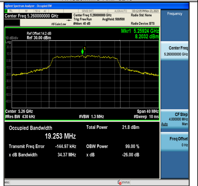
11AC20MIMO-Ant7-5260
