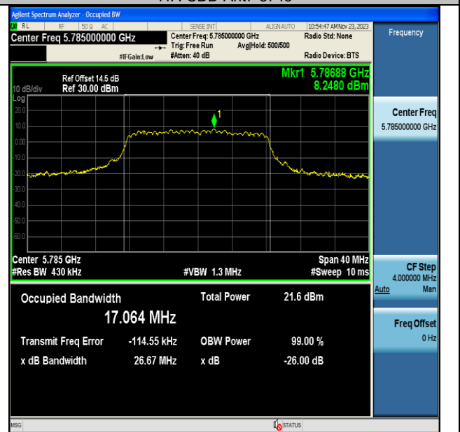
11A-CDD-Ant7-5785
