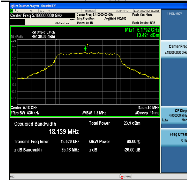
11N20MIMO-Ant6-5180
