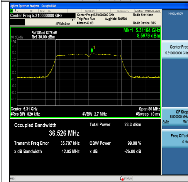
11N40MIMO-Ant6-5310
