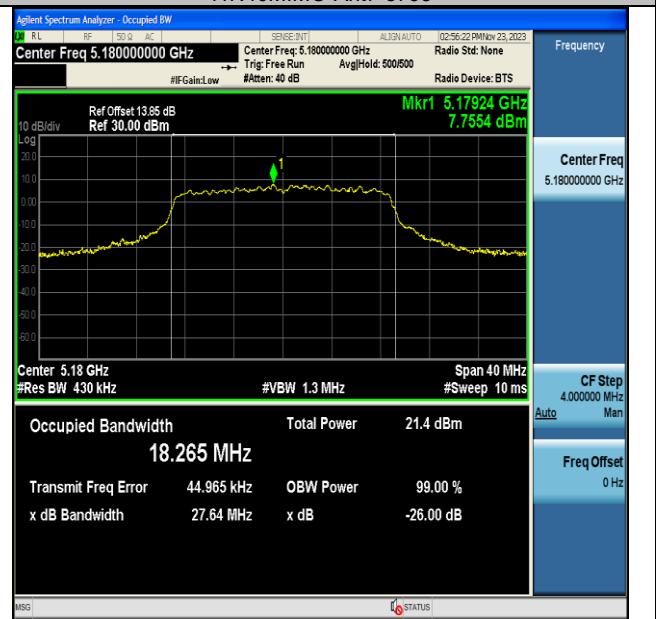
11AC20MIMO-Ant7-5180
