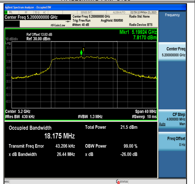
11AC20MIMO-Ant7-5200
