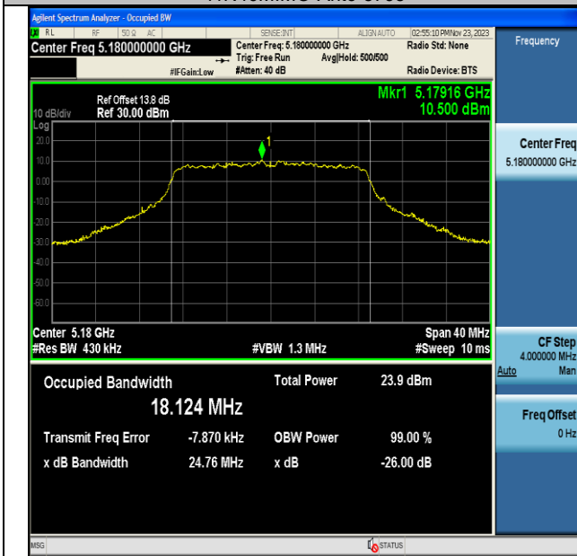
11AC20MIMO-Ant6-5180
