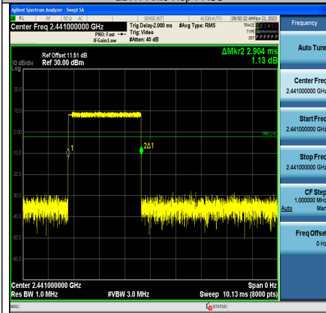
2DH5-Ant6-Hop-PASS
