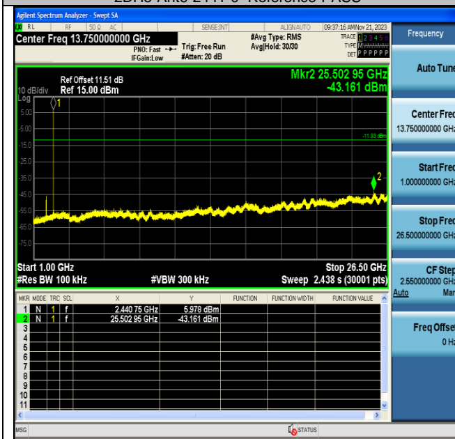
2DH5-Ant6-2441-1000~26500-PASS
