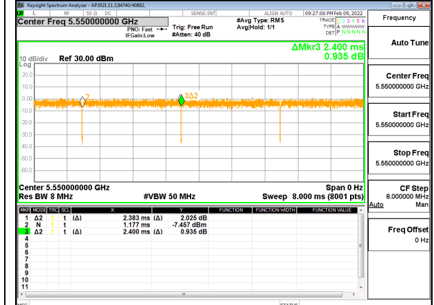
802.11ax HE40 OFDMA, RU size 484T MODE
