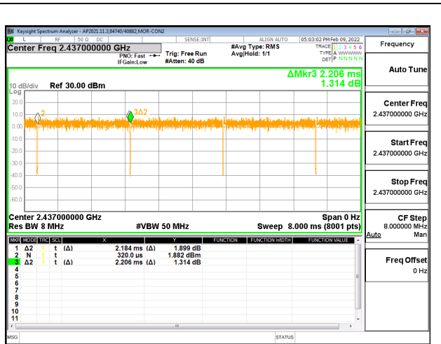
802.11ax HE20 OFDMA, RU index 106T MODE,2TX
