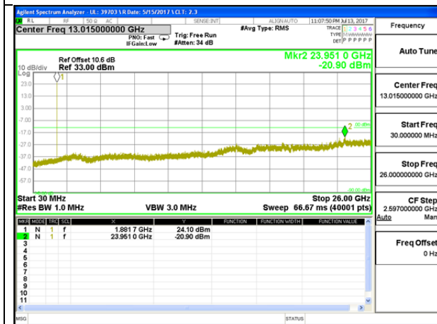
LTE B25 3MHz QPSK Middle Channel
