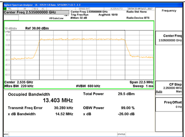
LTE B7 15MHz 16QAM Middle Channel
