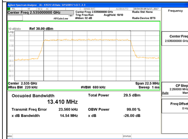
LTE B7 15MHz QPSK Middle Channel
